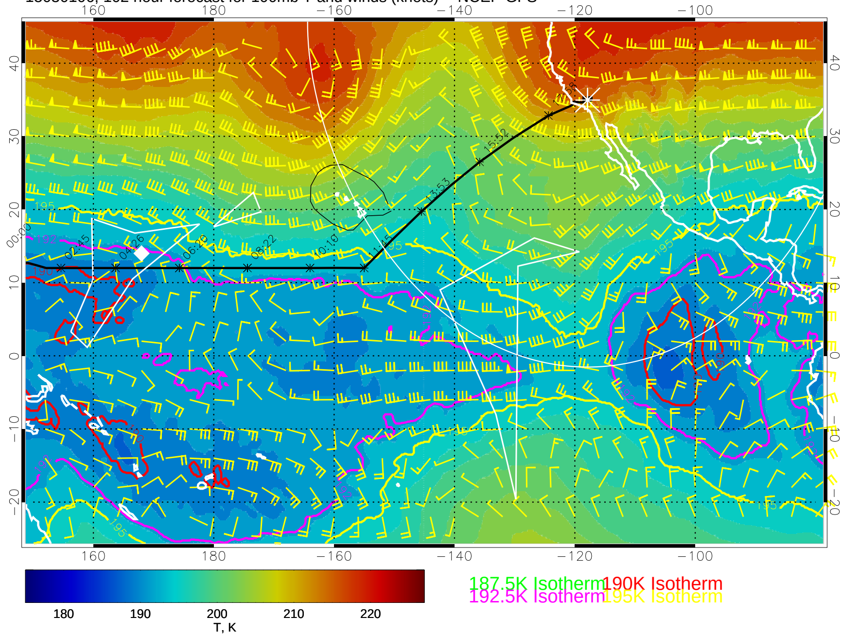
15030106, 102 hour forecast for 100mb T and winds (knots) -- NCEP GFS
