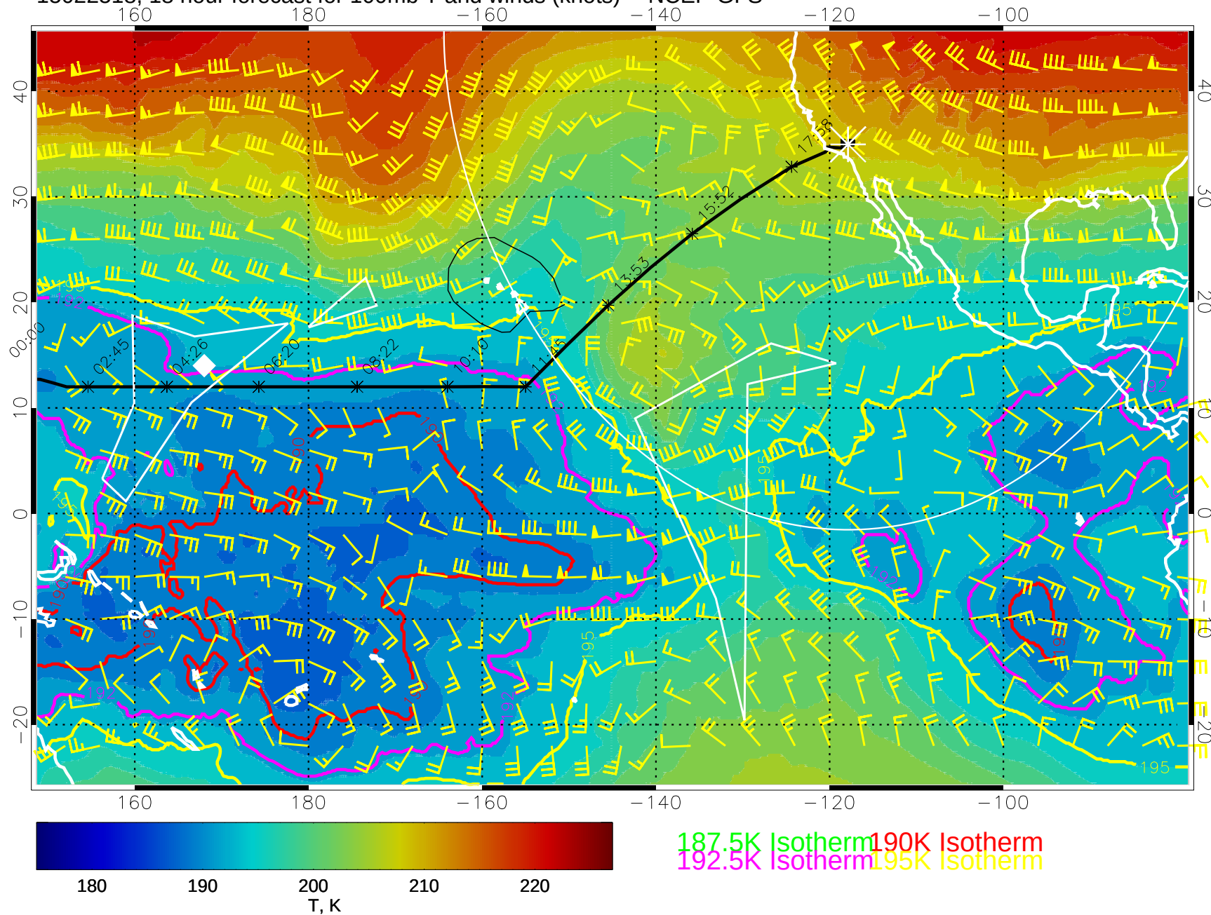
15022518, 18 hour forecast for 100mb T and winds (knots) -- NCEP GFS
