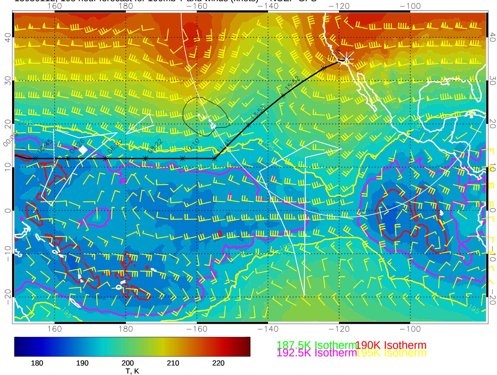
15030112, 108 hour forecast for 100mb T and winds (knots) -- NCEP GFS
