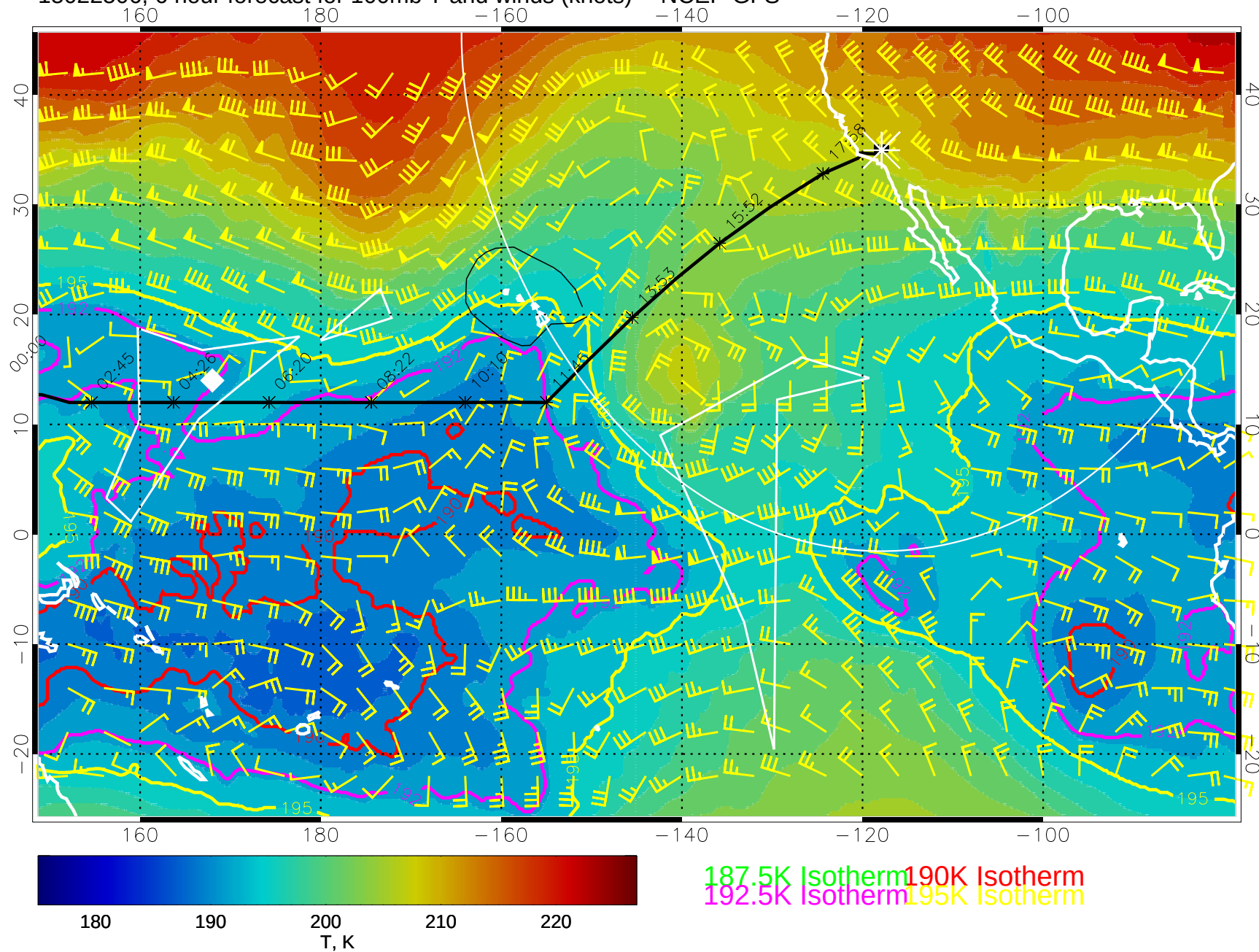
15022506, 6 hour forecast for 100mb T and winds (knots) -- NCEP GFS
