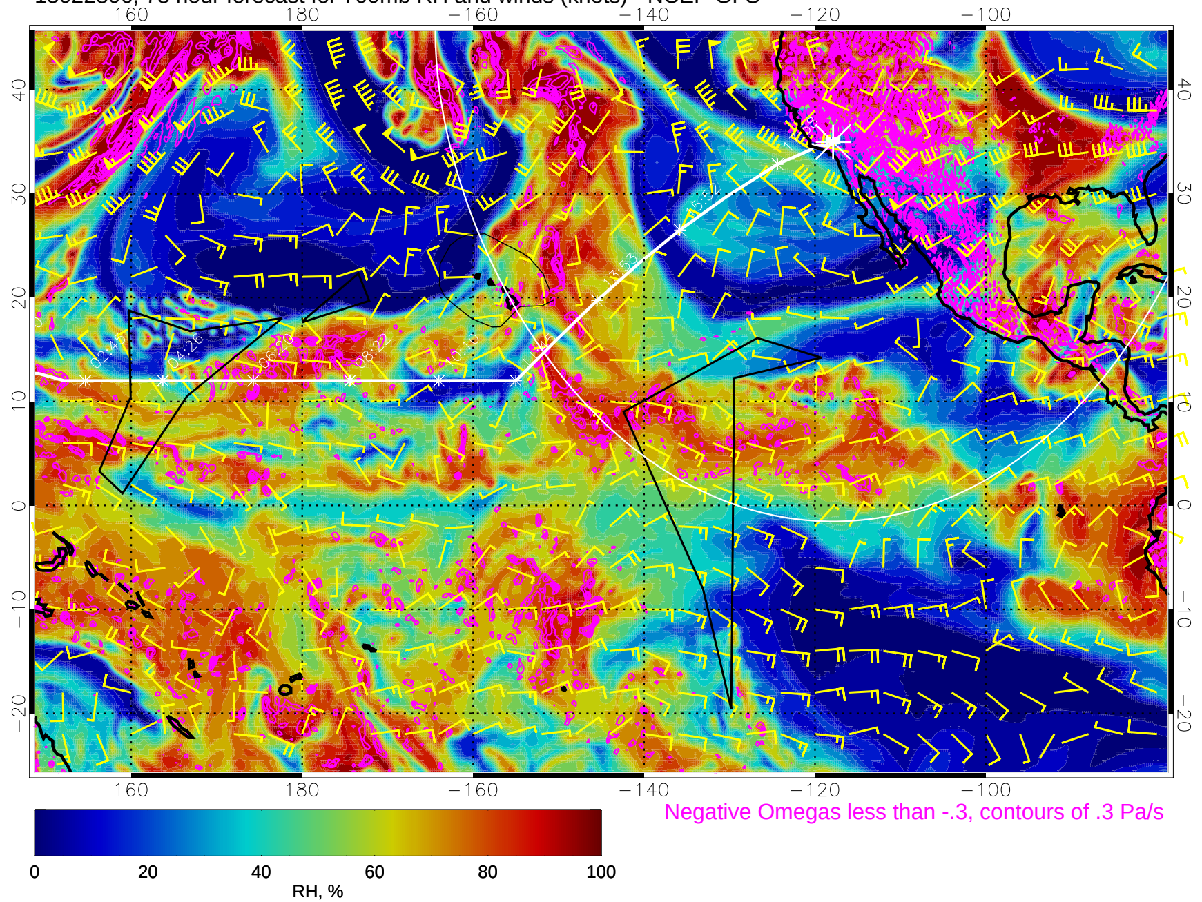
15022806, 78 hour forecast for 700mb RH and winds (knots) - NCEP GFS
