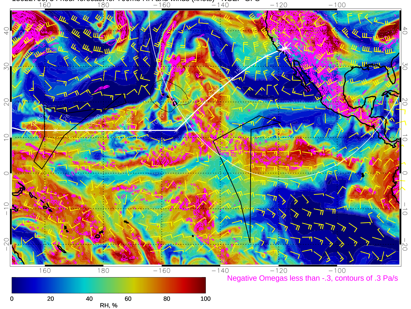
15022706, 54 hour forecast for 700mb RH and winds (knots) - NCEP GFS
