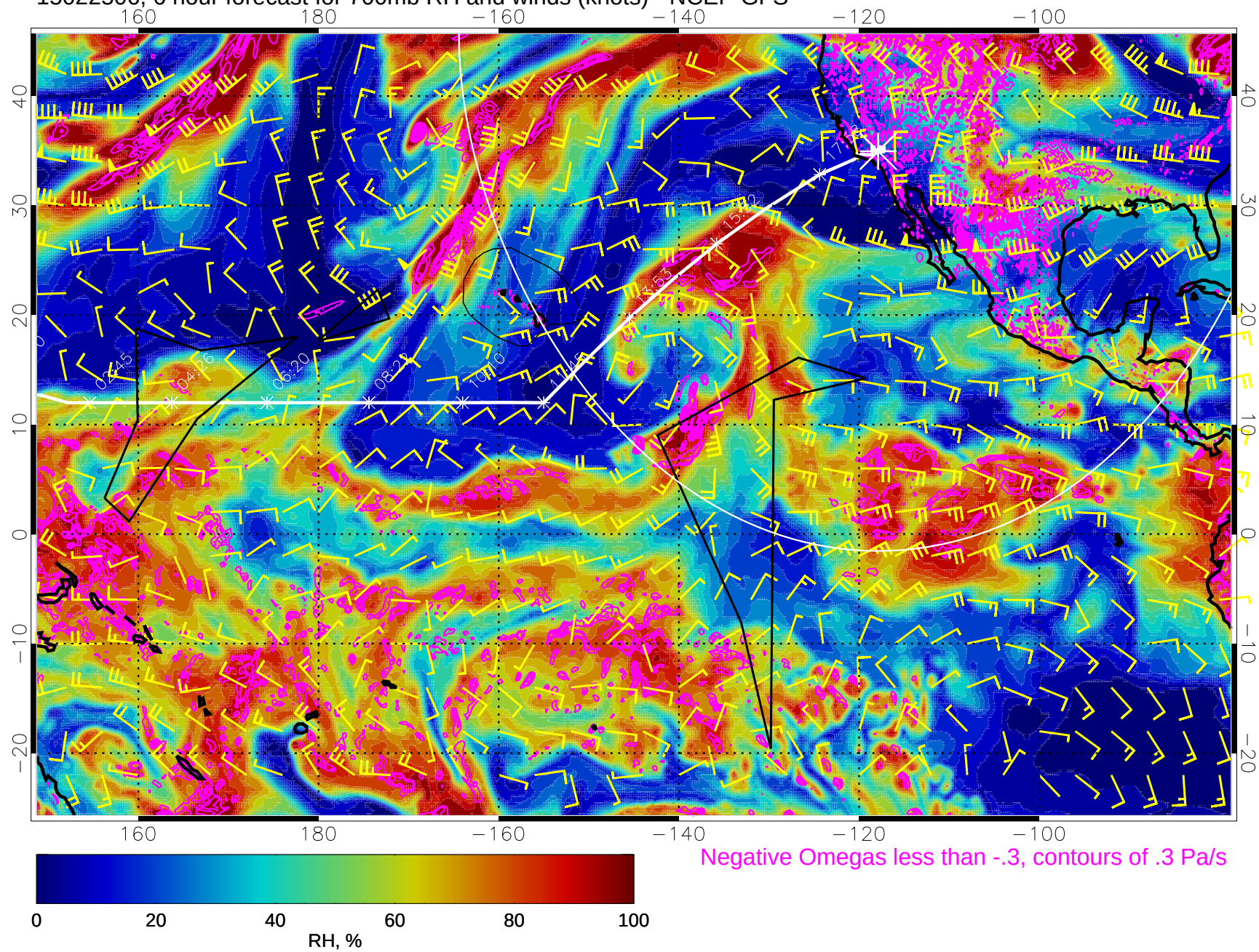
15022506, 6 hour forecast for 700mb RH and winds (knots) - NCEP GFS
