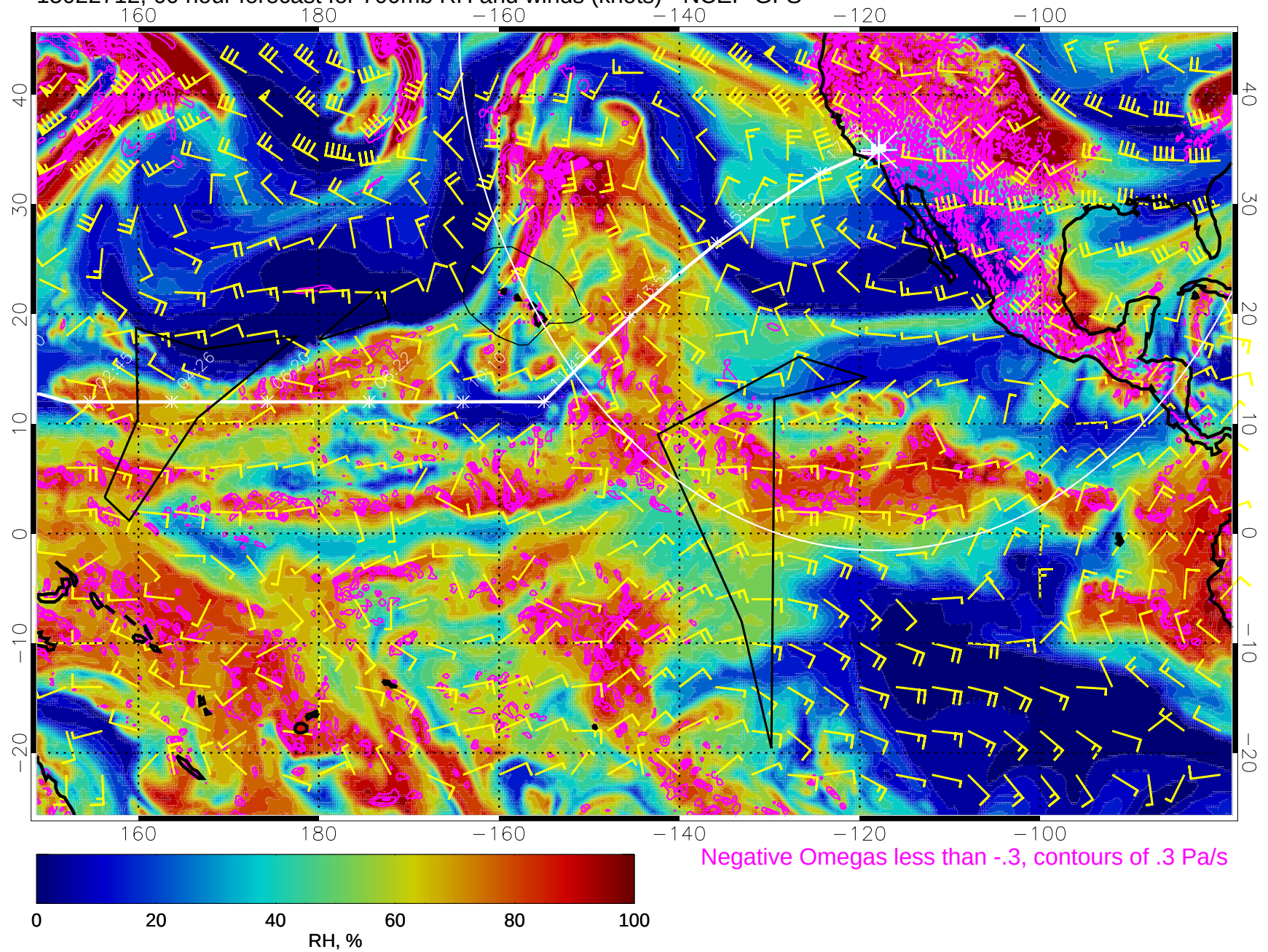
15022712, 60 hour forecast for 700mb RH and winds (knots) - NCEP GFS
