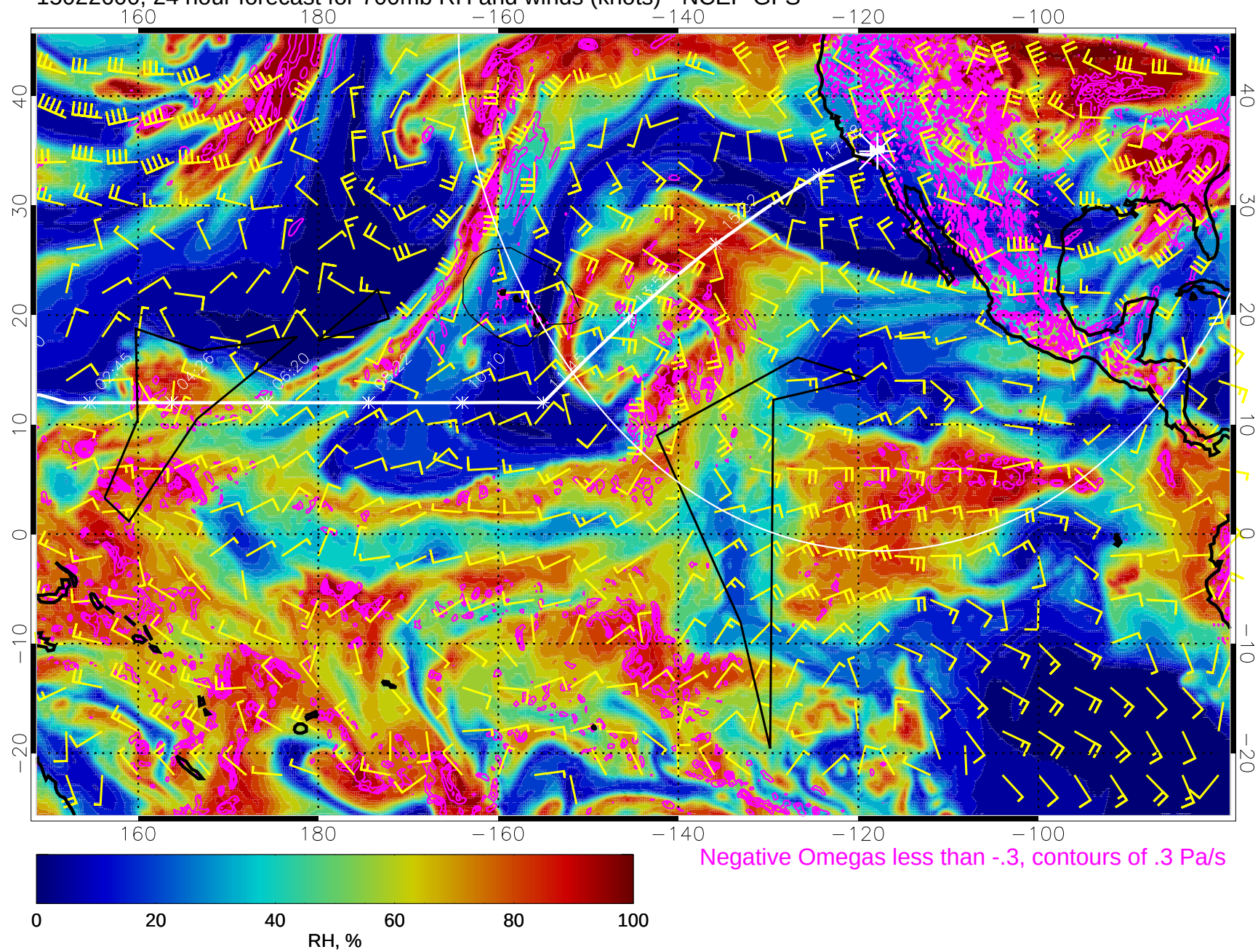
15022600, 24 hour forecast for 700mb RH and winds (knots) - NCEP GFS
