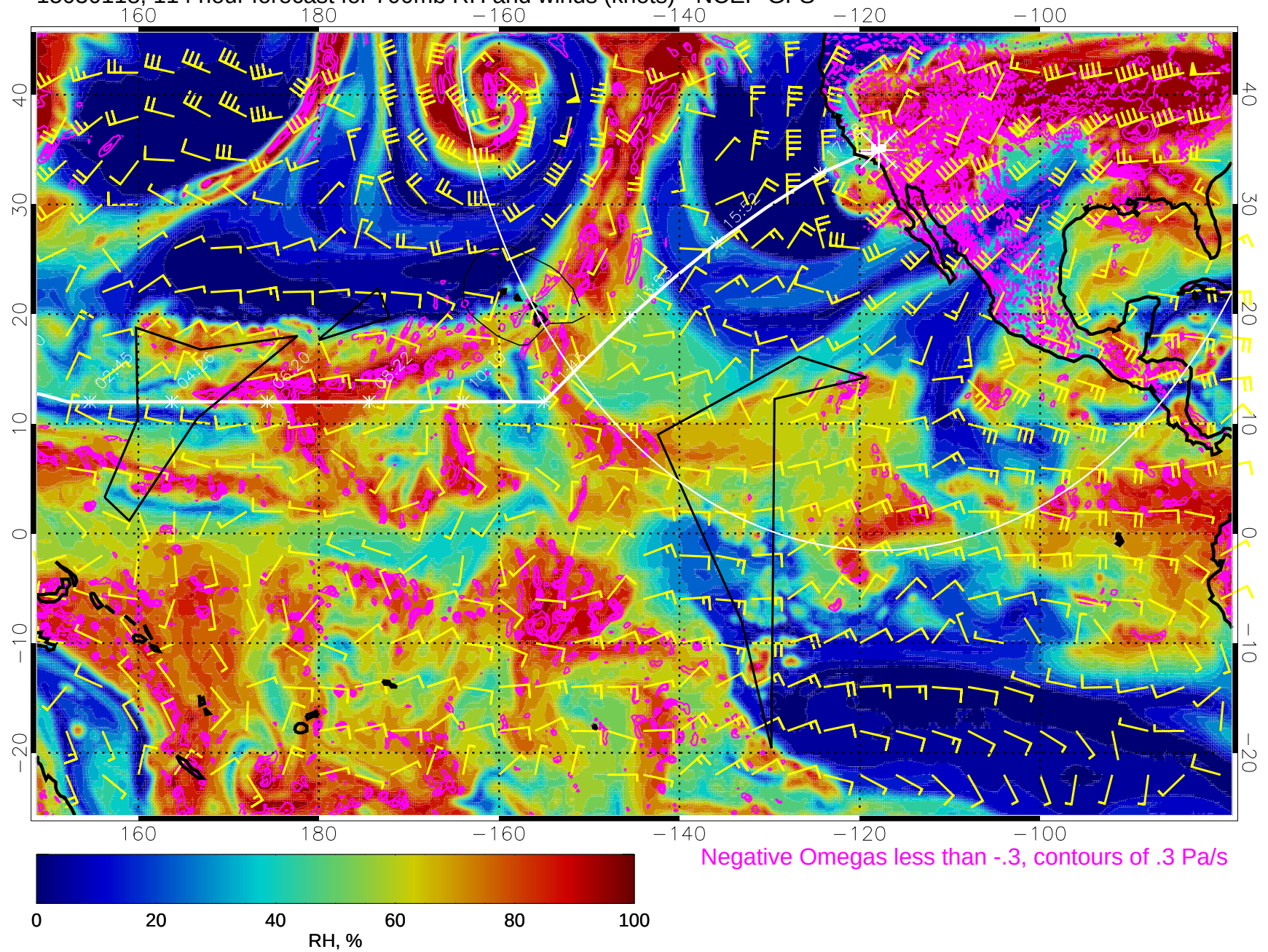
15030118, 114 hour forecast for 700mb RH and winds (knots) - NCEP GFS
