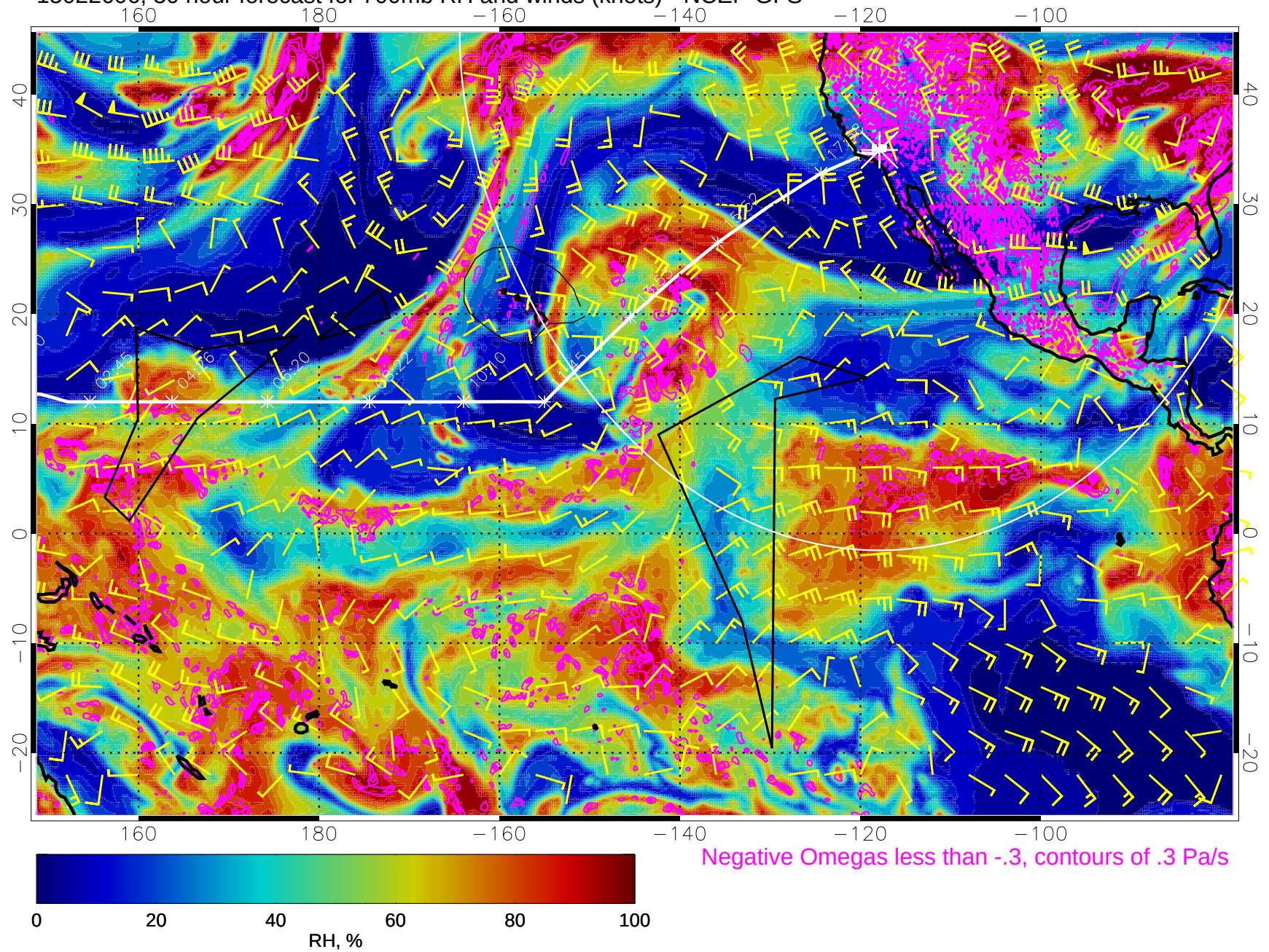
15022606, 30 hour forecast for 700mb RH and winds (knots) - NCEP GFS
