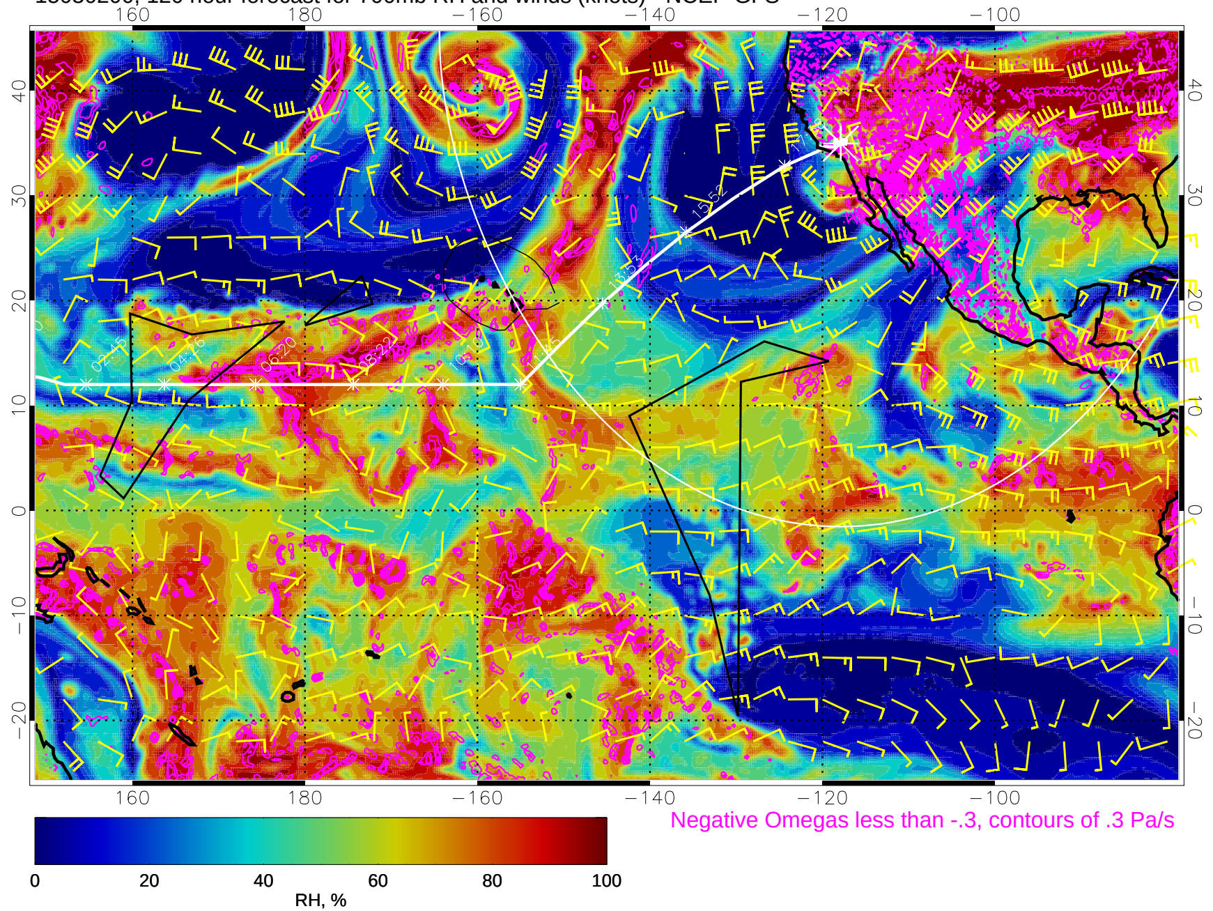
15030200, 120 hour forecast for 700mb RH and winds (knots) - NCEP GFS
