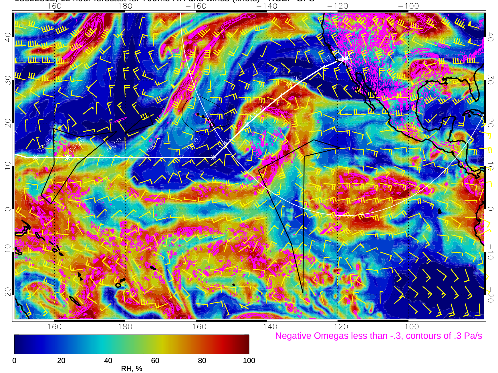
15022512, 12 hour forecast for 700mb RH and winds (knots) - NCEP GFS
