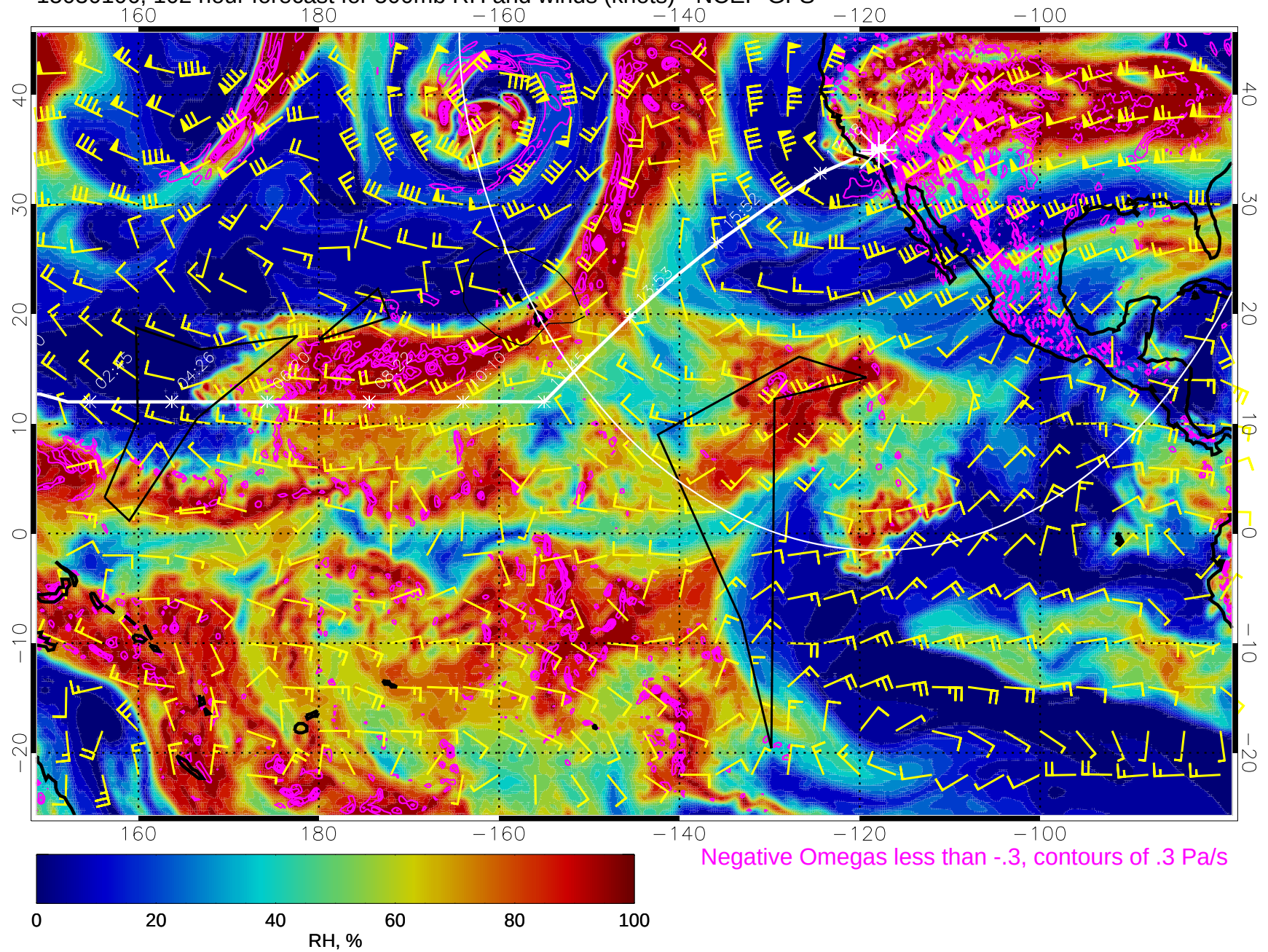
15030106, 102 hour forecast for 500mb RH and winds (knots) - NCEP GFS
