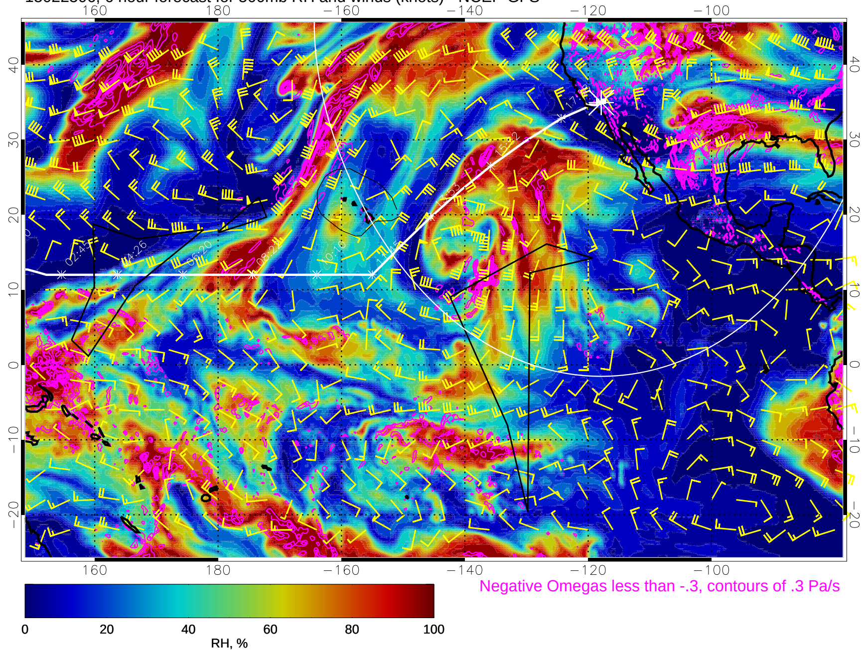
15022506, 6 hour forecast for 500mb RH and winds (knots) - NCEP GFS
