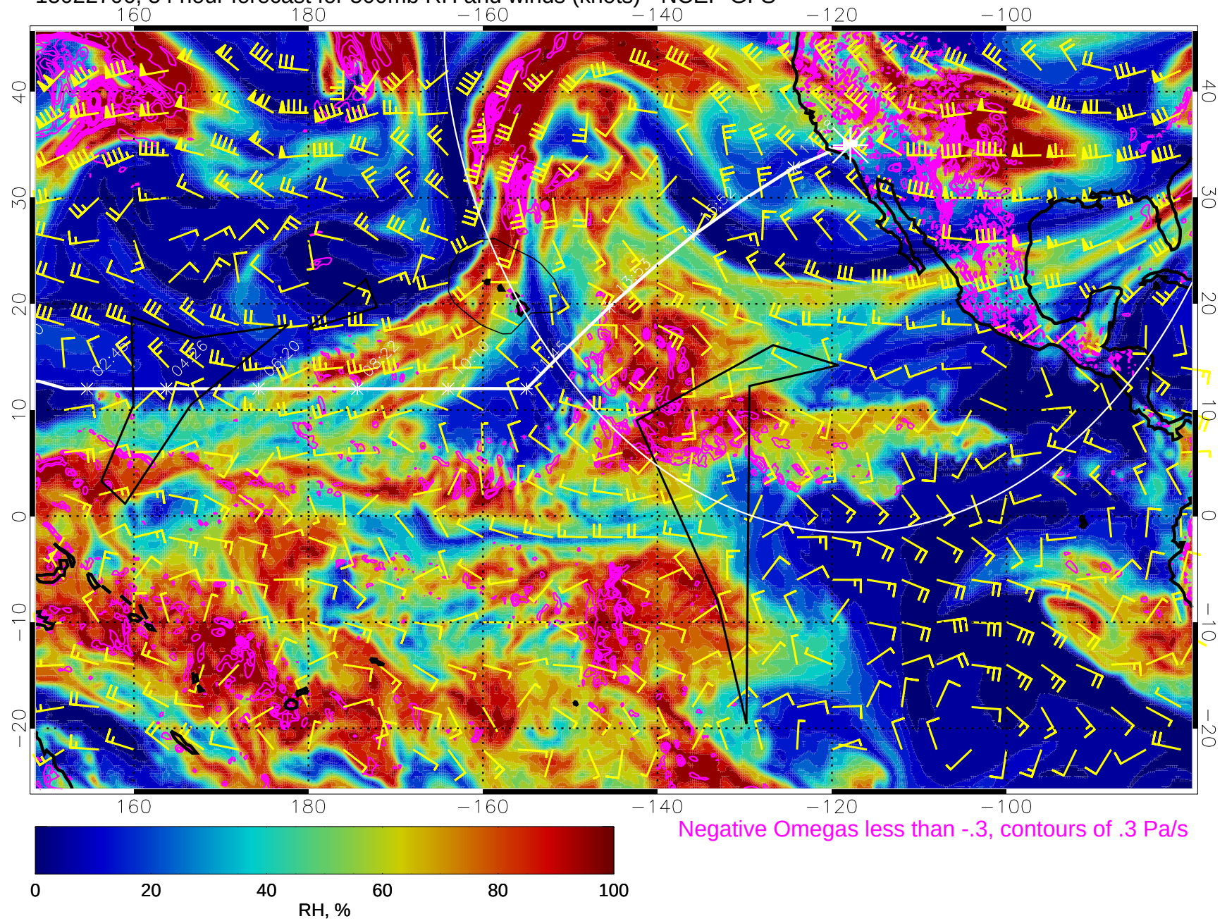
15022706, 54 hour forecast for 500mb RH and winds (knots) - NCEP GFS
