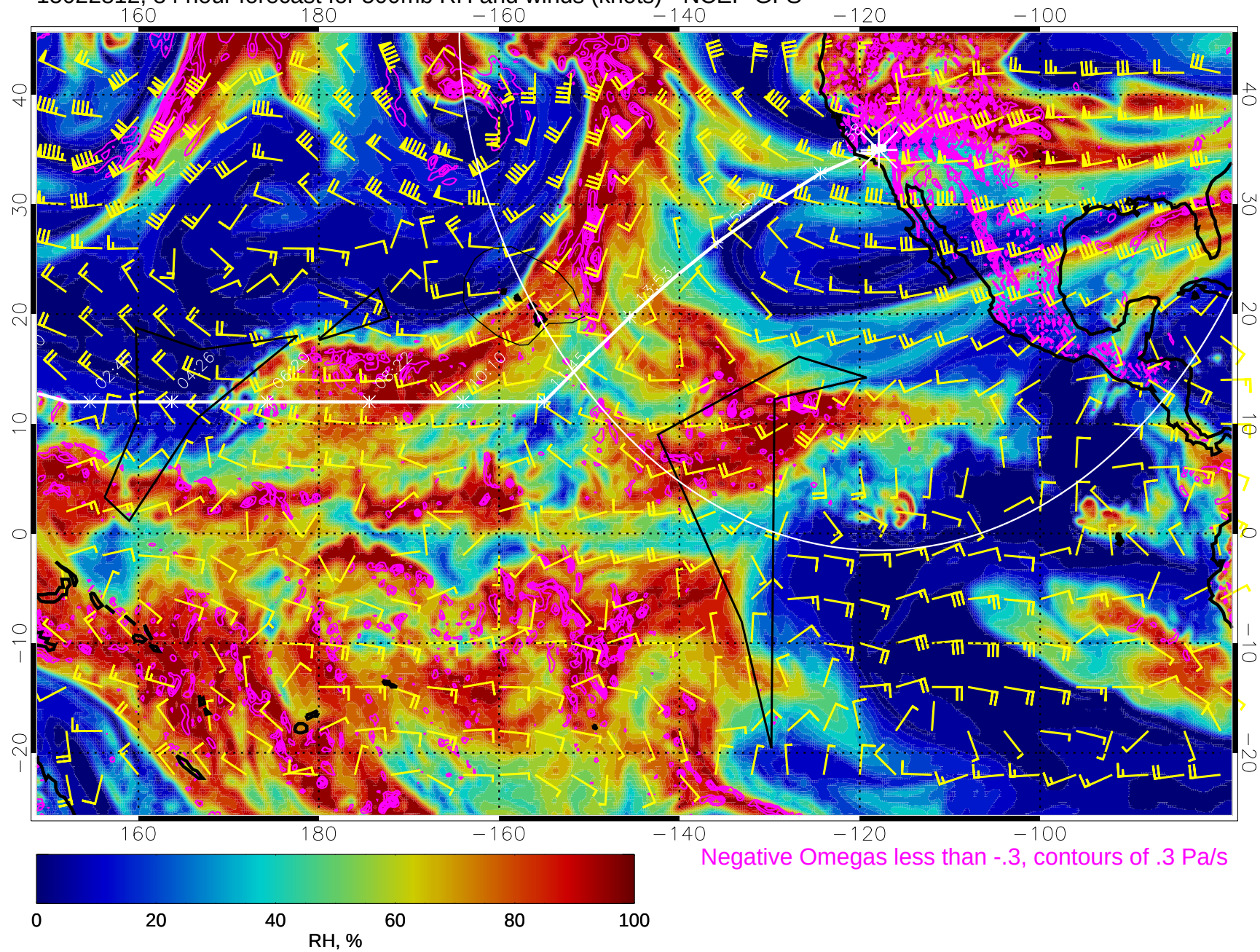
15022812, 84 hour forecast for 500mb RH and winds (knots) - NCEP GFS
