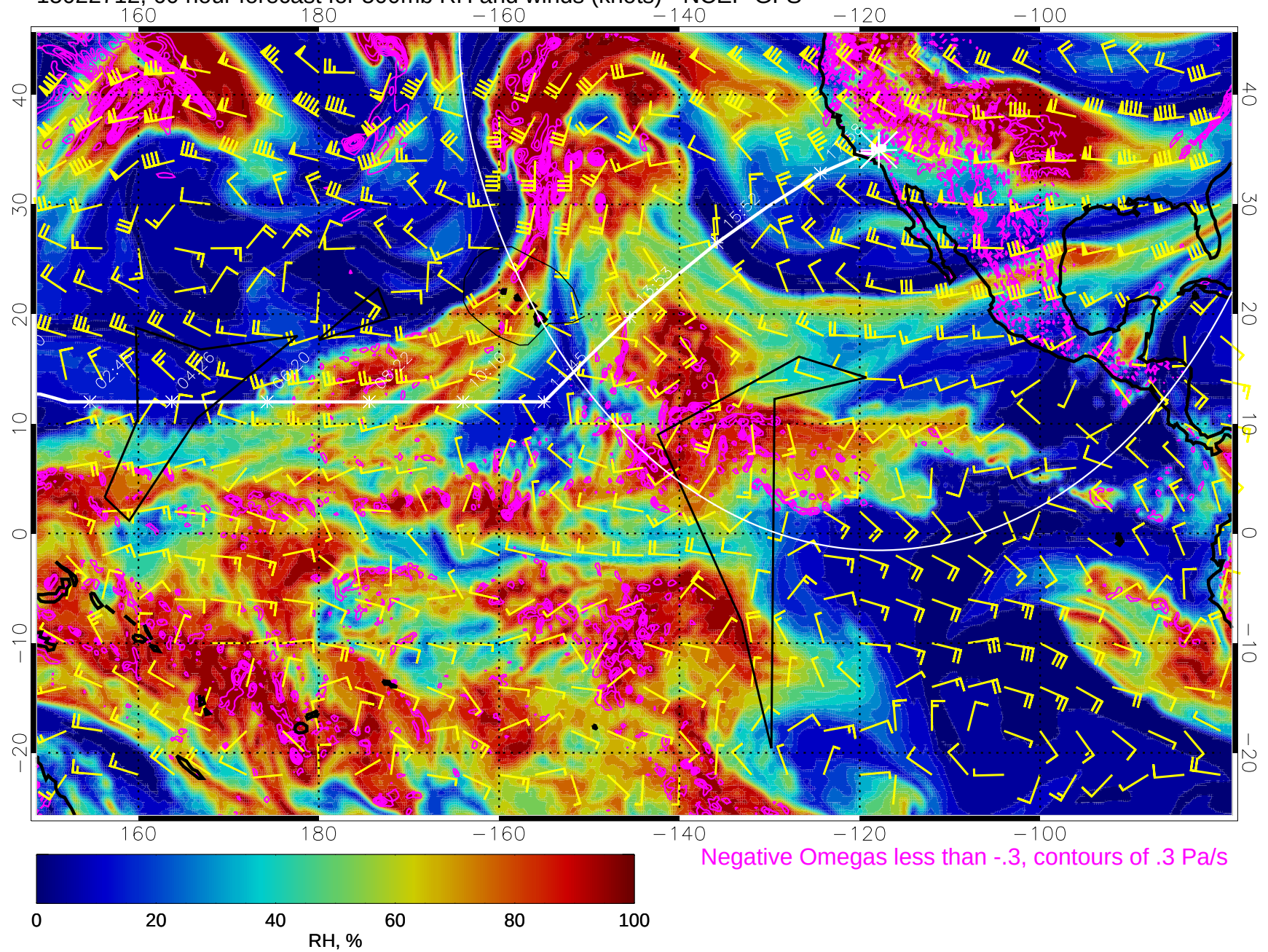
15022712, 60 hour forecast for 500mb RH and winds (knots) - NCEP GFS
