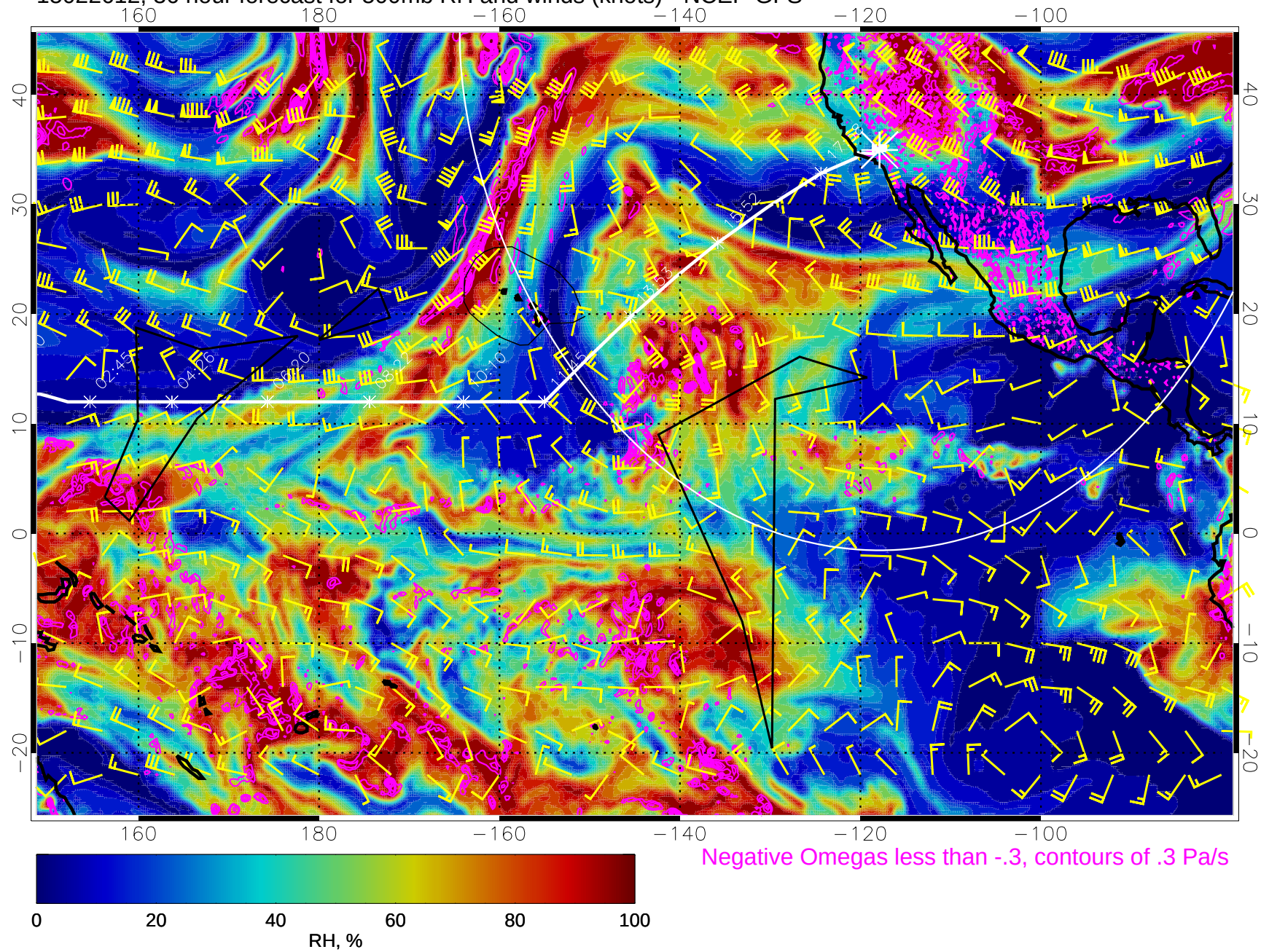
15022612, 36 hour forecast for 500mb RH and winds (knots) - NCEP GFS
