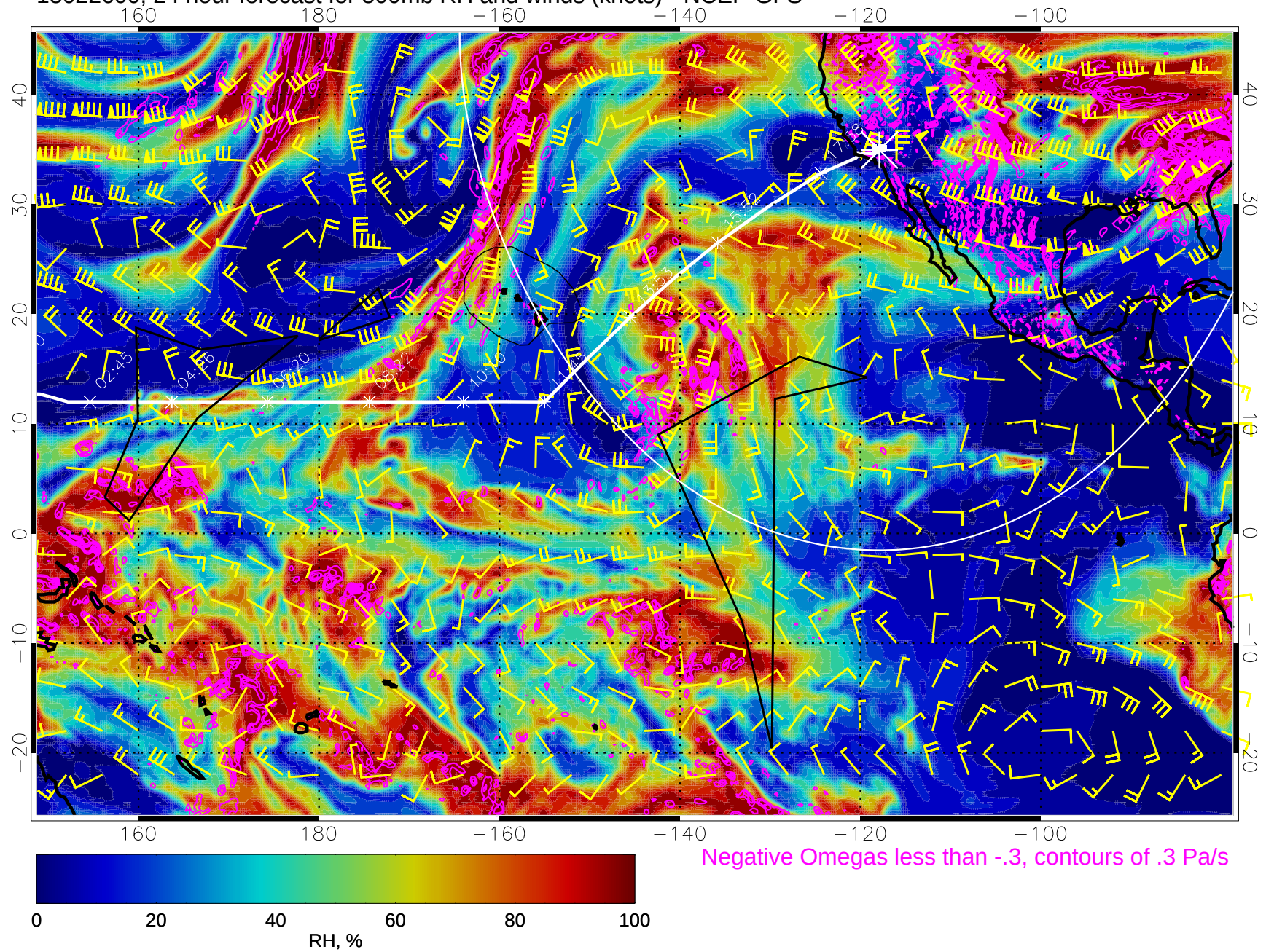
15022600, 24 hour forecast for 500mb RH and winds (knots) - NCEP GFS
