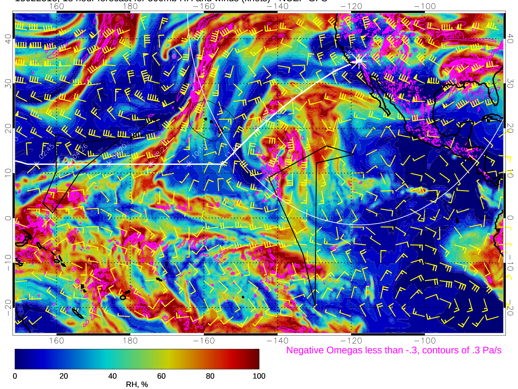
15022518, 18 hour forecast for 500mb RH and winds (knots) - NCEP GFS
