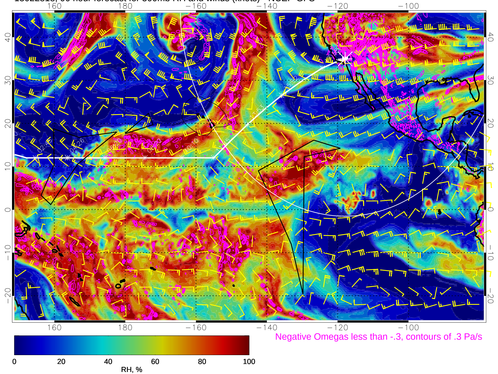
15022818, 90 hour forecast for 500mb RH and winds (knots) - NCEP GFS
