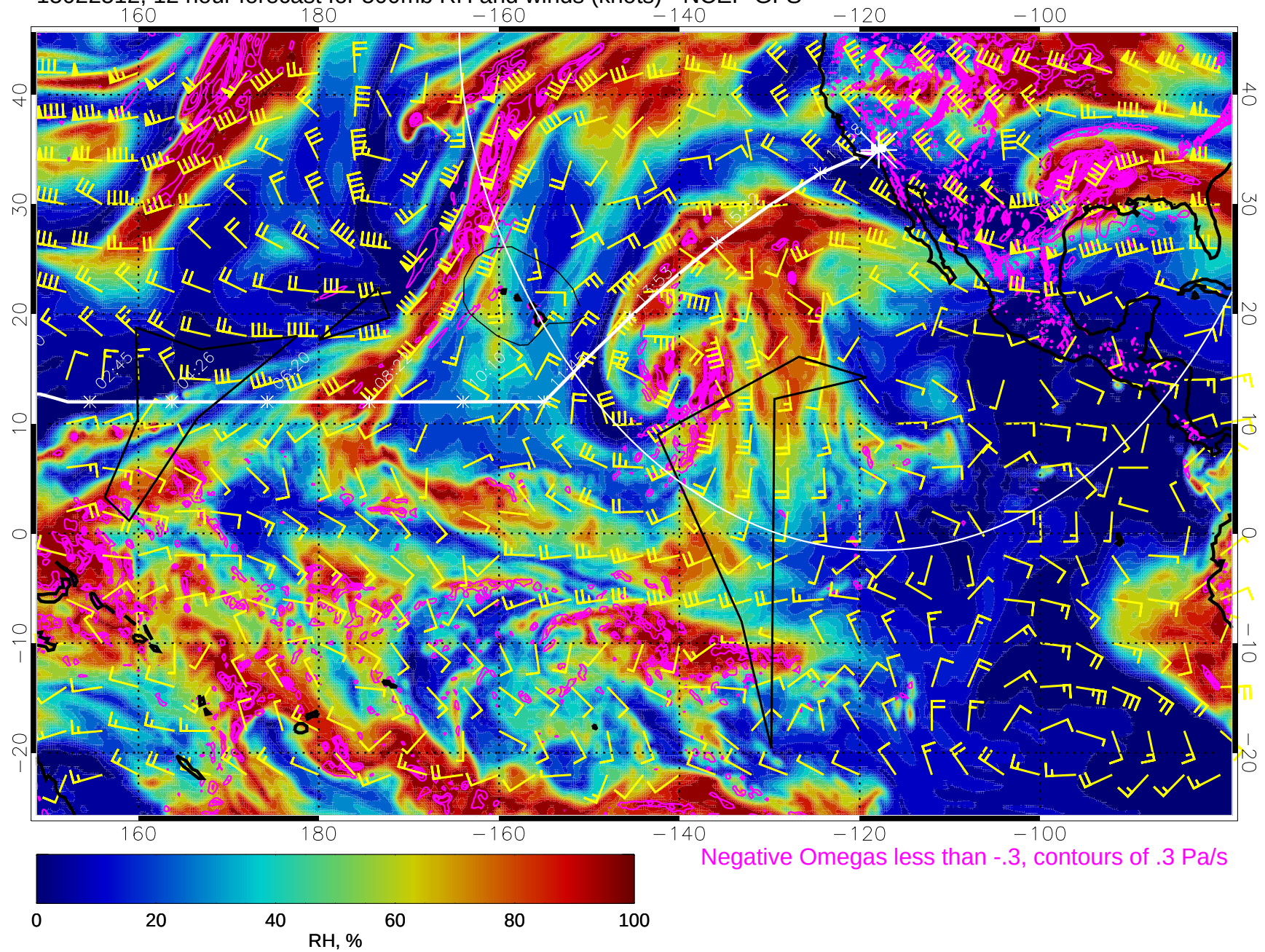
15022512, 12 hour forecast for 500mb RH and winds (knots) - NCEP GFS
