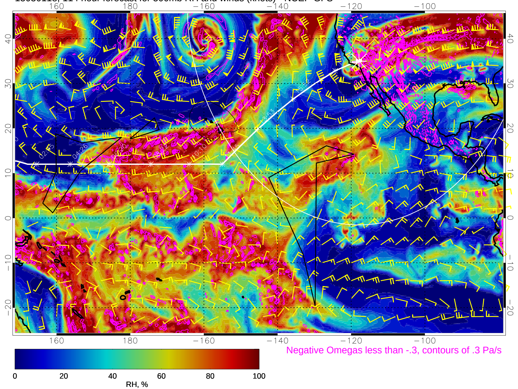
15030118, 114 hour forecast for 500mb RH and winds (knots) - NCEP GFS
