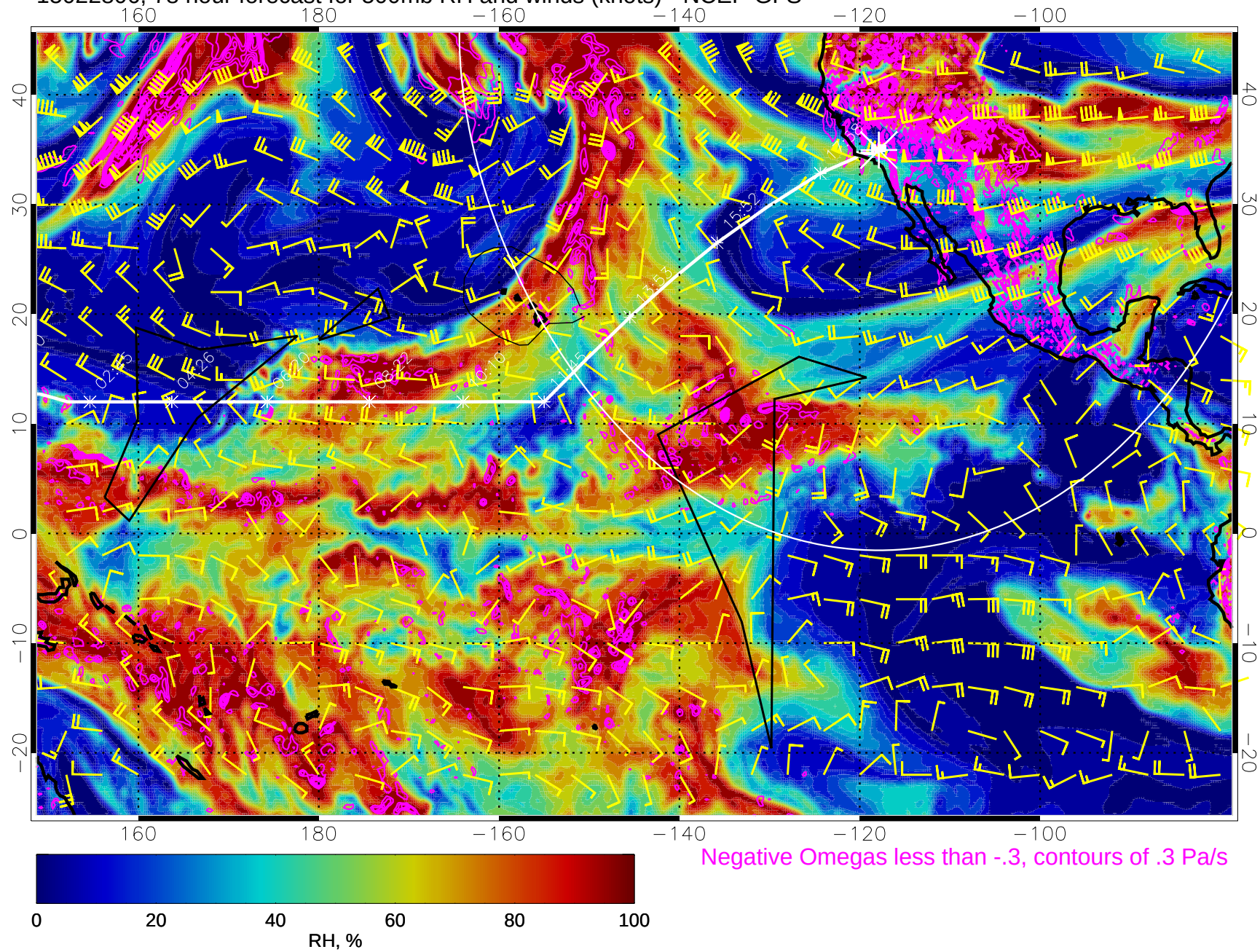
15022806, 78 hour forecast for 500mb RH and winds (knots) - NCEP GFS
