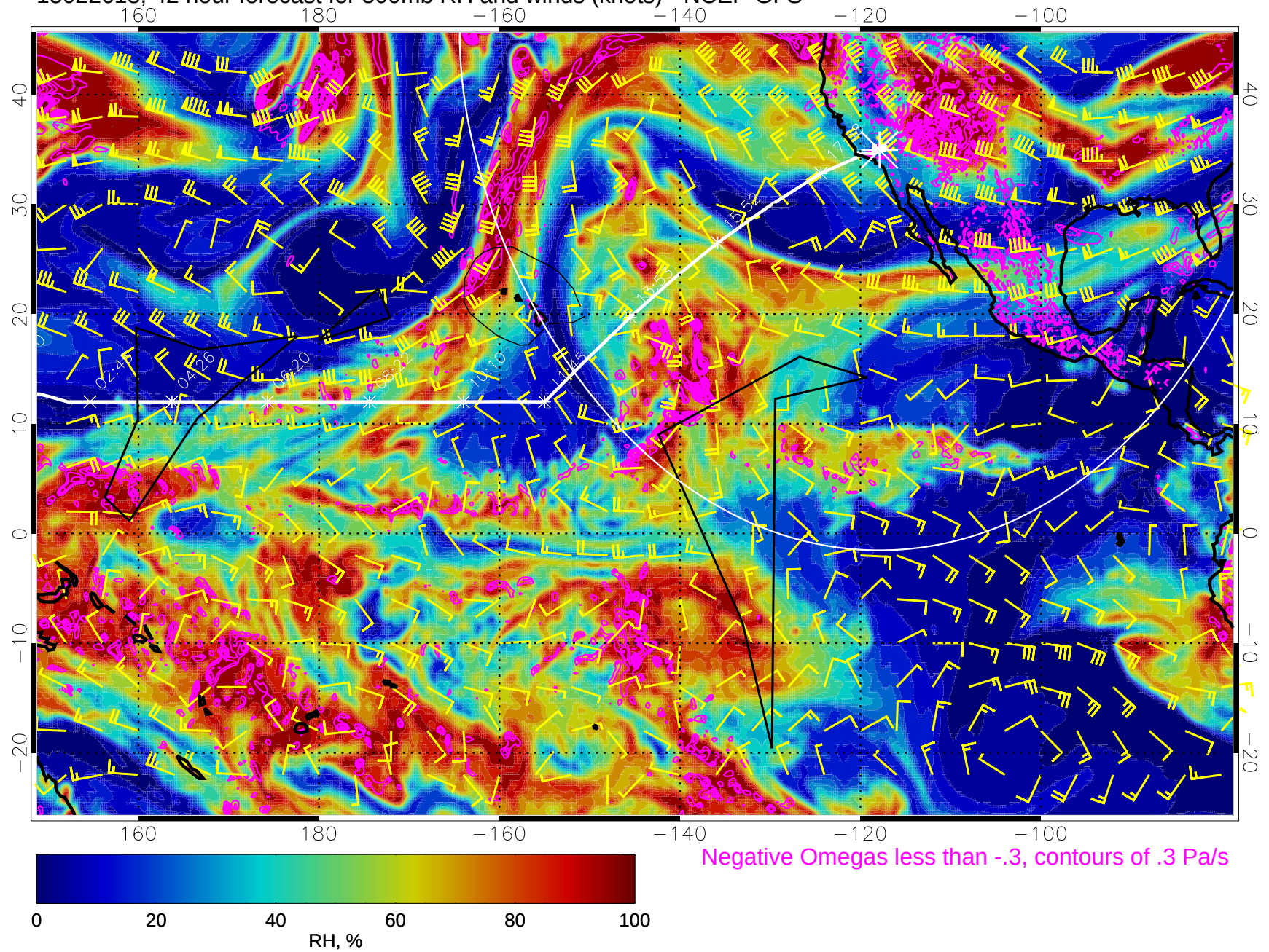
15022618, 42 hour forecast for 500mb RH and winds (knots) - NCEP GFS
