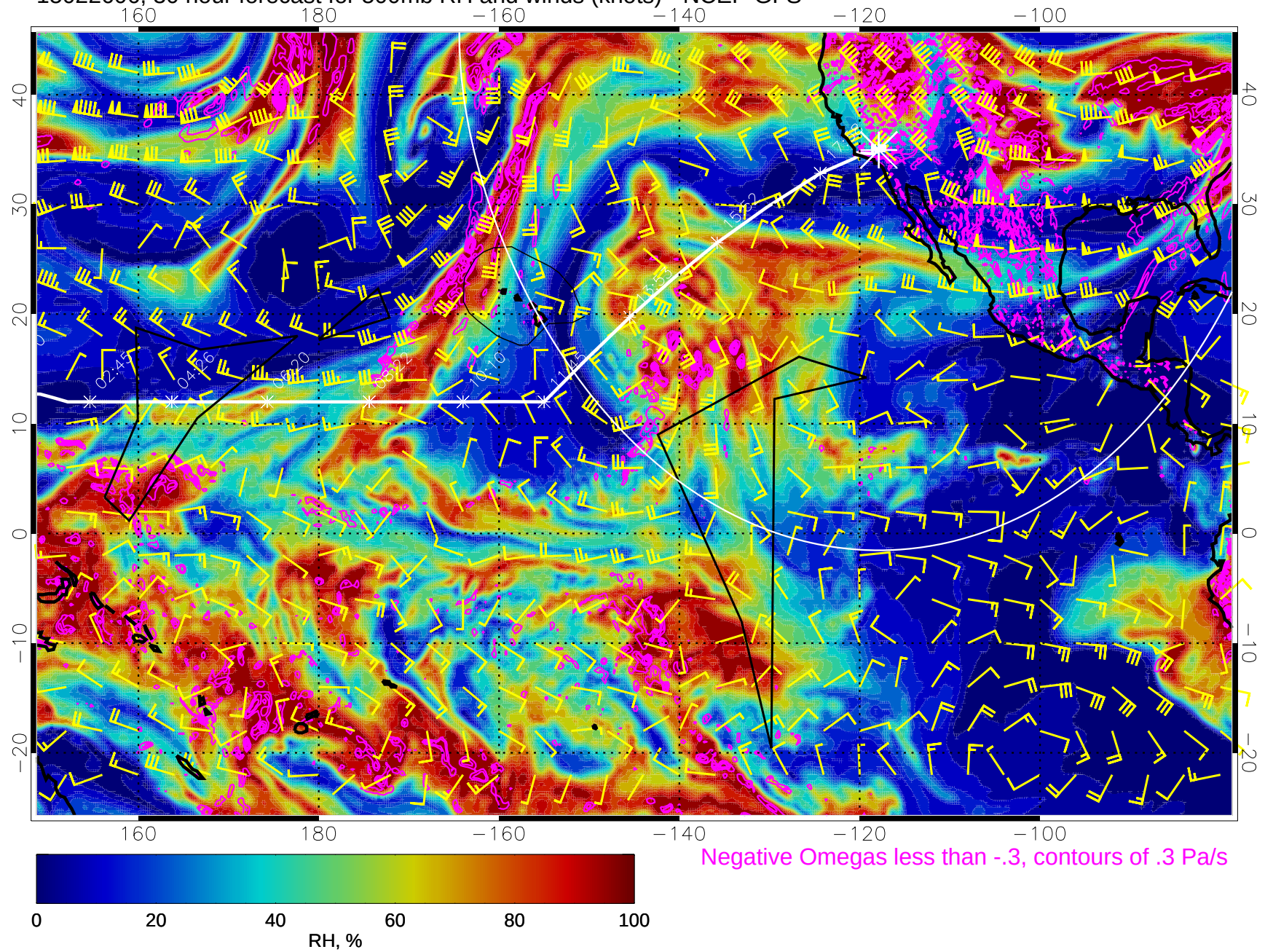
15022606, 30 hour forecast for 500mb RH and winds (knots) - NCEP GFS
