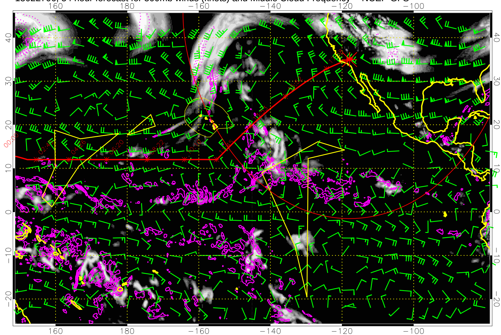
15022706, 54 hour forecast for 500mb winds (knots) and Middle Cloud Frequency -- NCEP GFS
