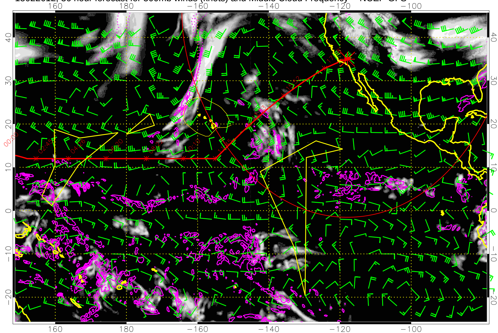
15022612, 36 hour forecast for 500mb winds (knots) and Middle Cloud Frequency -- NCEP GFS
