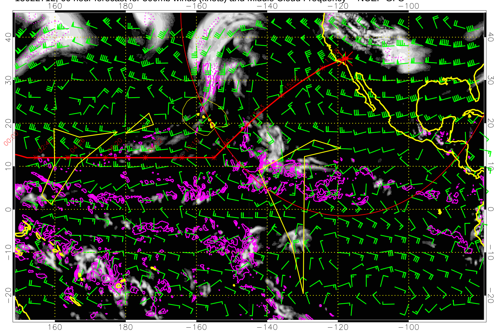
15022712, 60 hour forecast for 500mb winds (knots) and Middle Cloud Frequency -- NCEP GFS
