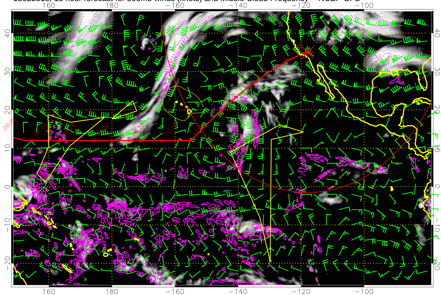
15022518, 18 hour forecast for 500mb winds (knots) and Middle Cloud Frequency -- NCEP GFS
