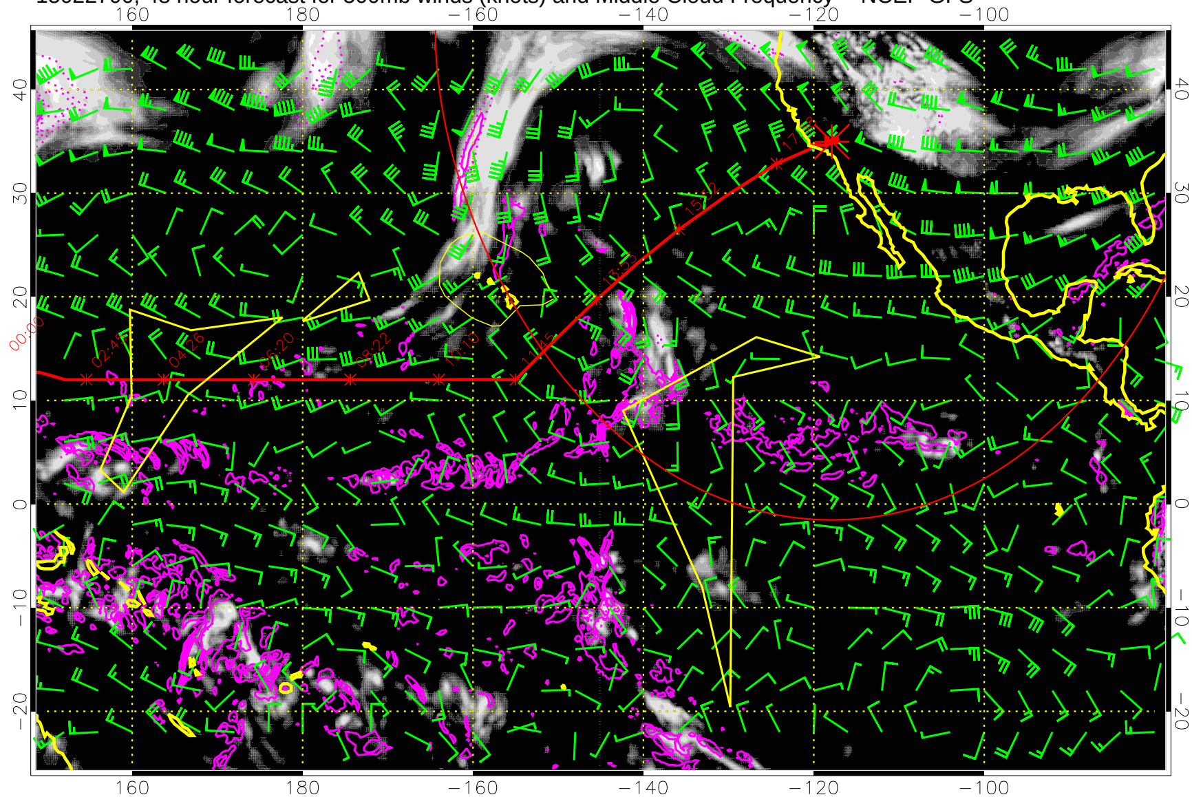
15022700, 48 hour forecast for 500mb winds (knots) and Middle Cloud Frequency -- NCEP GFS
