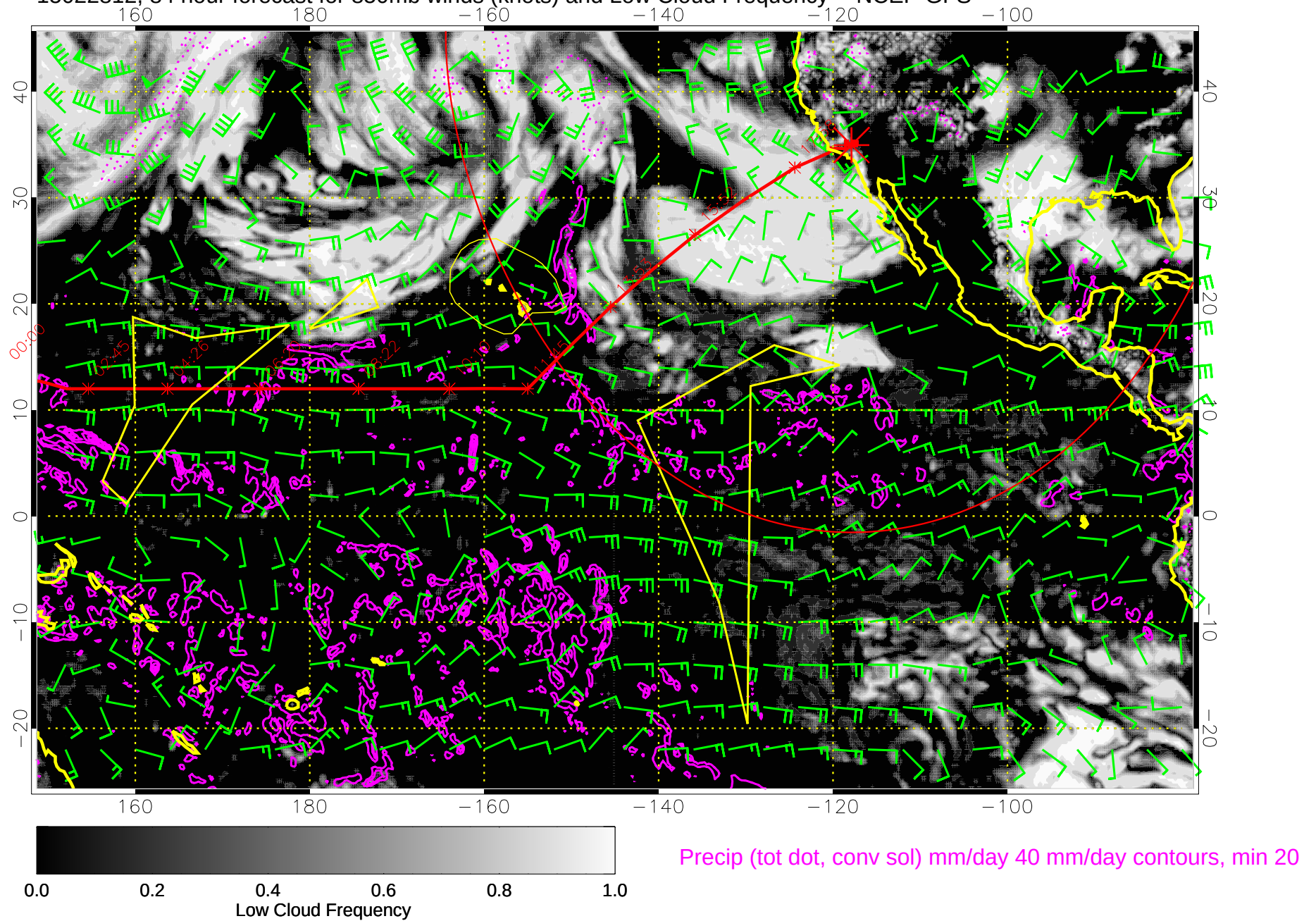
15022812, 84 hour forecast for 850mb winds (knots) and Low Cloud Frequency -- NCEP GFS
