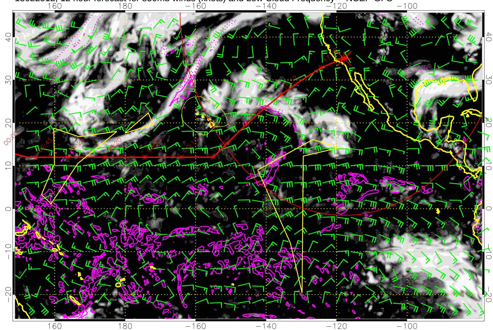
15022512, 12 hour forecast for 850mb winds (knots) and Low Cloud Frequency -- NCEP GFS
