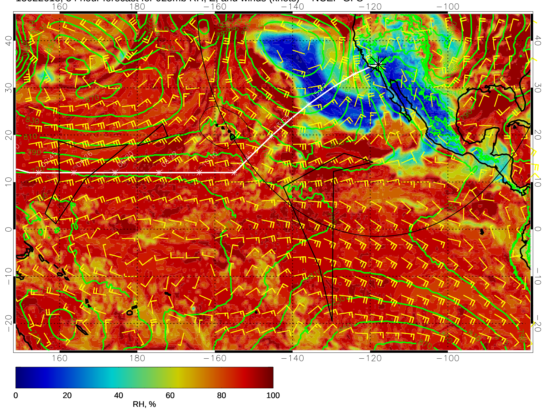
15022618, 54 hour forecast for 925mb RH, Z, and winds (knots) -- NCEP GFS
