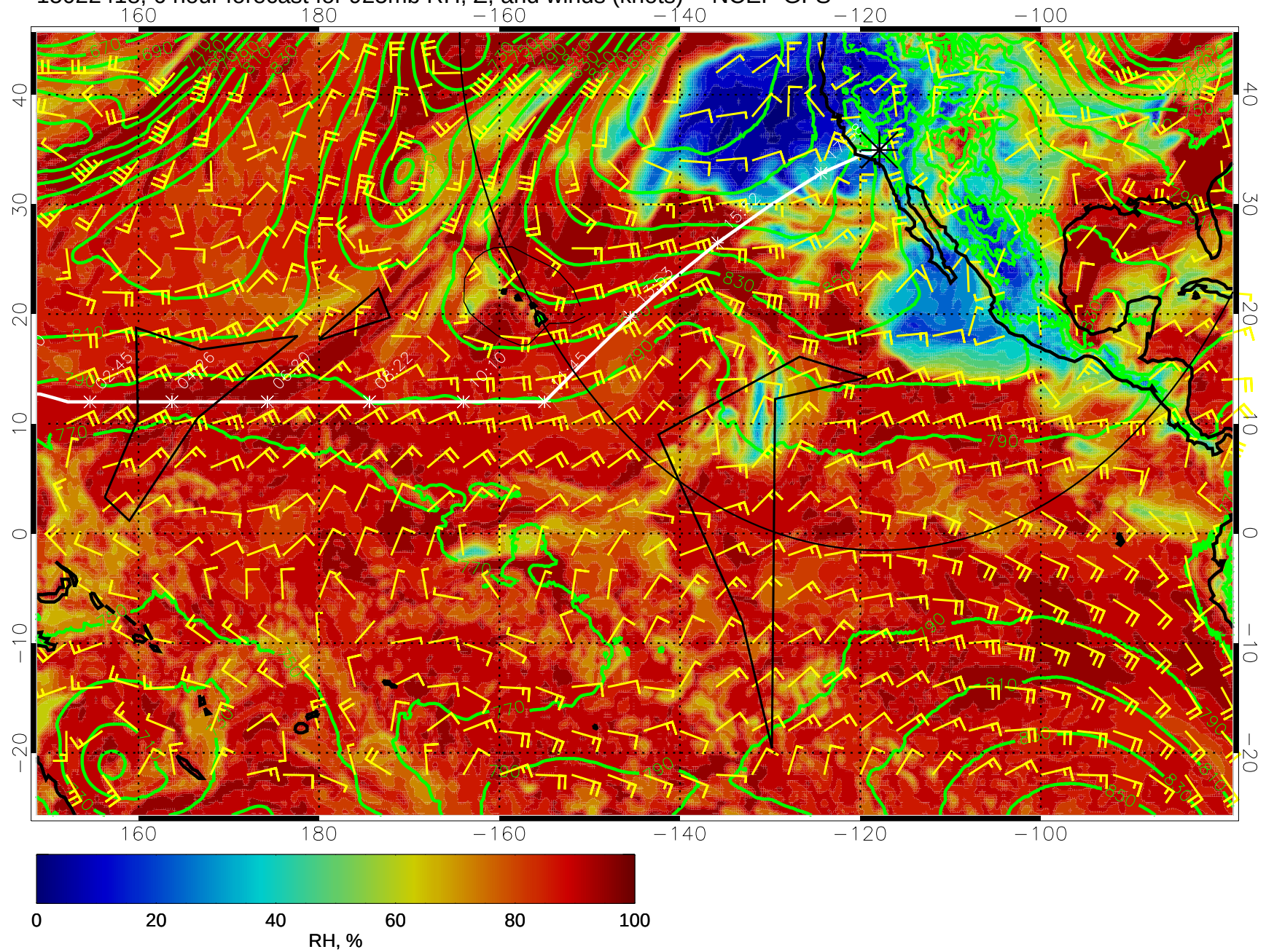
15022418, 6 hour forecast for 925mb RH, Z, and winds (knots) -- NCEP GFS
