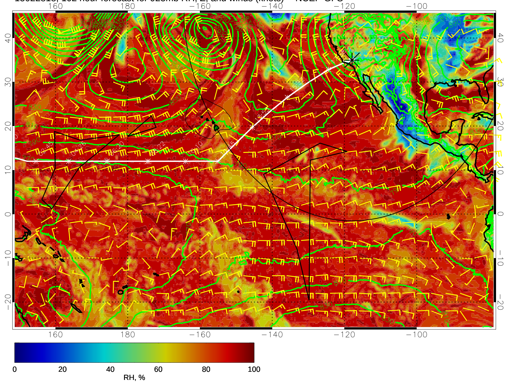
15022818, 102 hour forecast for 925mb RH, Z, and winds (knots) -- NCEP GFS
