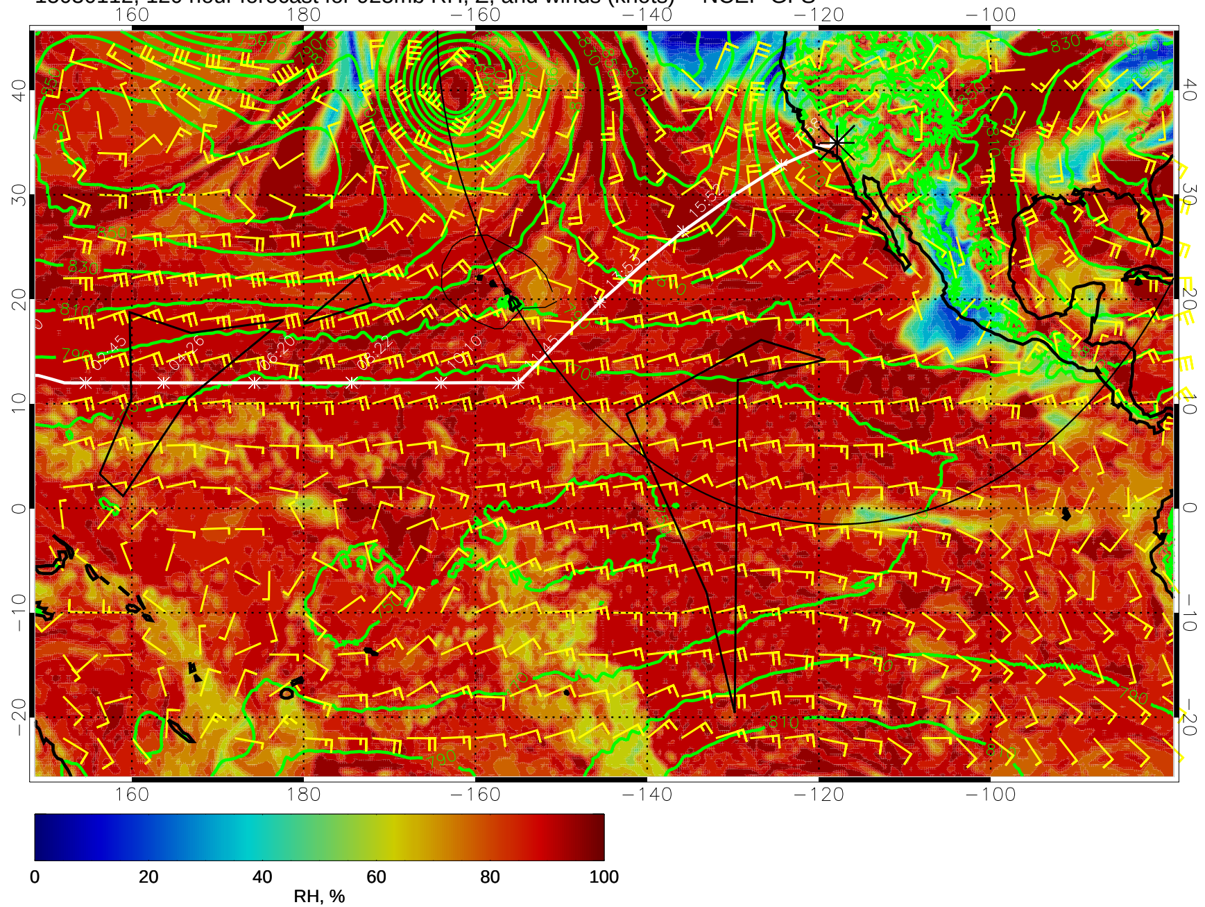
15030112, 120 hour forecast for 925mb RH, Z, and winds (knots) -- NCEP GFS
