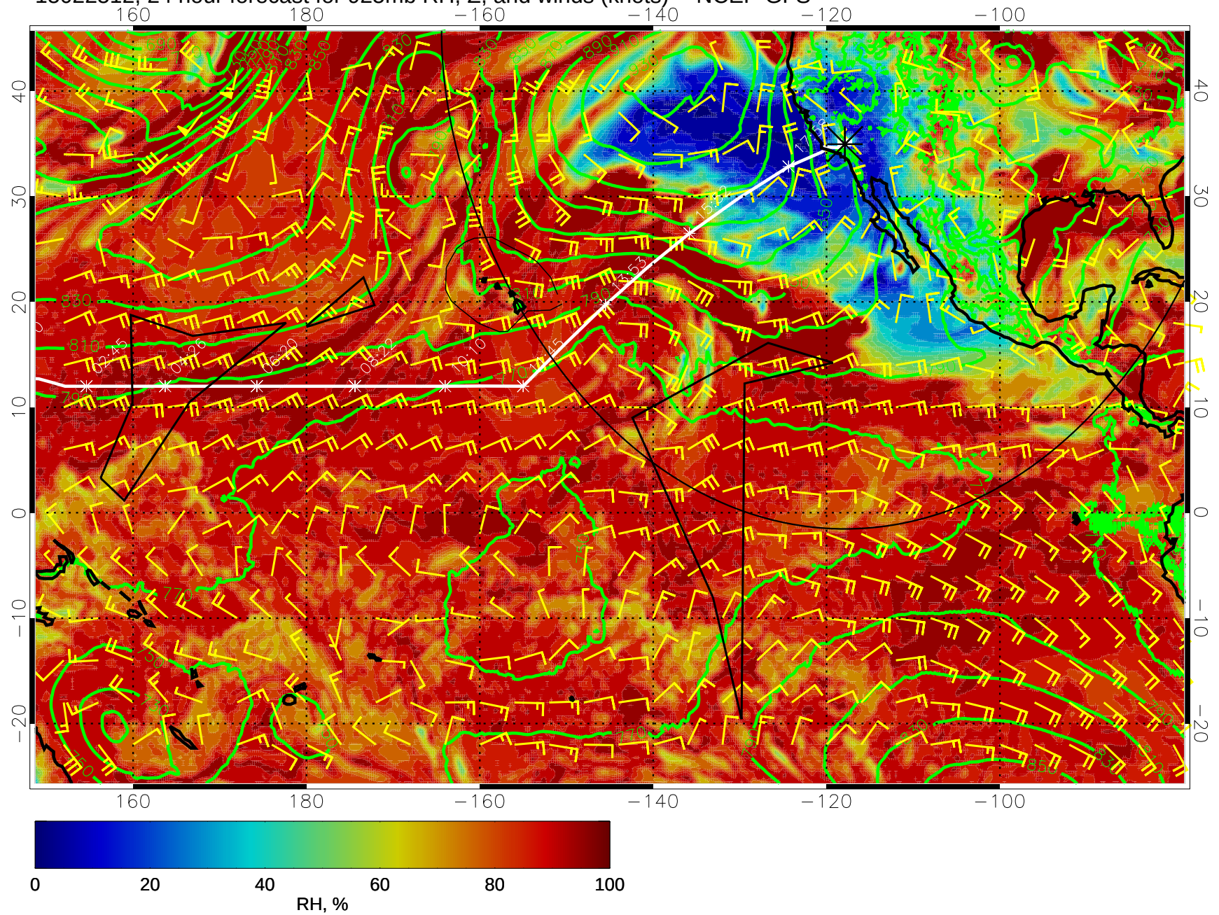
15022512, 24 hour forecast for 925mb RH, Z, and winds (knots) -- NCEP GFS
