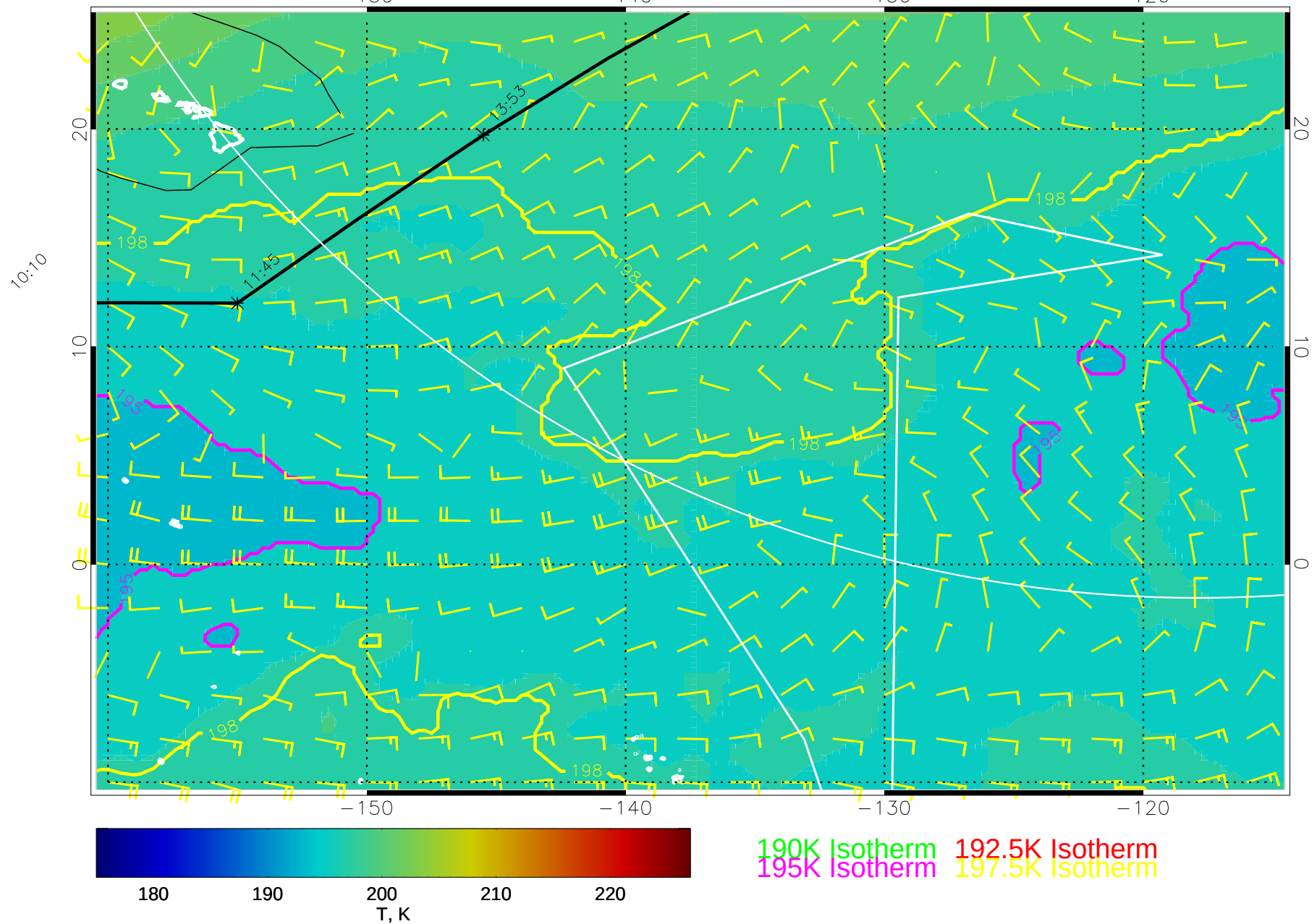
15022818, 102 hour forecast for 70mb T and winds (knots) -- NCEP GFS
