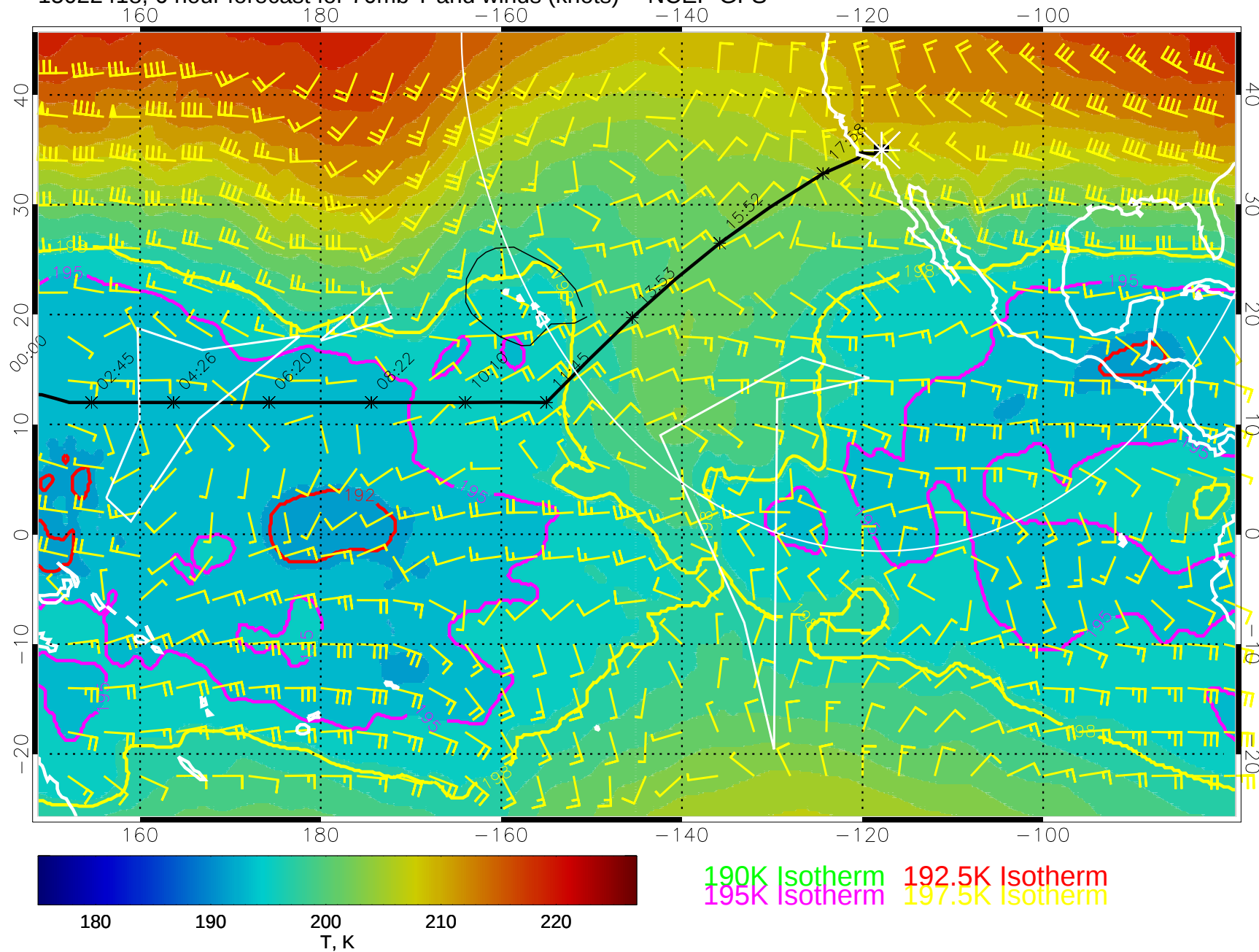
15022418, 6 hour forecast for 70mb T and winds (knots) -- NCEP GFS
