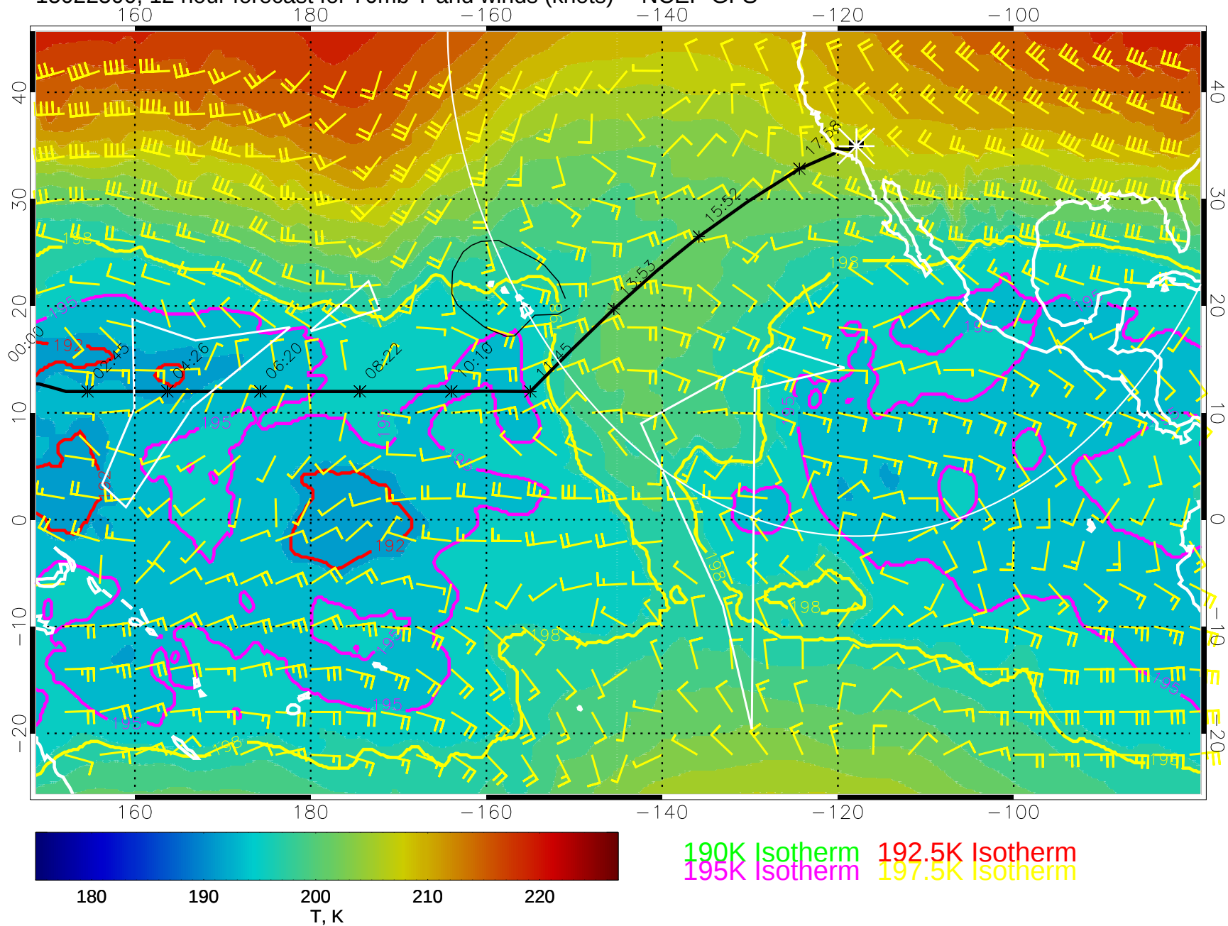
15022500, 12 hour forecast for 70mb T and winds (knots) -- NCEP GFS
