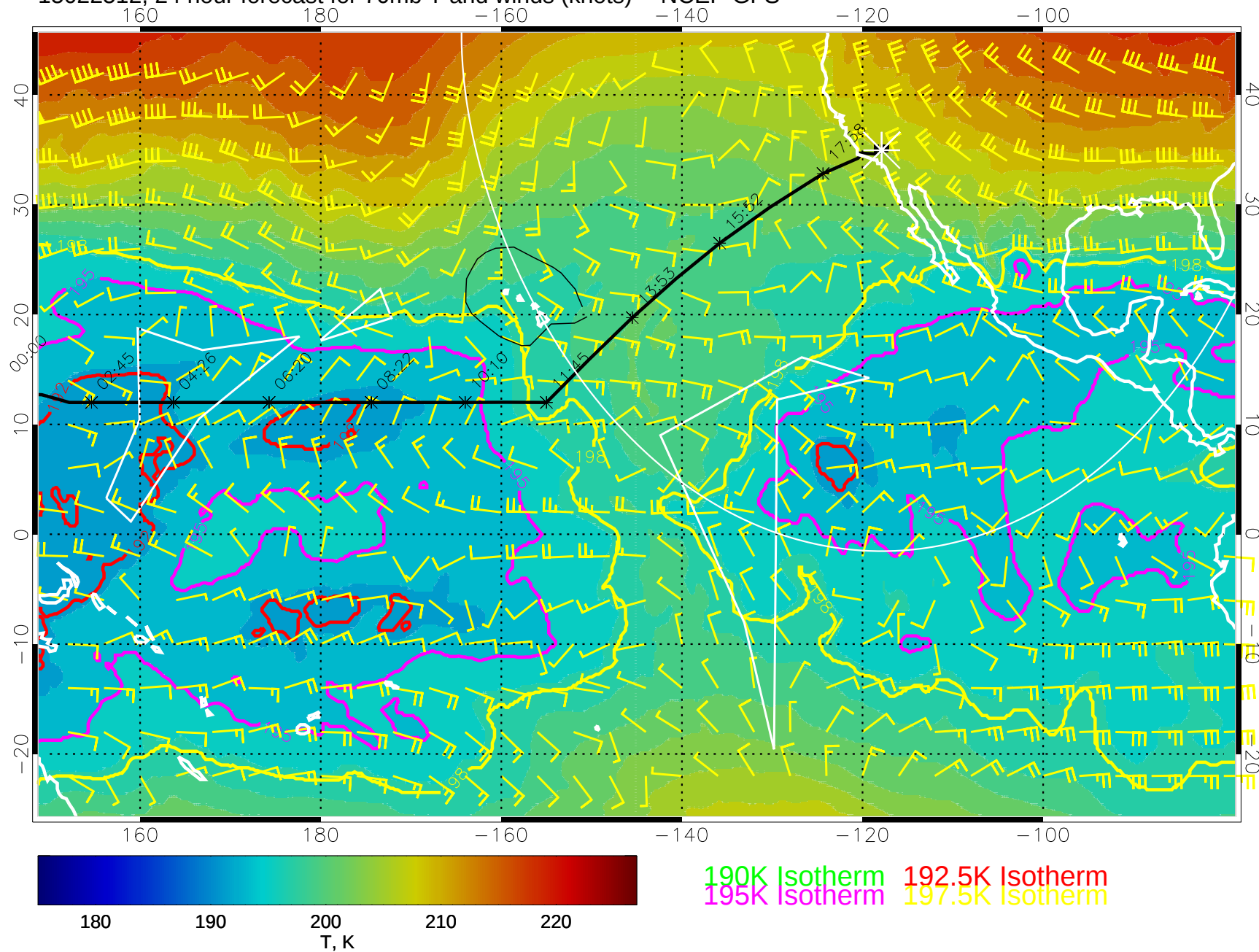
15022512, 24 hour forecast for 70mb T and winds (knots) -- NCEP GFS
