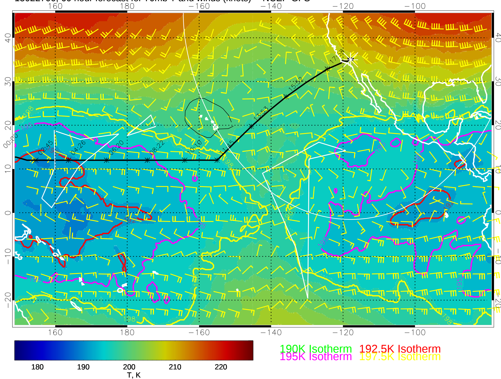
15022700, 60 hour forecast for 70mb T and winds (knots) -- NCEP GFS
