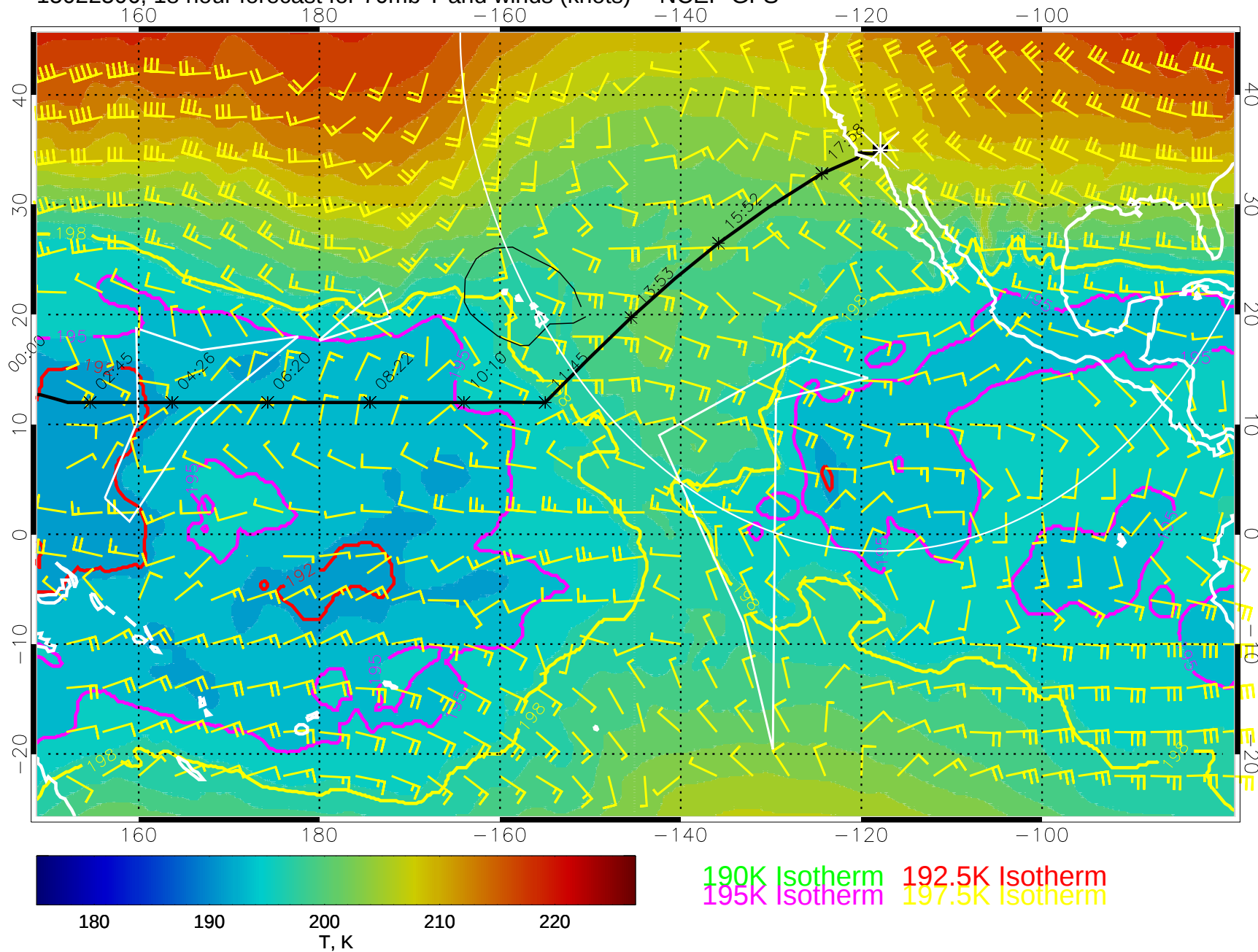
15022506, 18 hour forecast for 70mb T and winds (knots) -- NCEP GFS
