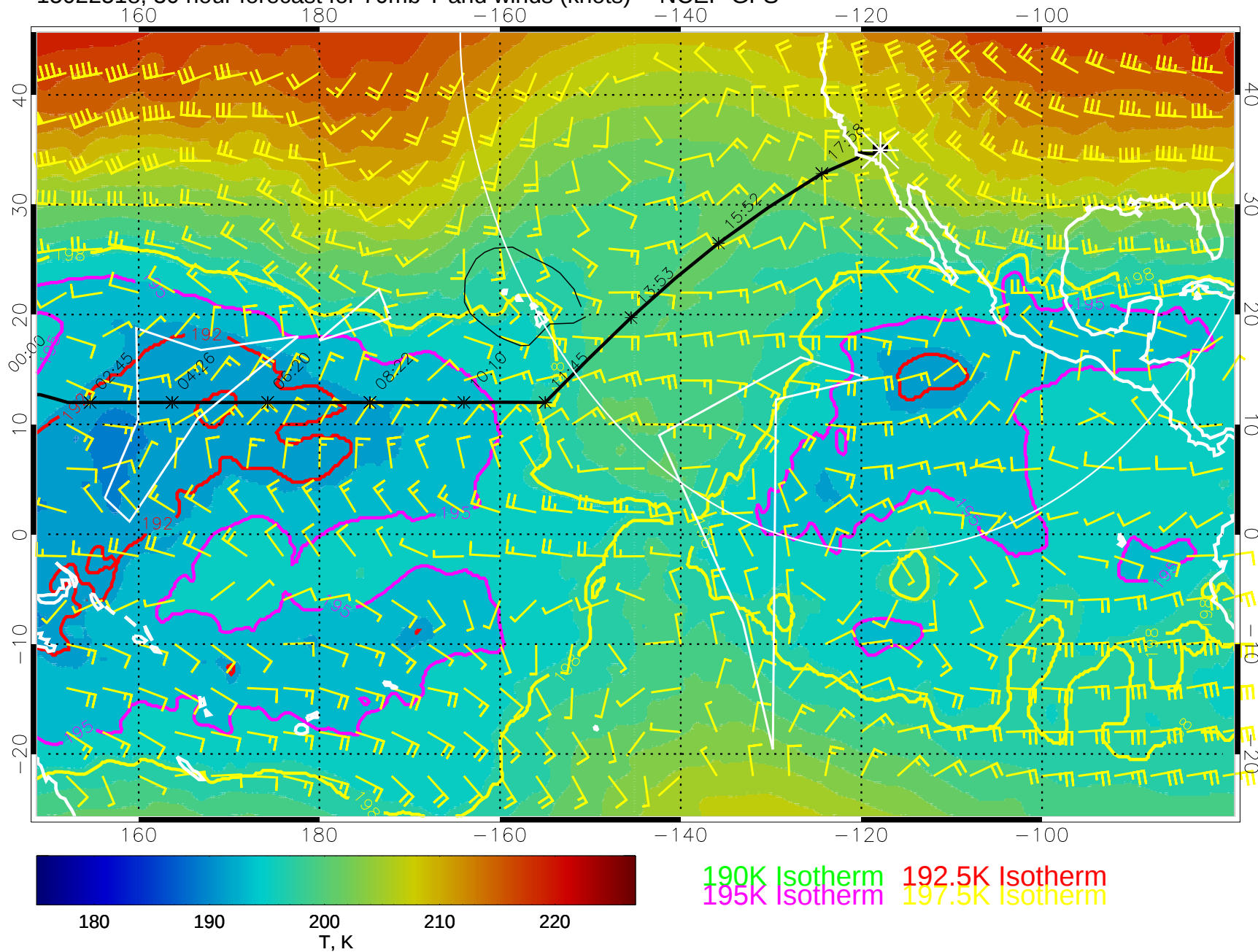
15022518, 30 hour forecast for 70mb T and winds (knots) -- NCEP GFS
