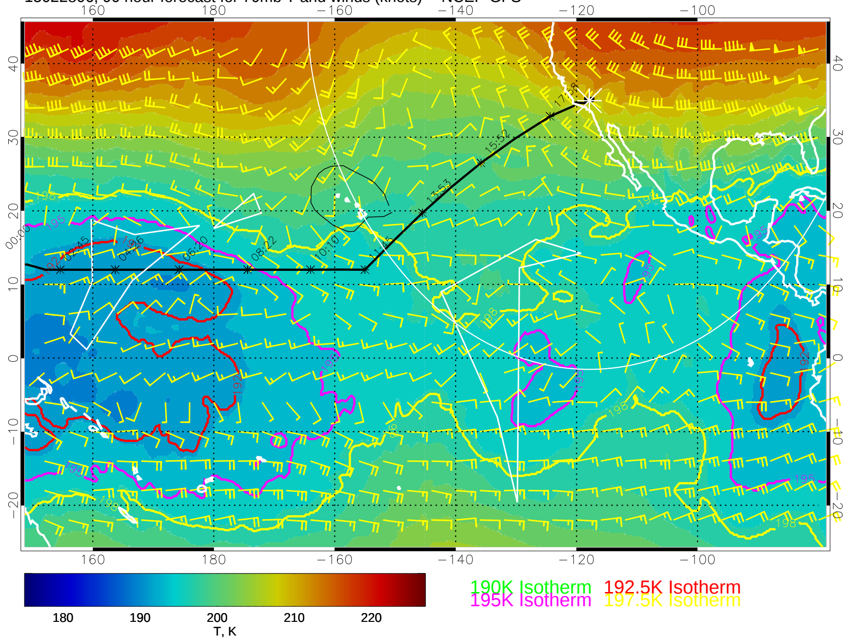
15022806, 90 hour forecast for 70mb T and winds (knots) -- NCEP GFS
