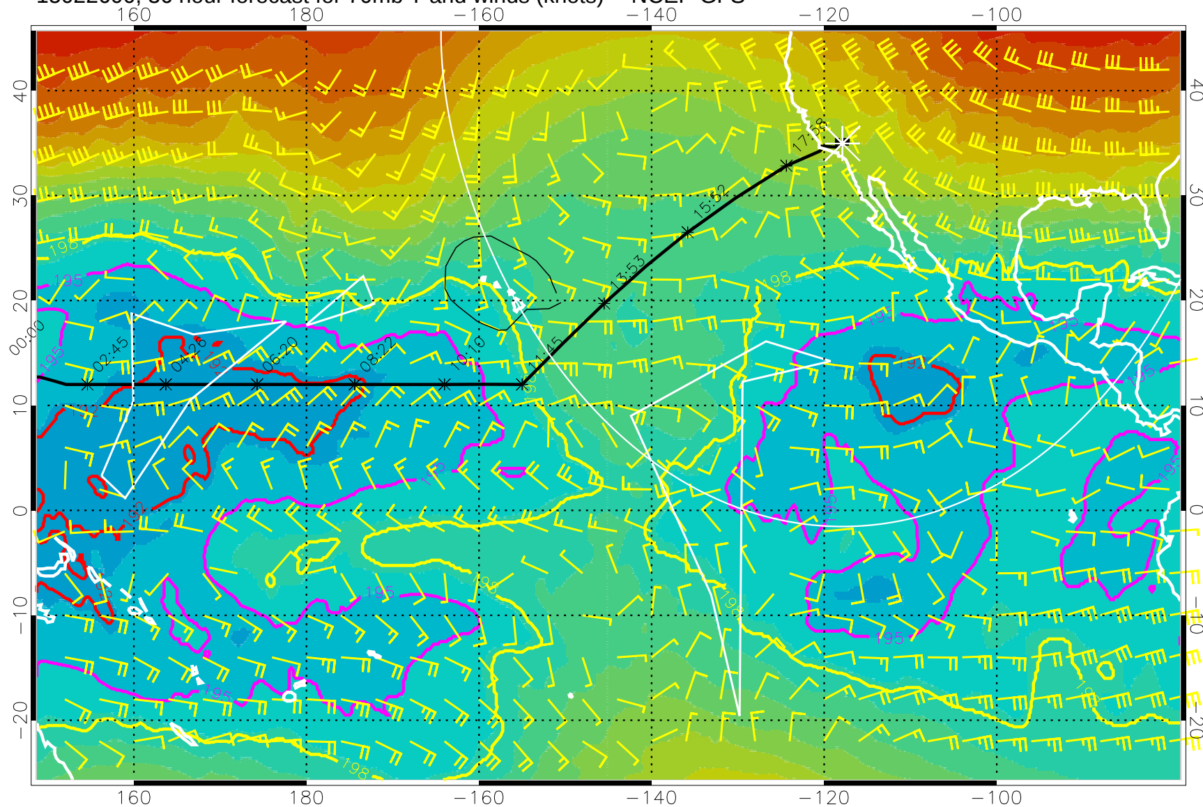
15022600, 36 hour forecast for 70mb T and winds (knots) -- NCEP GFS
