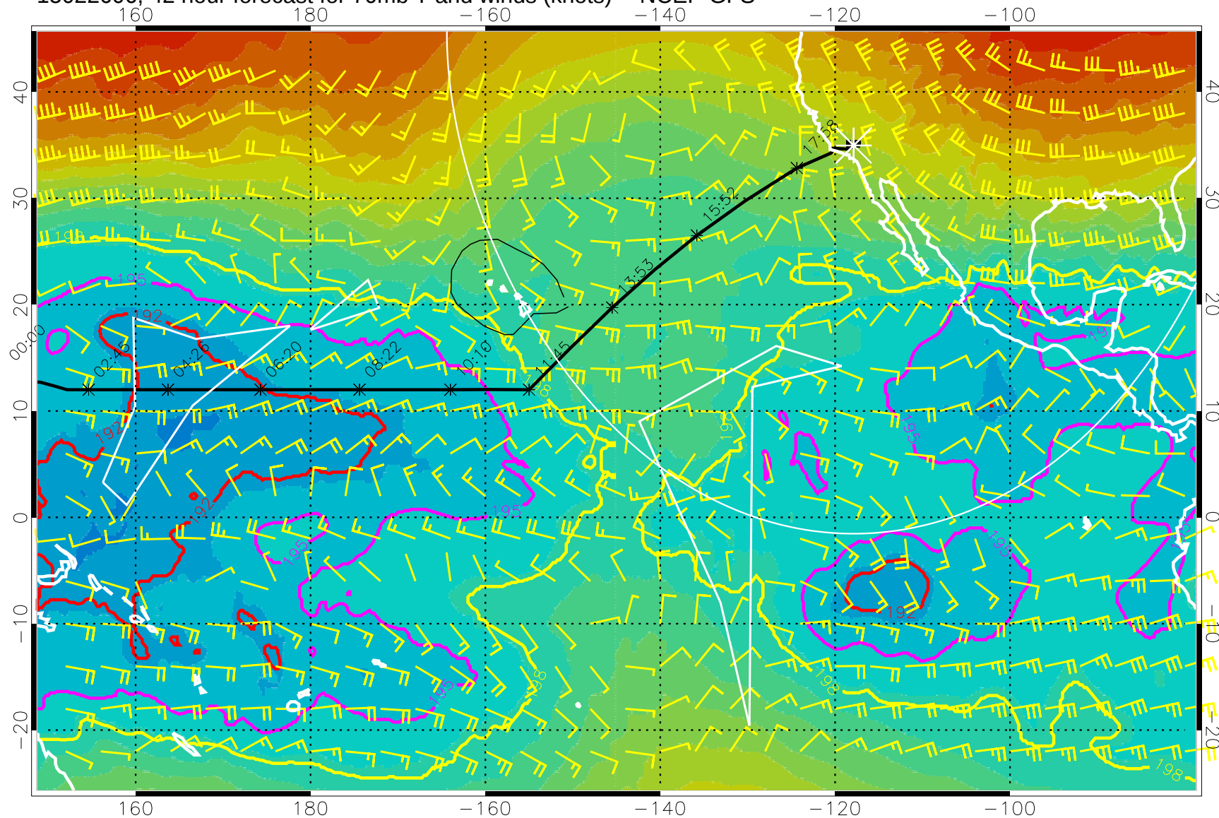
15022606, 42 hour forecast for 70mb T and winds (knots) -- NCEP GFS
