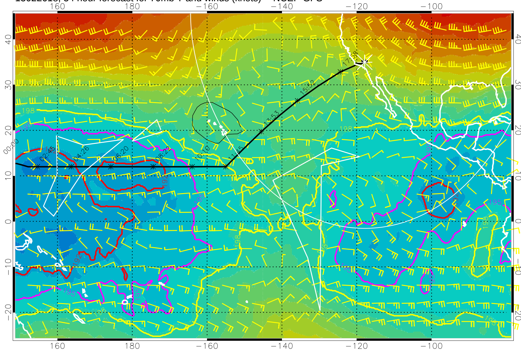
15022618, 54 hour forecast for 70mb T and winds (knots) -- NCEP GFS
