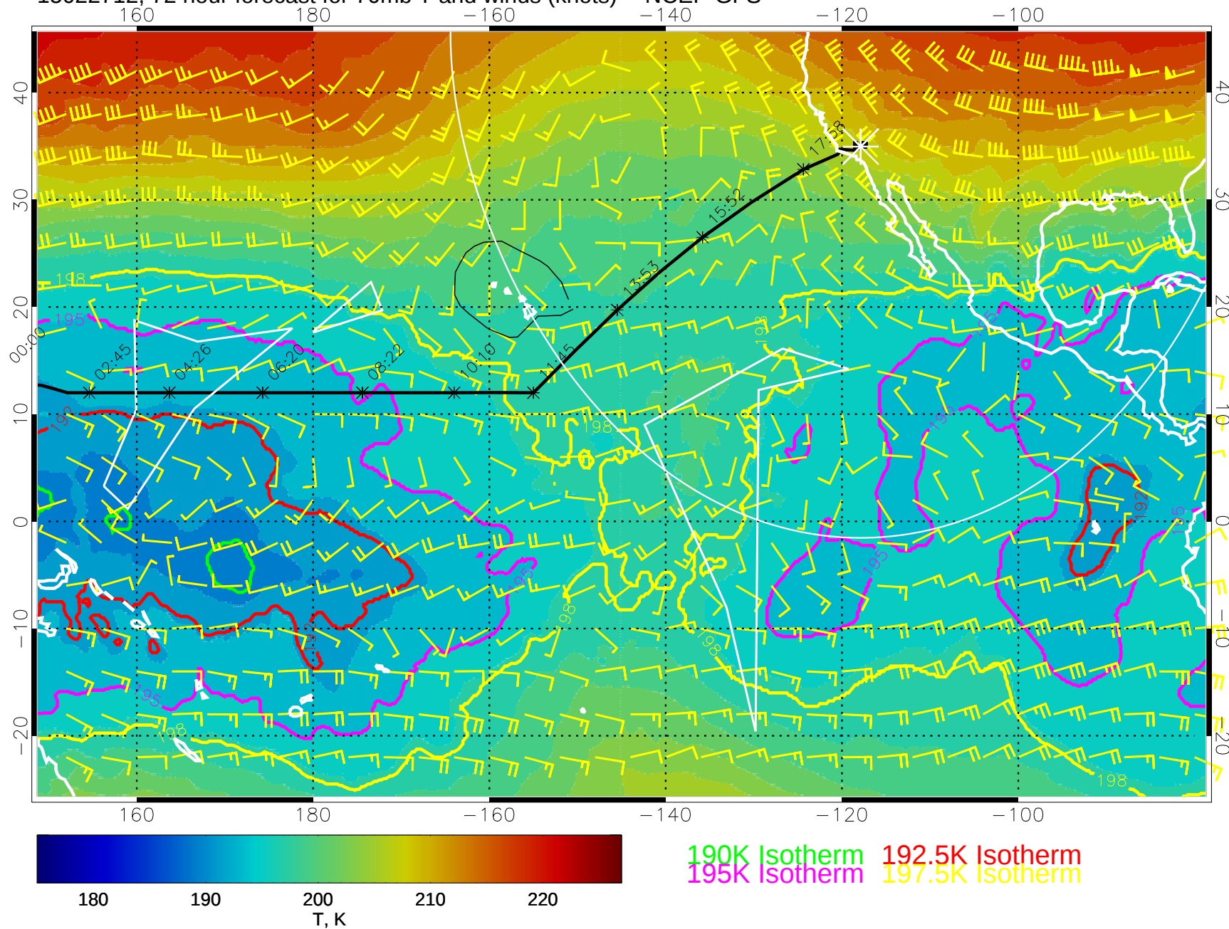
15022712, 72 hour forecast for 70mb T and winds (knots) -- NCEP GFS
