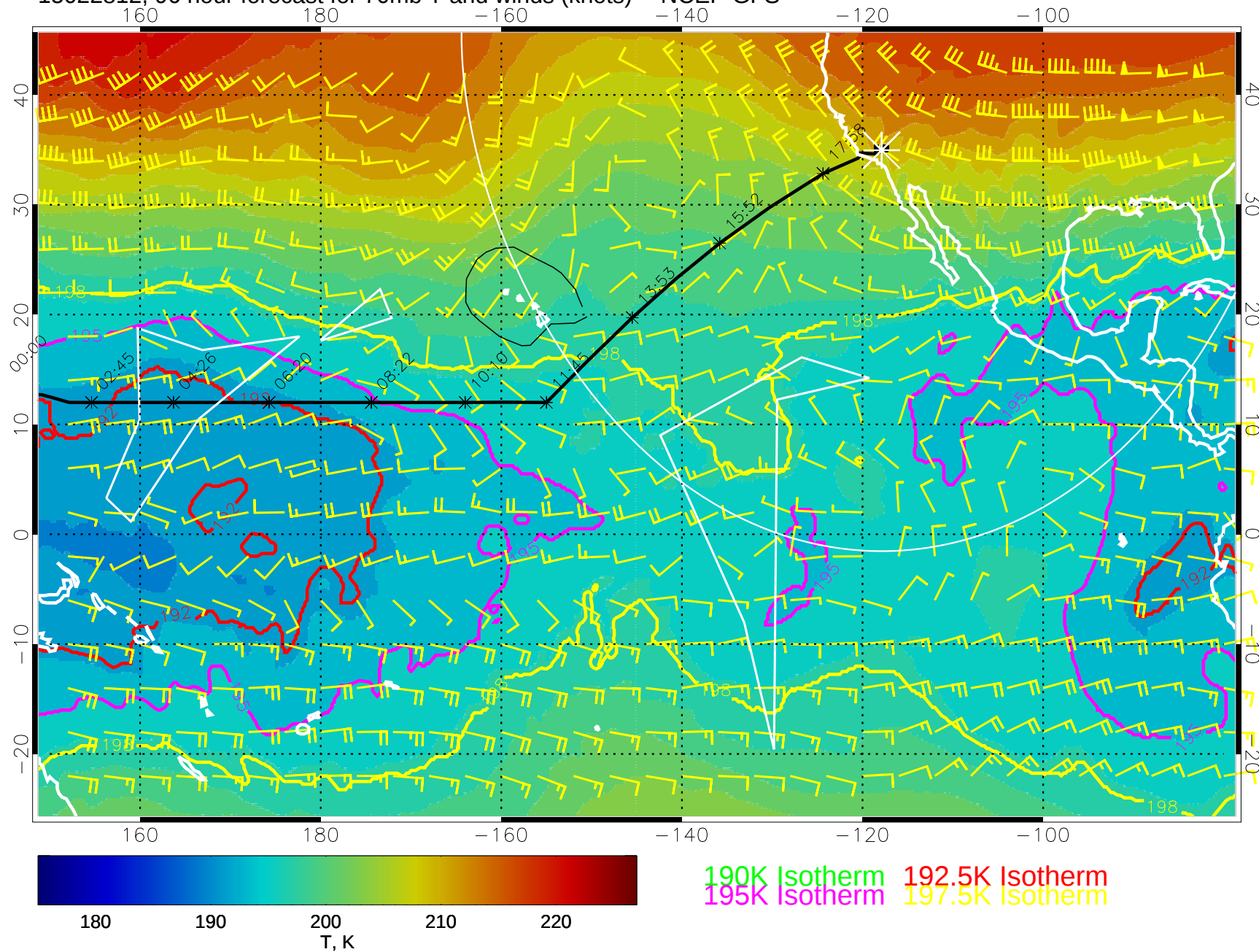
15022812, 96 hour forecast for 70mb T and winds (knots) -- NCEP GFS
