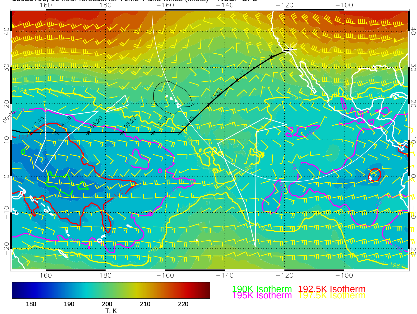
15022706, 66 hour forecast for 70mb T and winds (knots) -- NCEP GFS
