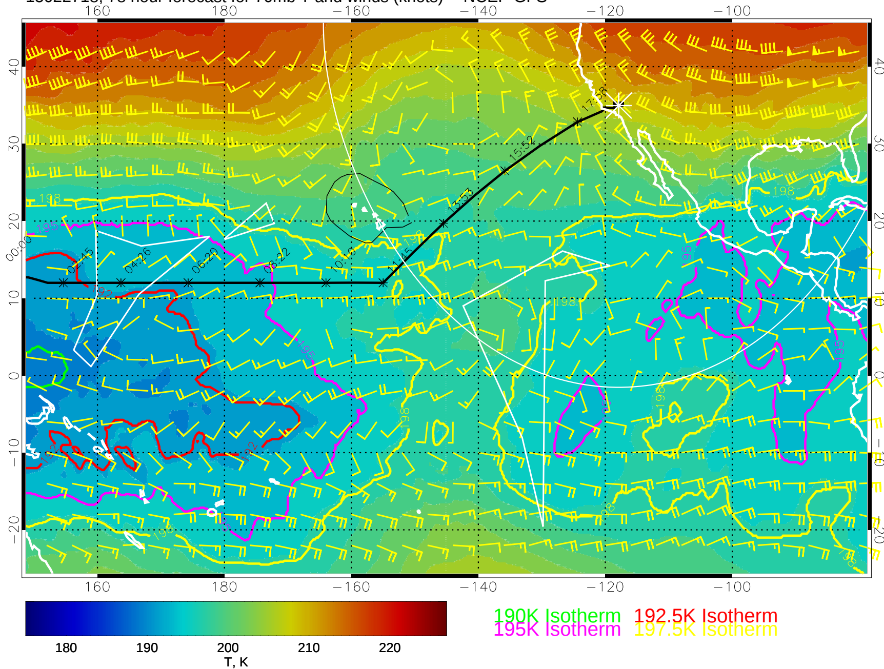
15022718, 78 hour forecast for 70mb T and winds (knots) -- NCEP GFS
