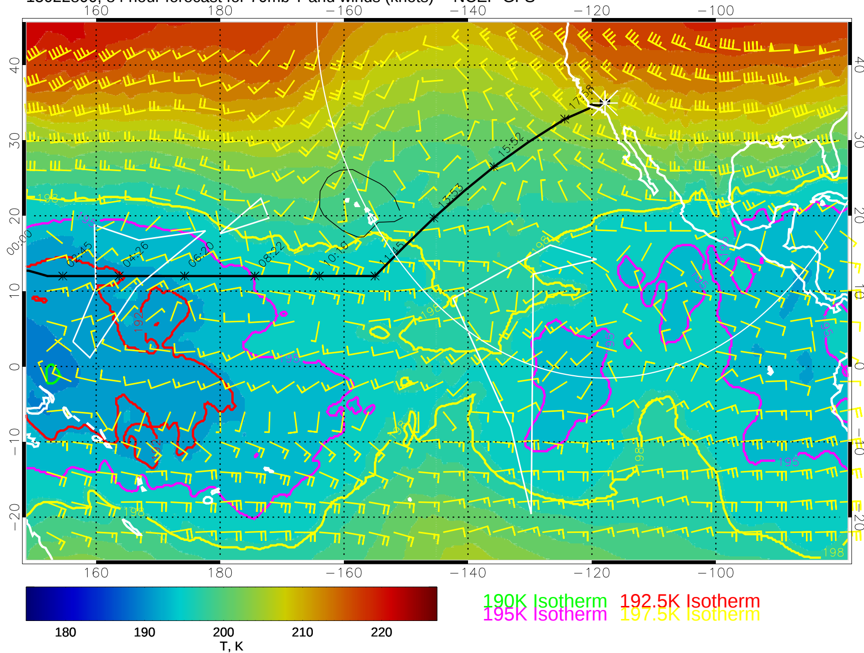
15022800, 84 hour forecast for 70mb T and winds (knots) -- NCEP GFS
