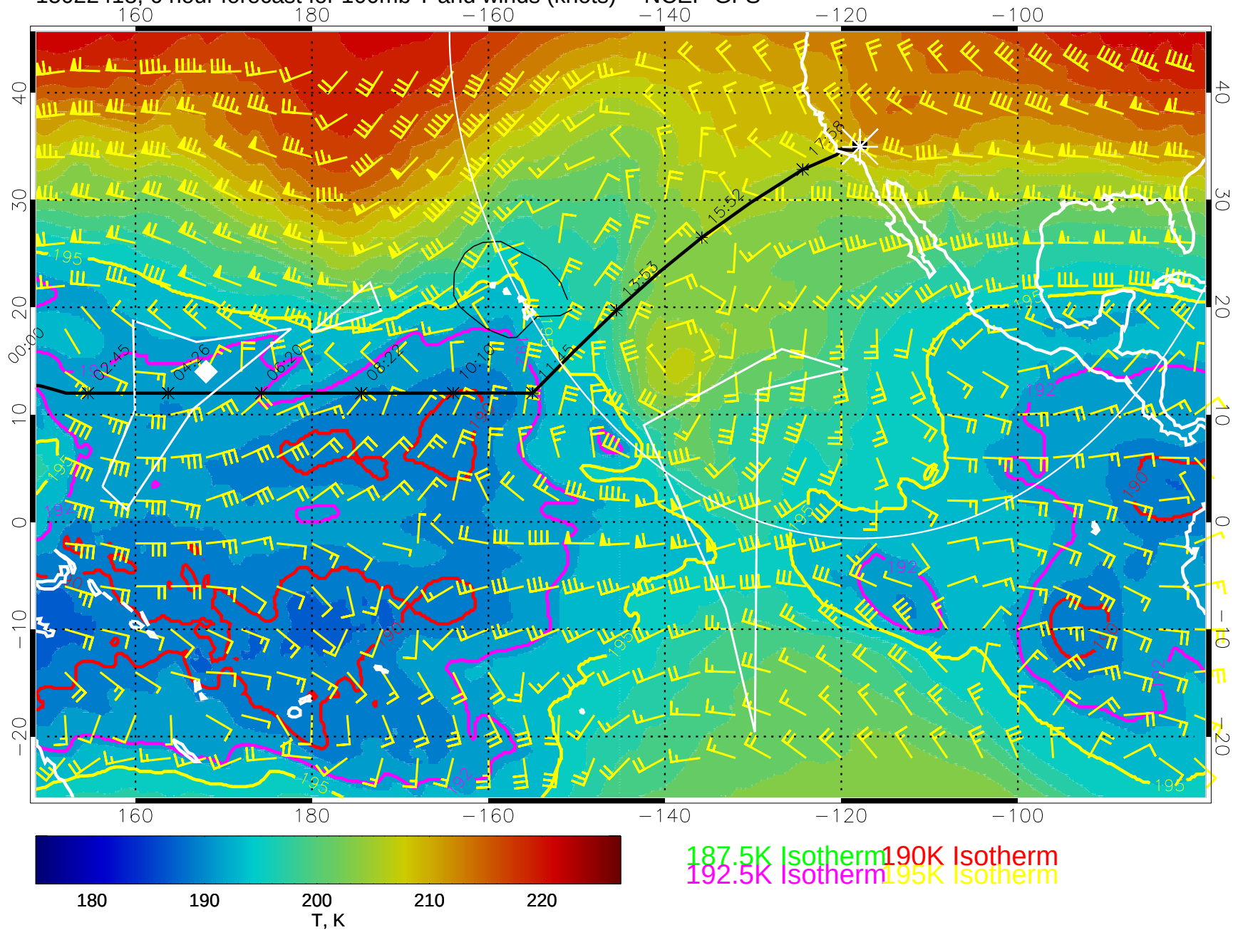
15022418, 6 hour forecast for 100mb T and winds (knots) -- NCEP GFS
