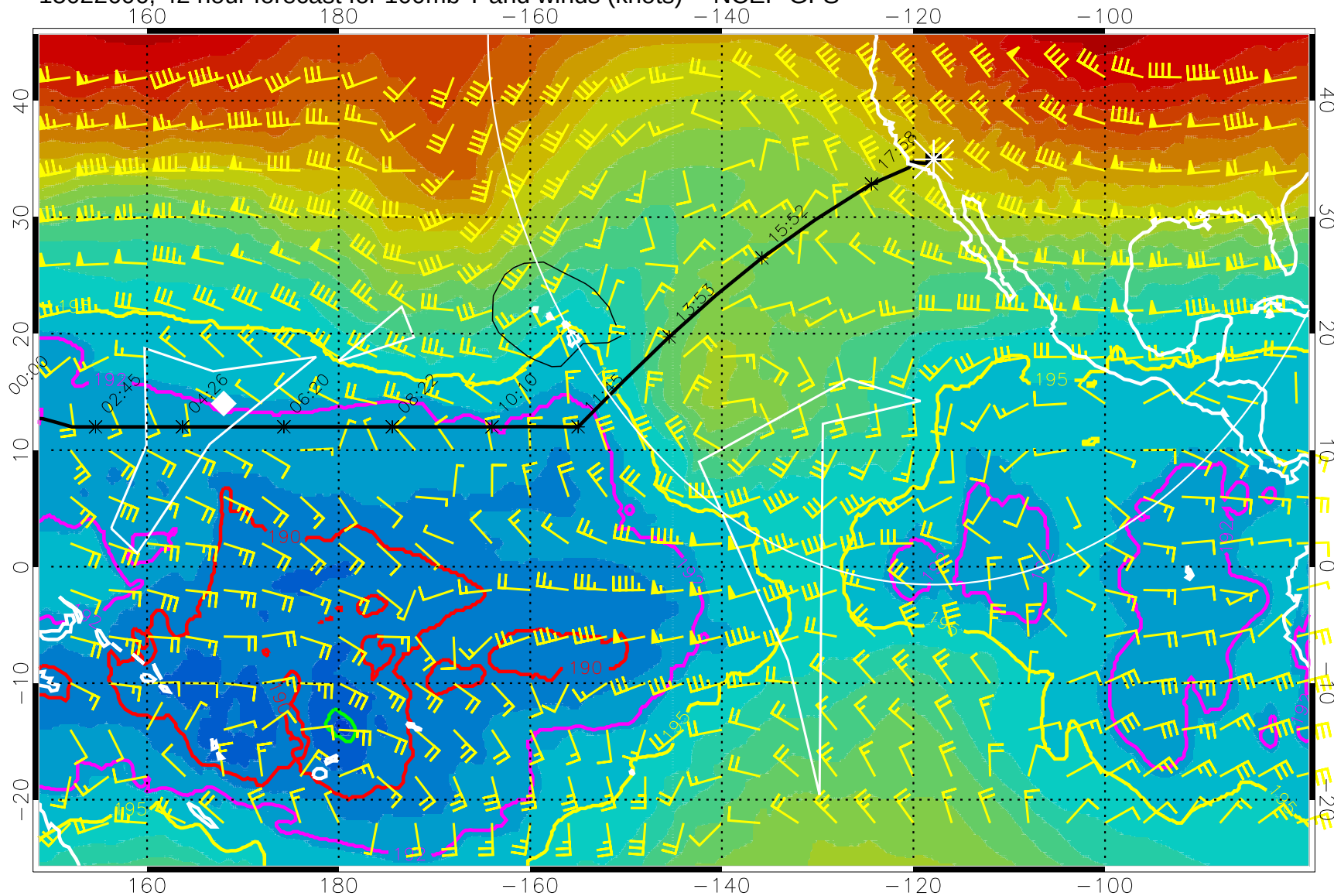
15022606, 42 hour forecast for 100mb T and winds (knots) -- NCEP GFS
