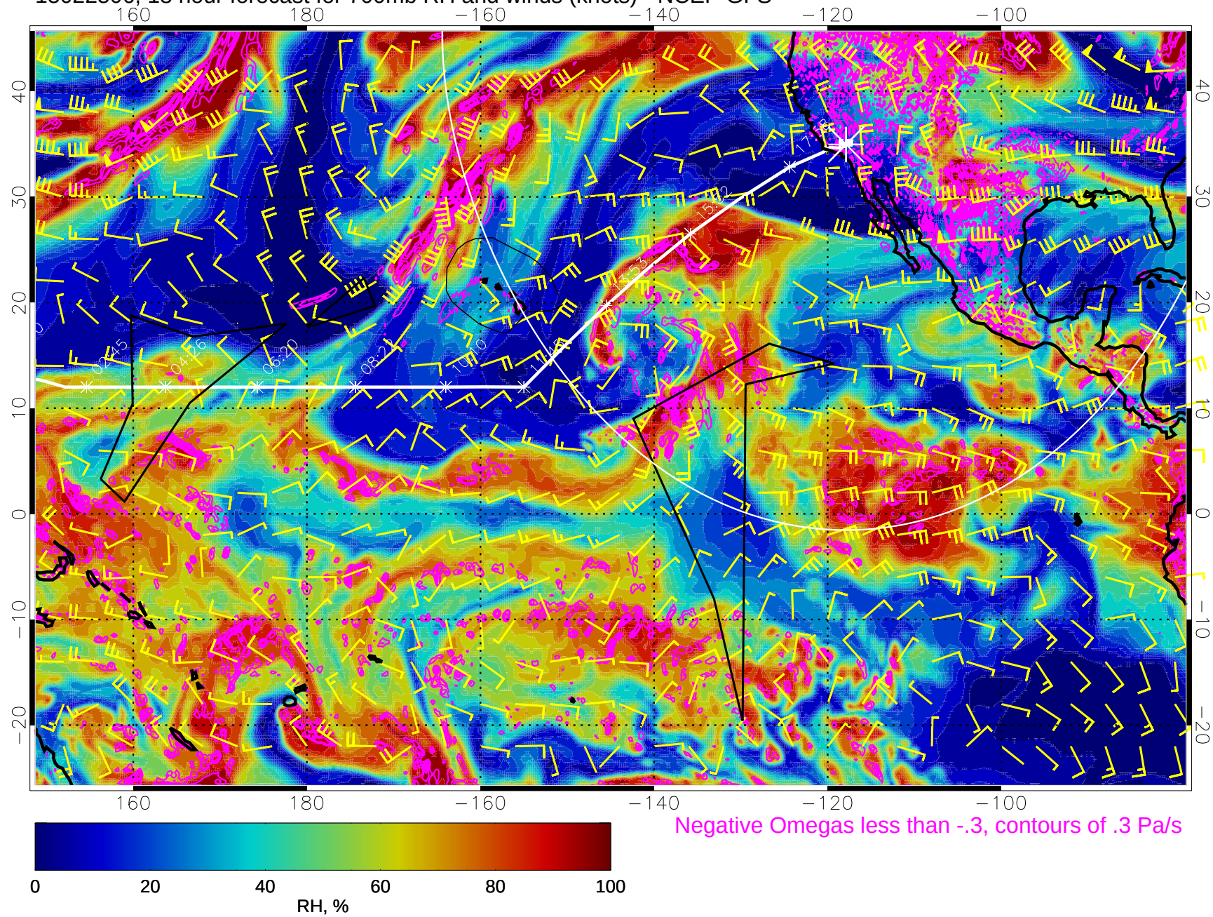
15022506, 18 hour forecast for 700mb RH and winds (knots) - NCEP GFS
