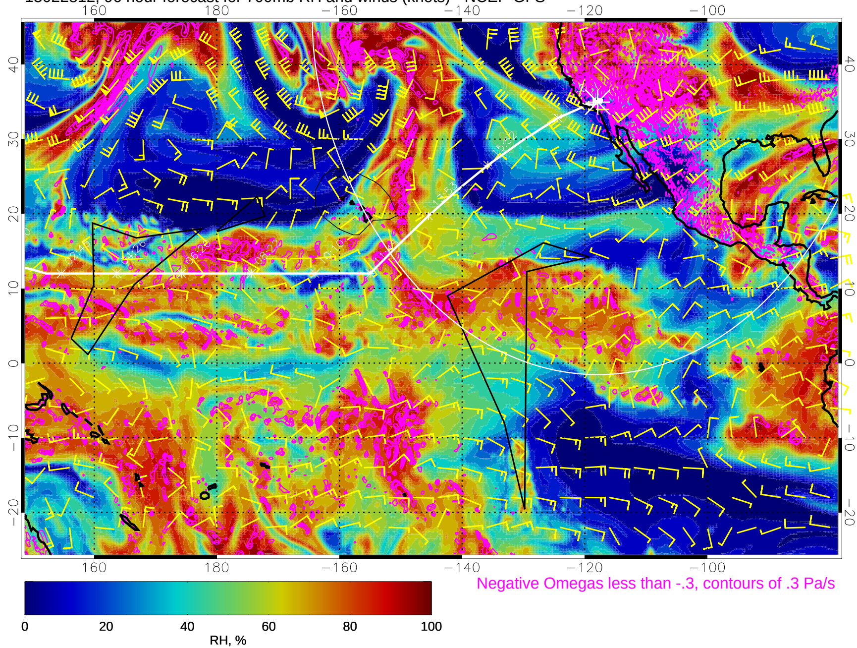
15022812, 96 hour forecast for 700mb RH and winds (knots) - NCEP GFS
