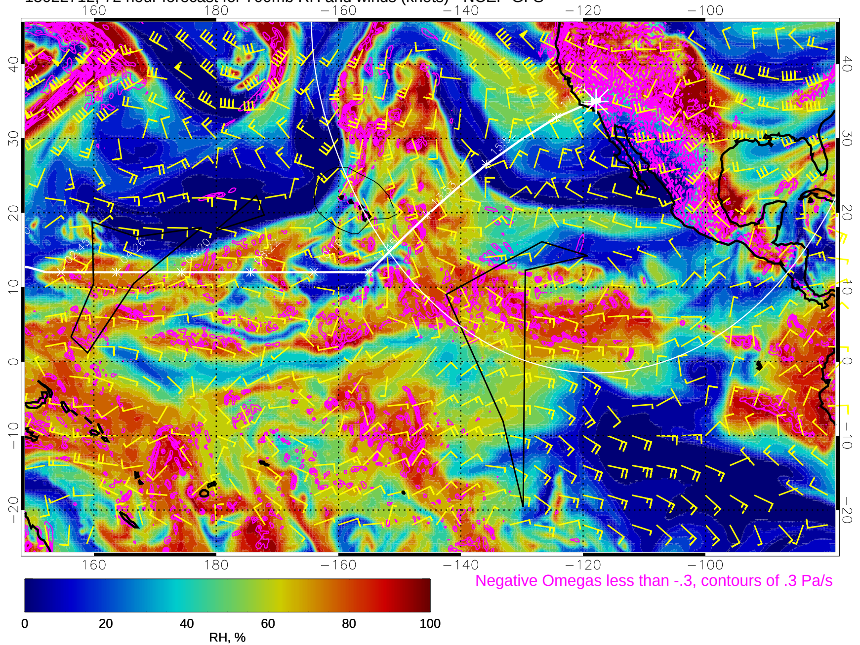
15022712, 72 hour forecast for 700mb RH and winds (knots) - NCEP GFS
