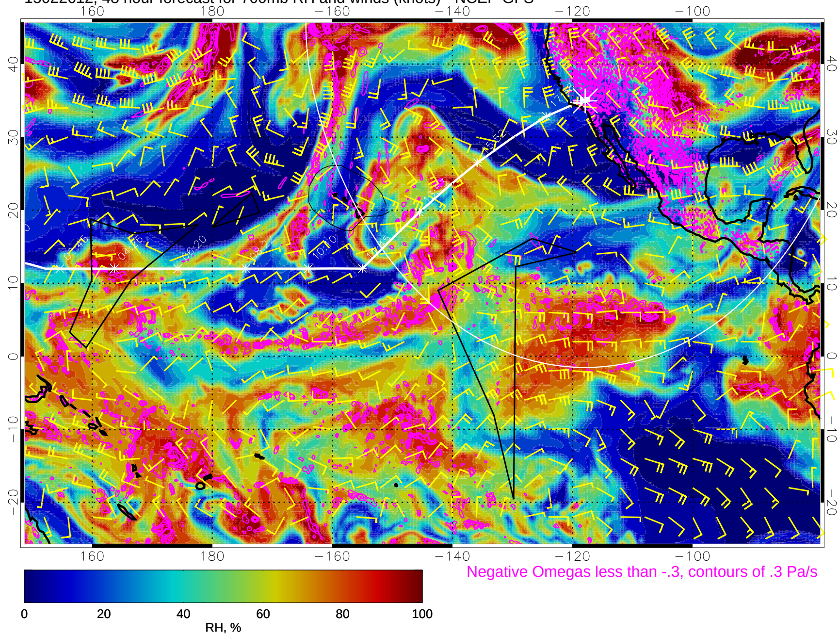
15022612, 48 hour forecast for 700mb RH and winds (knots) - NCEP GFS
