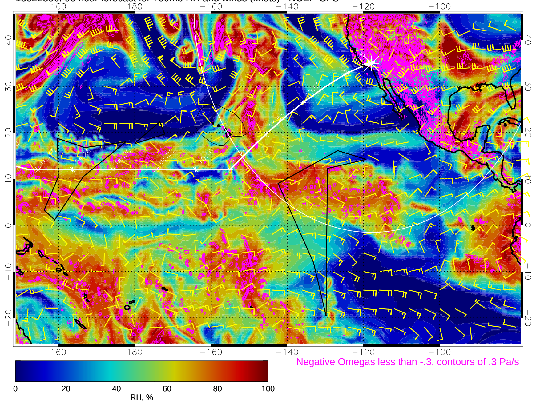
15022806, 90 hour forecast for 700mb RH and winds (knots) - NCEP GFS
