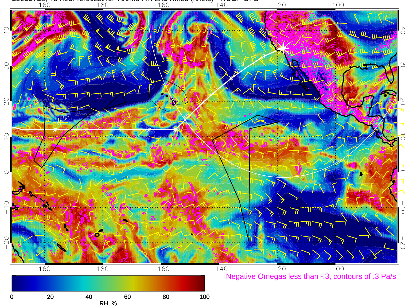
15022718, 78 hour forecast for 700mb RH and winds (knots) - NCEP GFS
