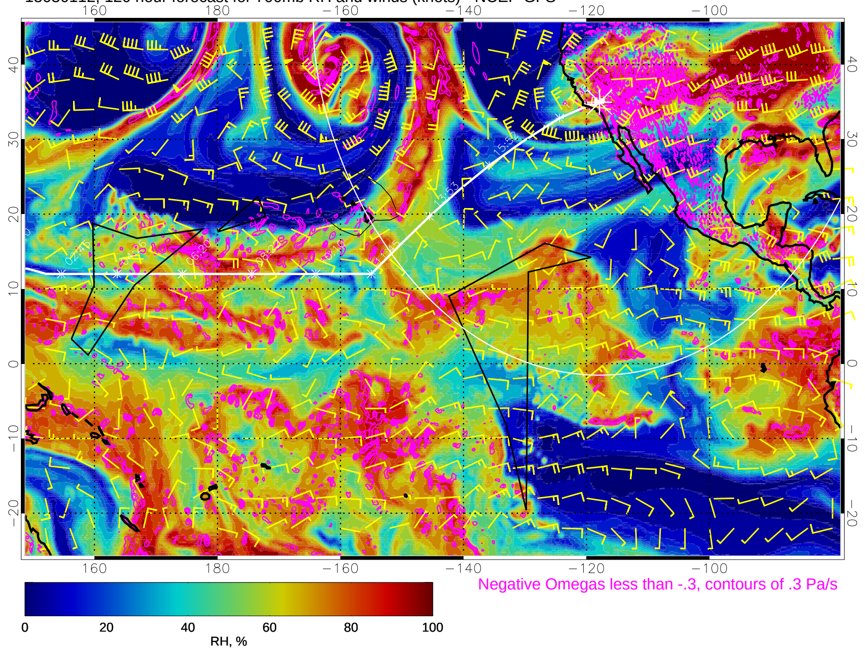
15030112, 120 hour forecast for 700mb RH and winds (knots) - NCEP GFS
