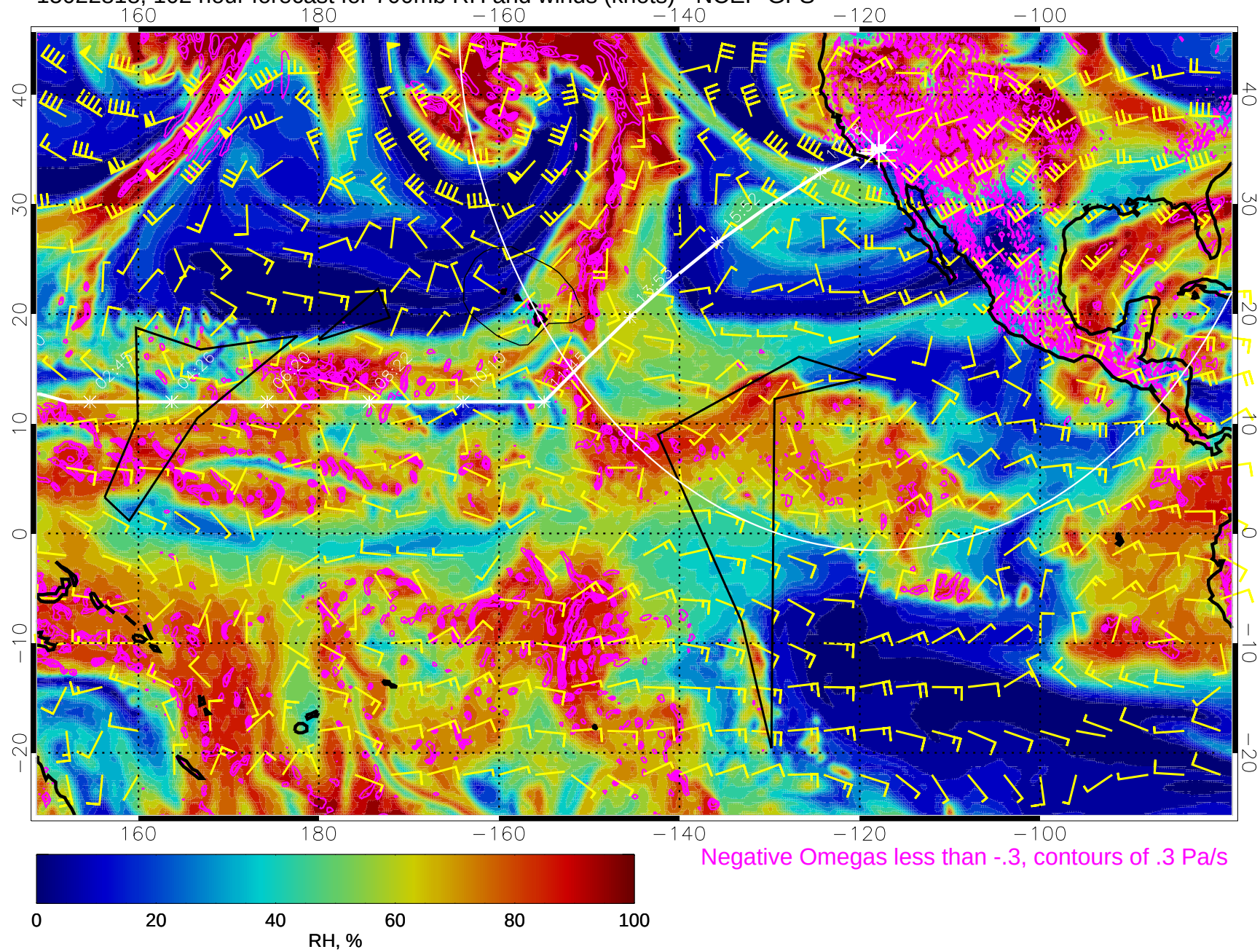
15022818, 102 hour forecast for 700mb RH and winds (knots) - NCEP GFS
