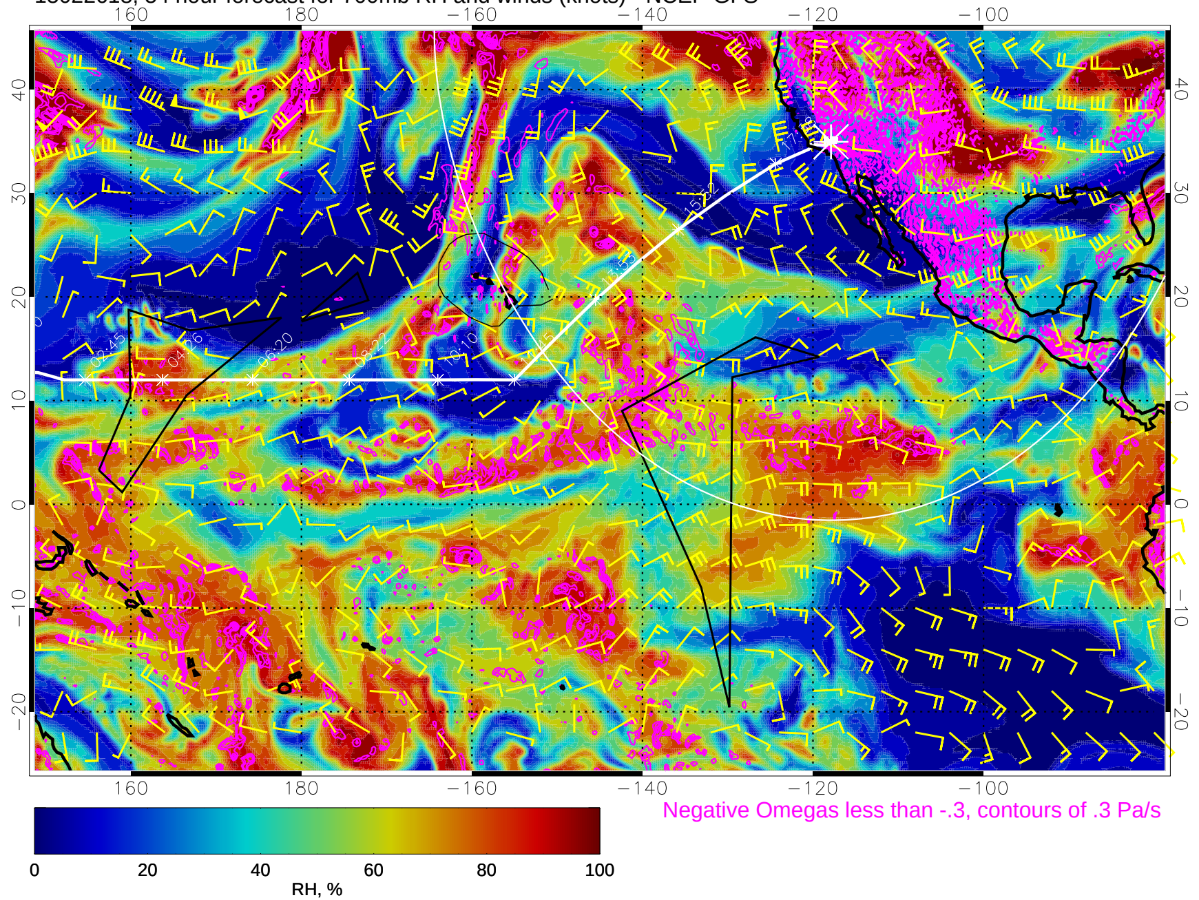
15022618, 54 hour forecast for 700mb RH and winds (knots) - NCEP GFS
