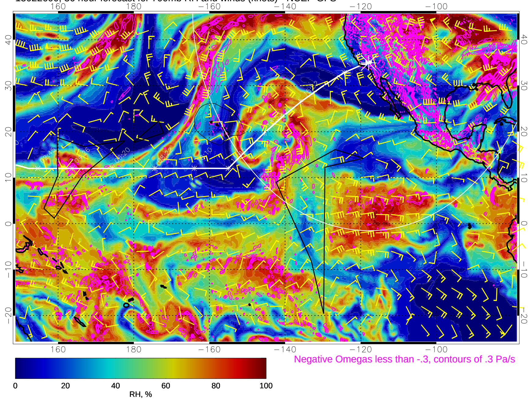
15022600, 36 hour forecast for 700mb RH and winds (knots) - NCEP GFS
