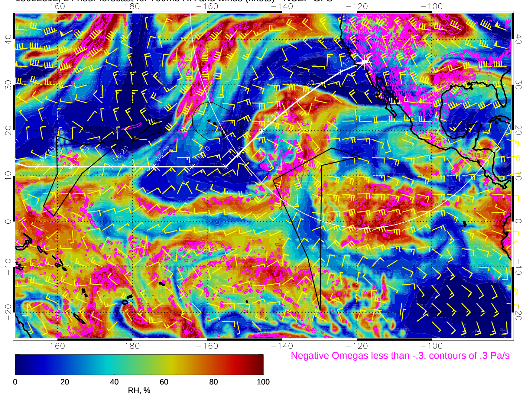
15022512, 24 hour forecast for 700mb RH and winds (knots) - NCEP GFS
