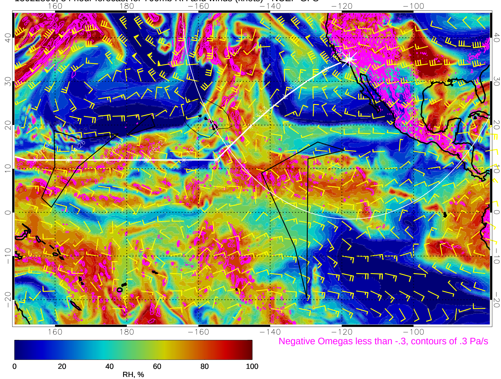
15022800, 84 hour forecast for 700mb RH and winds (knots) - NCEP GFS
