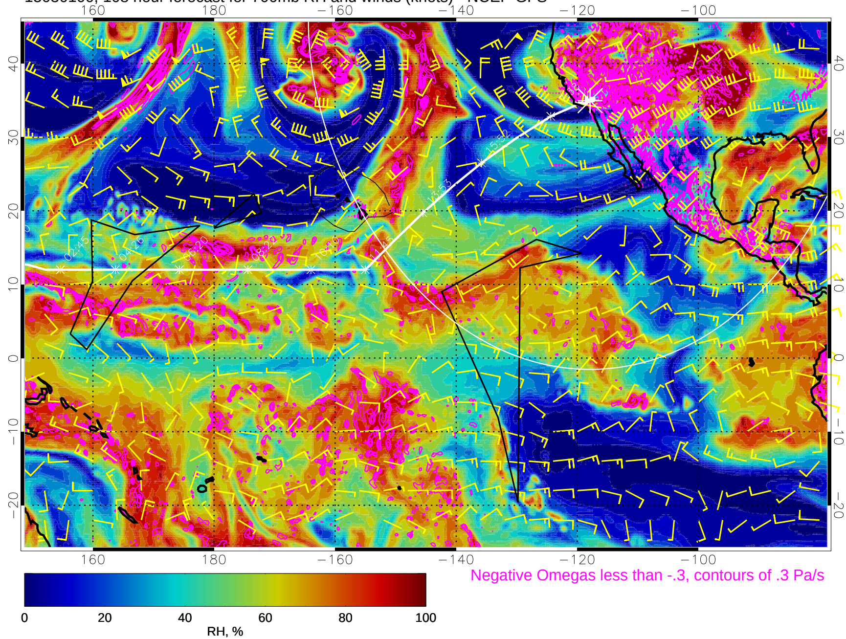
15030100, 108 hour forecast for 700mb RH and winds (knots) - NCEP GFS
