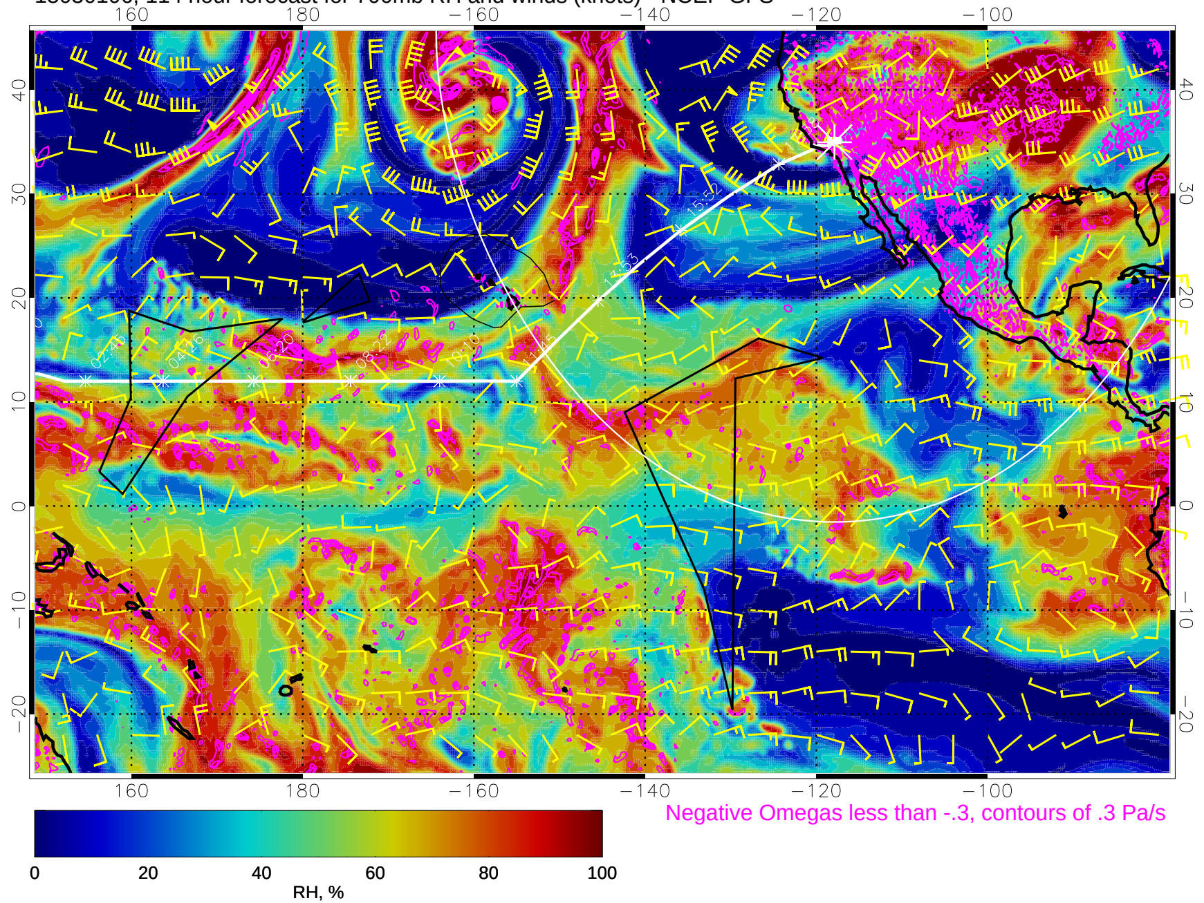
15030106, 114 hour forecast for 700mb RH and winds (knots) - NCEP GFS
