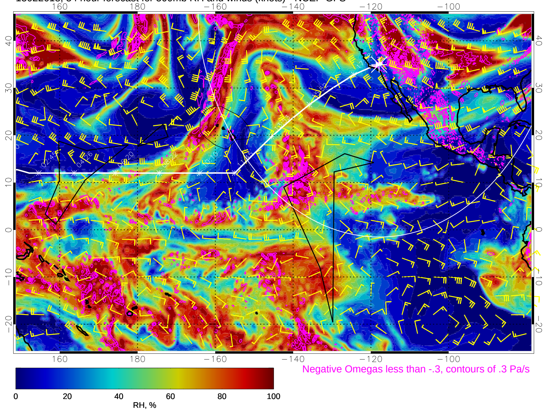
15022618, 54 hour forecast for 500mb RH and winds (knots) - NCEP GFS
