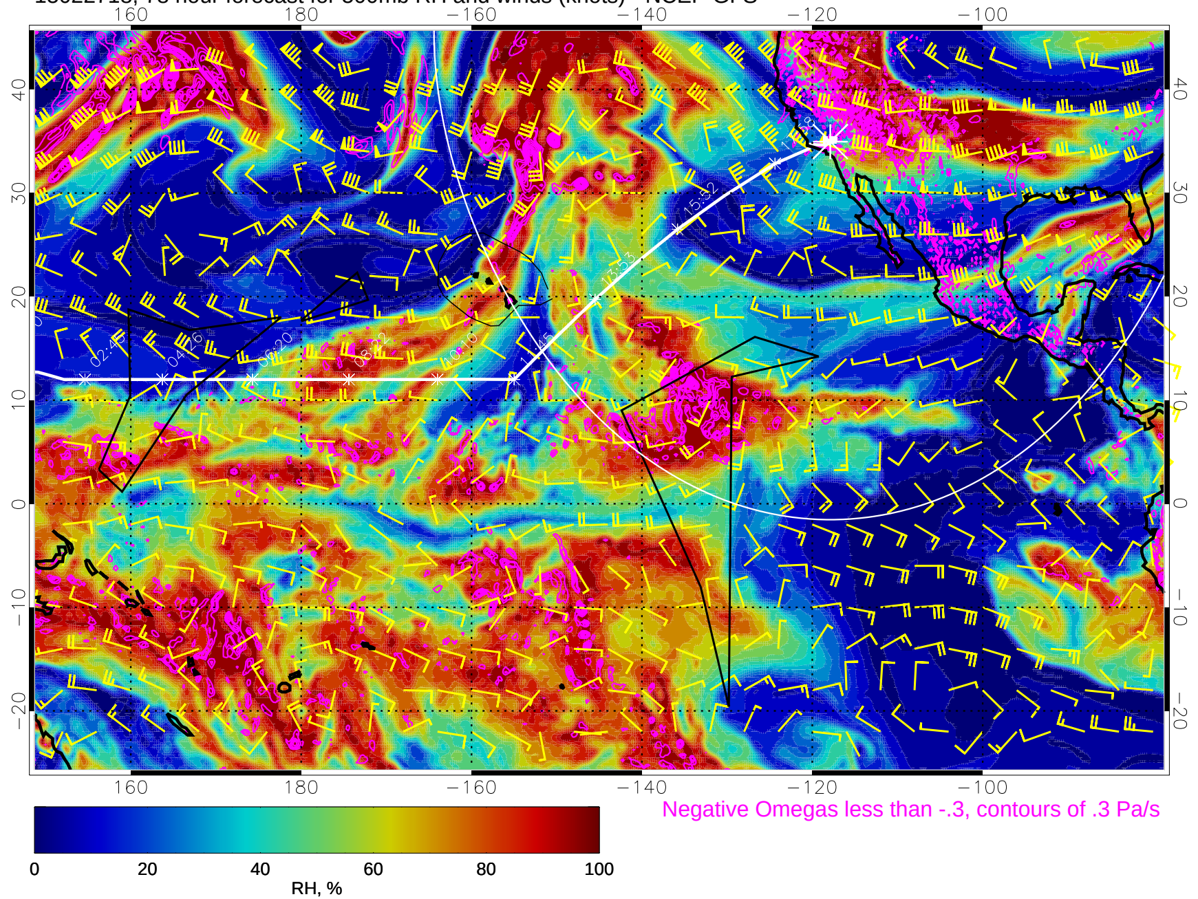
15022718, 78 hour forecast for 500mb RH and winds (knots) - NCEP GFS
