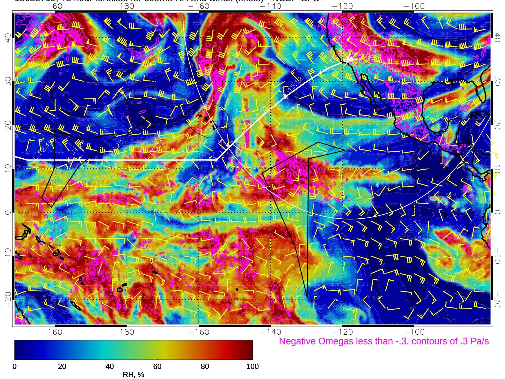
15022712, 72 hour forecast for 500mb RH and winds (knots) - NCEP GFS
