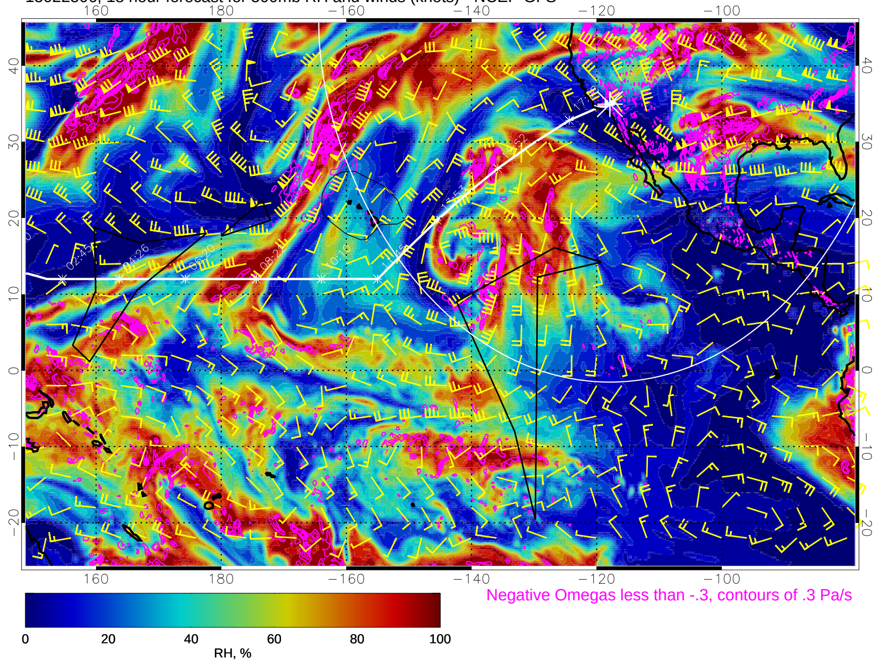
15022506, 18 hour forecast for 500mb RH and winds (knots) - NCEP GFS
