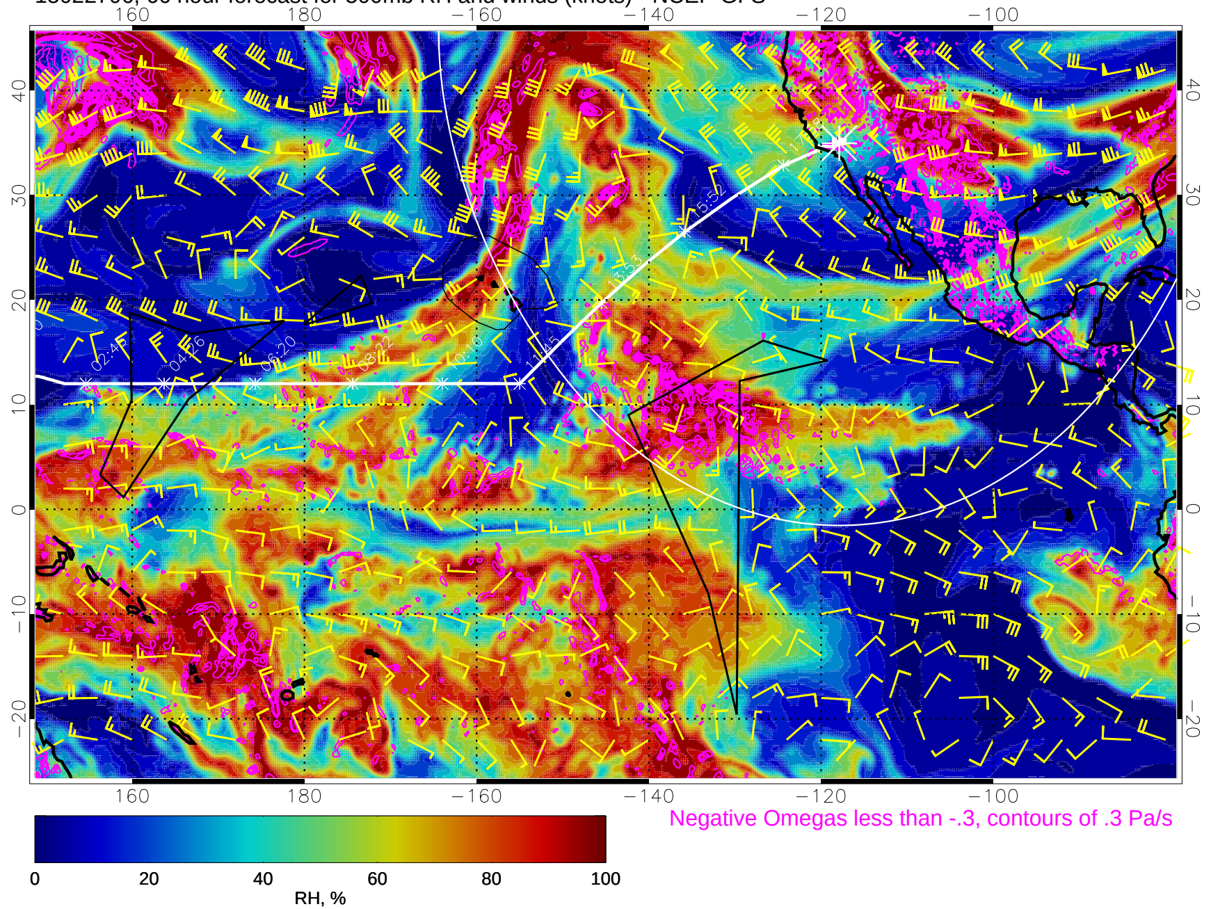
15022706, 66 hour forecast for 500mb RH and winds (knots) - NCEP GFS
