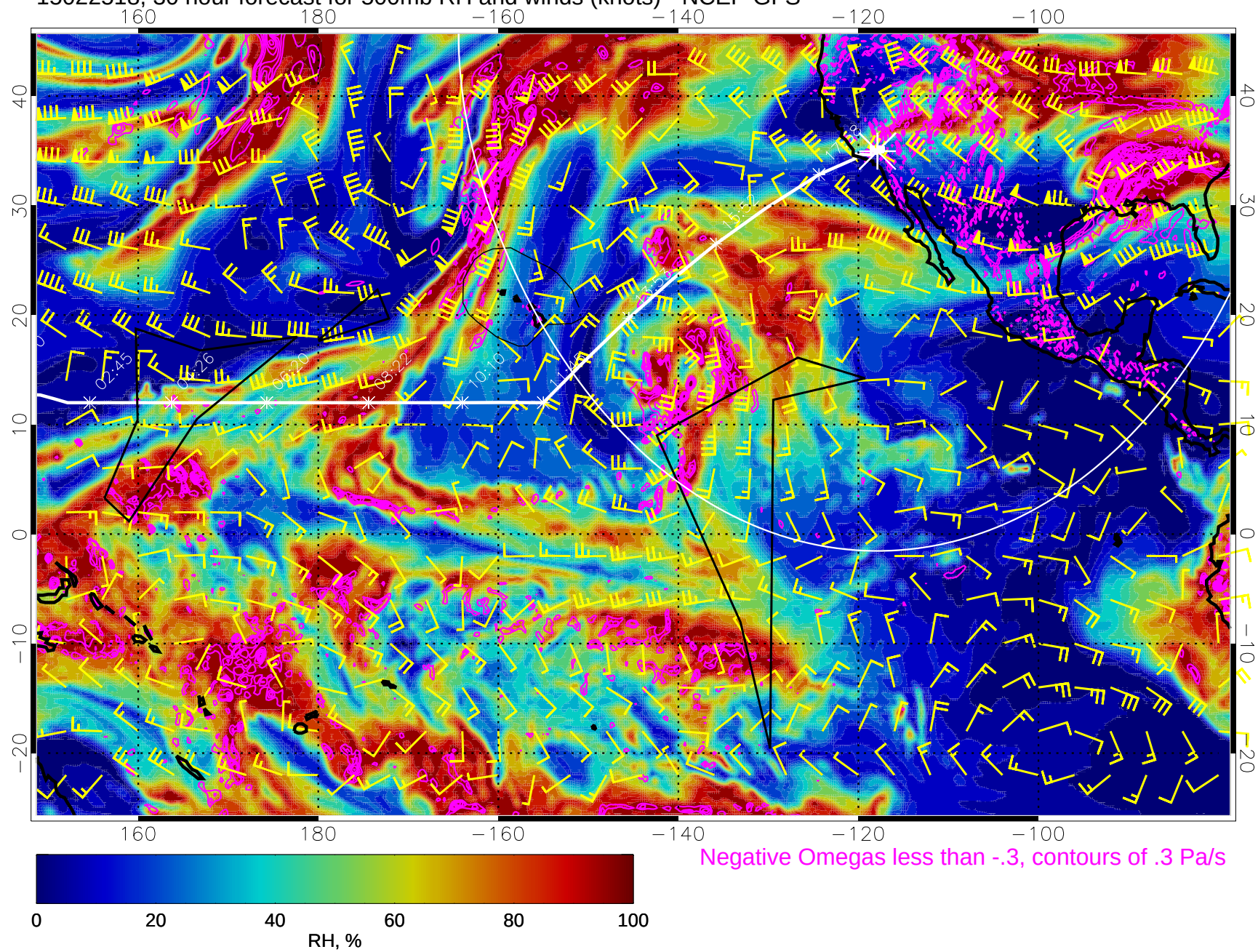
15022518, 30 hour forecast for 500mb RH and winds (knots) - NCEP GFS
