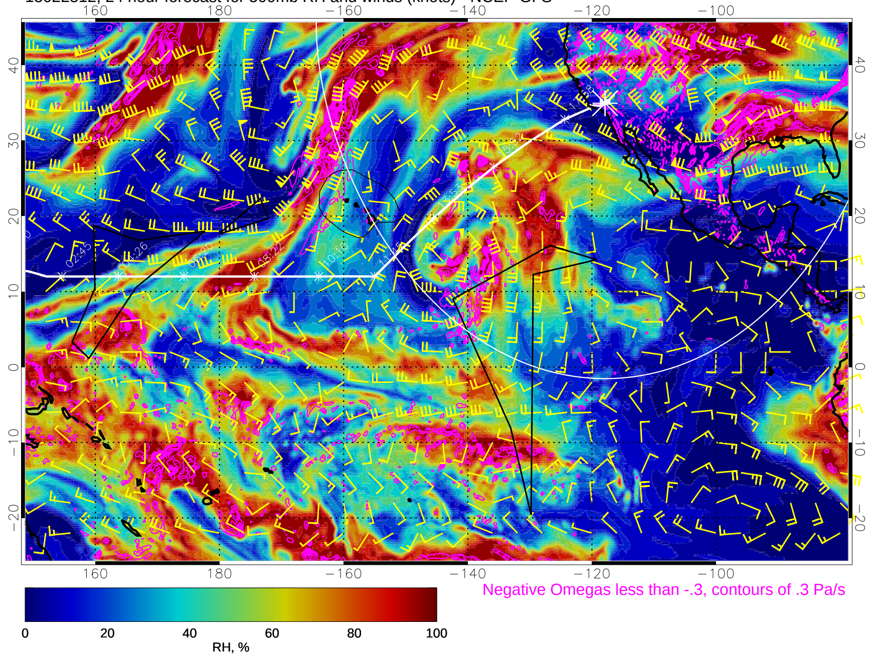
15022512, 24 hour forecast for 500mb RH and winds (knots) - NCEP GFS
