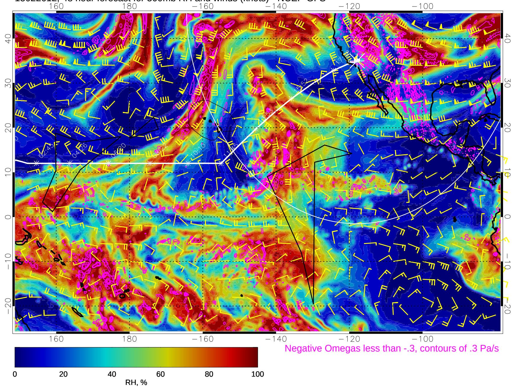
15022612, 48 hour forecast for 500mb RH and winds (knots) - NCEP GFS
