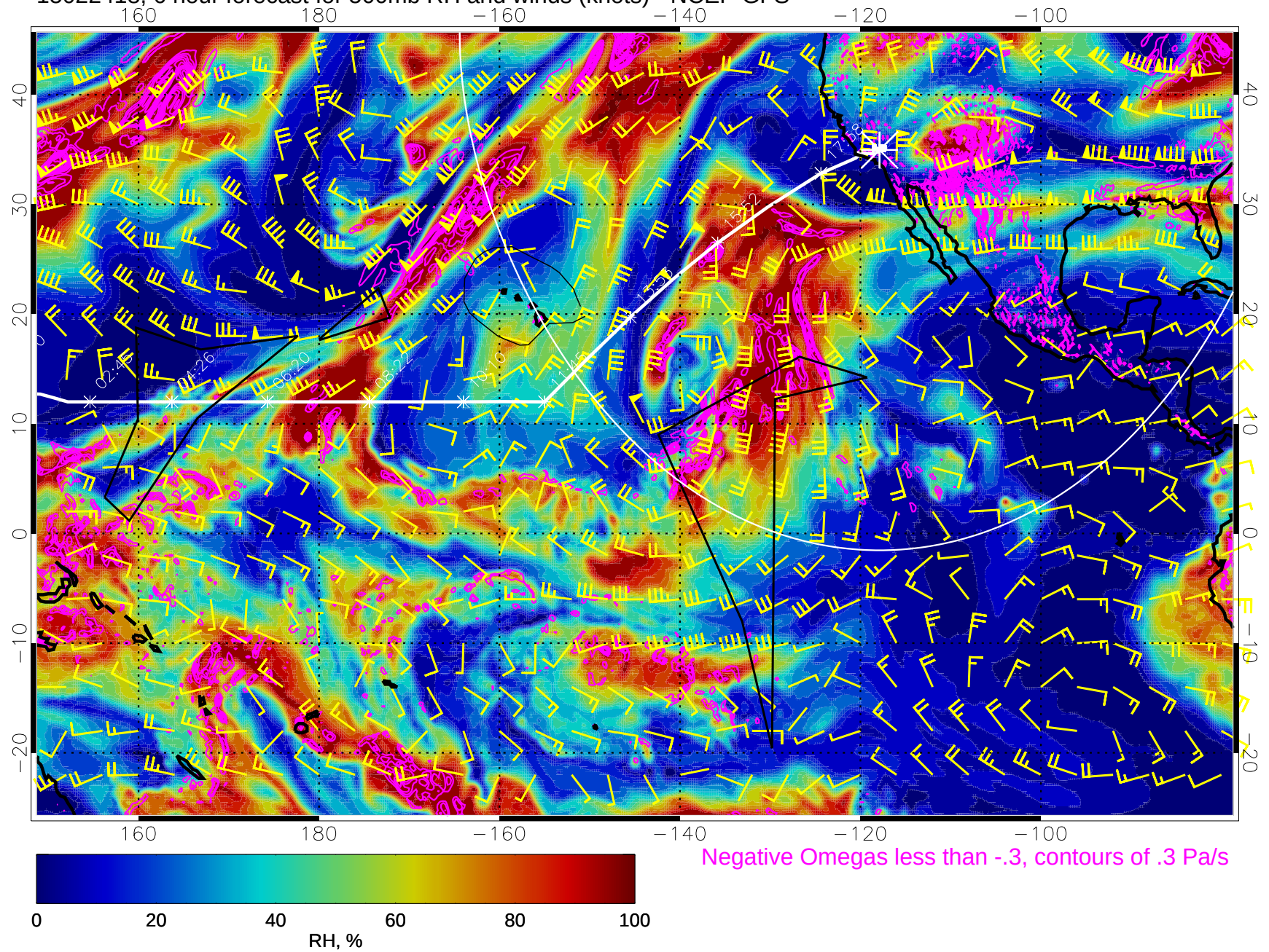
15022418, 6 hour forecast for 500mb RH and winds (knots) - NCEP GFS
