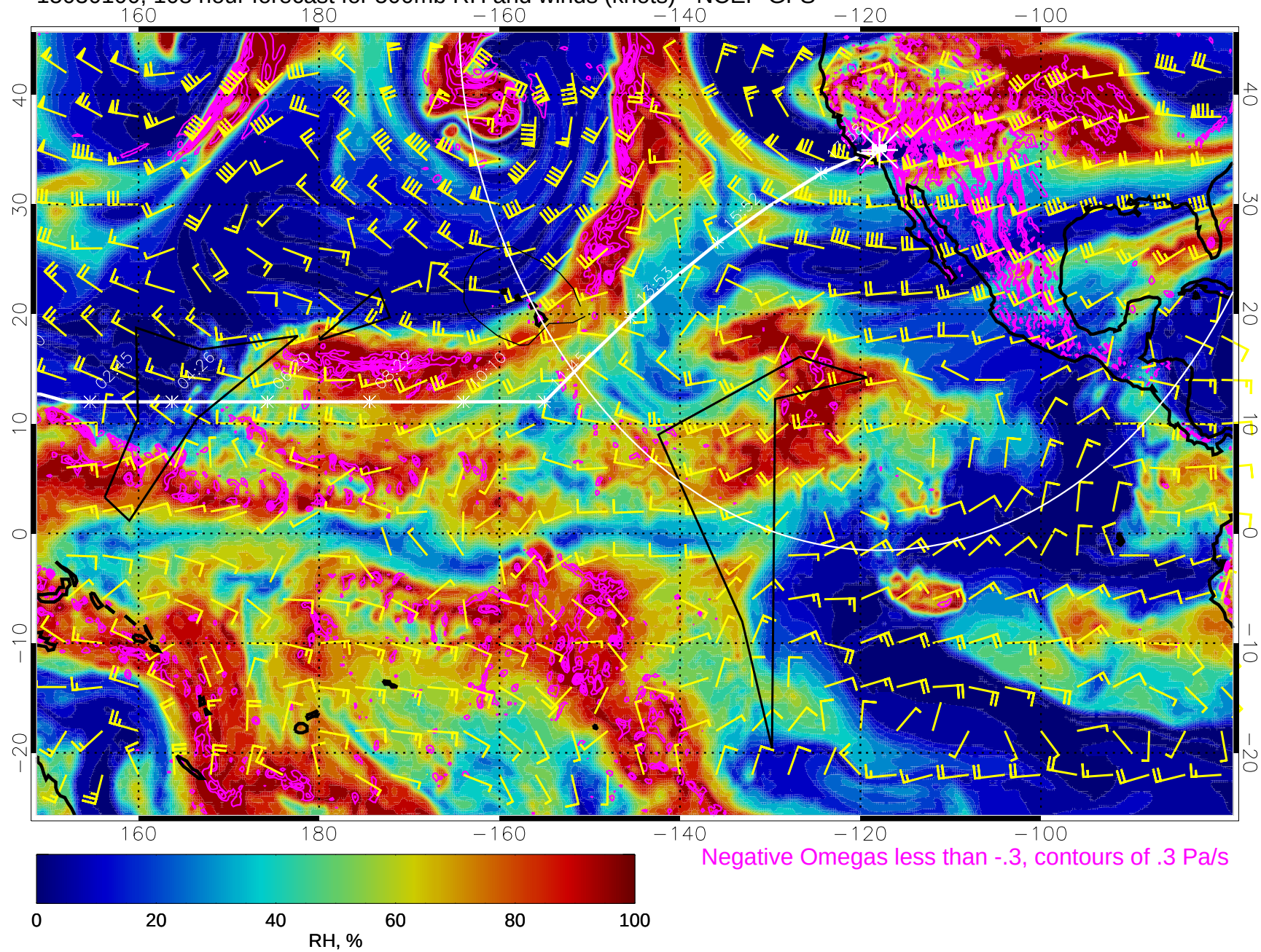
15030100, 108 hour forecast for 500mb RH and winds (knots) - NCEP GFS
