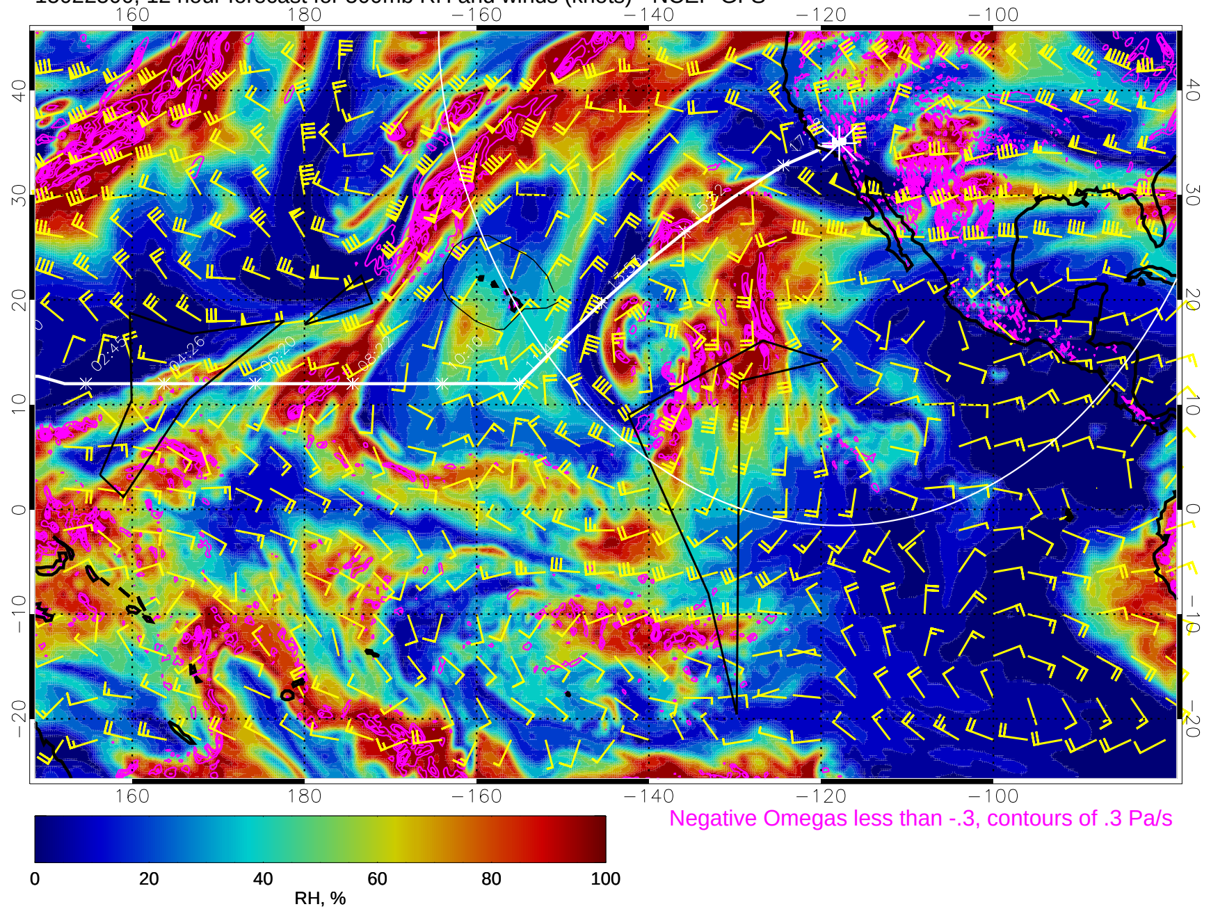
15022500, 12 hour forecast for 500mb RH and winds (knots) - NCEP GFS
