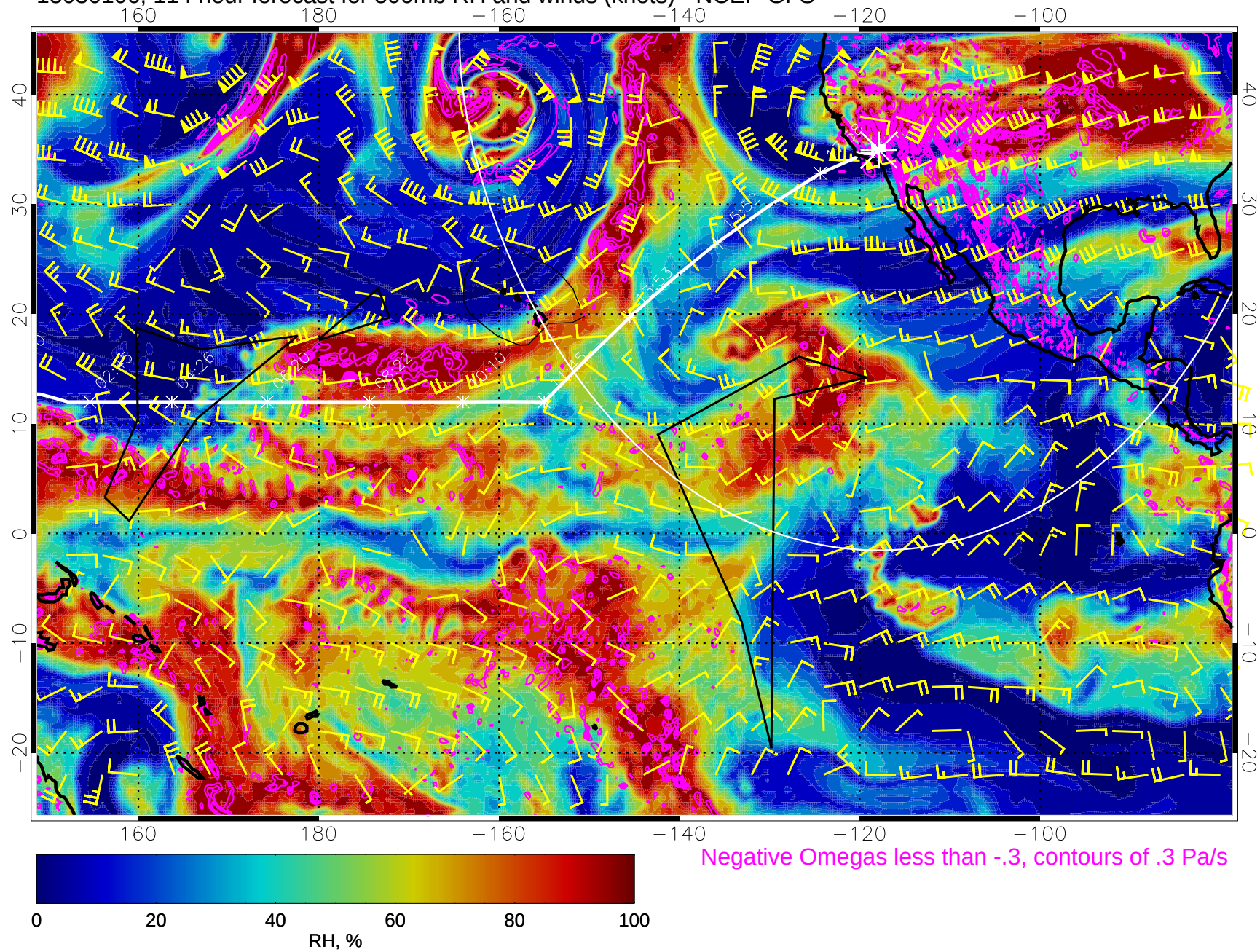
15030106, 114 hour forecast for 500mb RH and winds (knots) - NCEP GFS
