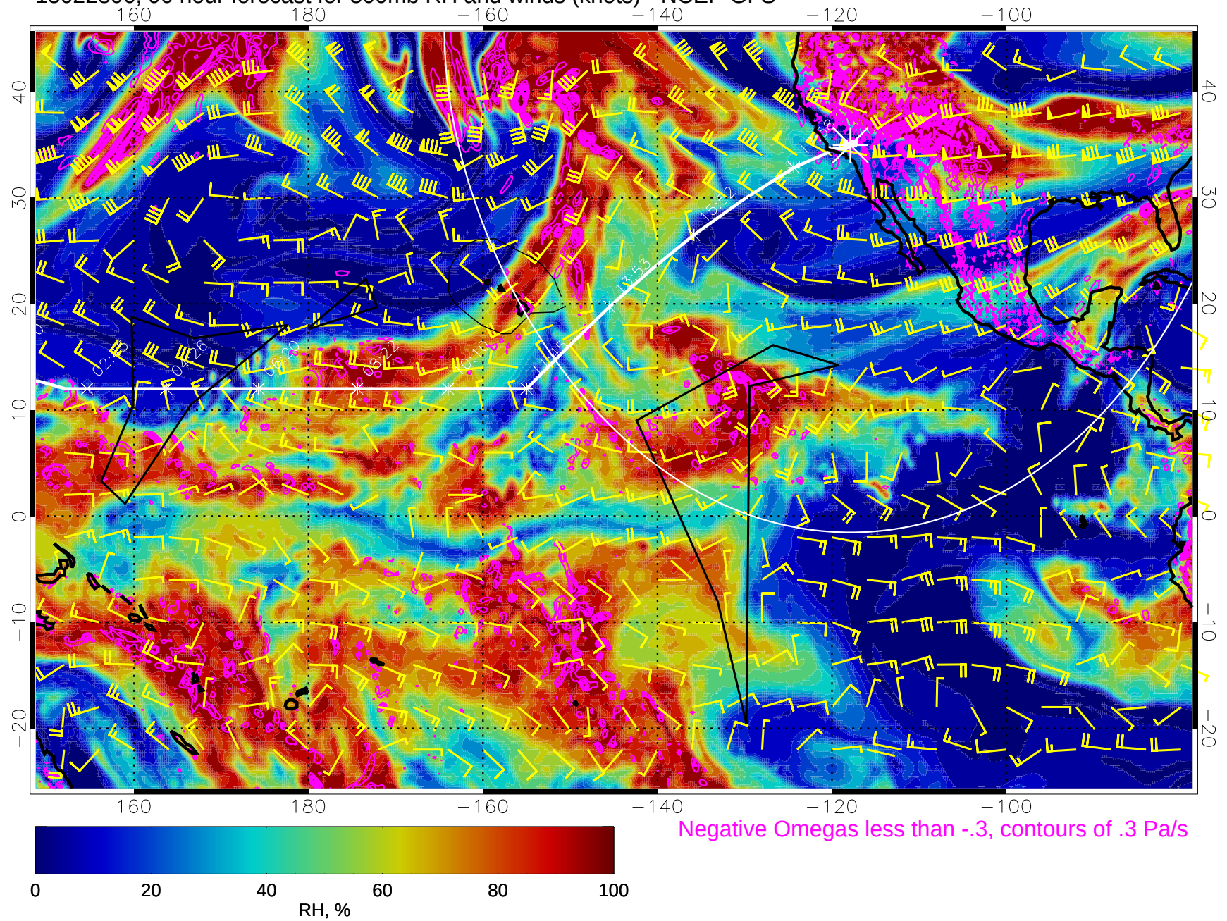
15022806, 90 hour forecast for 500mb RH and winds (knots) - NCEP GFS
