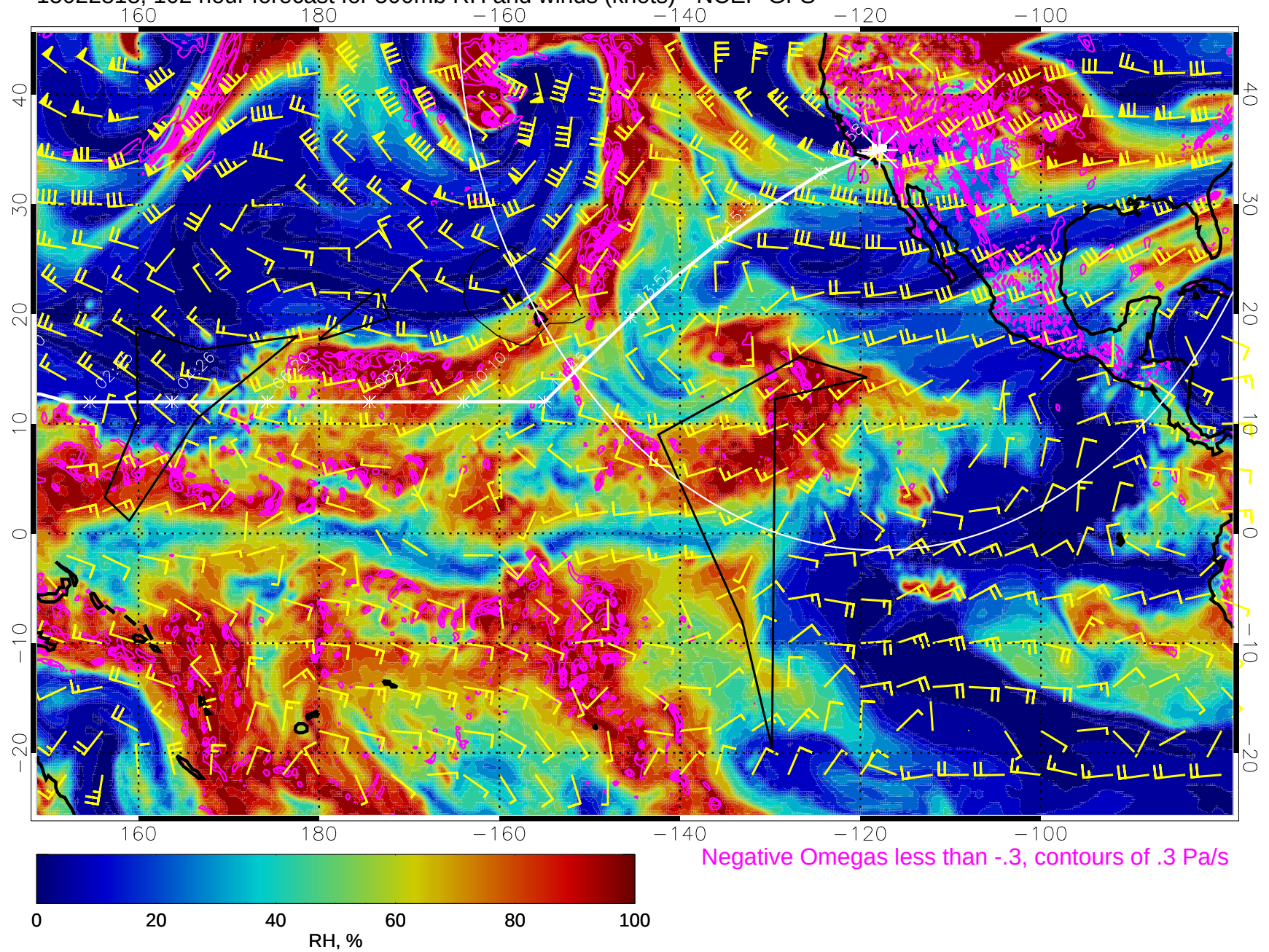
15022818, 102 hour forecast for 500mb RH and winds (knots) - NCEP GFS
