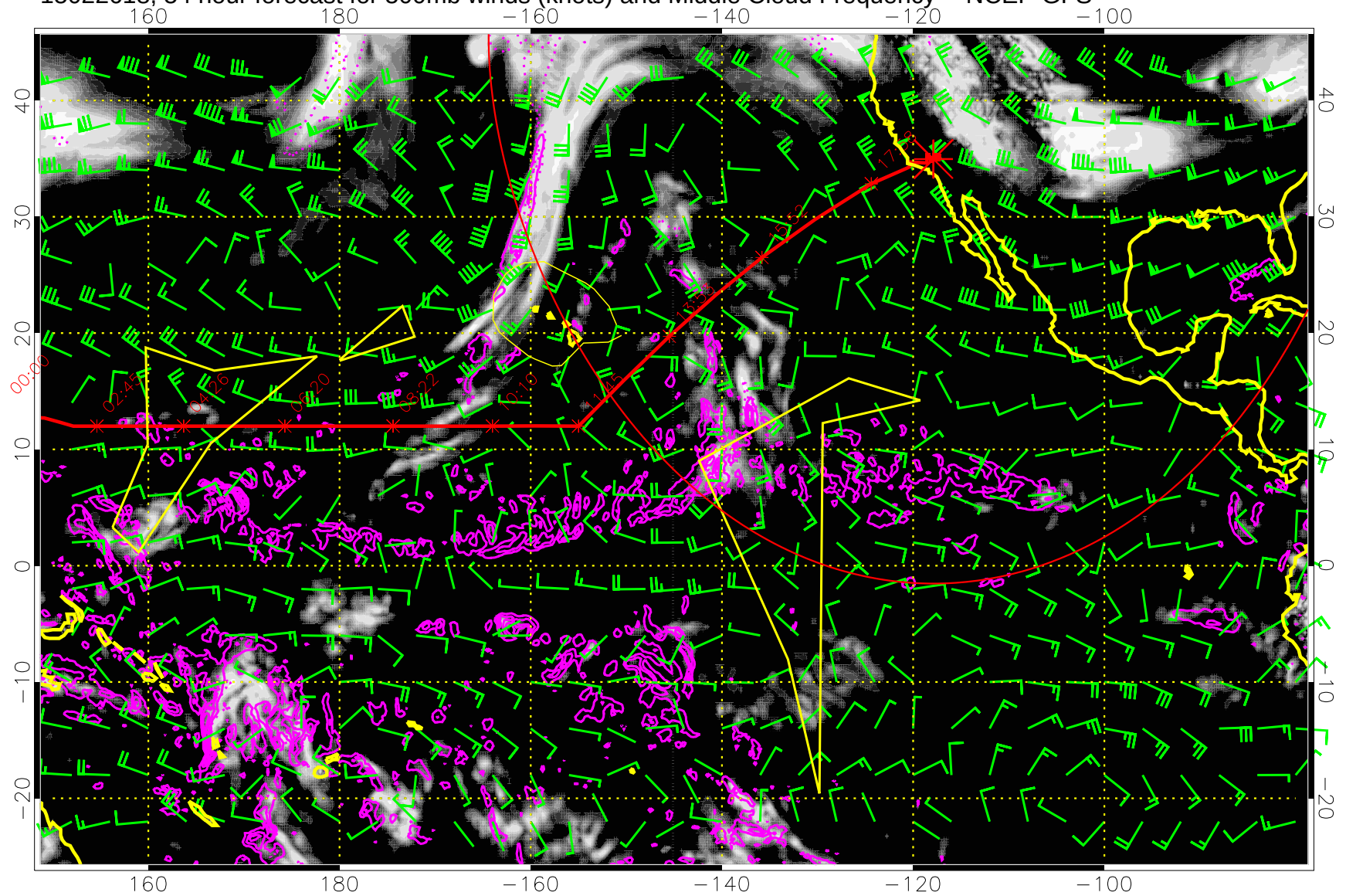
15022618, 54 hour forecast for 500mb winds (knots) and Middle Cloud Frequency -- NCEP GFS
