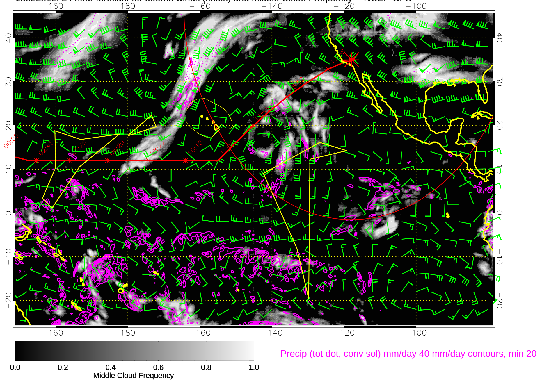
15022512, 24 hour forecast for 500mb winds (knots) and Middle Cloud Frequency -- NCEP GFS
