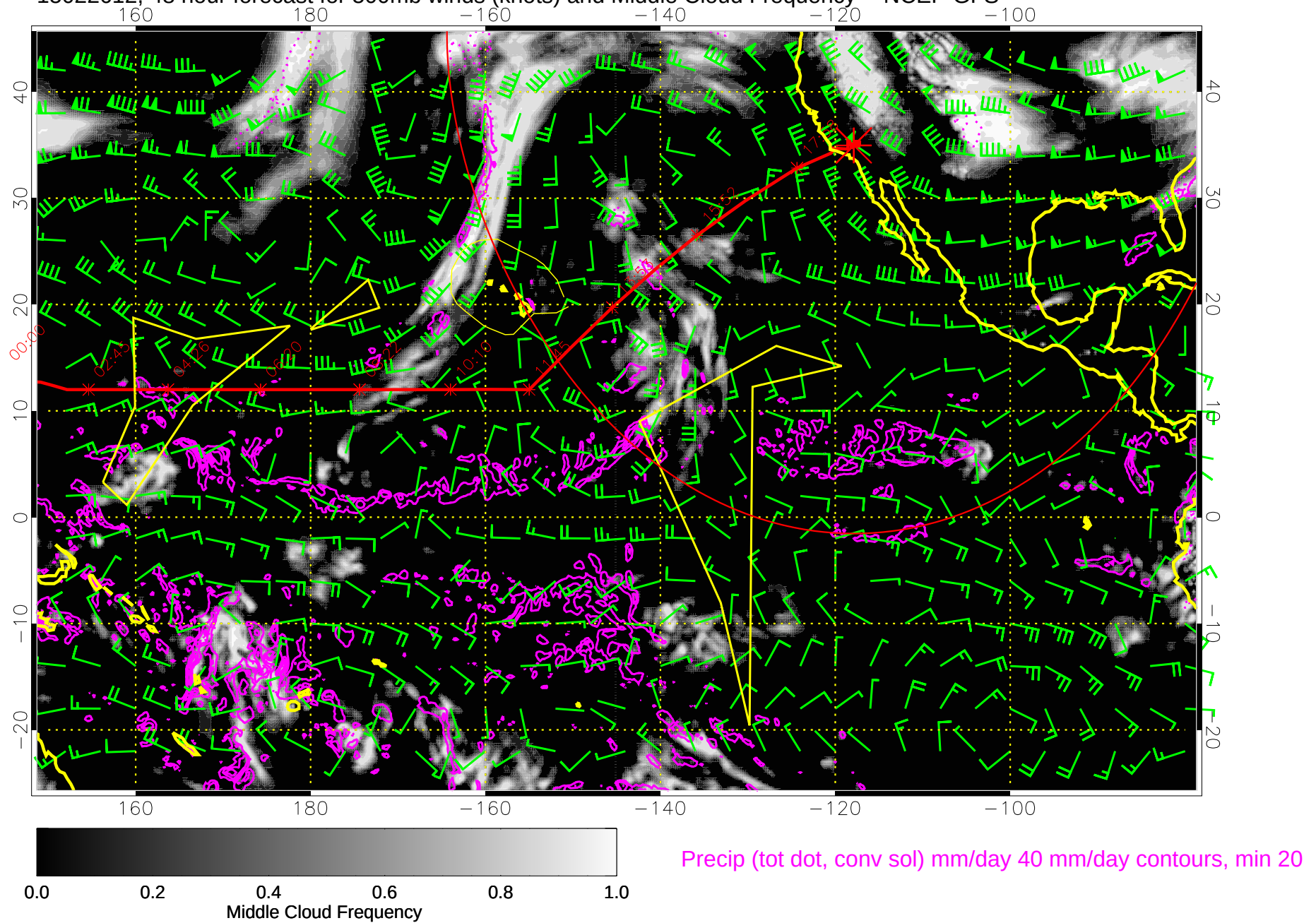
15022612, 48 hour forecast for 500mb winds (knots) and Middle Cloud Frequency -- NCEP GFS
