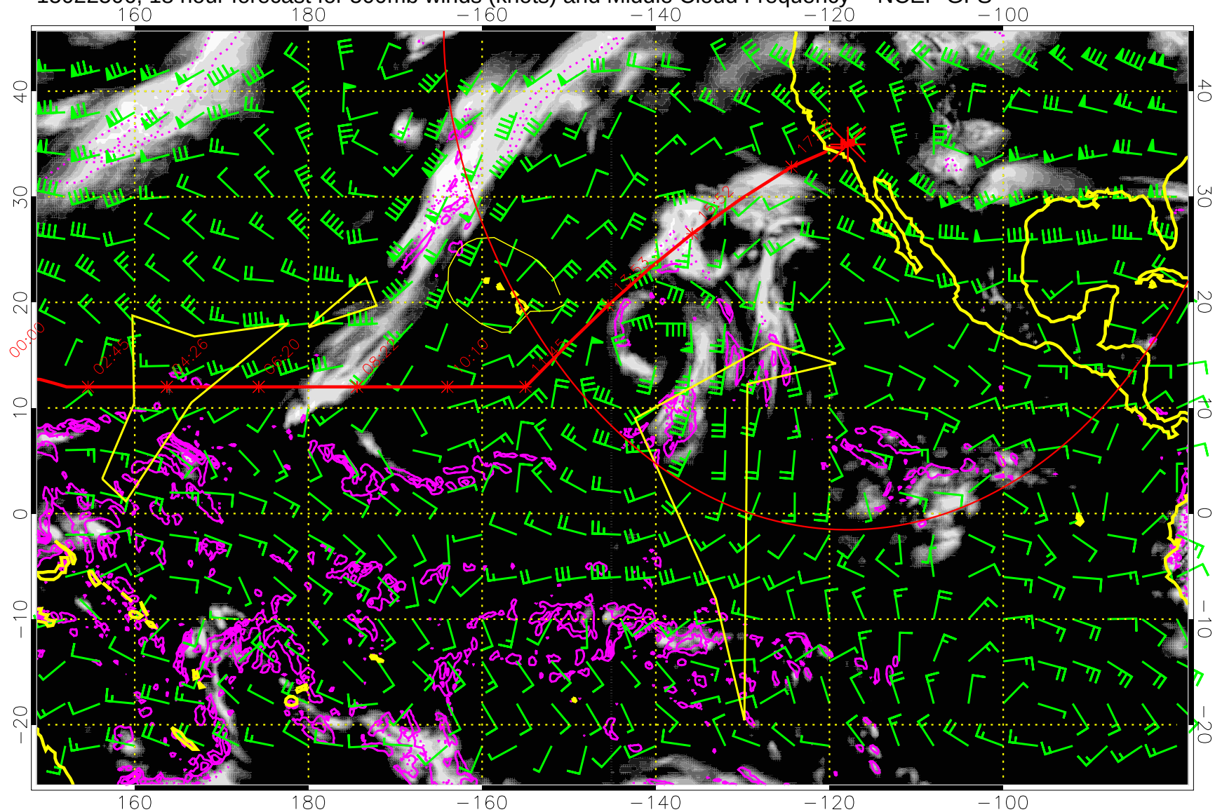
15022506, 18 hour forecast for 500mb winds (knots) and Middle Cloud Frequency -- NCEP GFS
