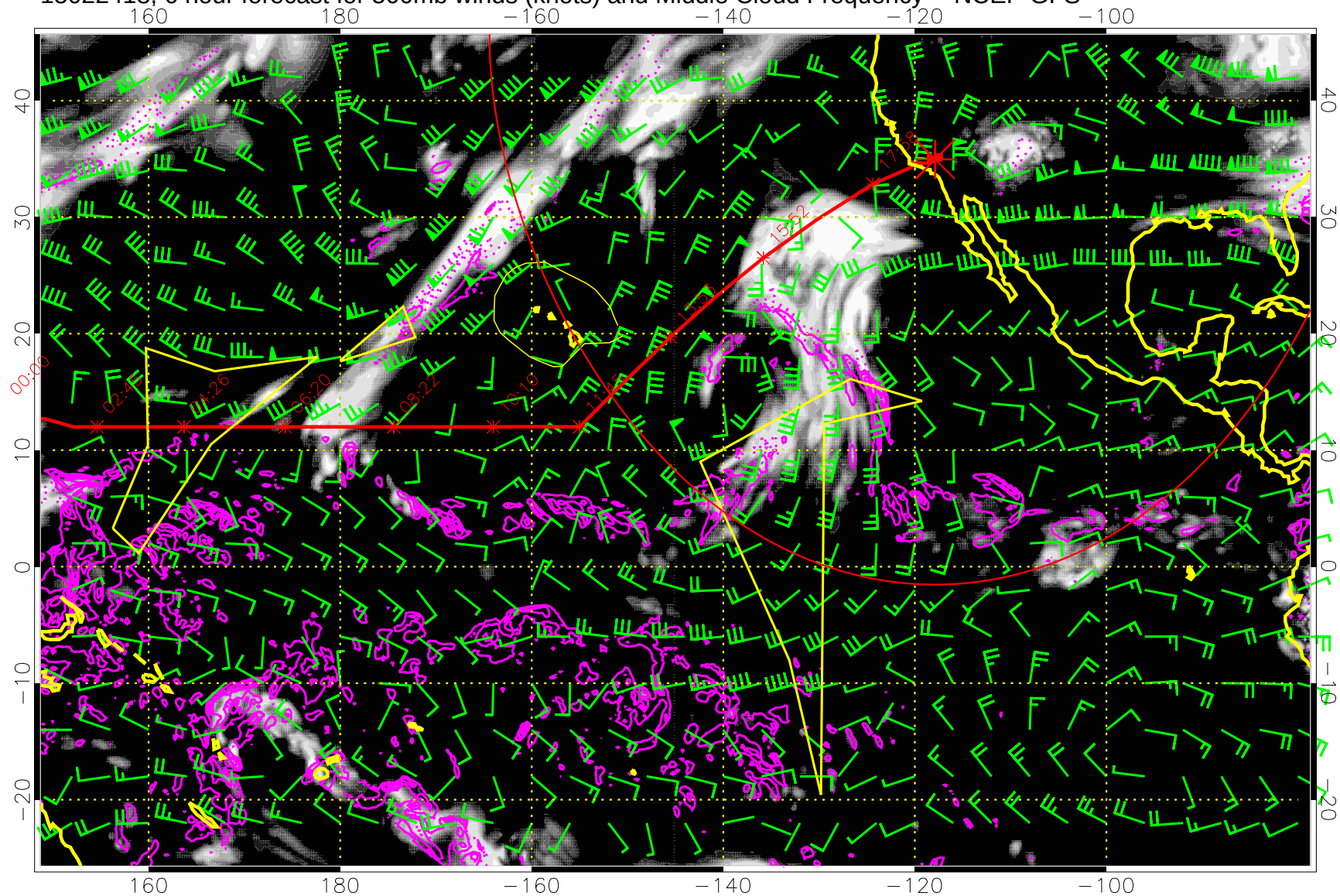
15022418, 6 hour forecast for 500mb winds (knots) and Middle Cloud Frequency -- NCEP GFS
