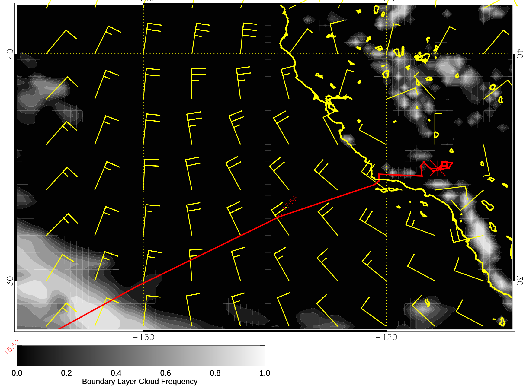
15030112, 120 hour forecast for surface winds (knots) and Boundary Layer Cloud Frequency -- NCEP GFS
