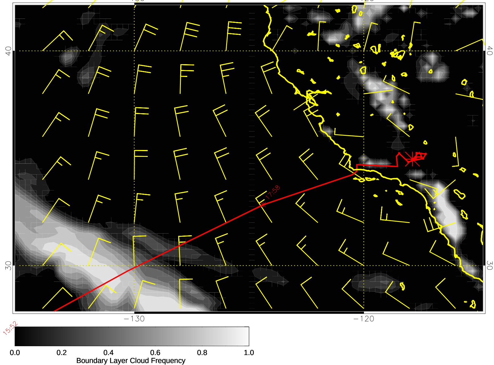
15030106, 114 hour forecast for surface winds (knots) and Boundary Layer Cloud Frequency -- NCEP GFS
