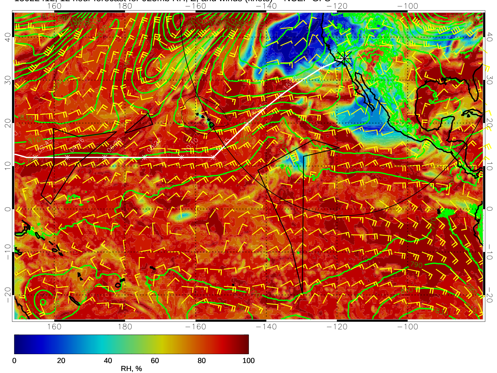
15022412, 12 hour forecast for 925mb RH, Z, and winds (knots) -- NCEP GFS
