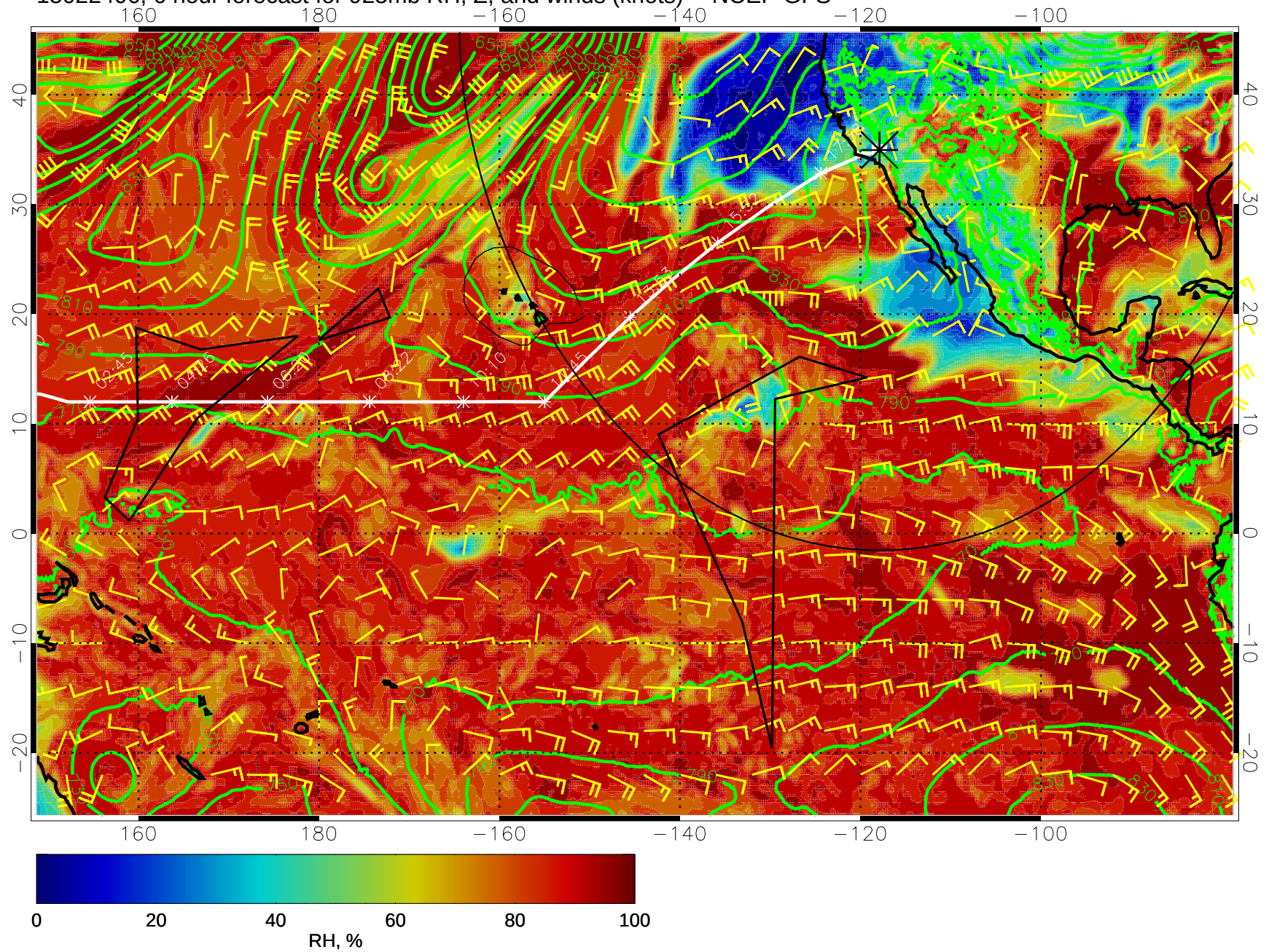
15022406, 6 hour forecast for 925mb RH, Z, and winds (knots) -- NCEP GFS
