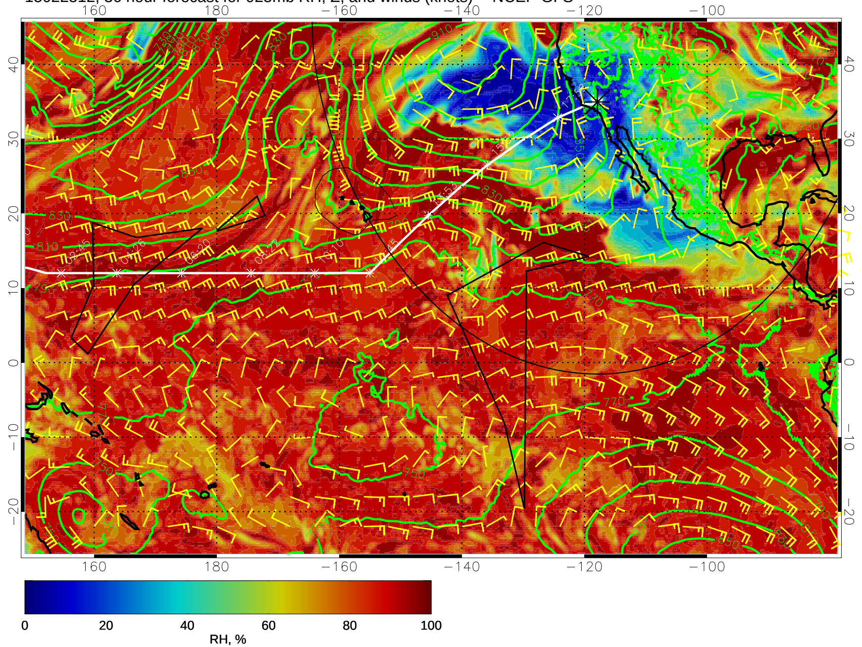
15022512, 36 hour forecast for 925mb RH, Z, and winds (knots) -- NCEP GFS
