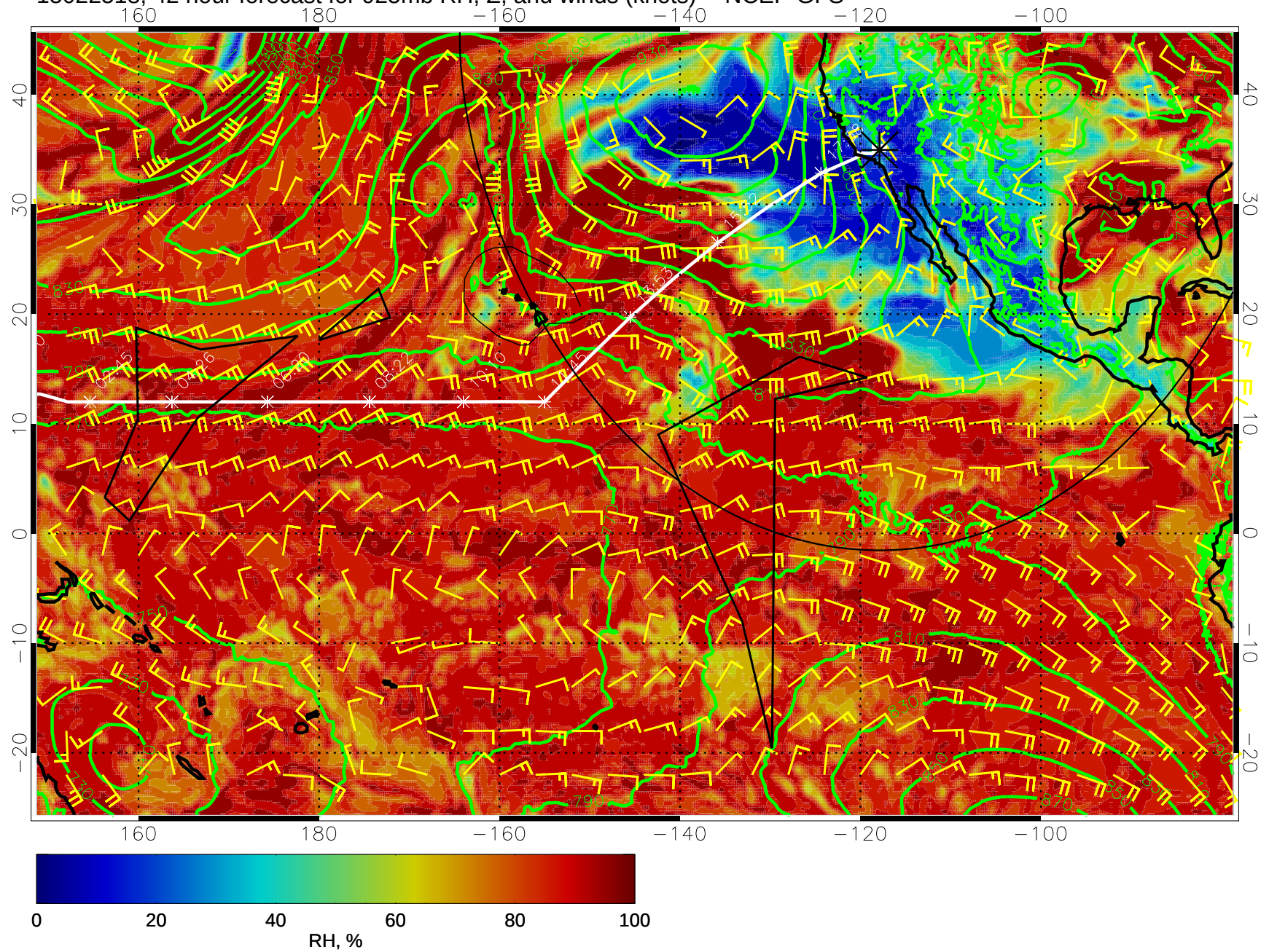
15022518, 42 hour forecast for 925mb RH, Z, and winds (knots) -- NCEP GFS
