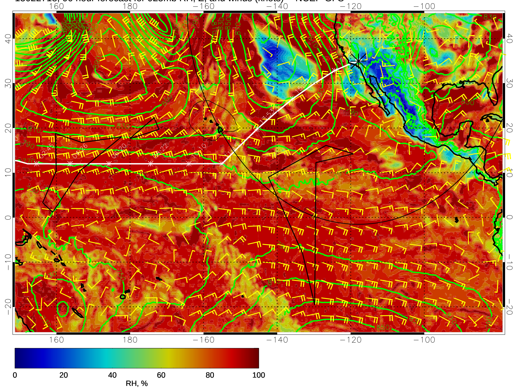
15022718, 90 hour forecast for 925mb RH, Z, and winds (knots) -- NCEP GFS
