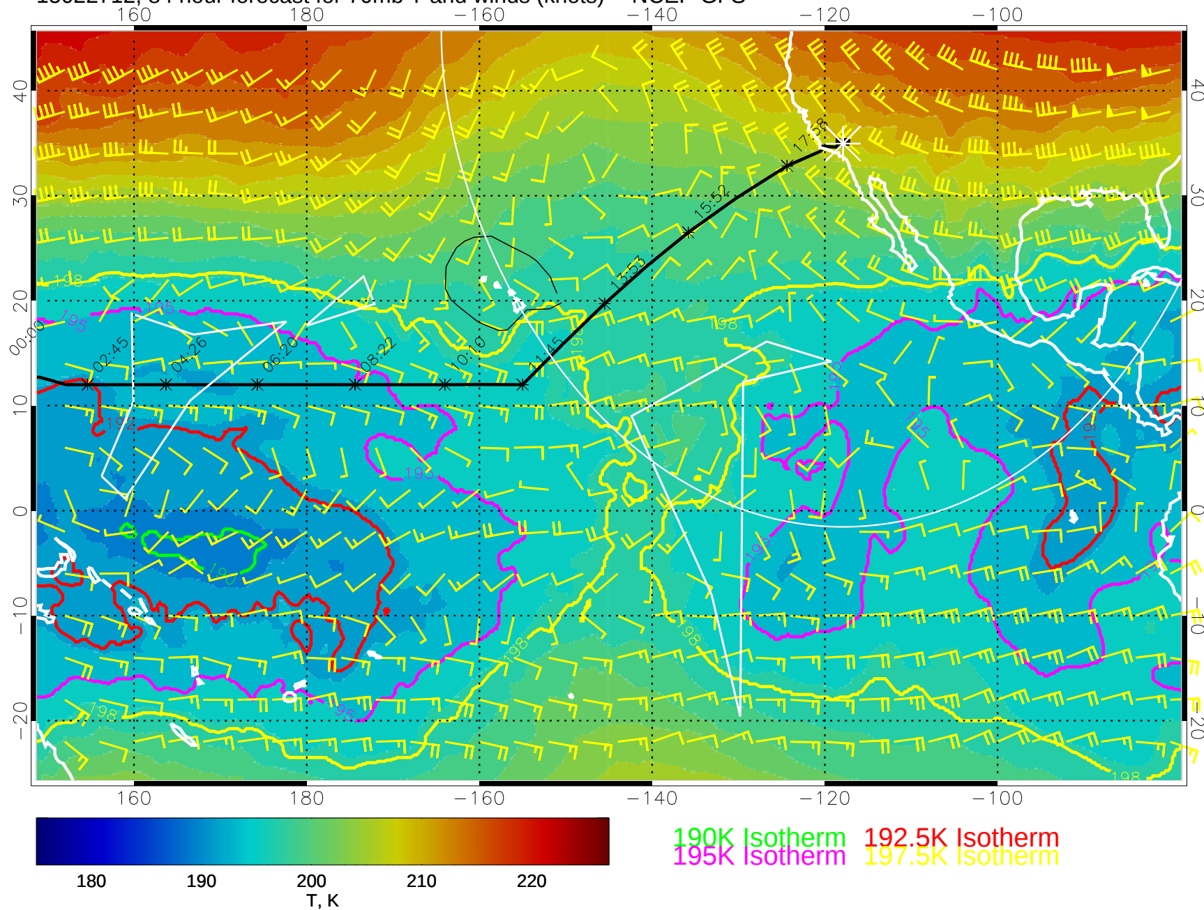
15022712, 84 hour forecast for 70mb T and winds (knots) -- NCEP GFS
