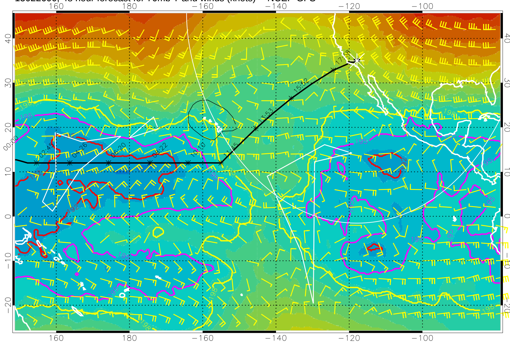
15022600, 48 hour forecast for 70mb T and winds (knots) -- NCEP GFS
