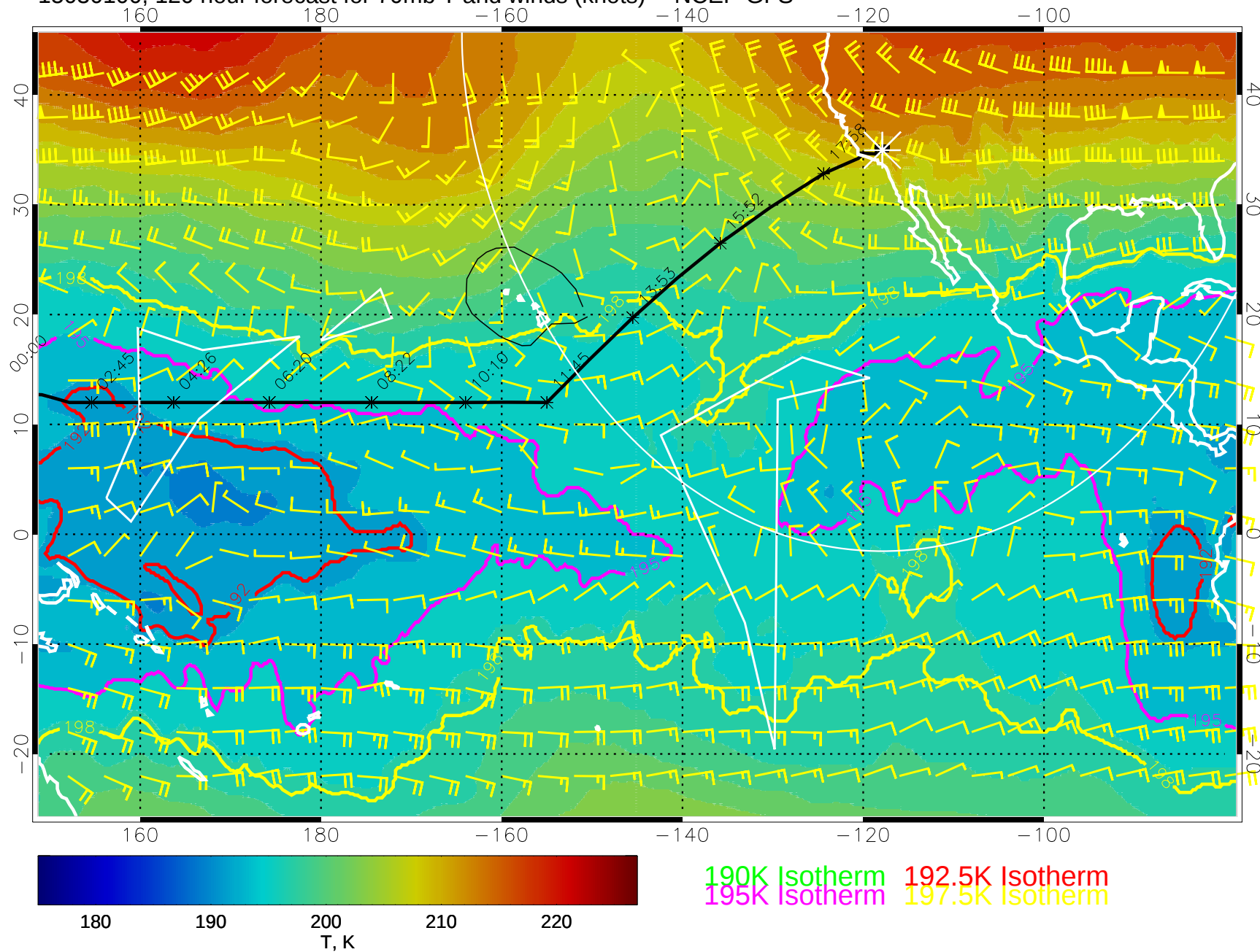
15030100, 120 hour forecast for 70mb T and winds (knots) -- NCEP GFS
