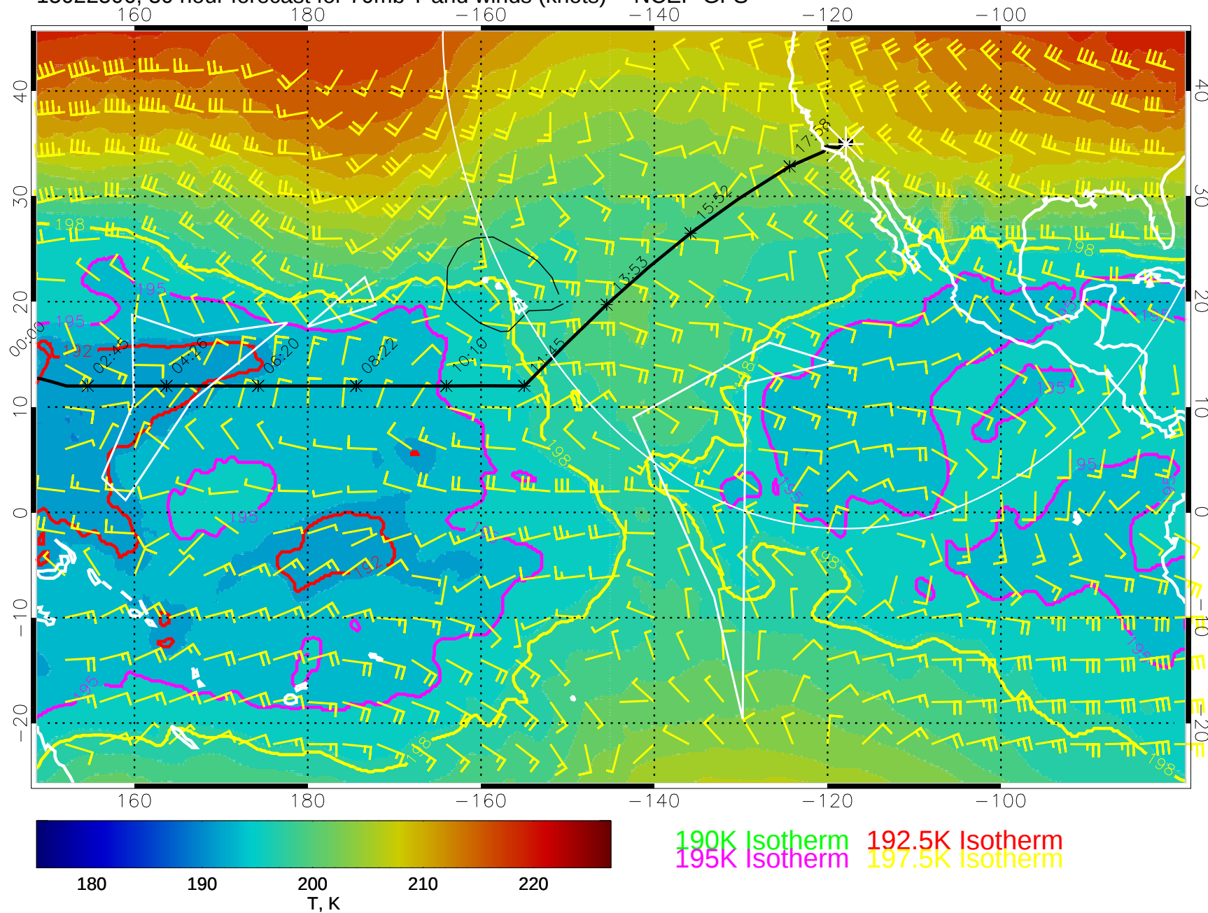
15022506, 30 hour forecast for 70mb T and winds (knots) -- NCEP GFS
