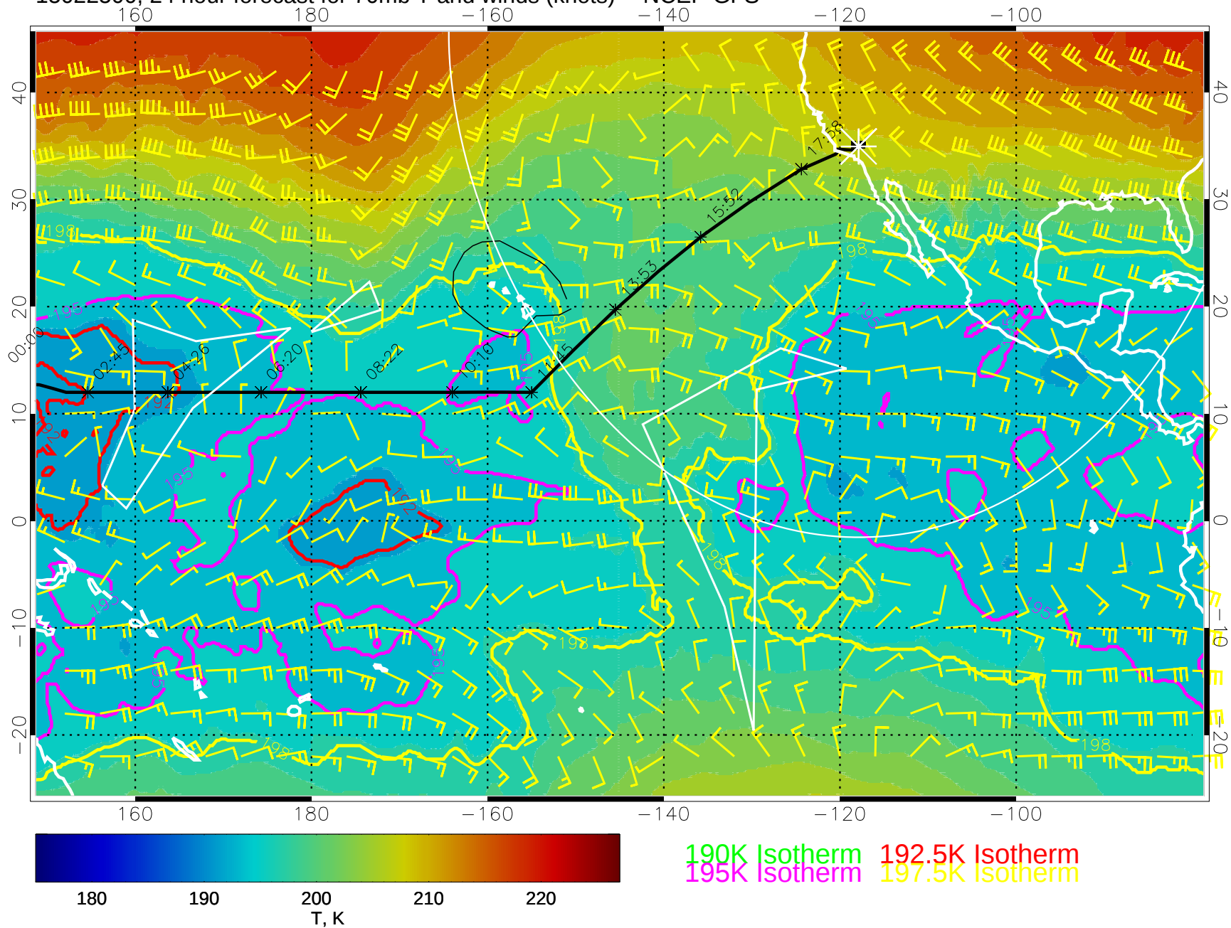
15022500, 24 hour forecast for 70mb T and winds (knots) -- NCEP GFS
