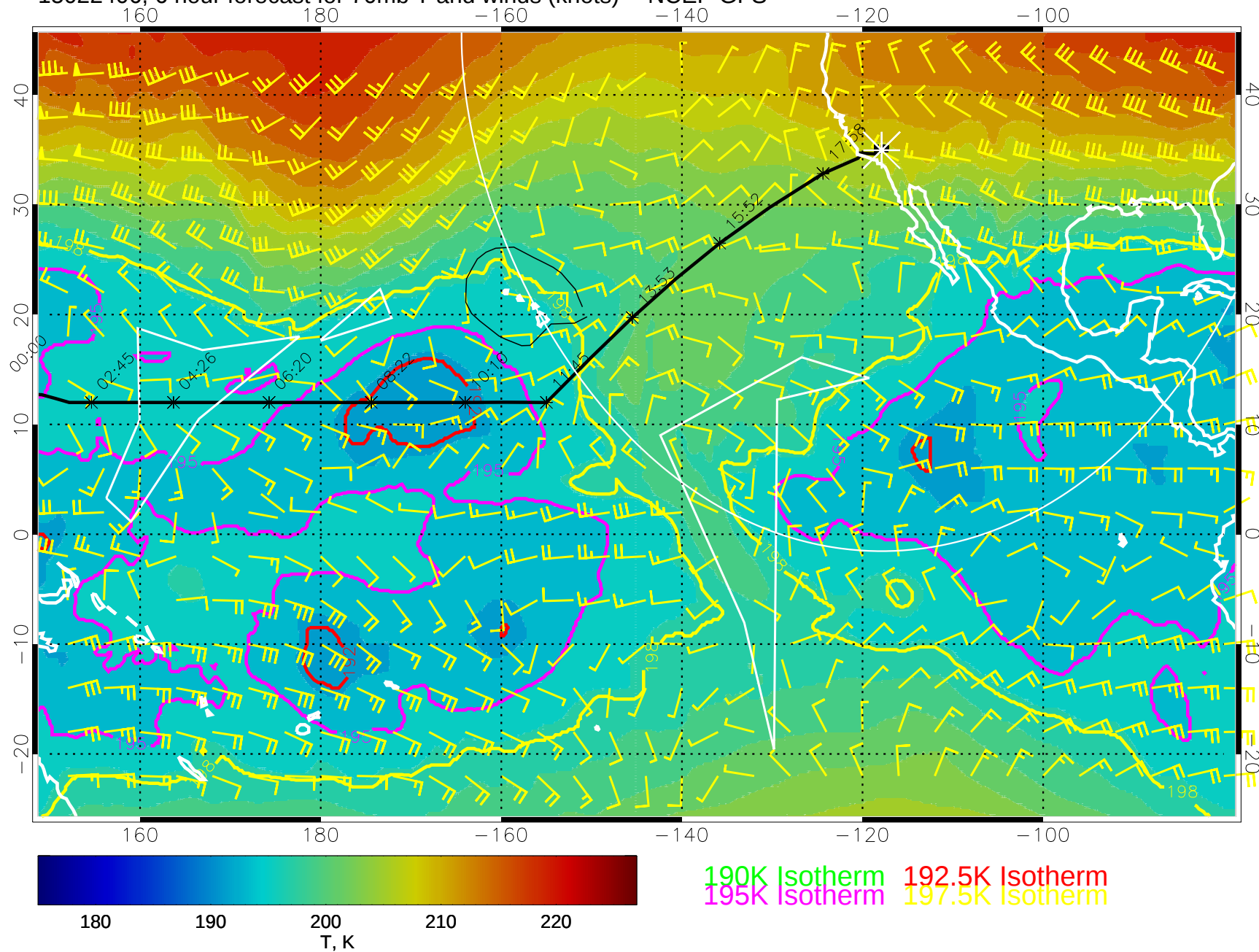
15022406, 6 hour forecast for 70mb T and winds (knots) -- NCEP GFS
