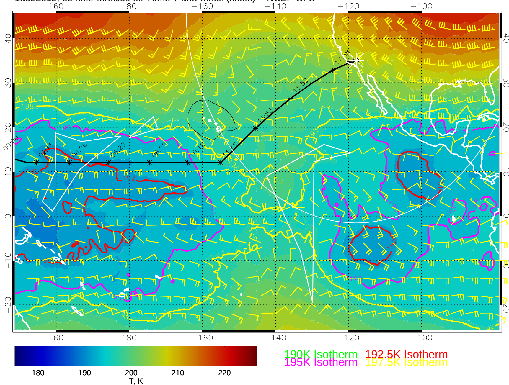
15022612, 60 hour forecast for 70mb T and winds (knots) -- NCEP GFS
