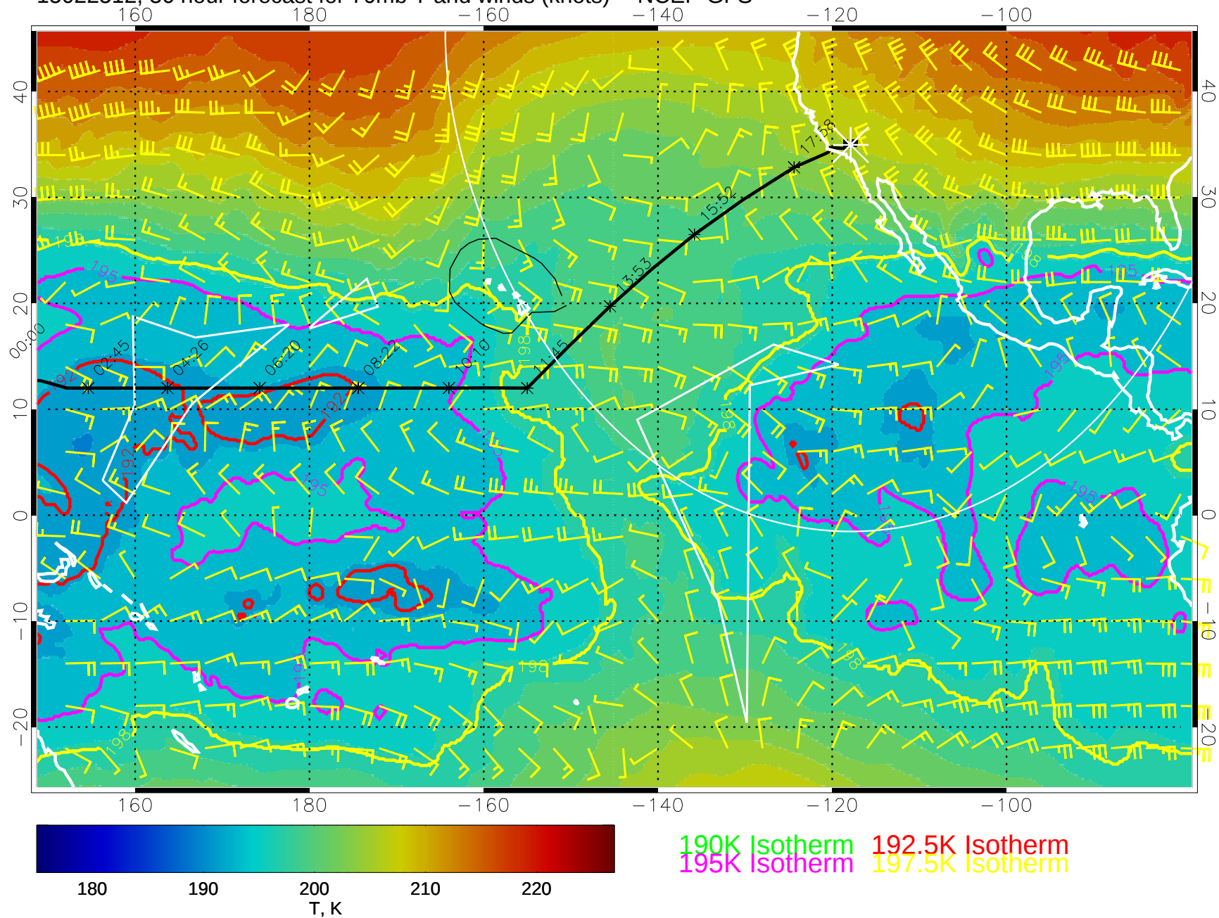
15022512, 36 hour forecast for 70mb T and winds (knots) -- NCEP GFS
