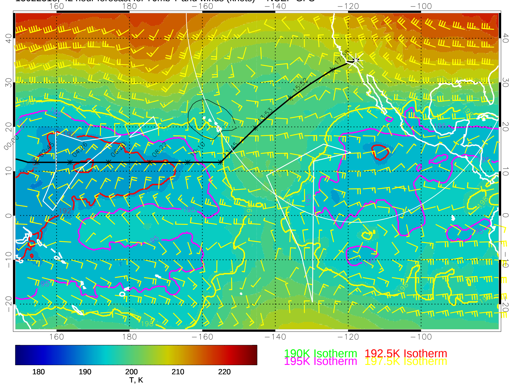
15022518, 42 hour forecast for 70mb T and winds (knots) -- NCEP GFS
