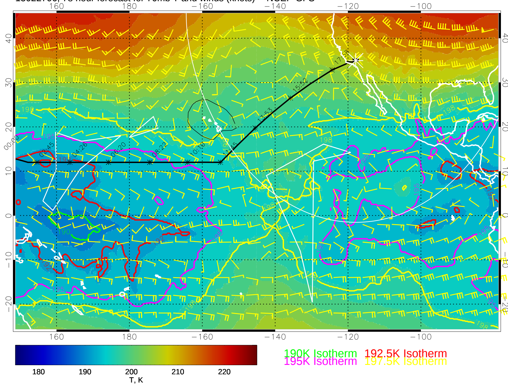
15022706, 78 hour forecast for 70mb T and winds (knots) -- NCEP GFS
