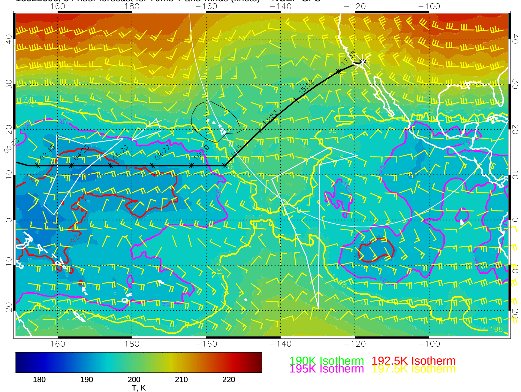
15022606, 54 hour forecast for 70mb T and winds (knots) -- NCEP GFS
