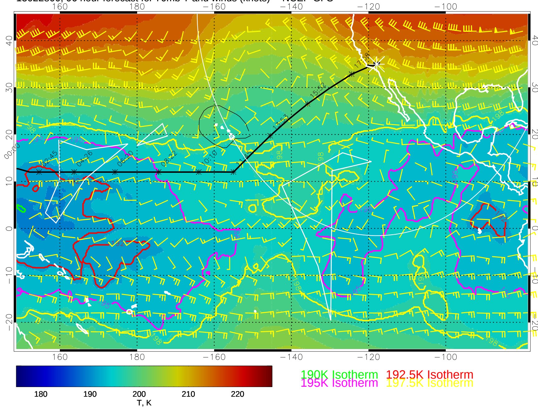
15022800, 96 hour forecast for 70mb T and winds (knots) -- NCEP GFS
