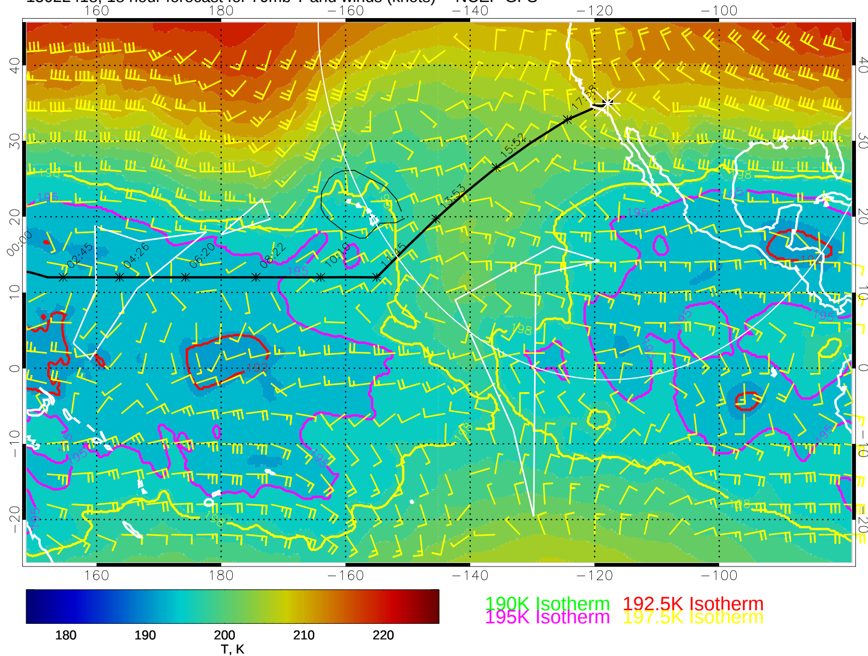
15022418, 18 hour forecast for 70mb T and winds (knots) -- NCEP GFS
