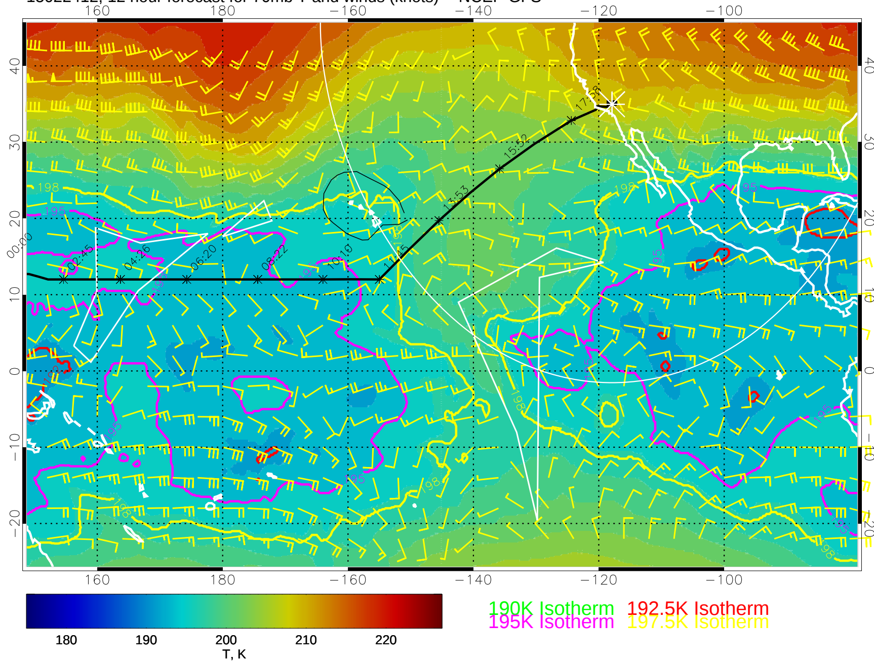
15022412, 12 hour forecast for 70mb T and winds (knots) -- NCEP GFS
