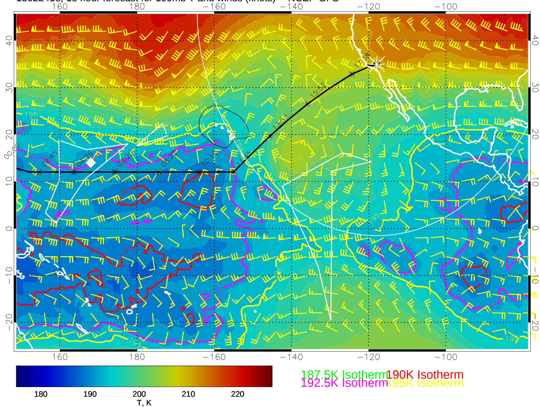
15022418, 18 hour forecast for 100mb T and winds (knots) -- NCEP GFS
