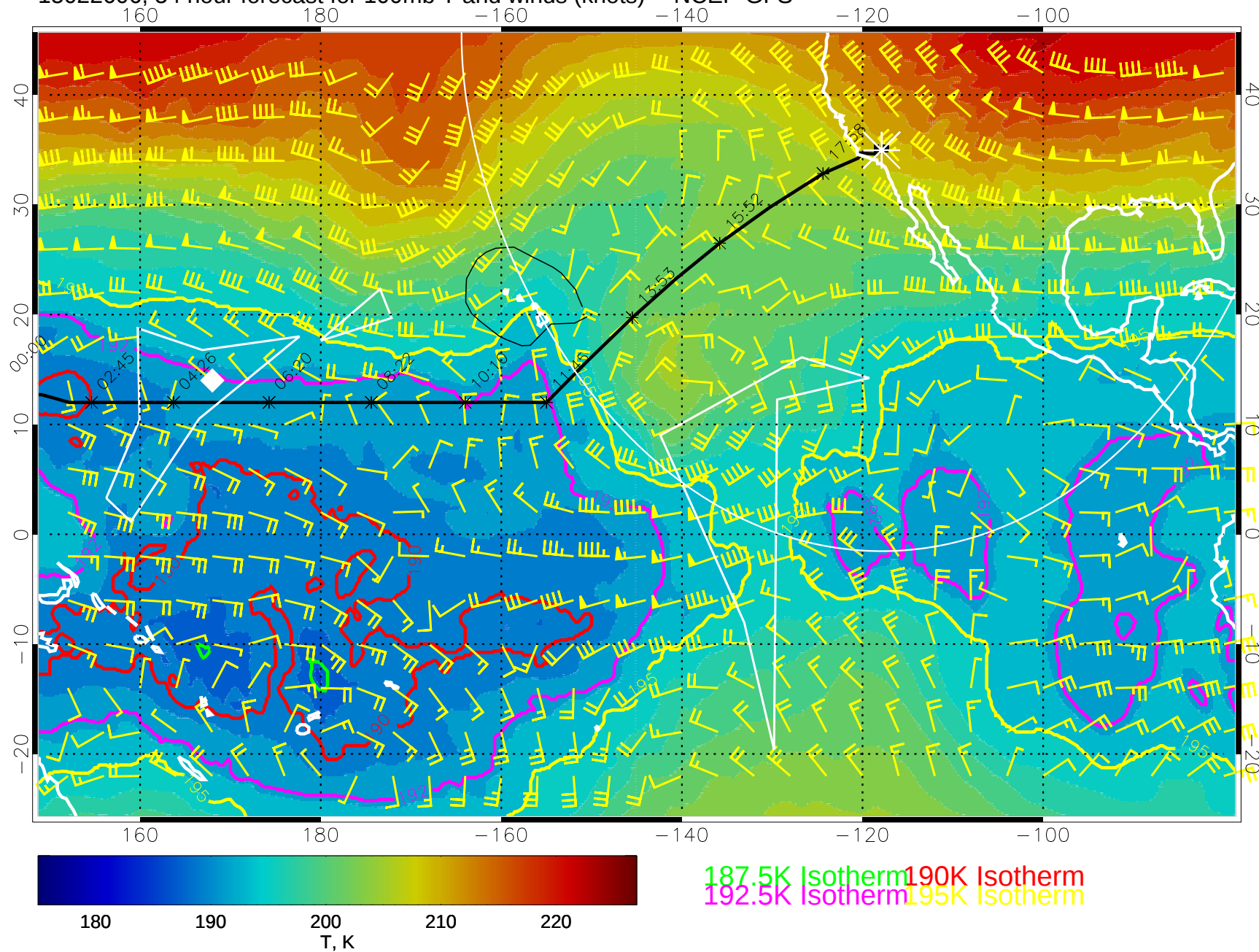
15022606, 54 hour forecast for 100mb T and winds (knots) -- NCEP GFS
