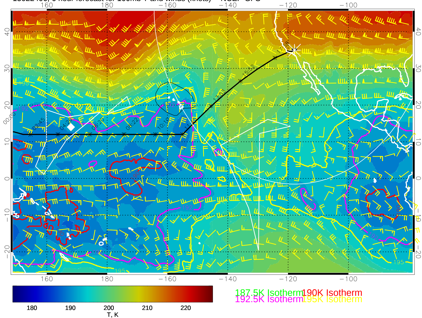
15022406, 6 hour forecast for 100mb T and winds (knots) -- NCEP GFS
