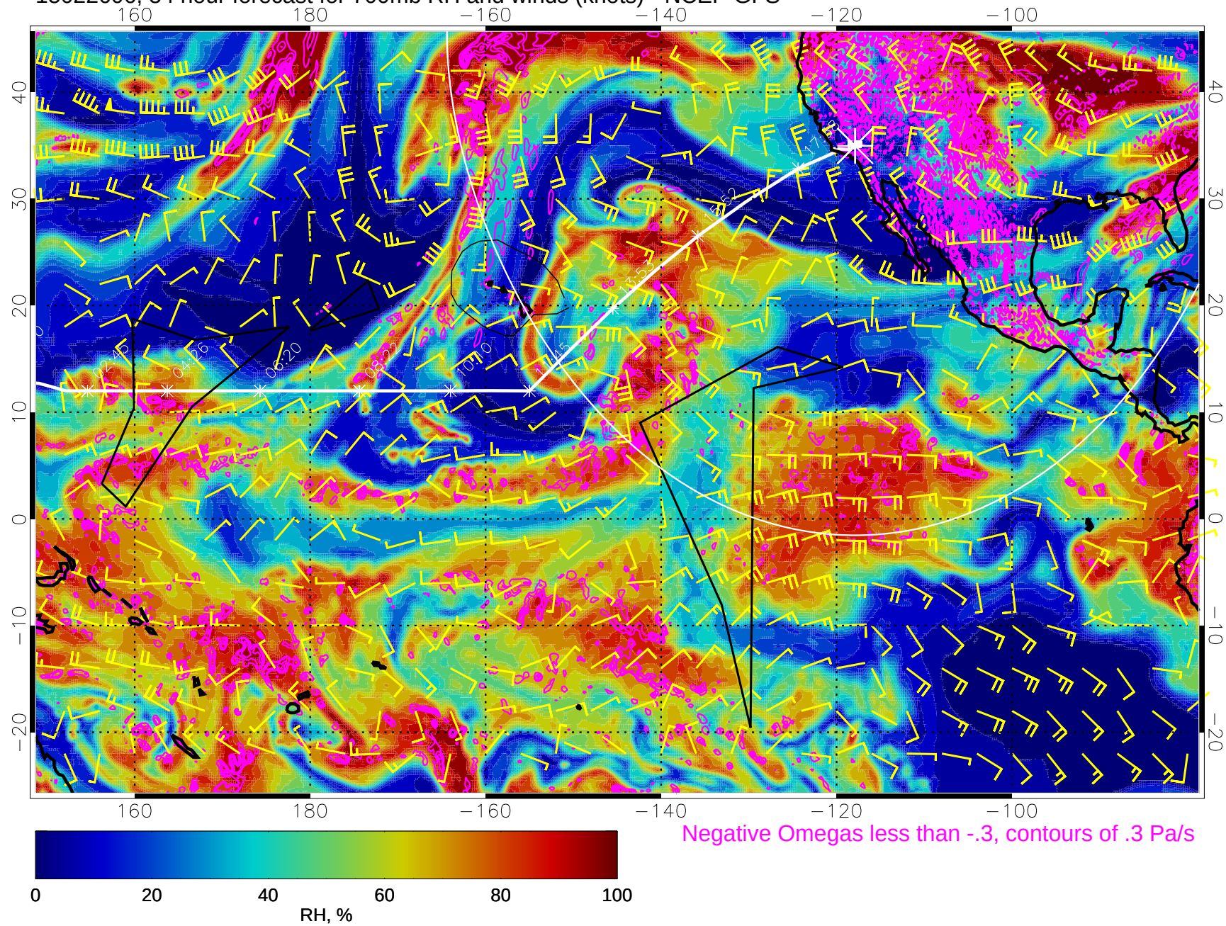
15022606, 54 hour forecast for 700mb RH and winds (knots) - NCEP GFS
