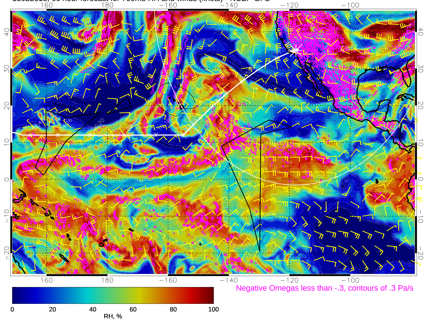
15022618, 66 hour forecast for 700mb RH and winds (knots) - NCEP GFS
