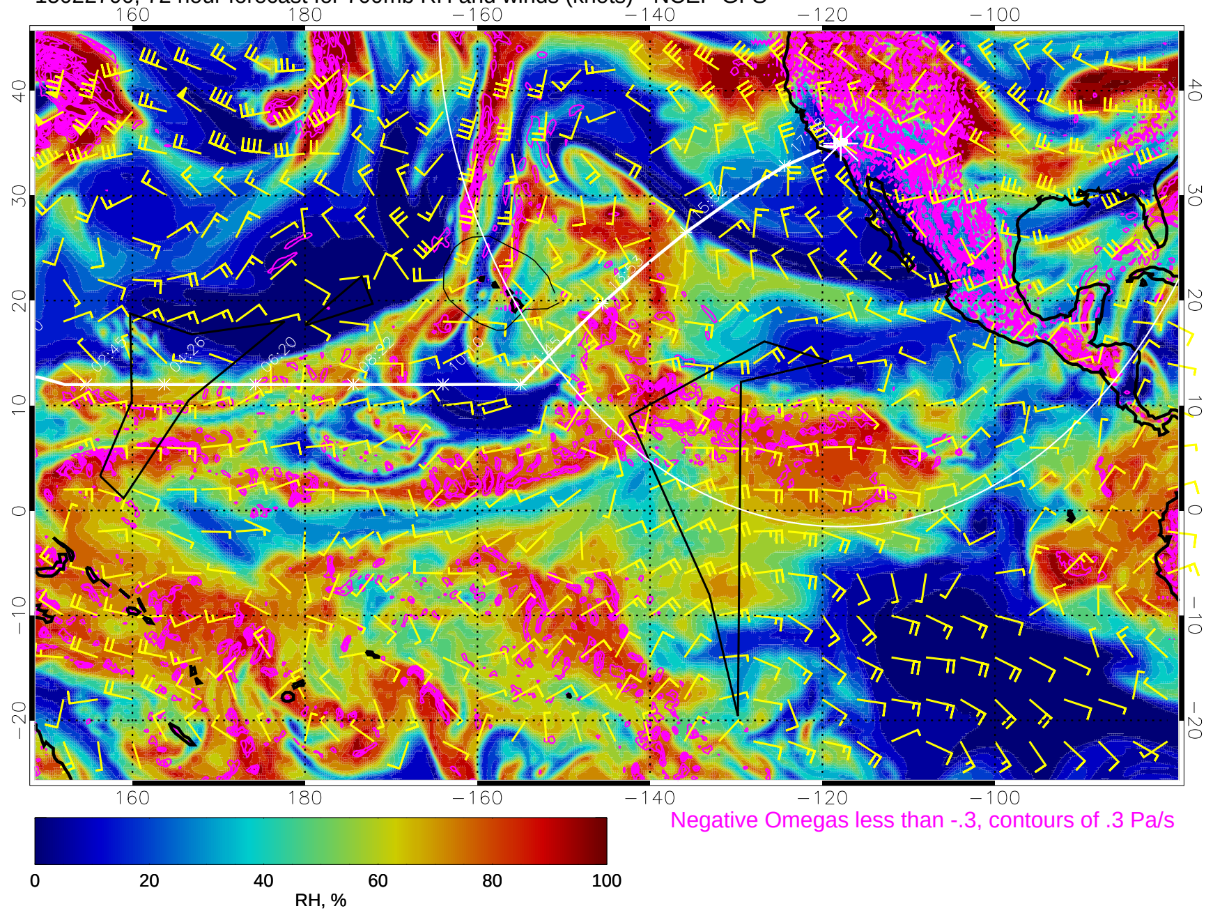
15022700, 72 hour forecast for 700mb RH and winds (knots) - NCEP GFS
