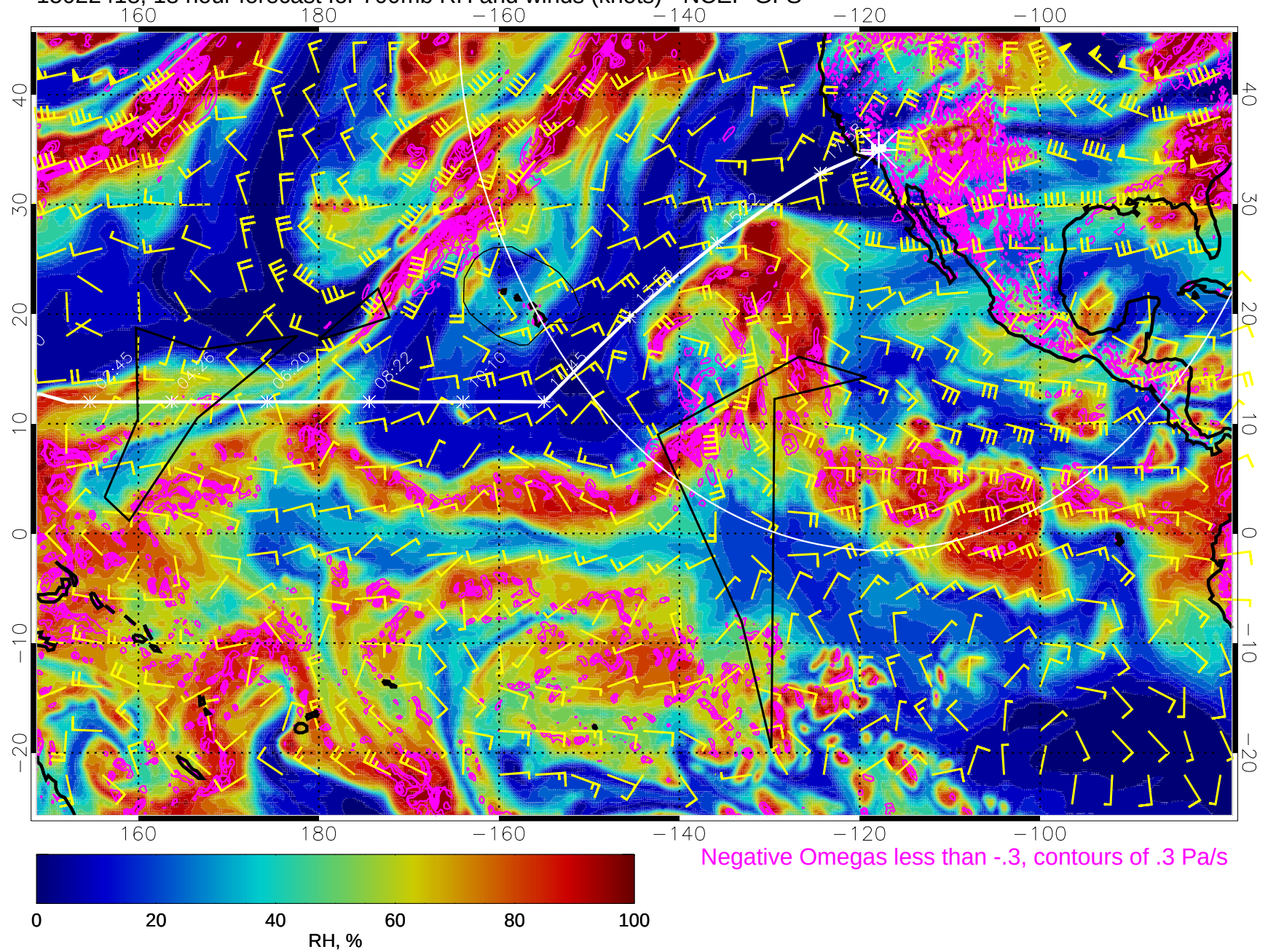
15022418, 18 hour forecast for 700mb RH and winds (knots) - NCEP GFS
