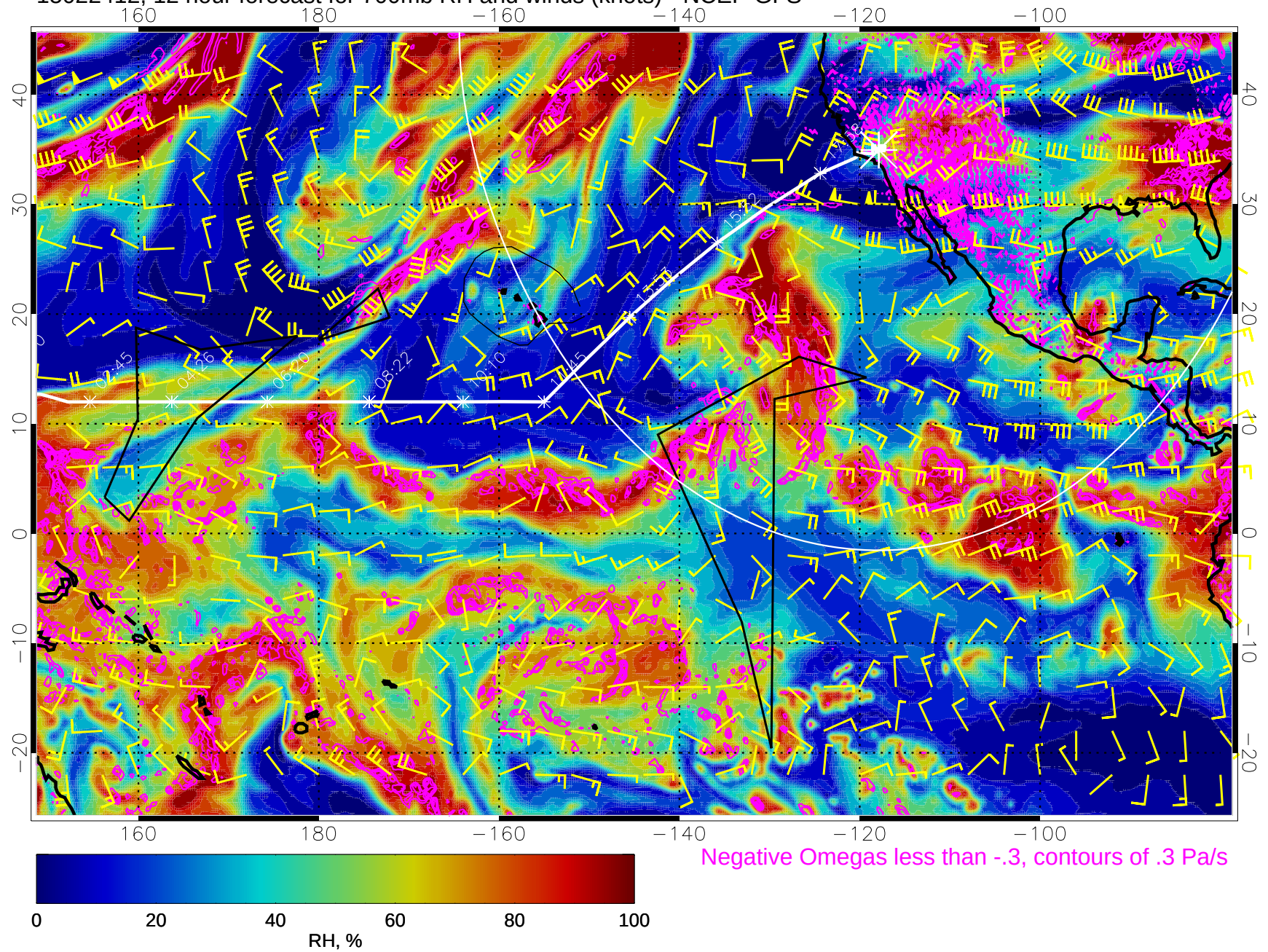
15022412, 12 hour forecast for 700mb RH and winds (knots) - NCEP GFS
