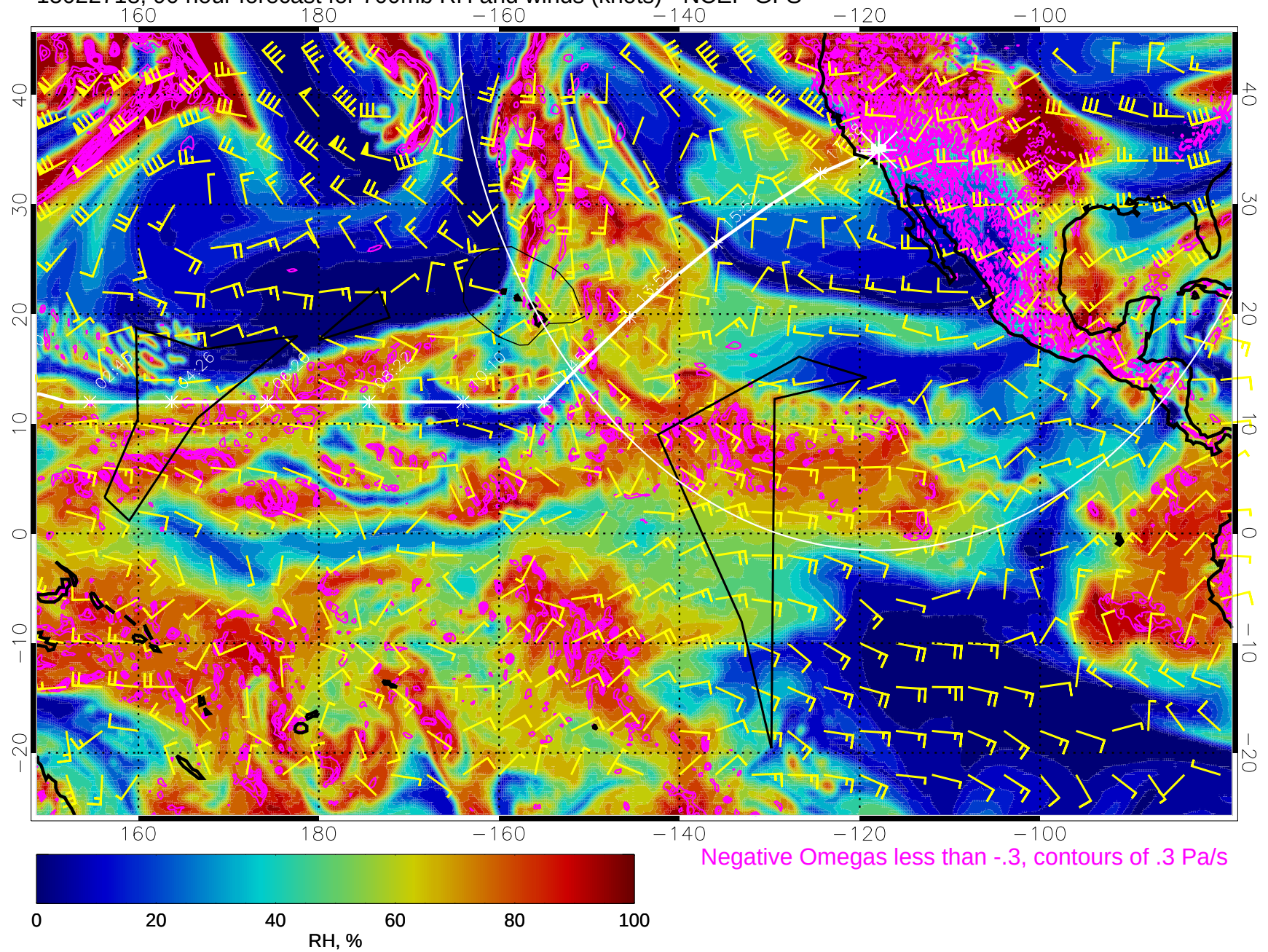
15022718, 90 hour forecast for 700mb RH and winds (knots) - NCEP GFS
