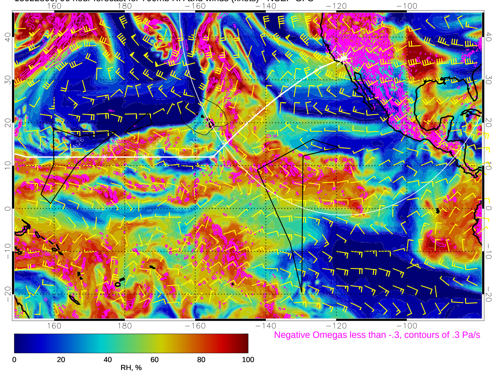
15022800, 96 hour forecast for 700mb RH and winds (knots) - NCEP GFS
