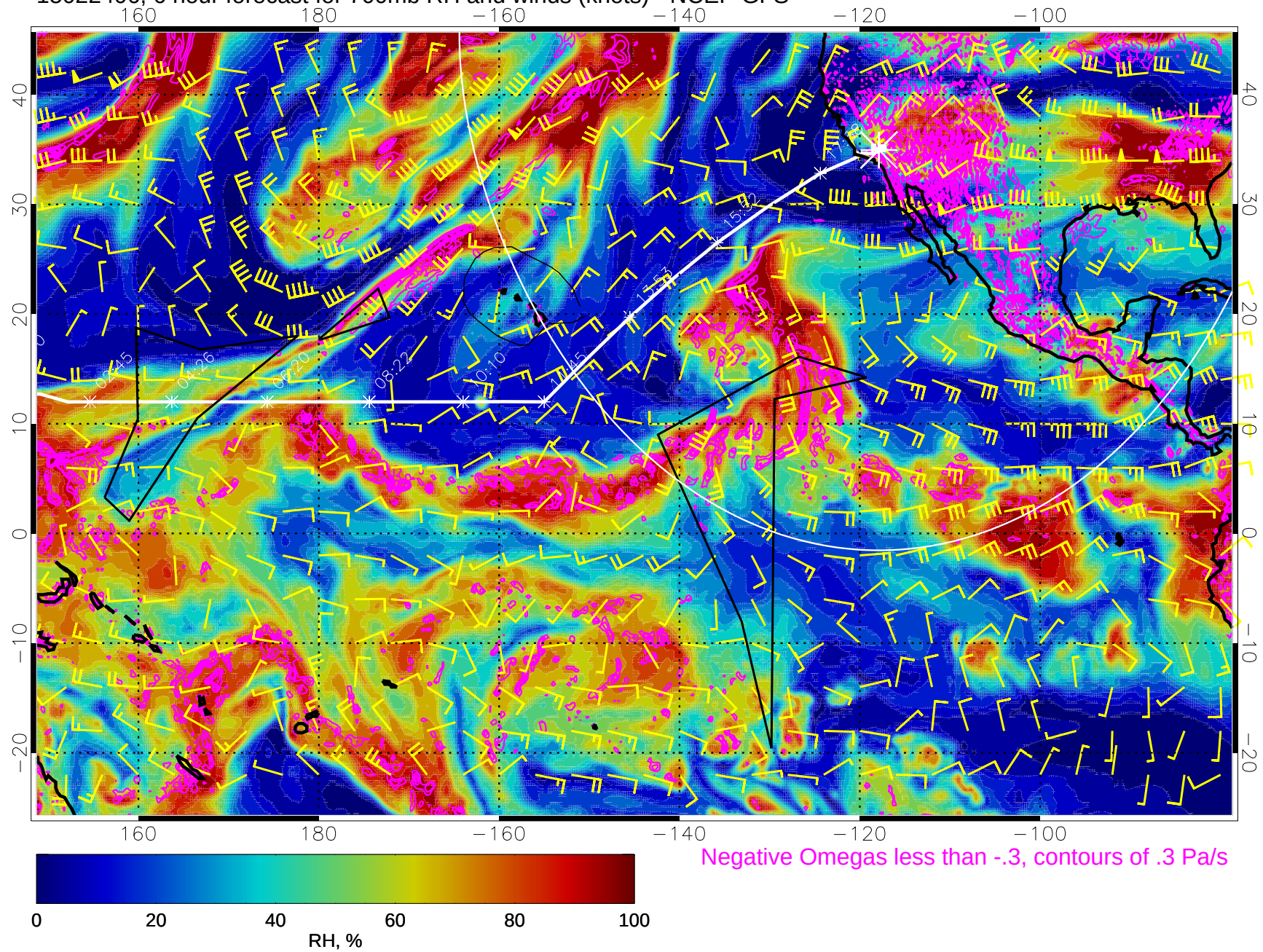
15022406, 6 hour forecast for 700mb RH and winds (knots) - NCEP GFS
