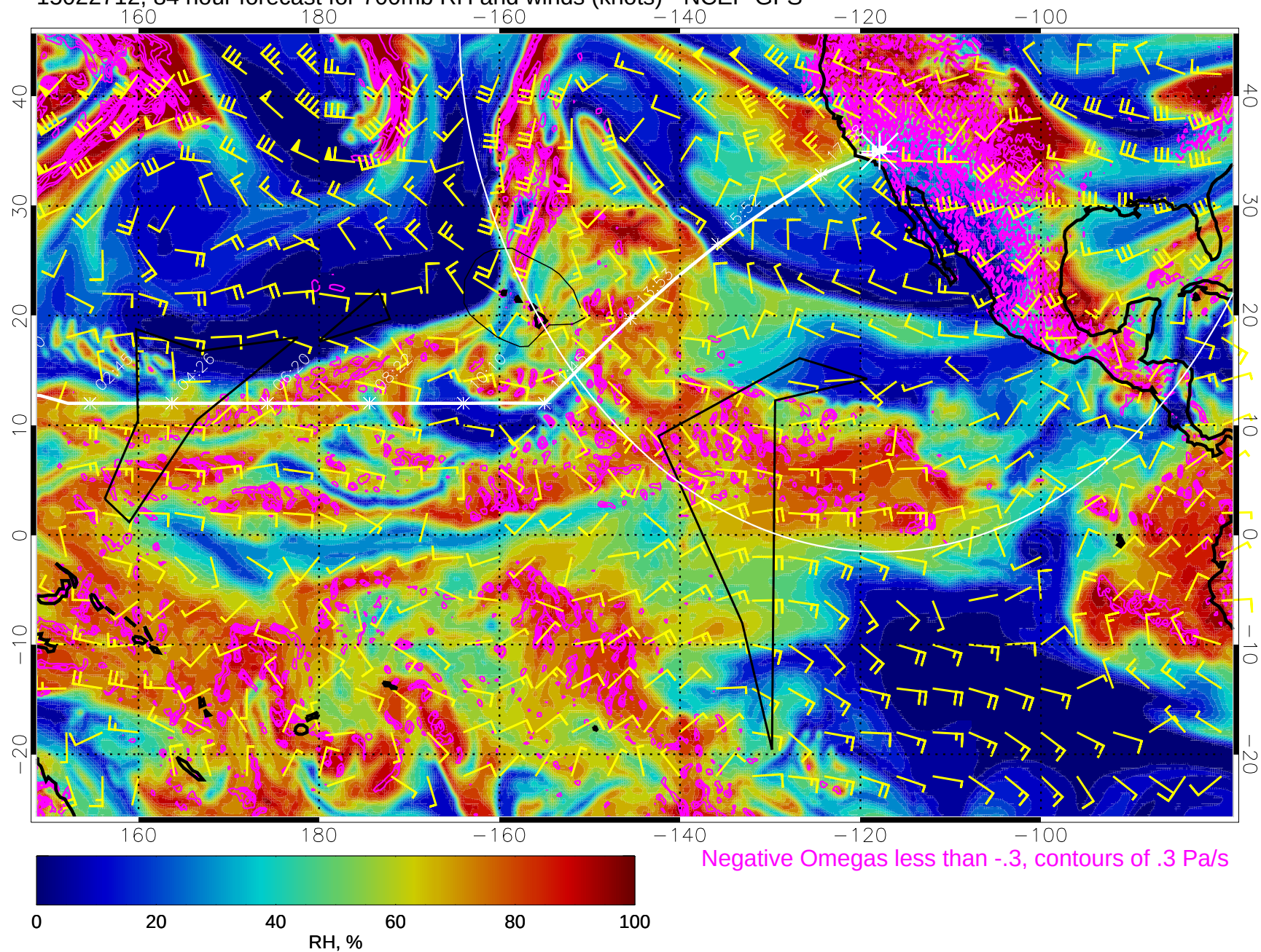
15022712, 84 hour forecast for 700mb RH and winds (knots) - NCEP GFS
