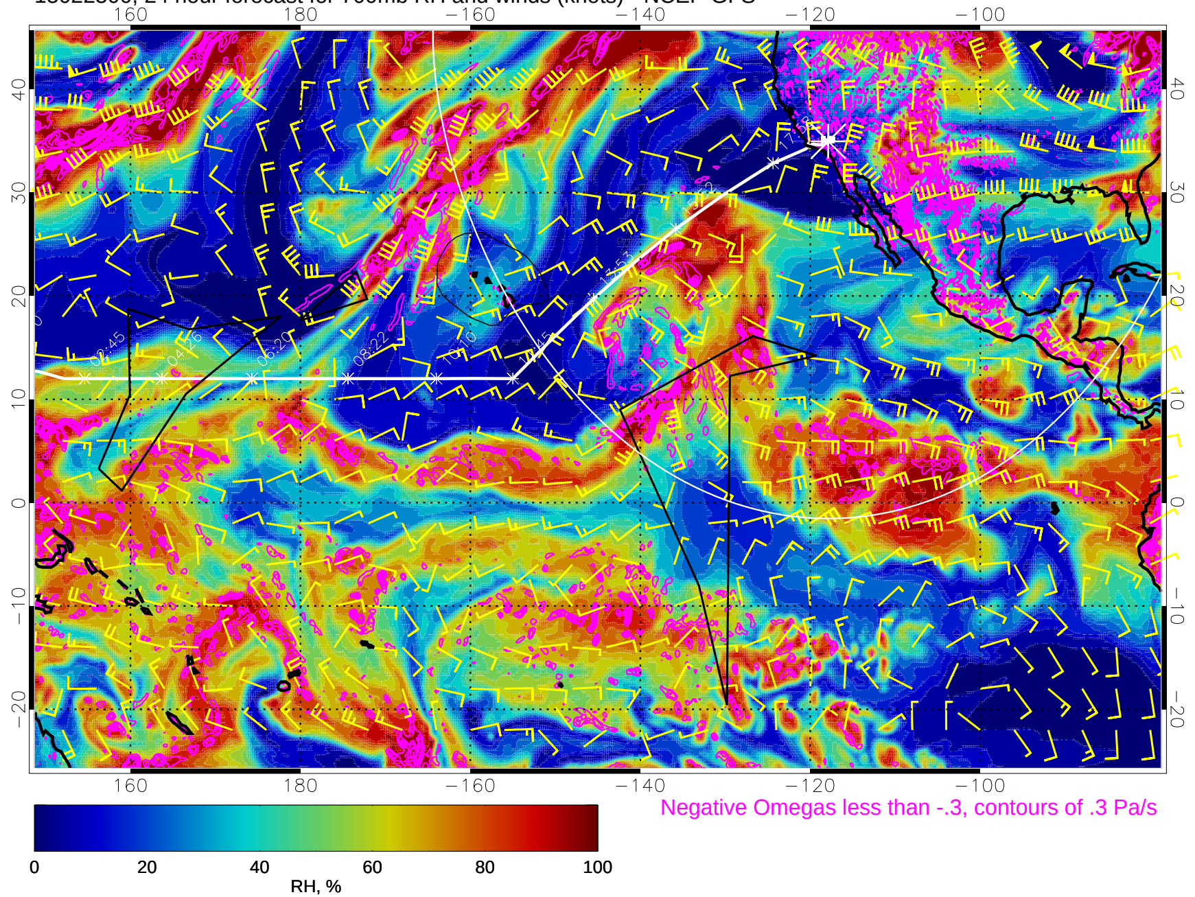
15022500, 24 hour forecast for 700mb RH and winds (knots) - NCEP GFS
