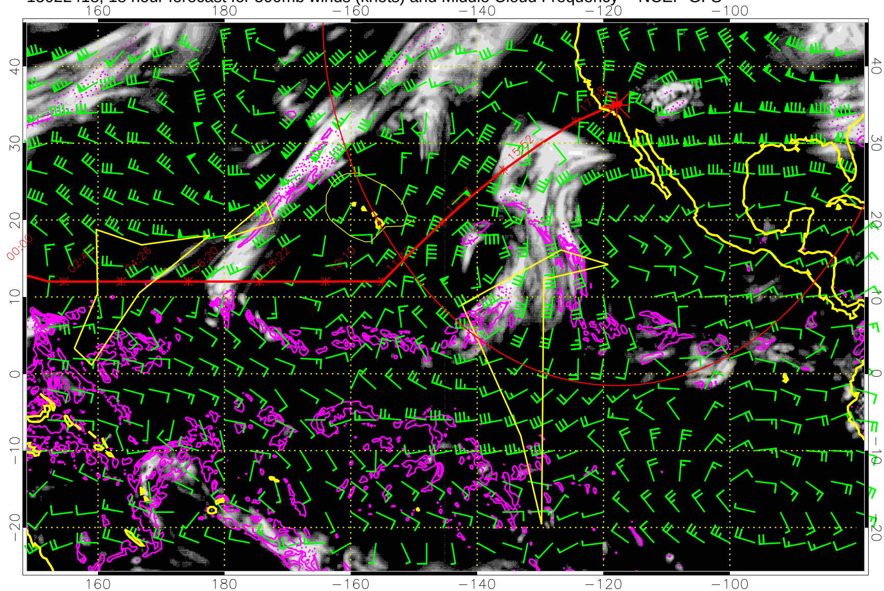
15022418, 18 hour forecast for 500mb winds (knots) and Middle Cloud Frequency -- NCEP GFS
