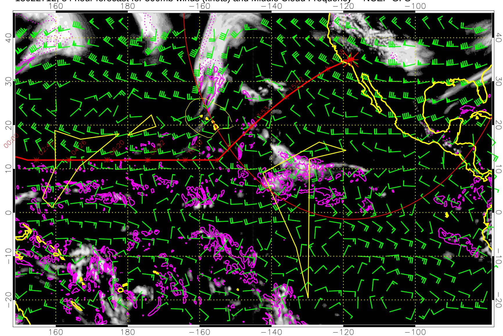
15022712, 84 hour forecast for 500mb winds (knots) and Middle Cloud Frequency -- NCEP GFS
