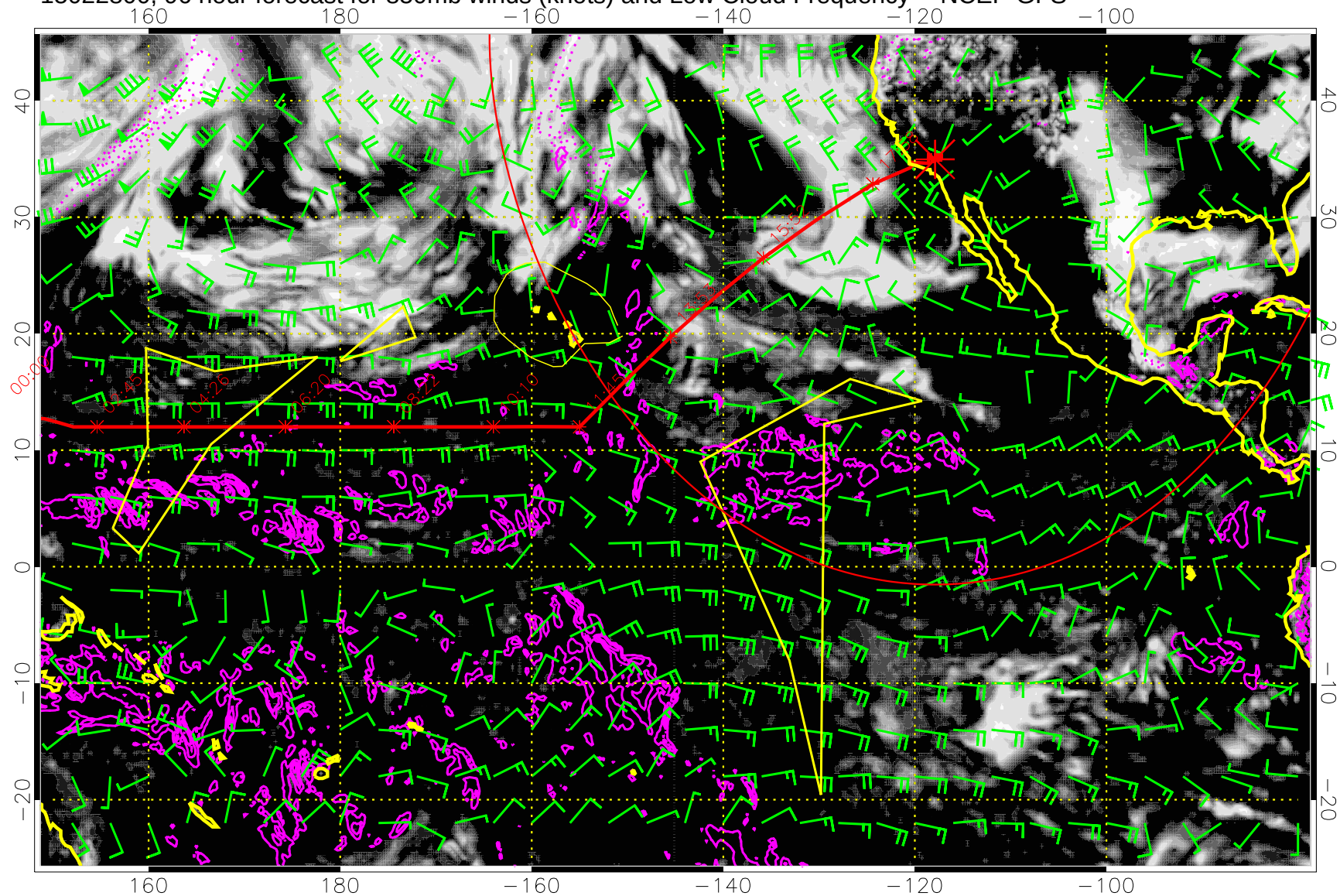
15022800, 96 hour forecast for 850mb winds (knots) and Low Cloud Frequency -- NCEP GFS
