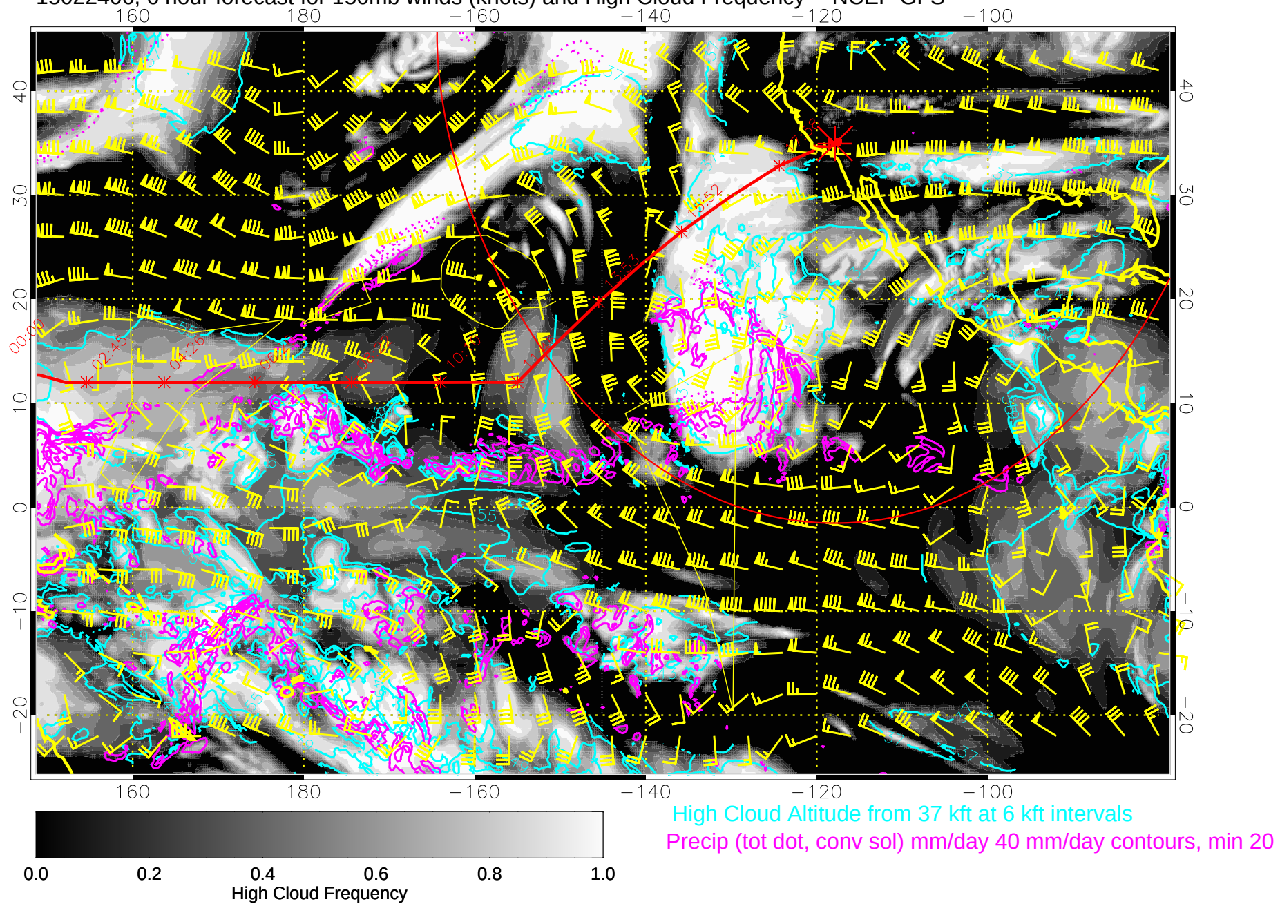
15022406, 6 hour forecast for 150mb winds (knots) and High Cloud Frequency -- NCEP GFS
