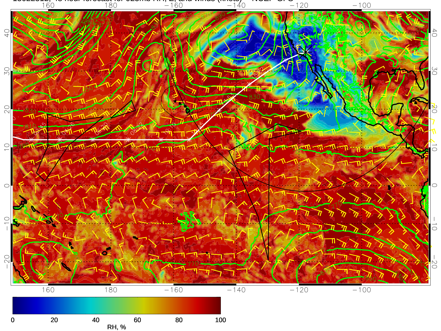
15022512, 48 hour forecast for 925mb RH, Z, and winds (knots) -- NCEP GFS
