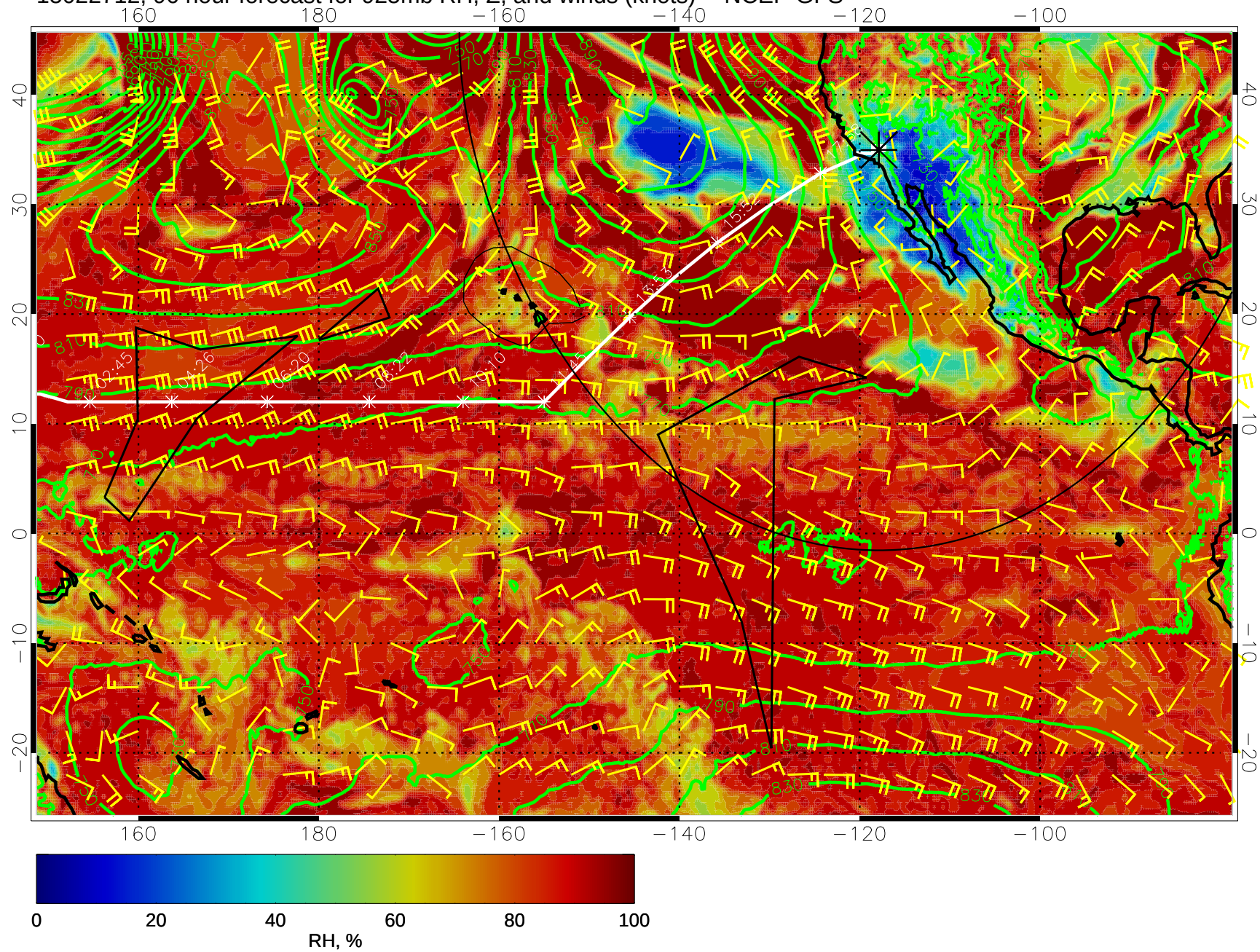
15022712, 96 hour forecast for 925mb RH, Z, and winds (knots) -- NCEP GFS
