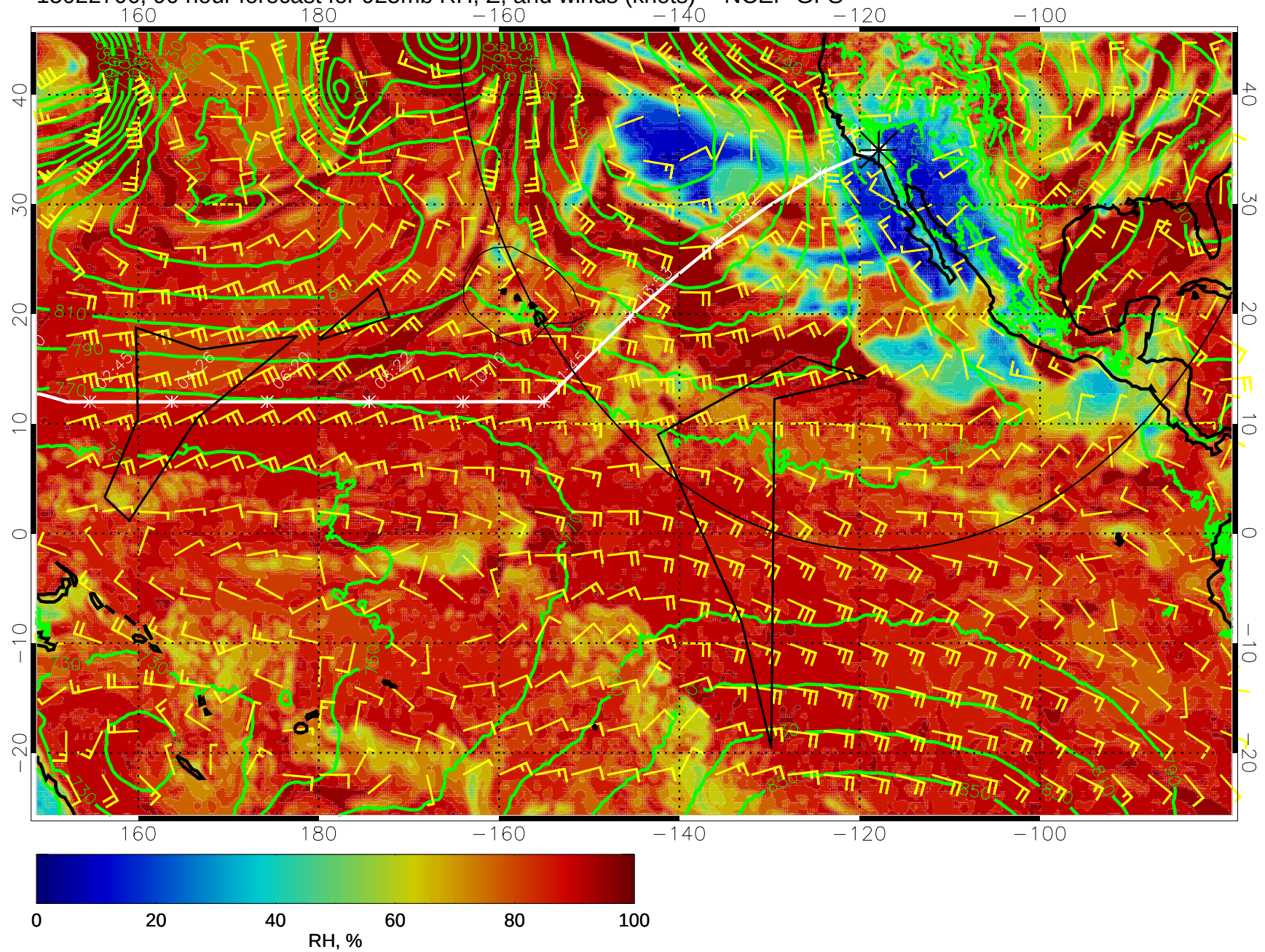
15022706, 90 hour forecast for 925mb RH, Z, and winds (knots) -- NCEP GFS
