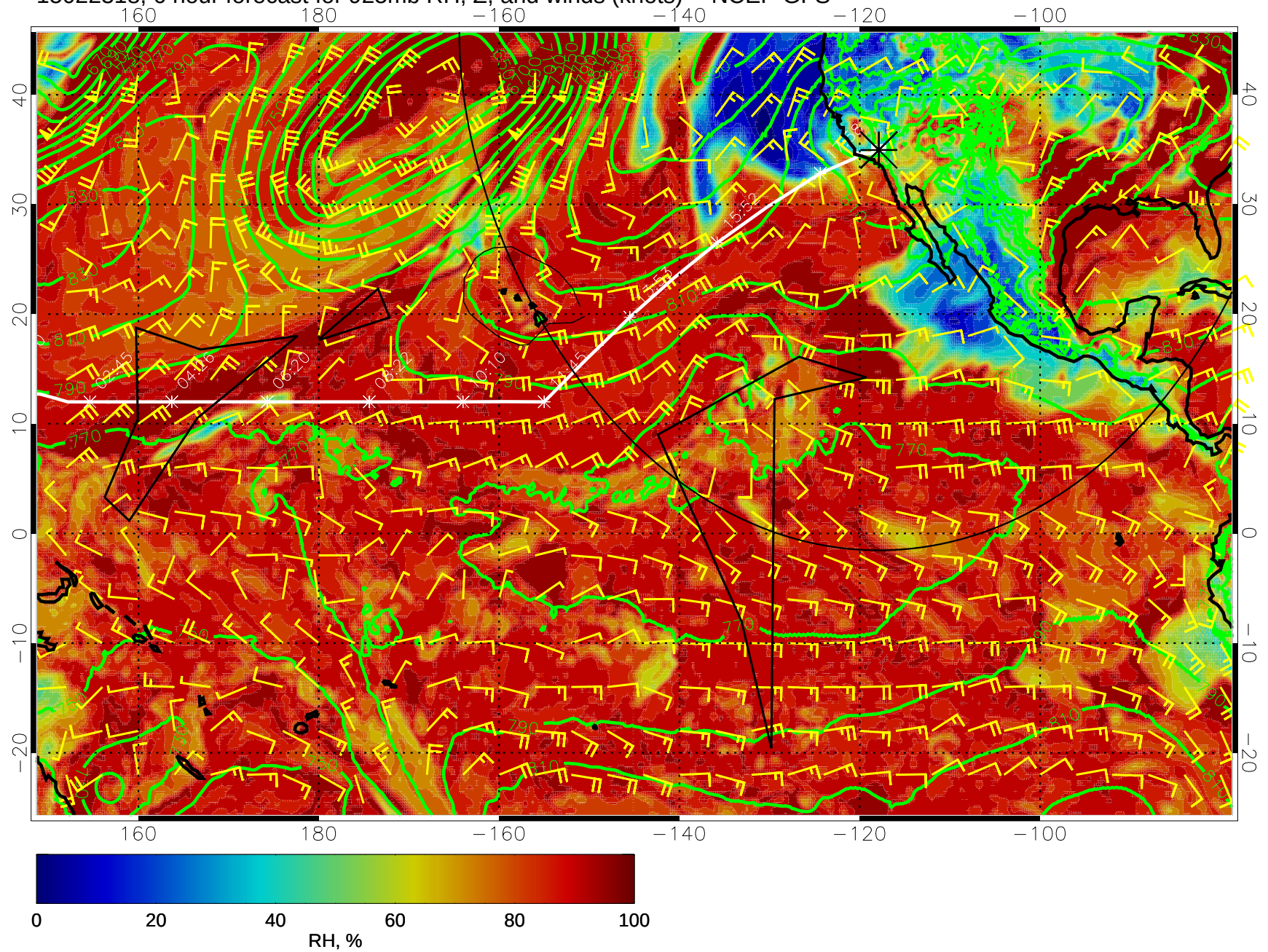
15022318, 6 hour forecast for 925mb RH, Z, and winds (knots) -- NCEP GFS
