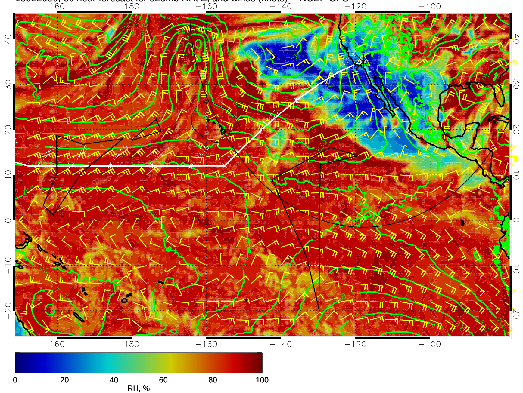
15022606, 66 hour forecast for 925mb RH, Z, and winds (knots) -- NCEP GFS
