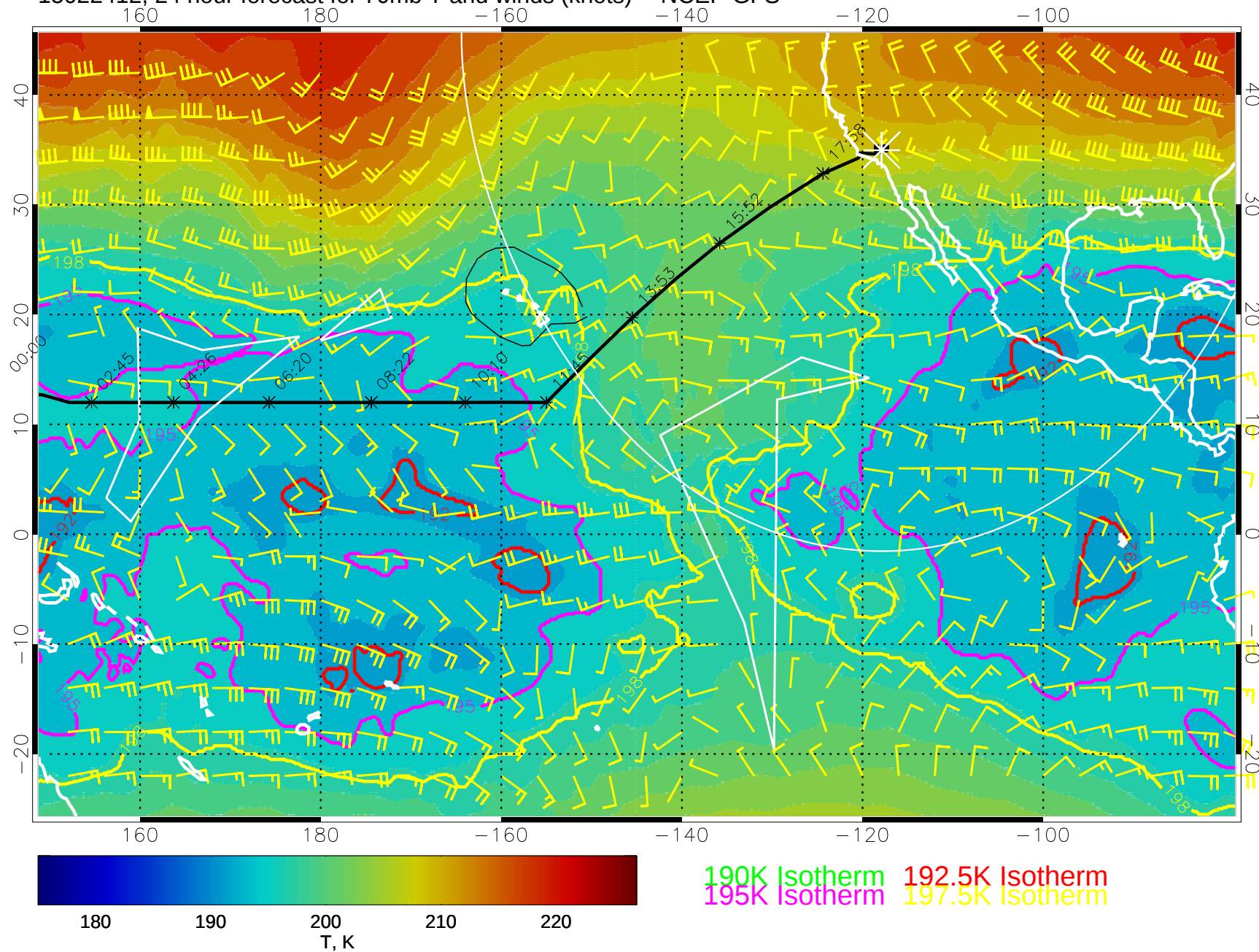
15022412, 24 hour forecast for 70mb T and winds (knots) -- NCEP GFS
