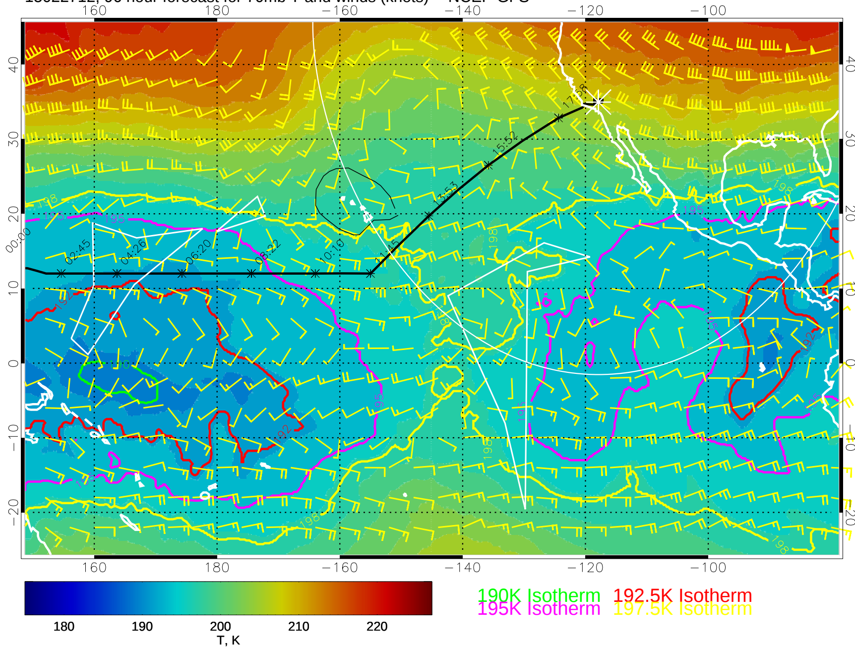
15022712, 96 hour forecast for 70mb T and winds (knots) -- NCEP GFS
