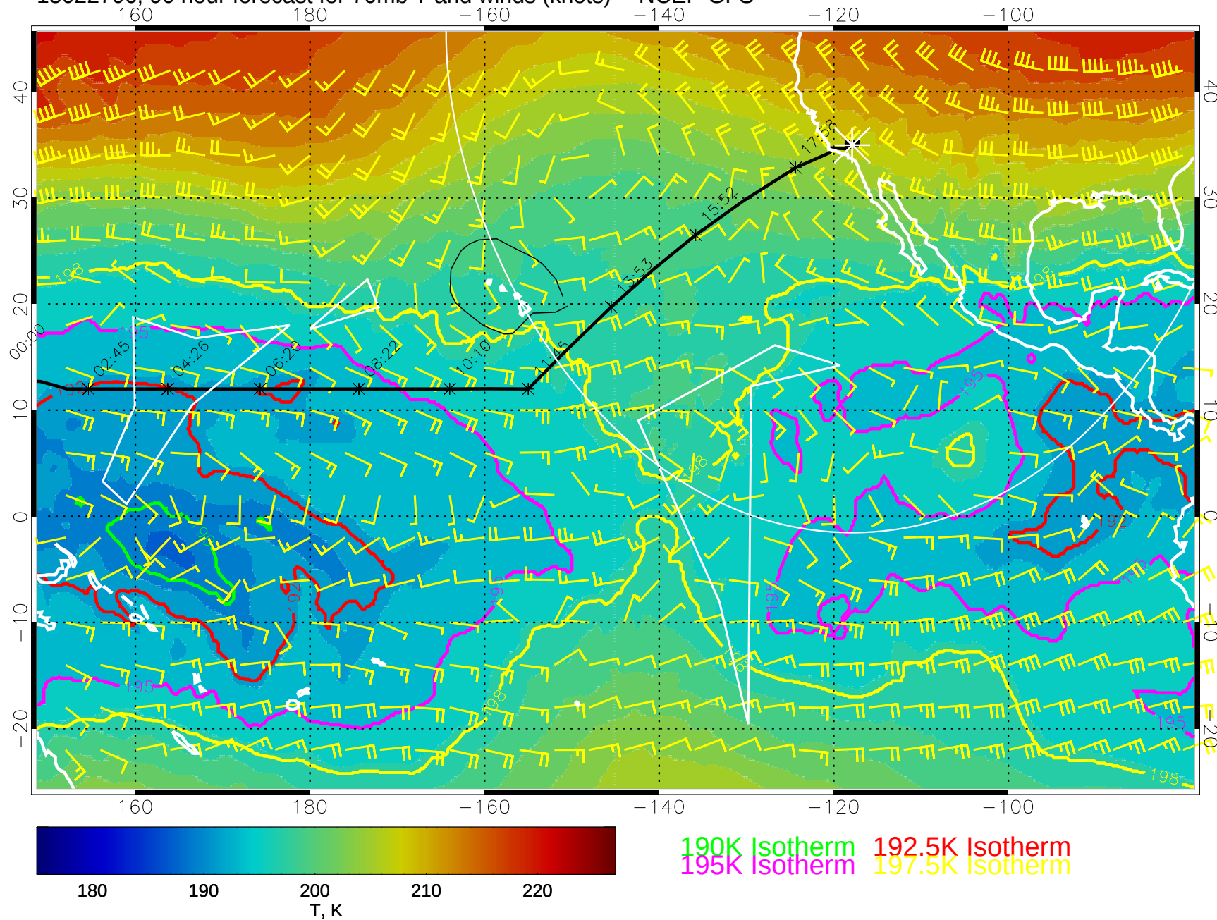
15022706, 90 hour forecast for 70mb T and winds (knots) -- NCEP GFS
