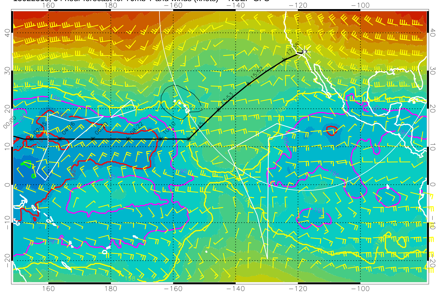
15022518, 54 hour forecast for 70mb T and winds (knots) -- NCEP GFS
