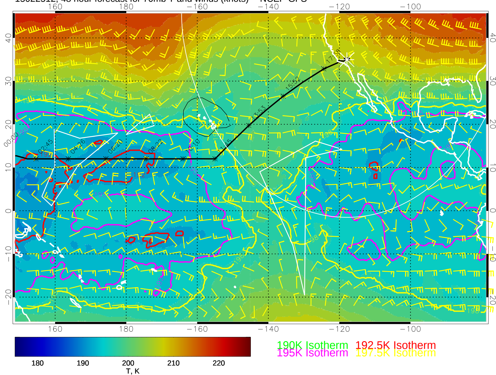
15022512, 48 hour forecast for 70mb T and winds (knots) -- NCEP GFS
