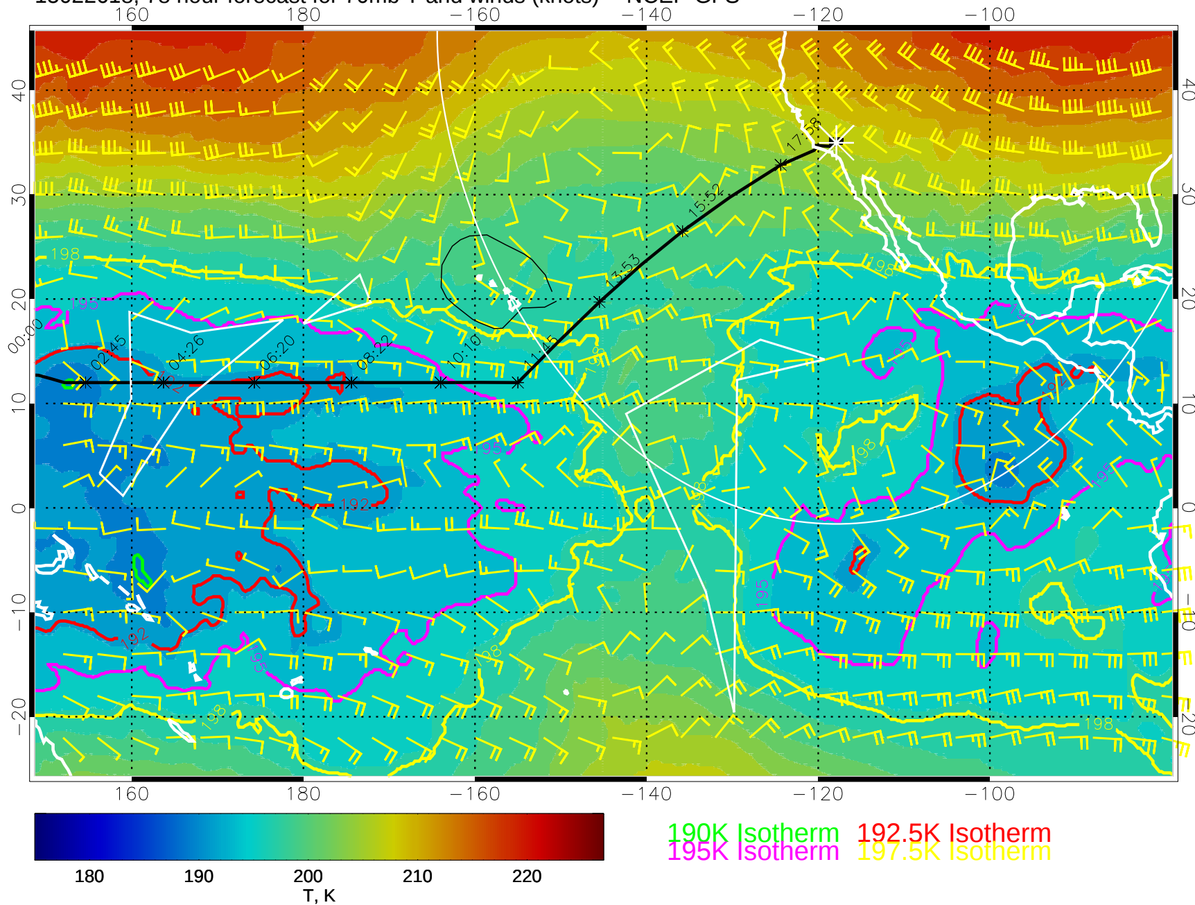
15022618, 78 hour forecast for 70mb T and winds (knots) -- NCEP GFS
