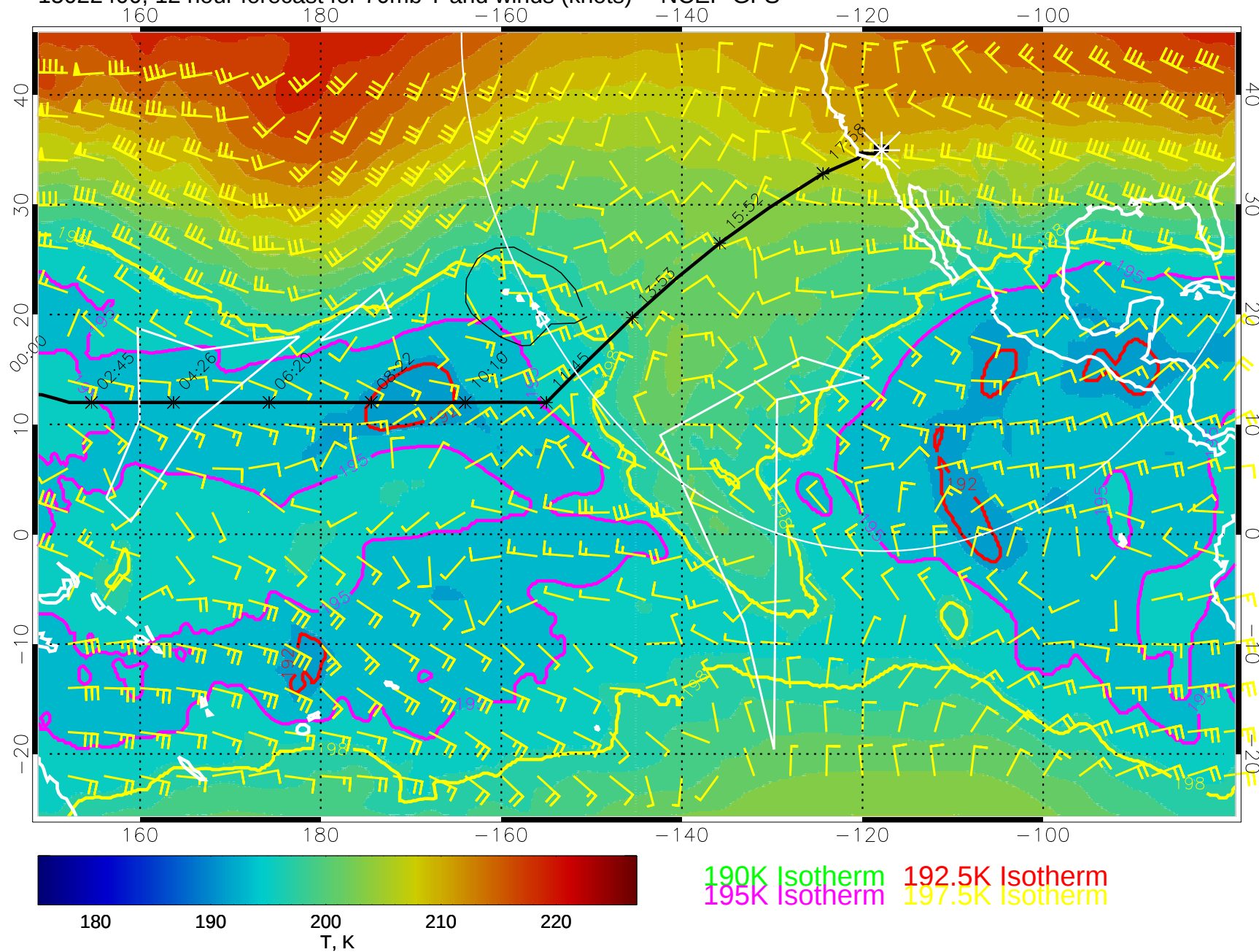
15022400, 12 hour forecast for 70mb T and winds (knots) -- NCEP GFS
