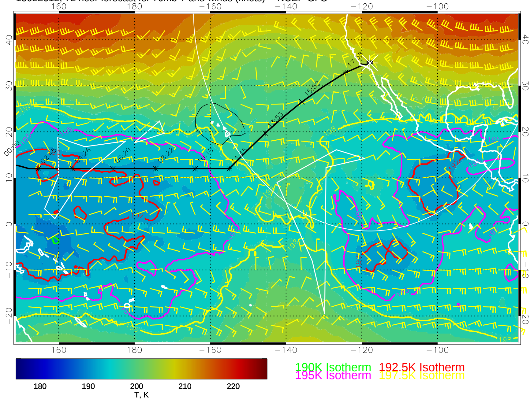
15022612, 72 hour forecast for 70mb T and winds (knots) -- NCEP GFS
