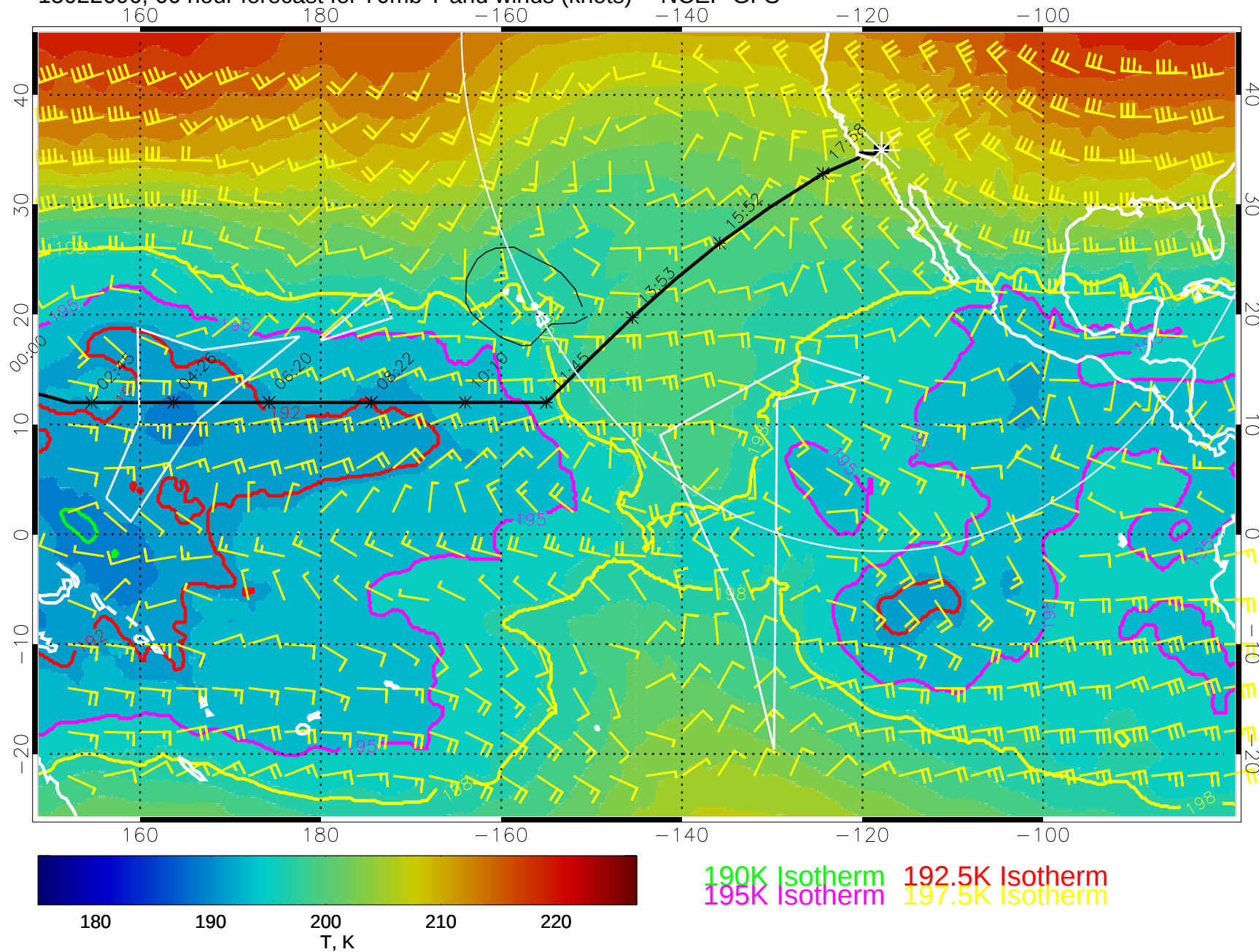
15022606, 66 hour forecast for 70mb T and winds (knots) -- NCEP GFS
