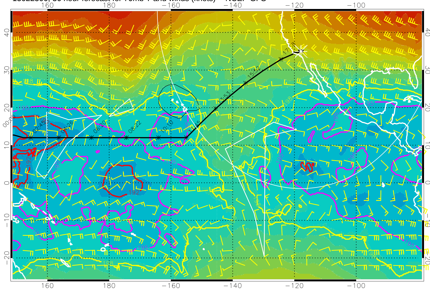
15022500, 36 hour forecast for 70mb T and winds (knots) -- NCEP GFS
