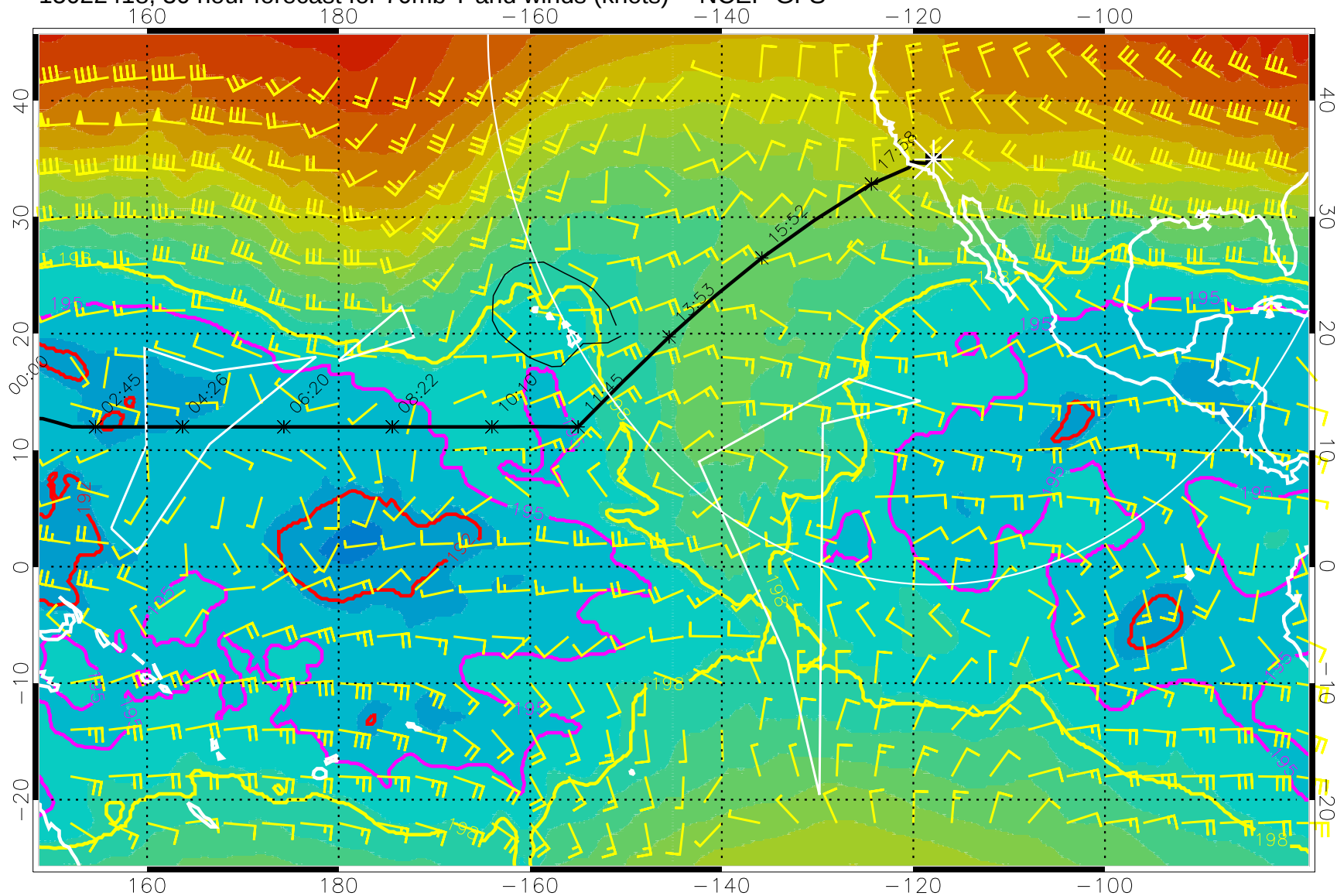
15022418, 30 hour forecast for 70mb T and winds (knots) -- NCEP GFS
