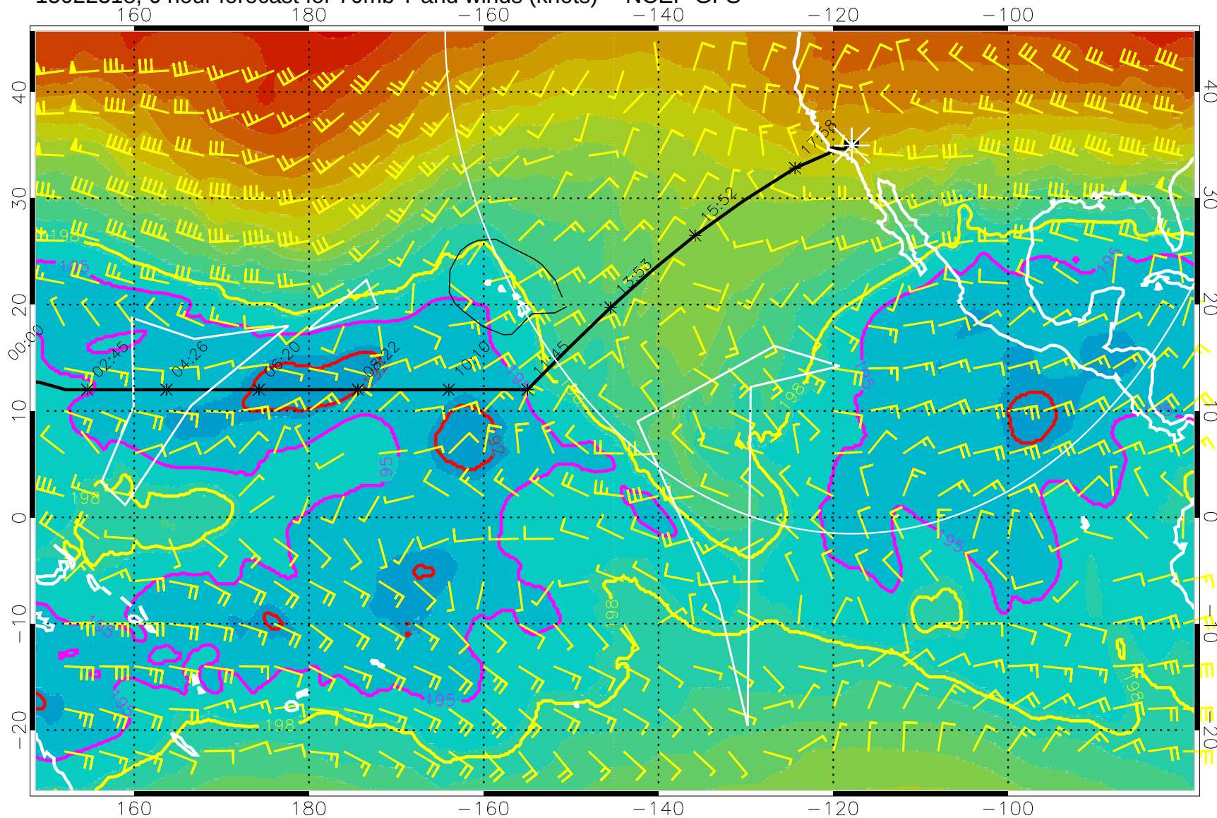
15022318, 6 hour forecast for 70mb T and winds (knots) -- NCEP GFS
