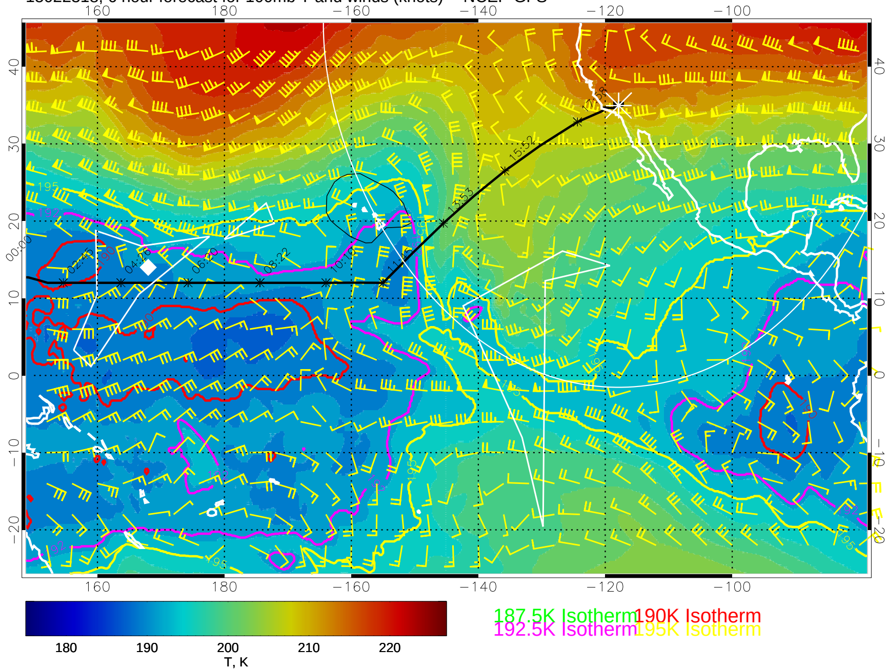
15022318, 6 hour forecast for 100mb T and winds (knots) -- NCEP GFS
