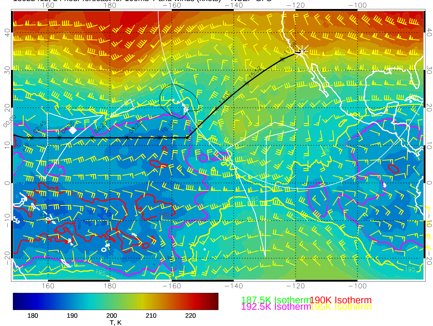
15022412, 24 hour forecast for 100mb T and winds (knots) -- NCEP GFS
