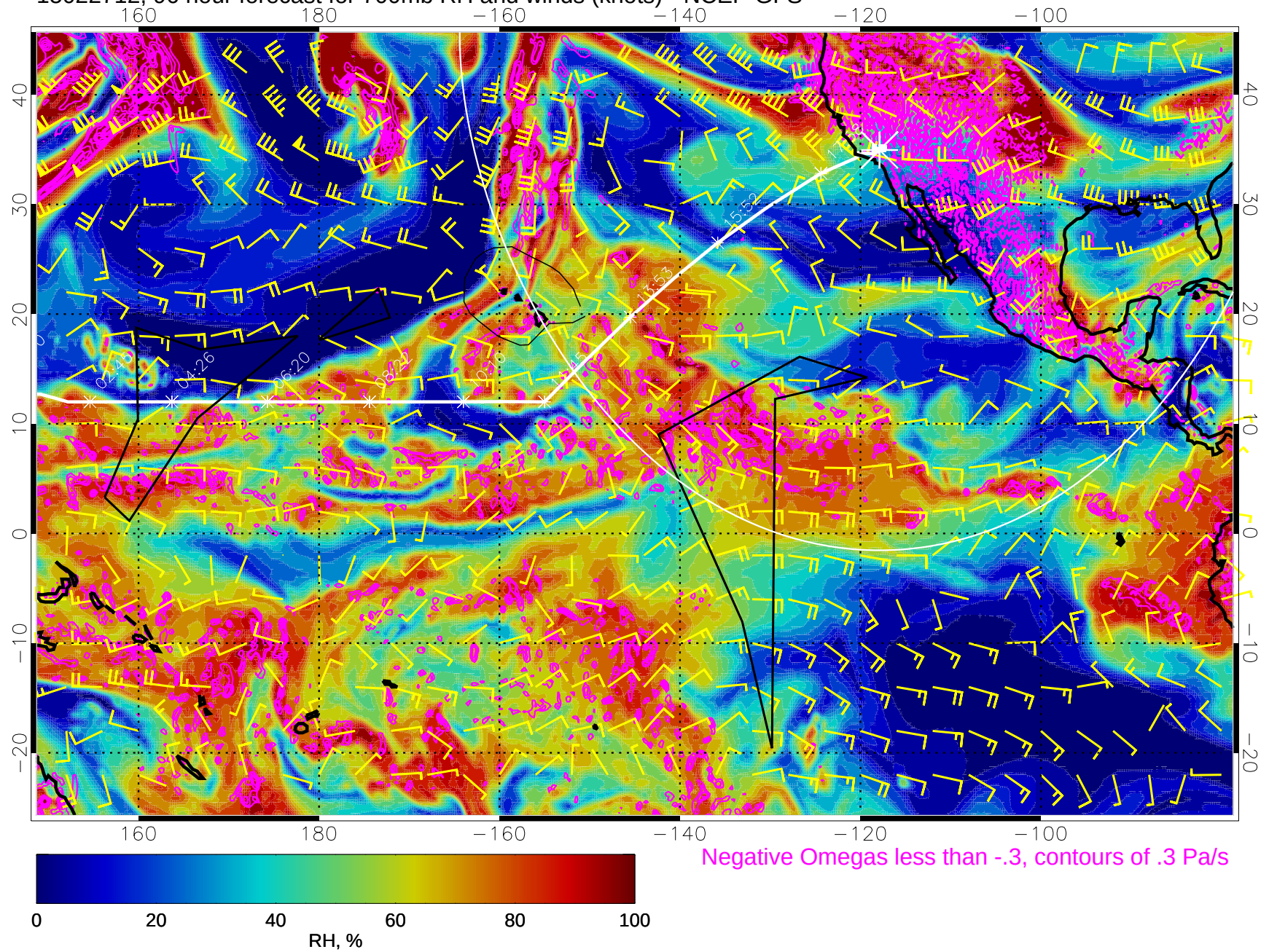
15022712, 96 hour forecast for 700mb RH and winds (knots) - NCEP GFS
