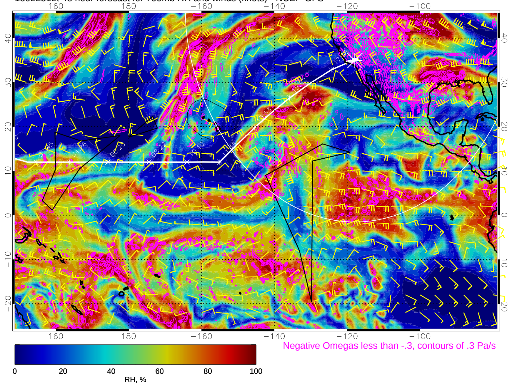
15022512, 48 hour forecast for 700mb RH and winds (knots) - NCEP GFS
