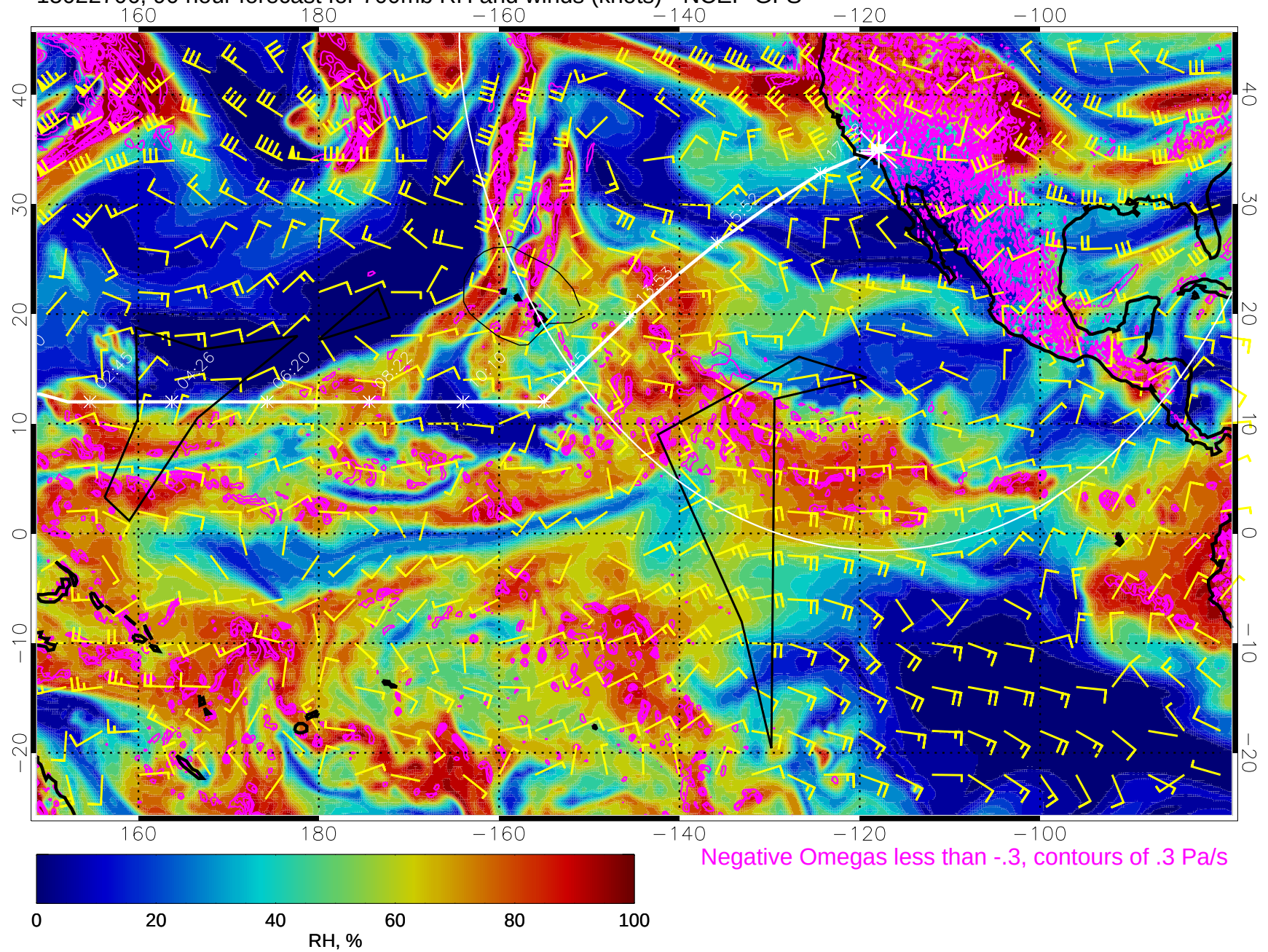
15022706, 90 hour forecast for 700mb RH and winds (knots) - NCEP GFS
