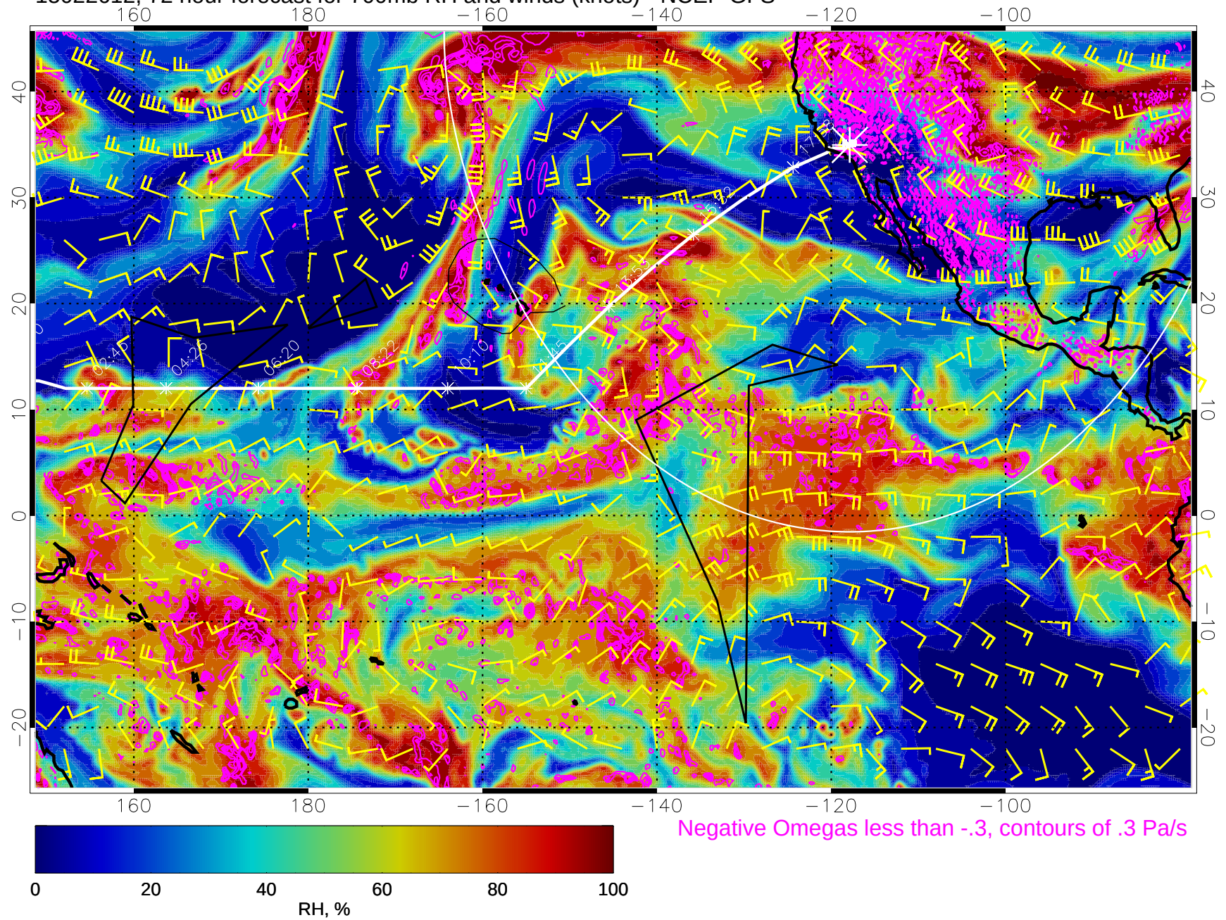
15022612, 72 hour forecast for 700mb RH and winds (knots) - NCEP GFS
