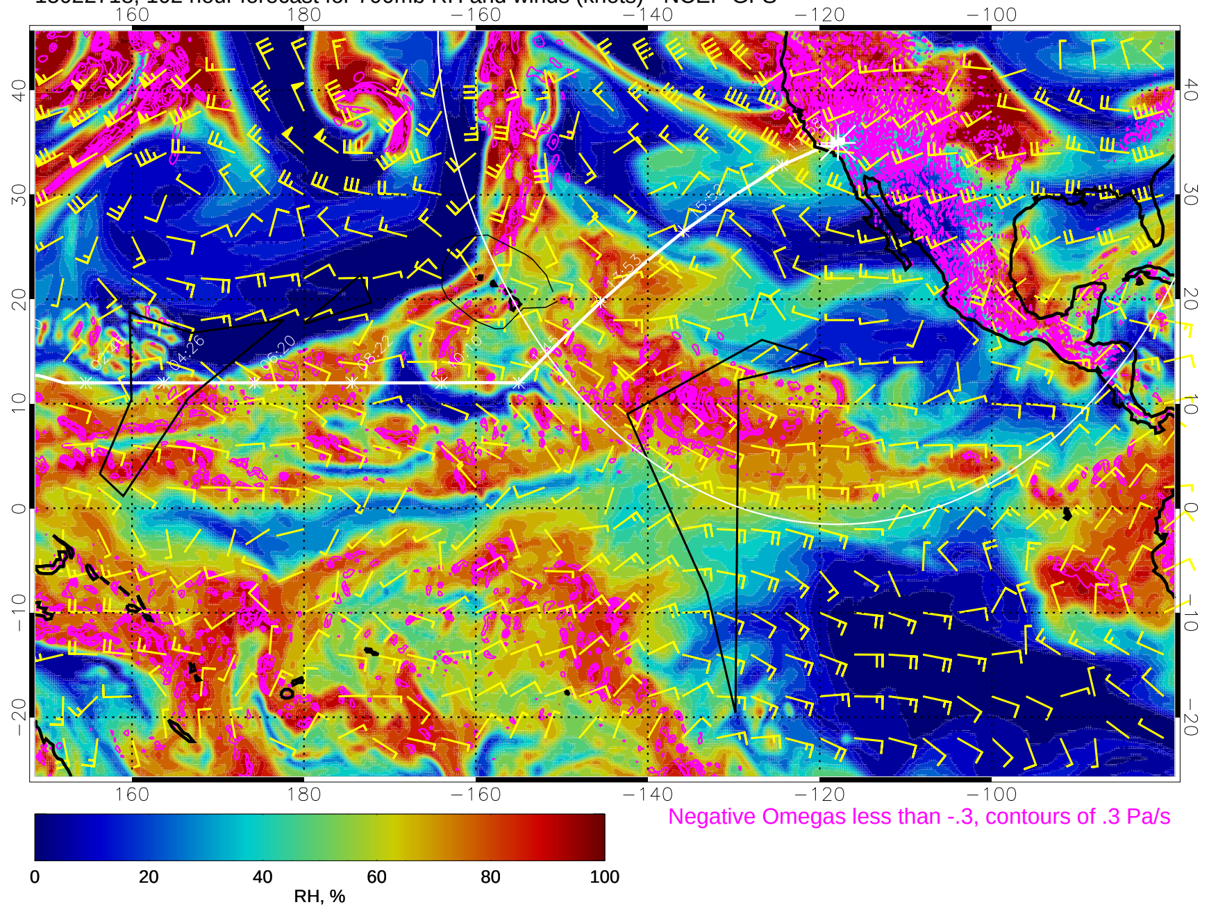
15022718, 102 hour forecast for 700mb RH and winds (knots) - NCEP GFS
