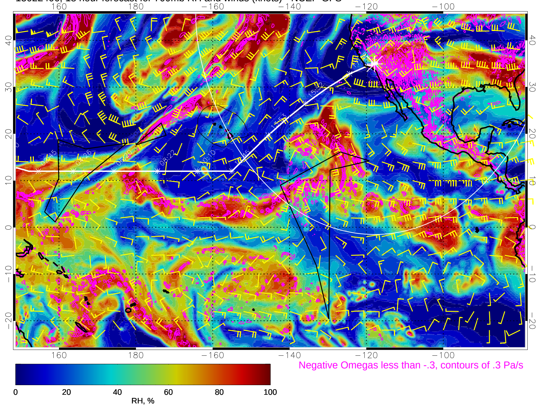
15022406, 18 hour forecast for 700mb RH and winds (knots) - NCEP GFS
