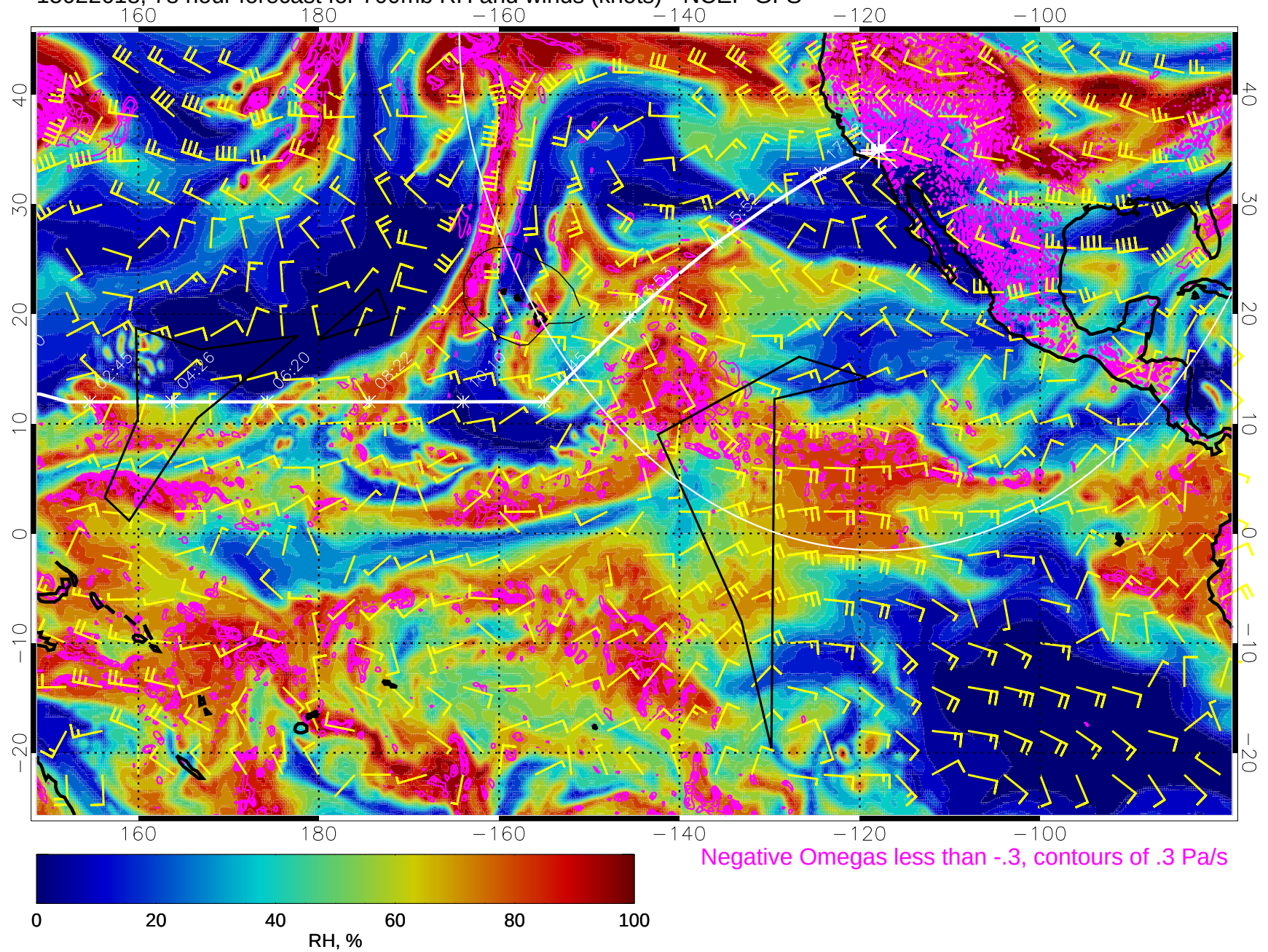
15022618, 78 hour forecast for 700mb RH and winds (knots) - NCEP GFS
