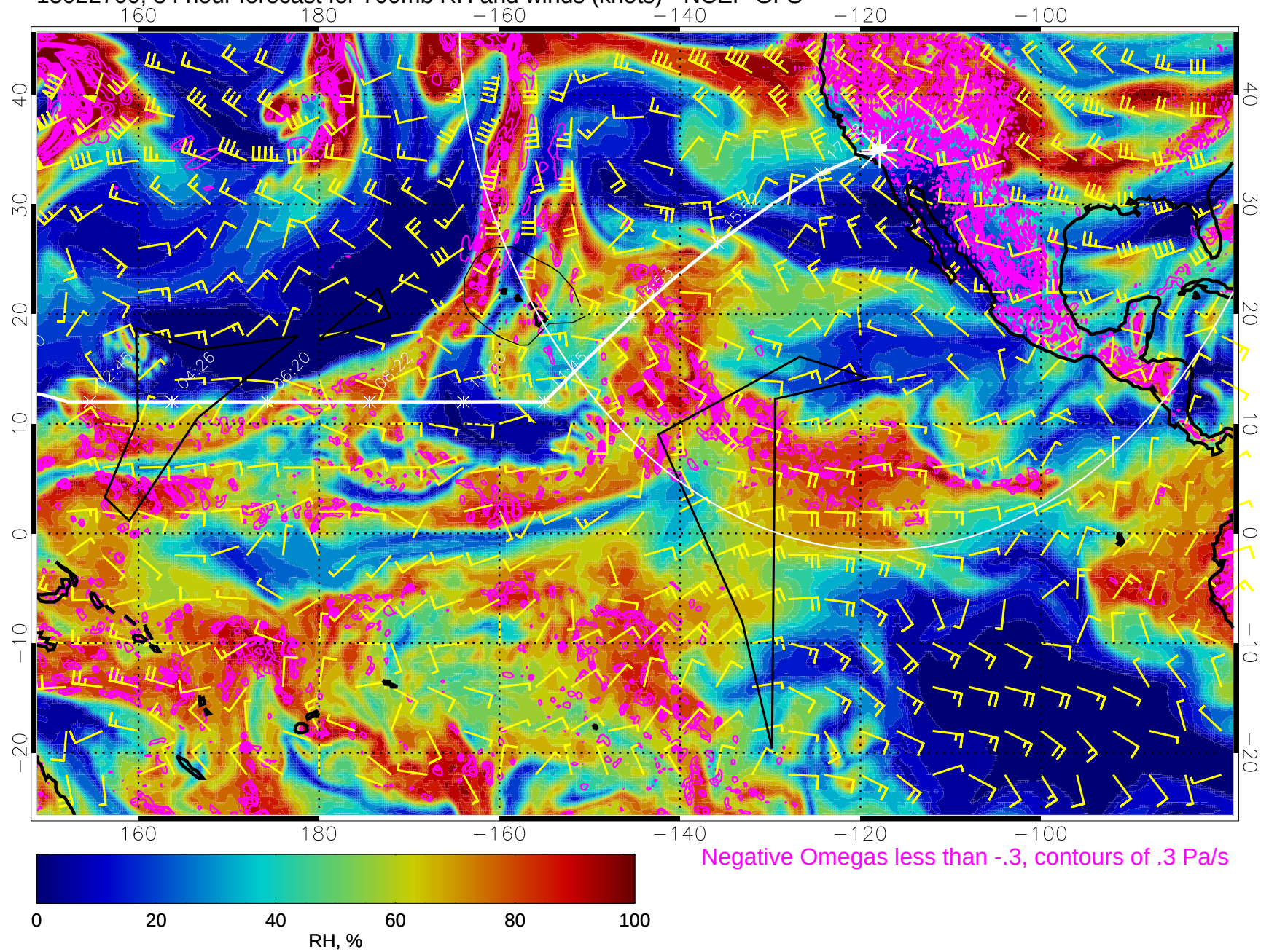
15022700, 84 hour forecast for 700mb RH and winds (knots) - NCEP GFS
