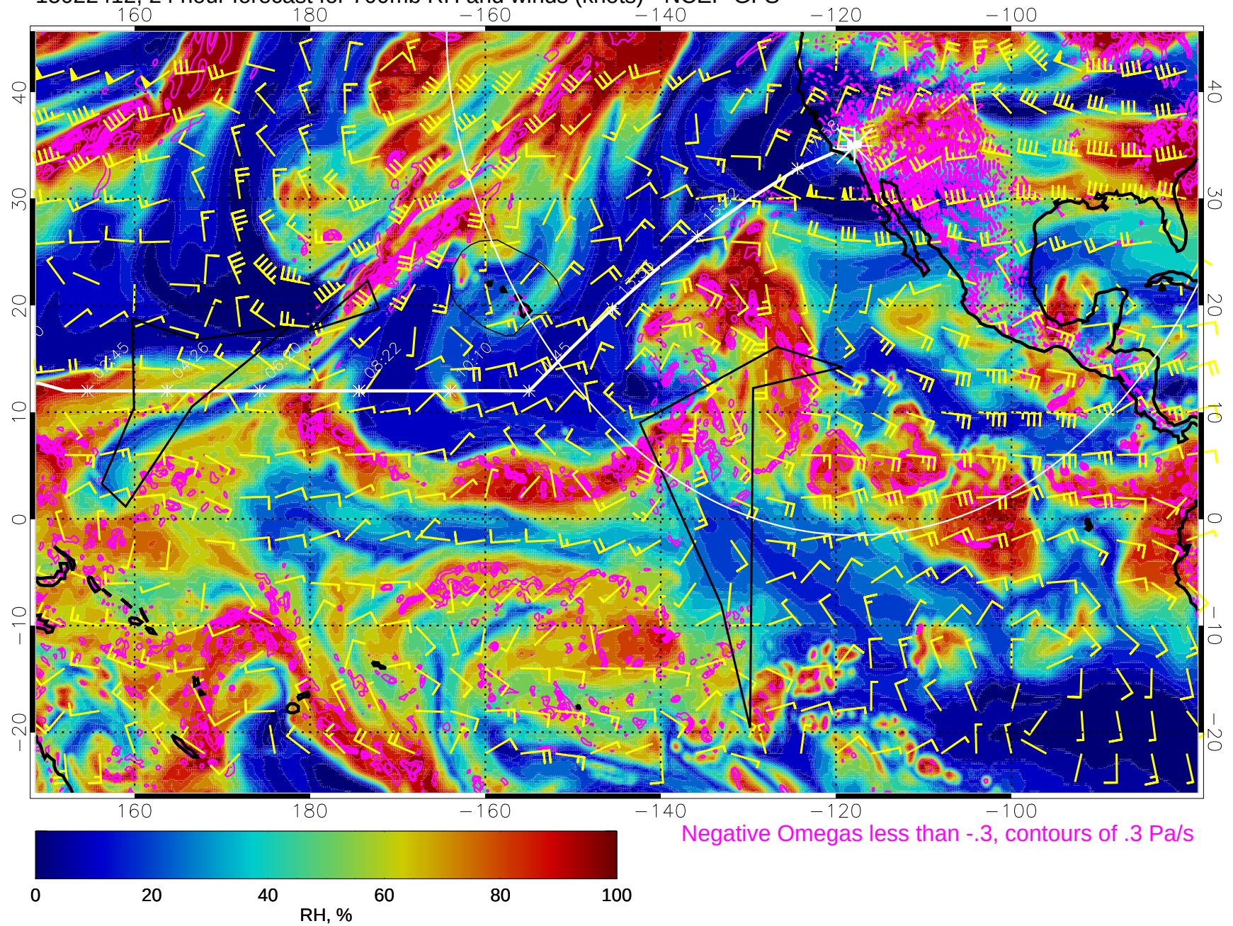
15022412, 24 hour forecast for 700mb RH and winds (knots) - NCEP GFS
