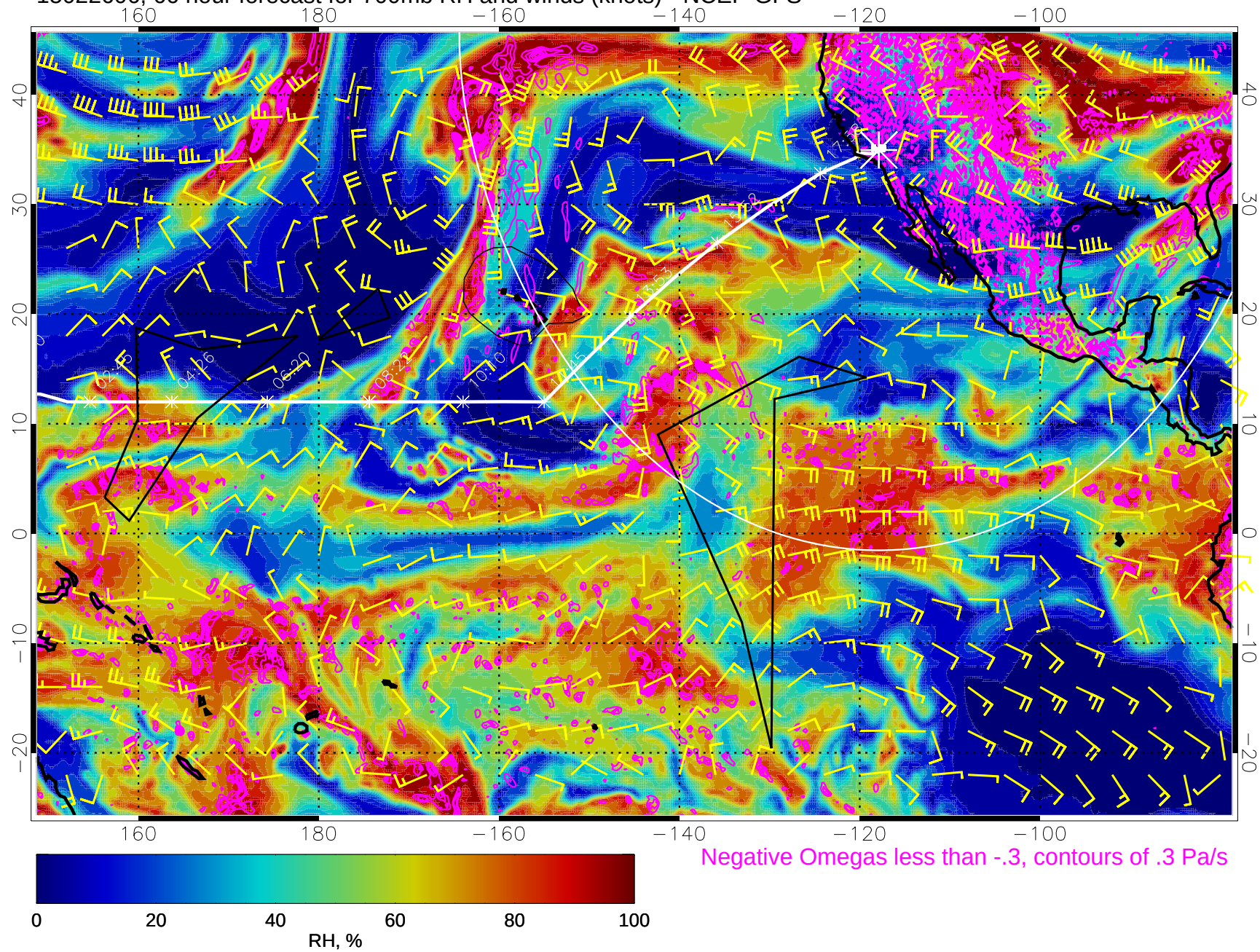
15022606, 66 hour forecast for 700mb RH and winds (knots) - NCEP GFS
