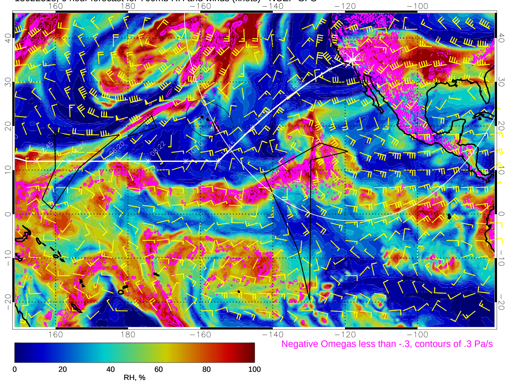
15022318, 6 hour forecast for 700mb RH and winds (knots) - NCEP GFS
