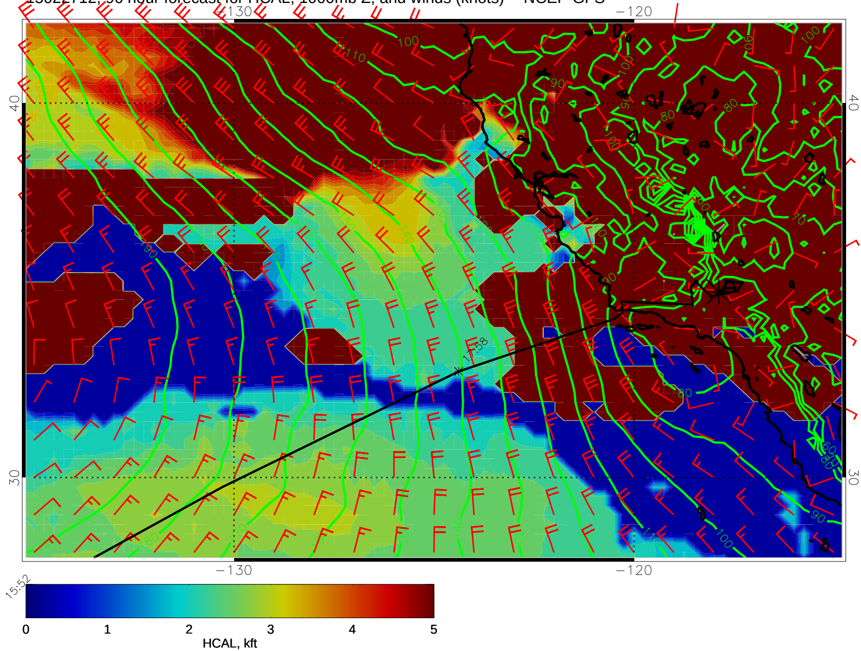
15022712, 96 hour forecast for HCAL, 1000mb Z, and winds (knots) -- NCEP GFS
