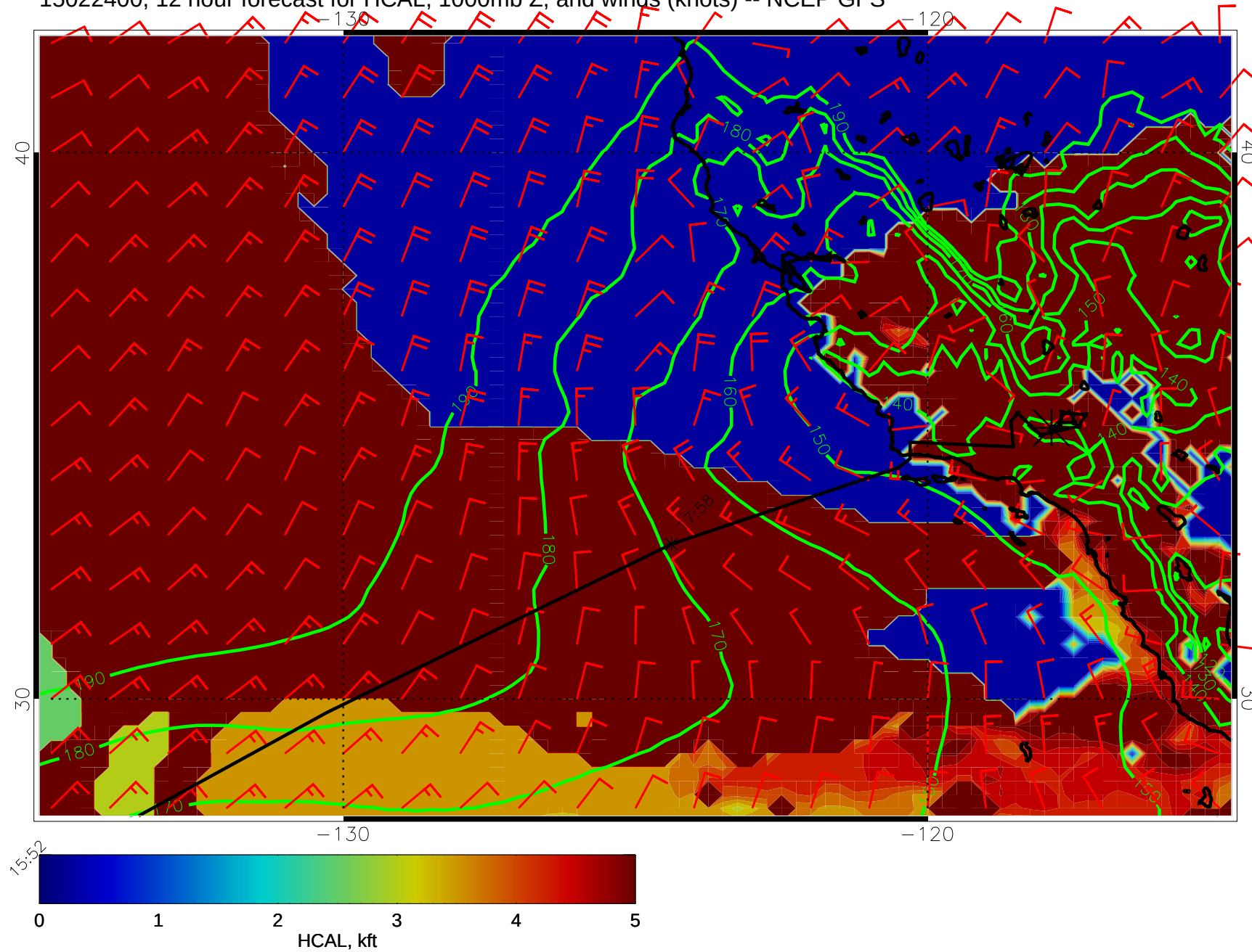
15022400, 12 hour forecast for HCAL, 1000mb Z, and winds (knots) -- NCEP GFS
