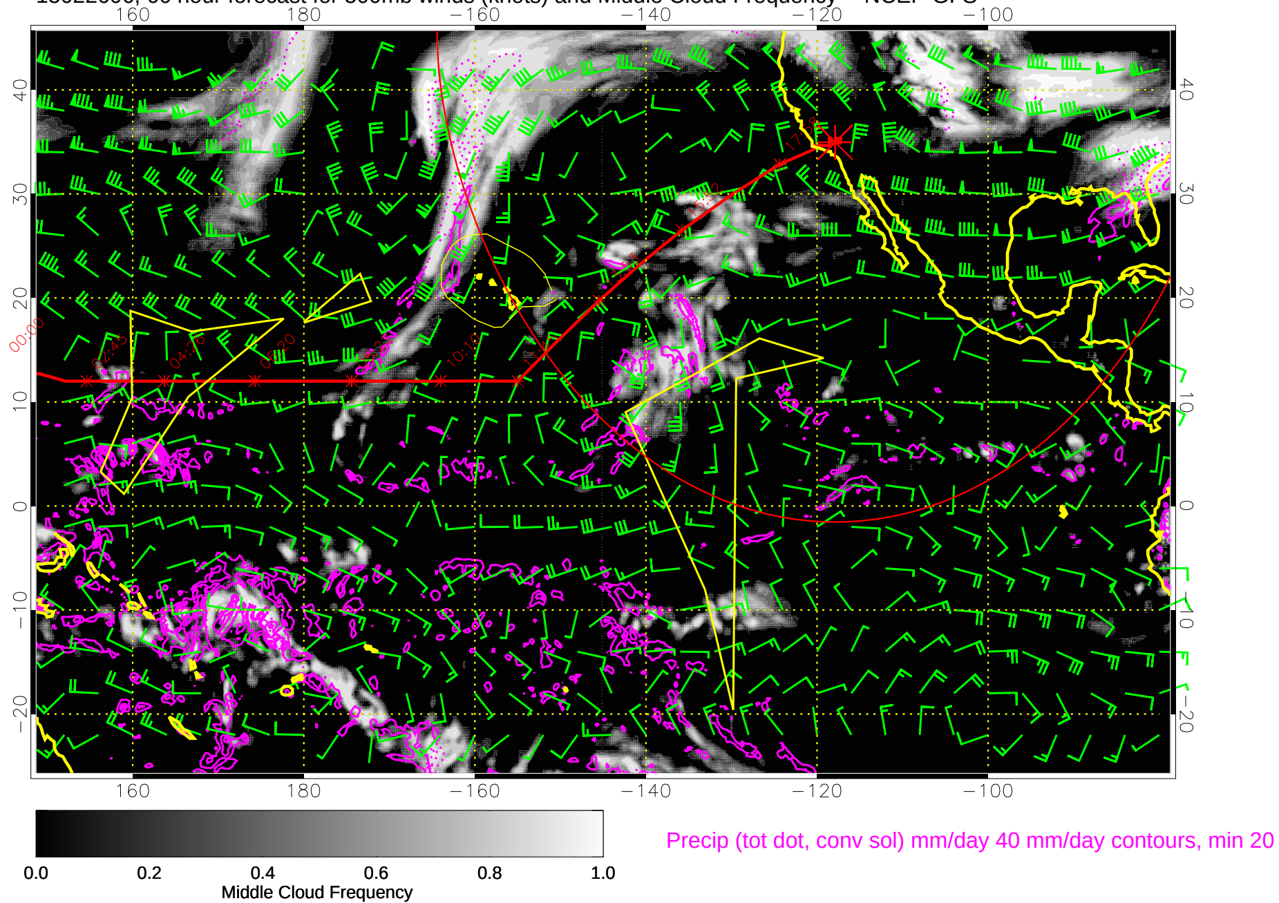
15022606, 66 hour forecast for 500mb winds (knots) and Middle Cloud Frequency -- NCEP GFS
