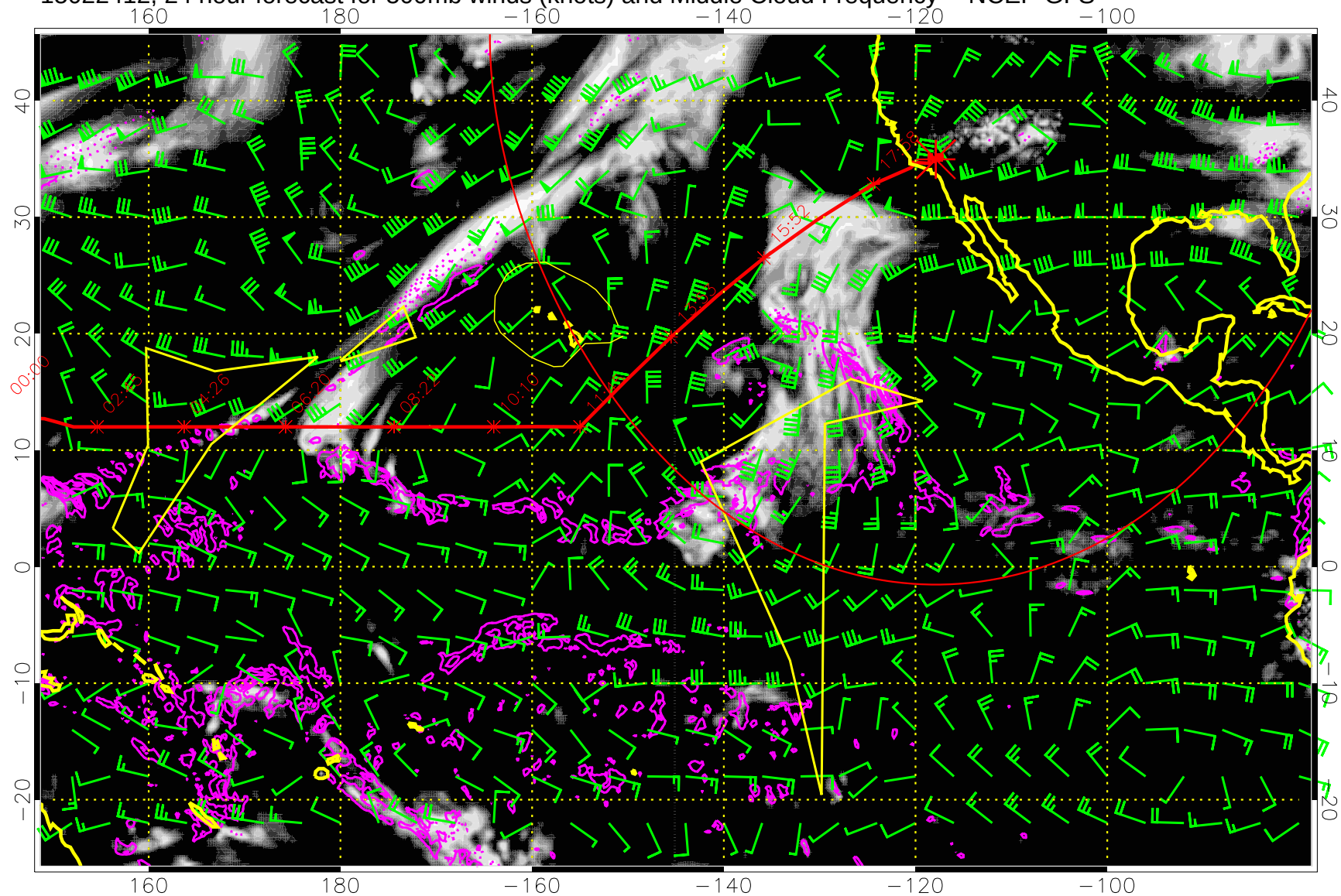
15022412, 24 hour forecast for 500mb winds (knots) and Middle Cloud Frequency -- NCEP GFS
