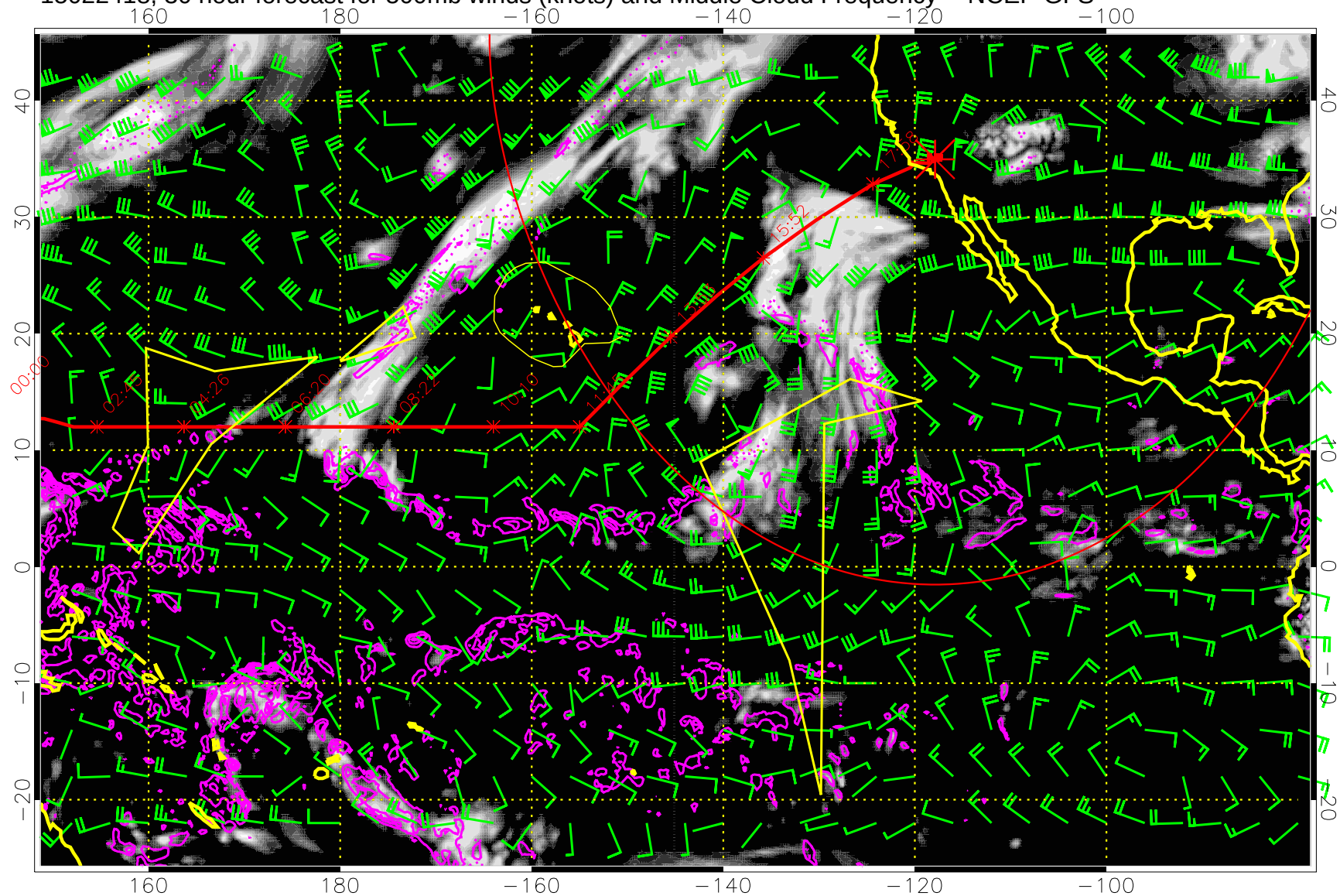
15022418, 30 hour forecast for 500mb winds (knots) and Middle Cloud Frequency -- NCEP GFS
