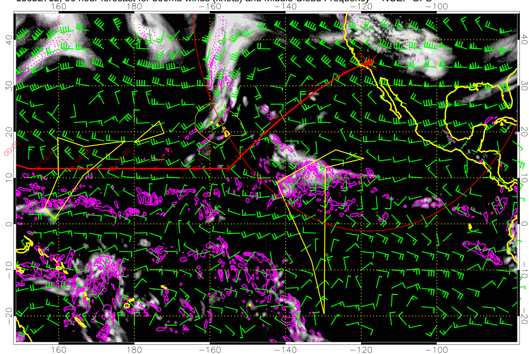
15022712, 96 hour forecast for 500mb winds (knots) and Middle Cloud Frequency -- NCEP GFS
