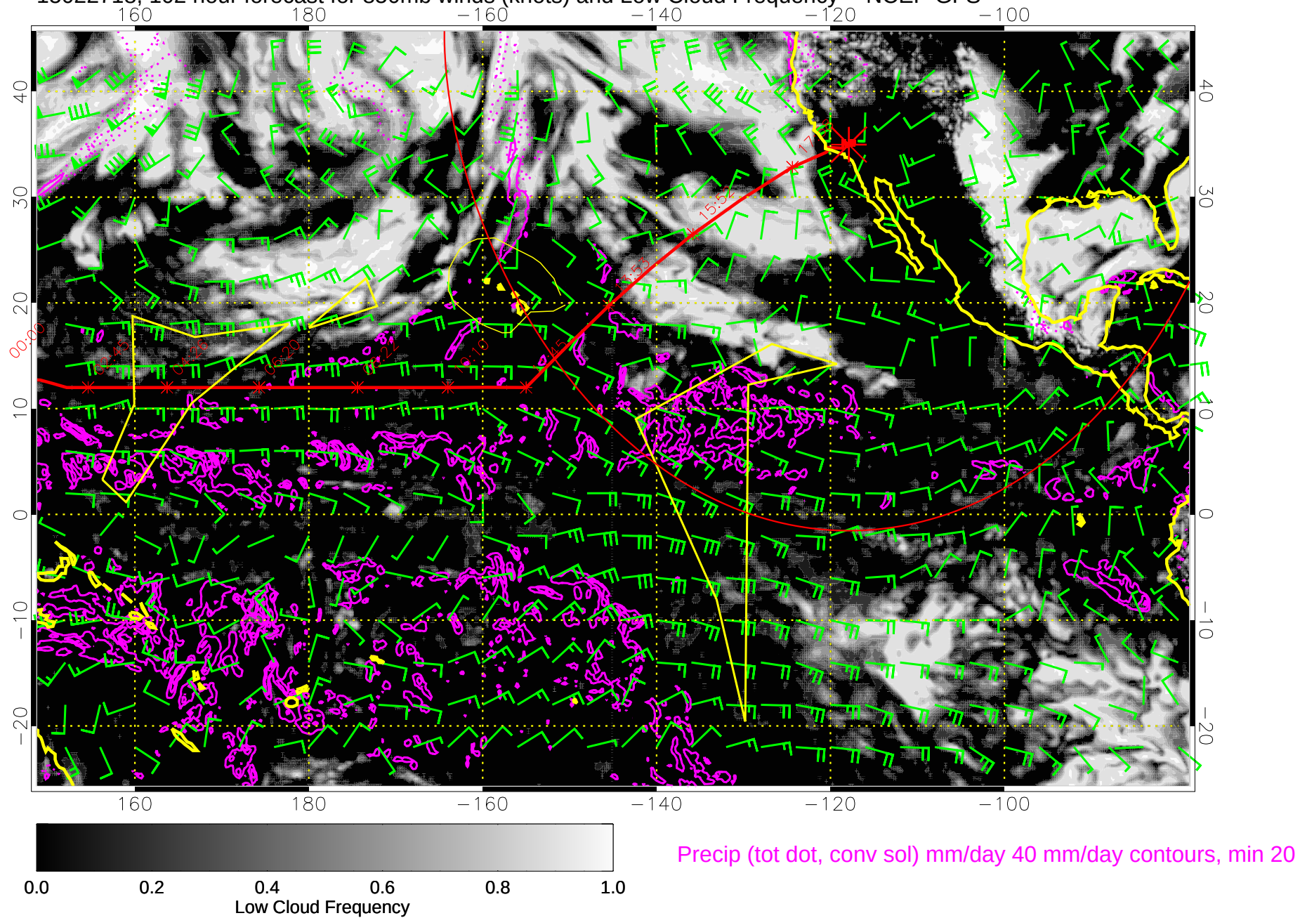
15022718, 102 hour forecast for 850mb winds (knots) and Low Cloud Frequency -- NCEP GFS
