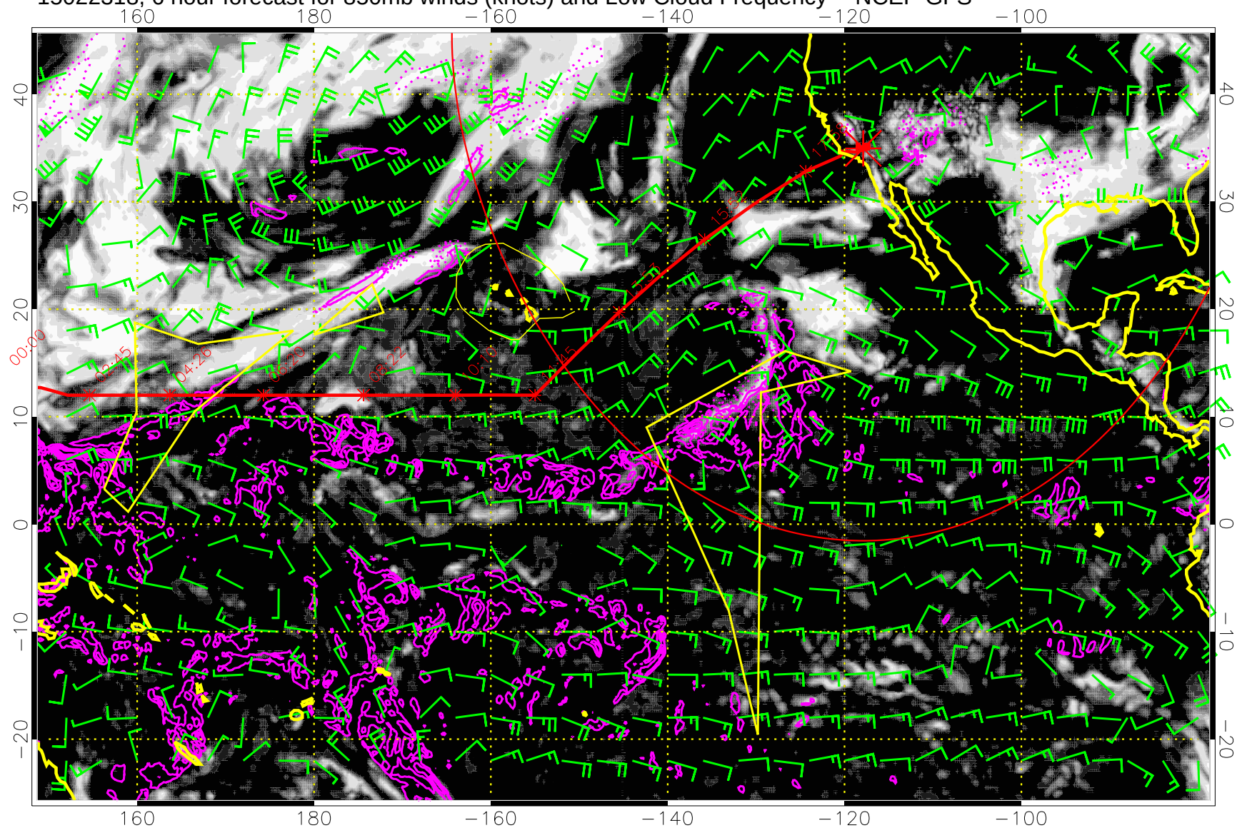
15022318, 6 hour forecast for 850mb winds (knots) and Low Cloud Frequency -- NCEP GFS
