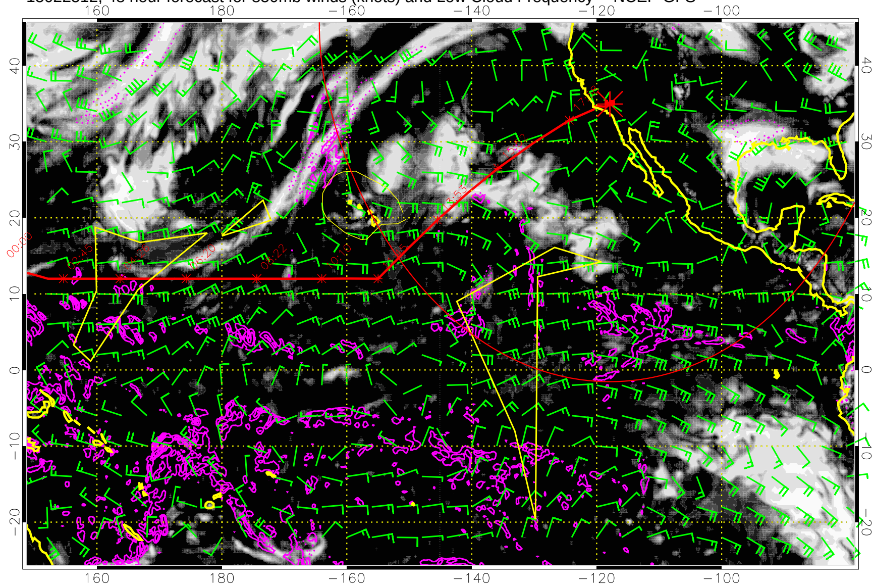
15022512, 48 hour forecast for 850mb winds (knots) and Low Cloud Frequency -- NCEP GFS
