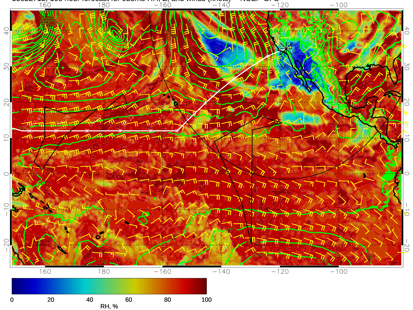
15022712, 108 hour forecast for 925mb RH, Z, and winds (knots) -- NCEP GFS
