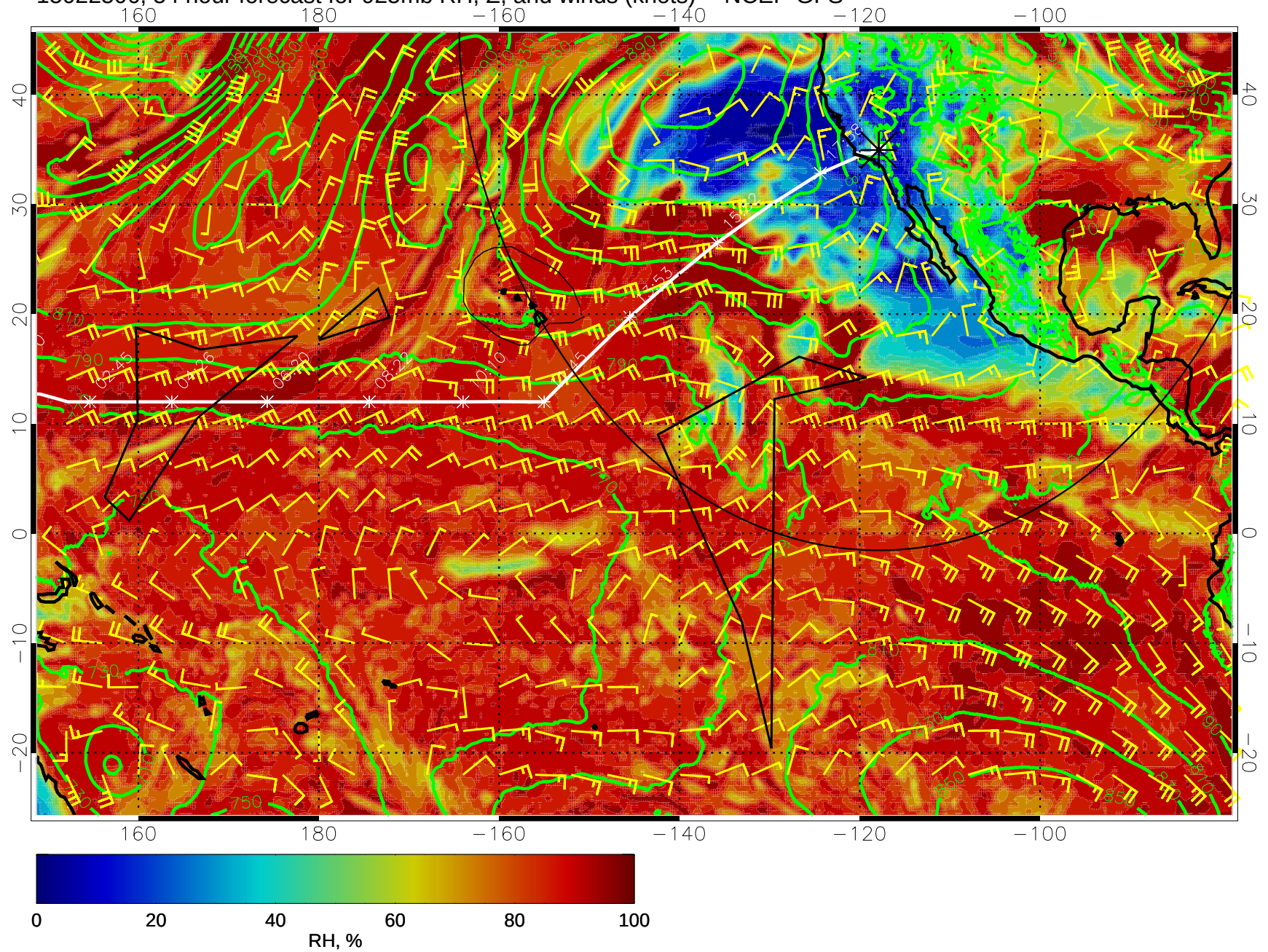
15022506, 54 hour forecast for 925mb RH, Z, and winds (knots) -- NCEP GFS
