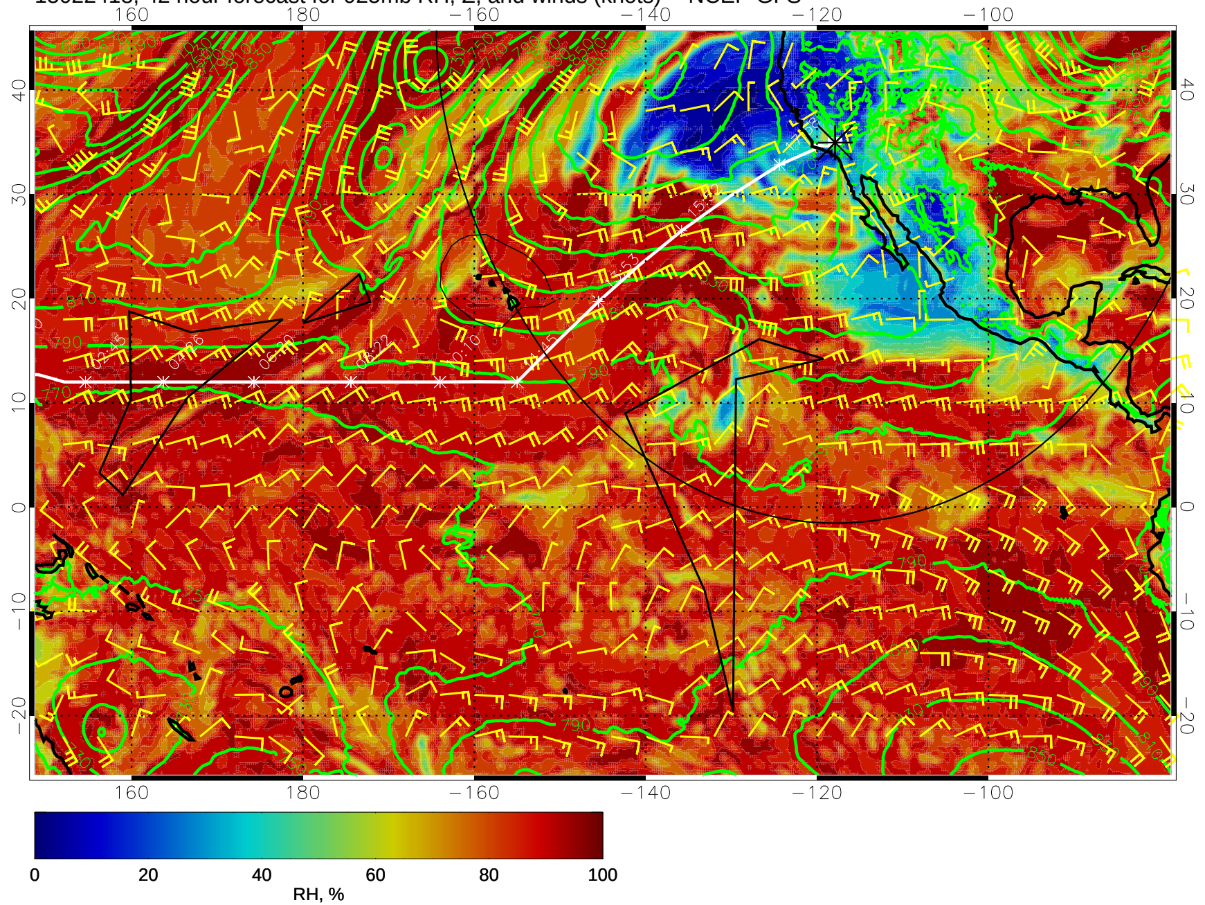
15022418, 42 hour forecast for 925mb RH, Z, and winds (knots) -- NCEP GFS
