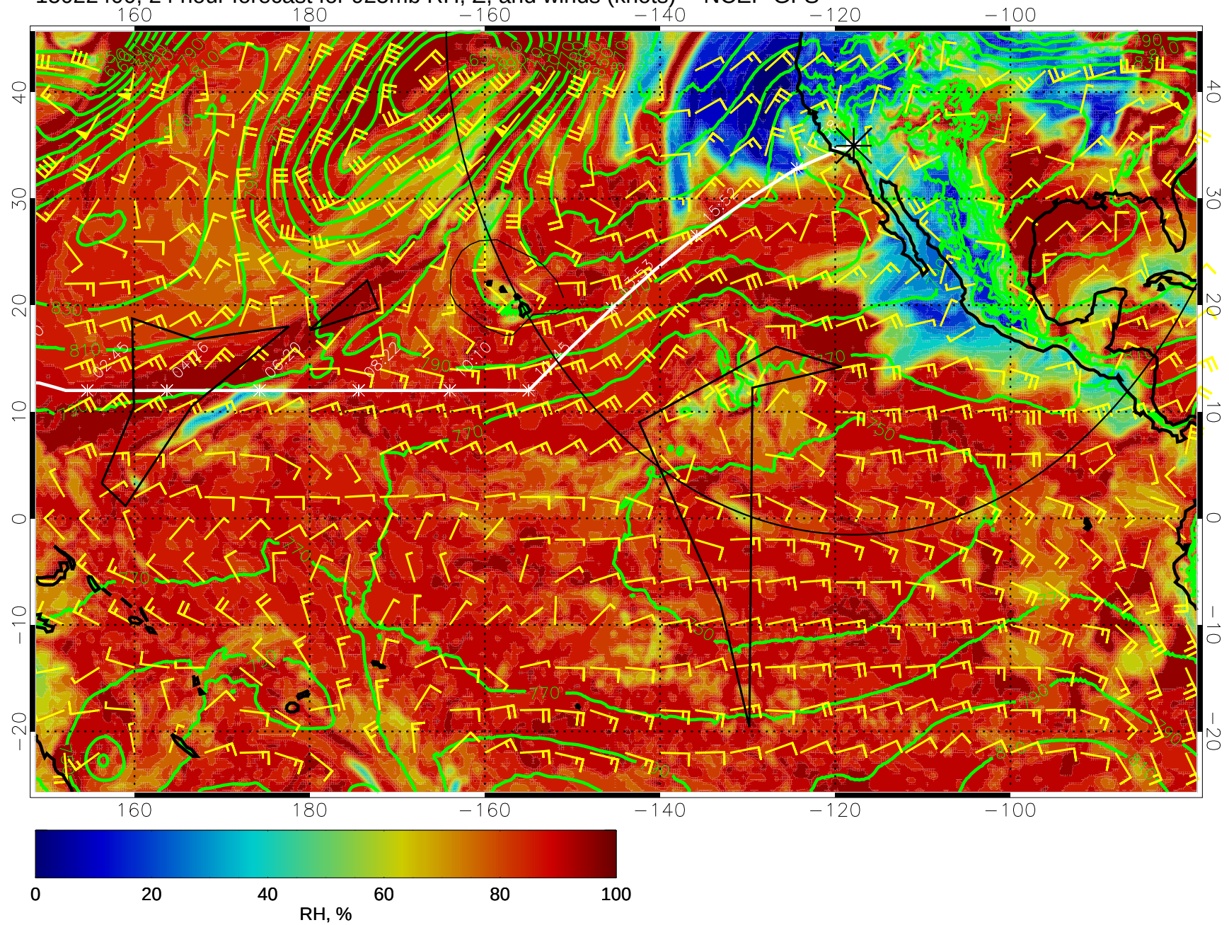
15022400, 24 hour forecast for 925mb RH, Z, and winds (knots) -- NCEP GFS
