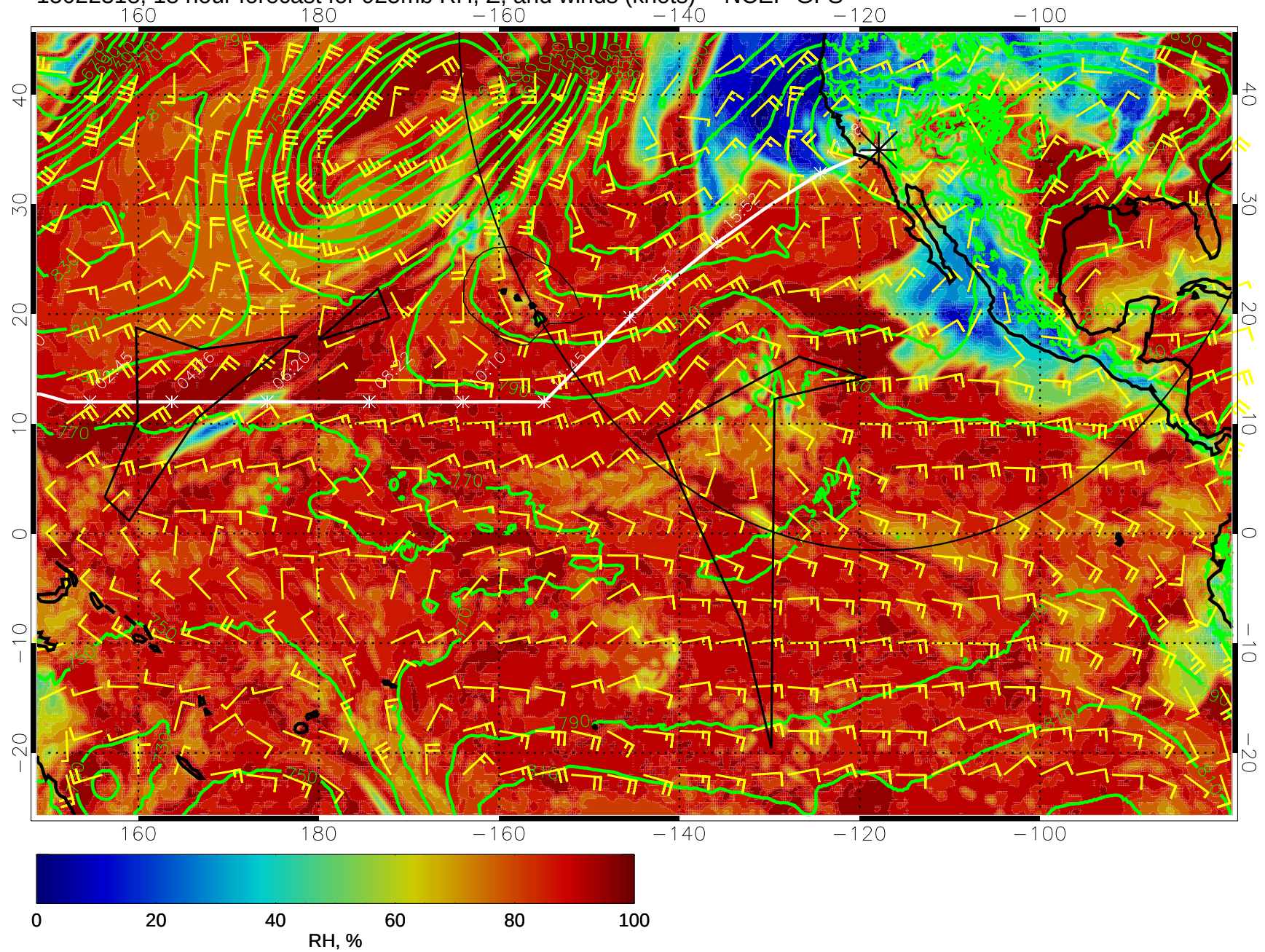
15022318, 18 hour forecast for 925mb RH, Z, and winds (knots) -- NCEP GFS
