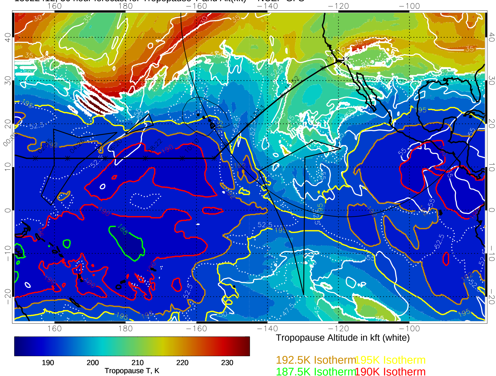
15022412, 36 hour forecast for Tropopause T and Alt(kft) -- NCEP GFS
