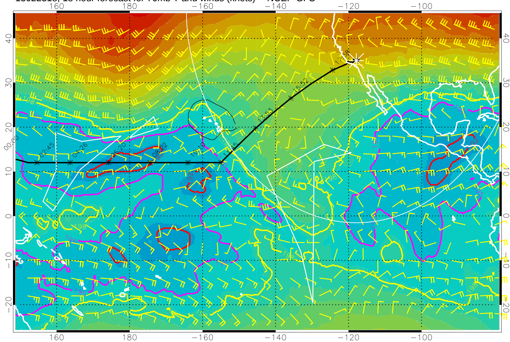
15022318, 18 hour forecast for 70mb T and winds (knots) -- NCEP GFS
