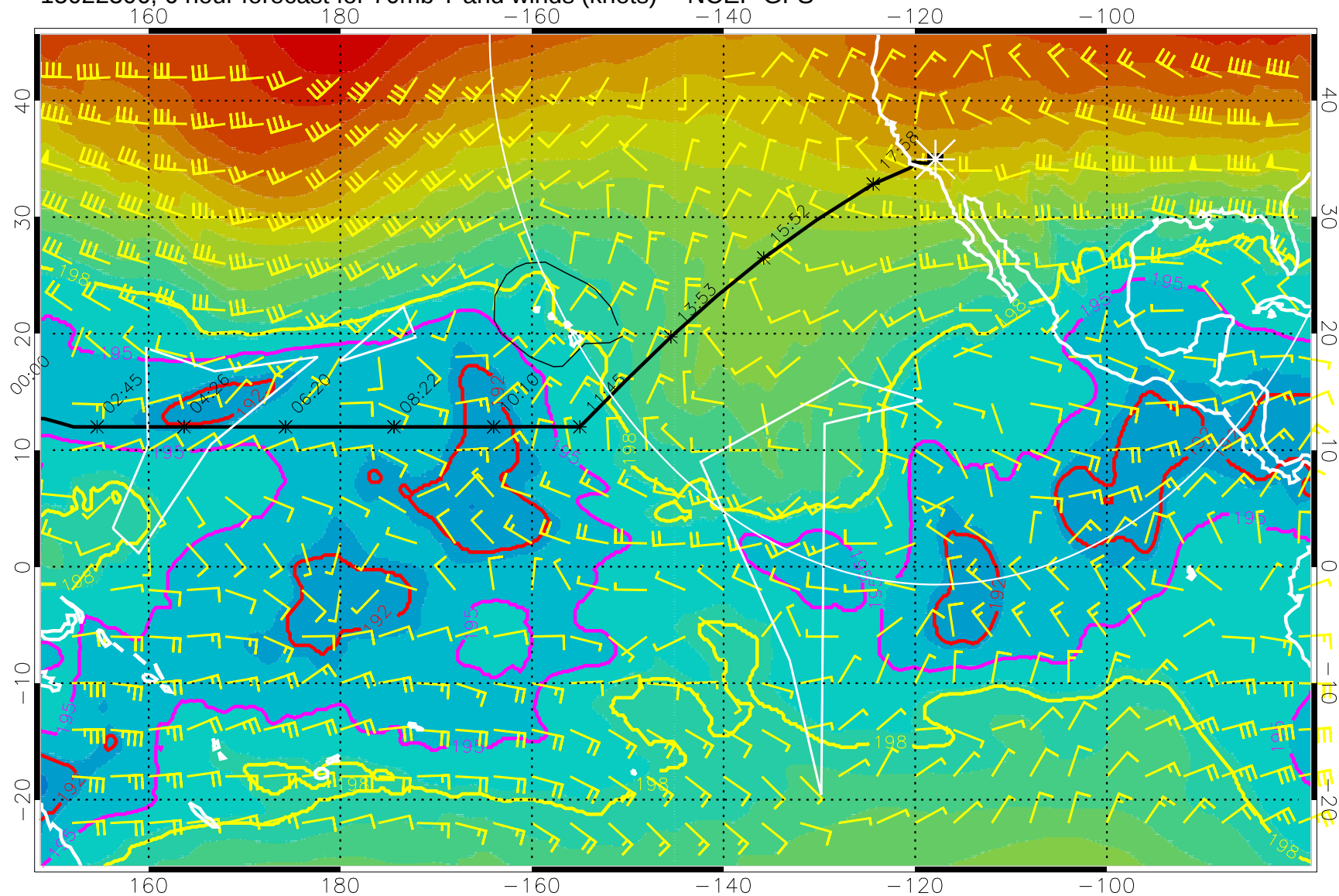
15022306, 6 hour forecast for 70mb T and winds (knots) -- NCEP GFS
