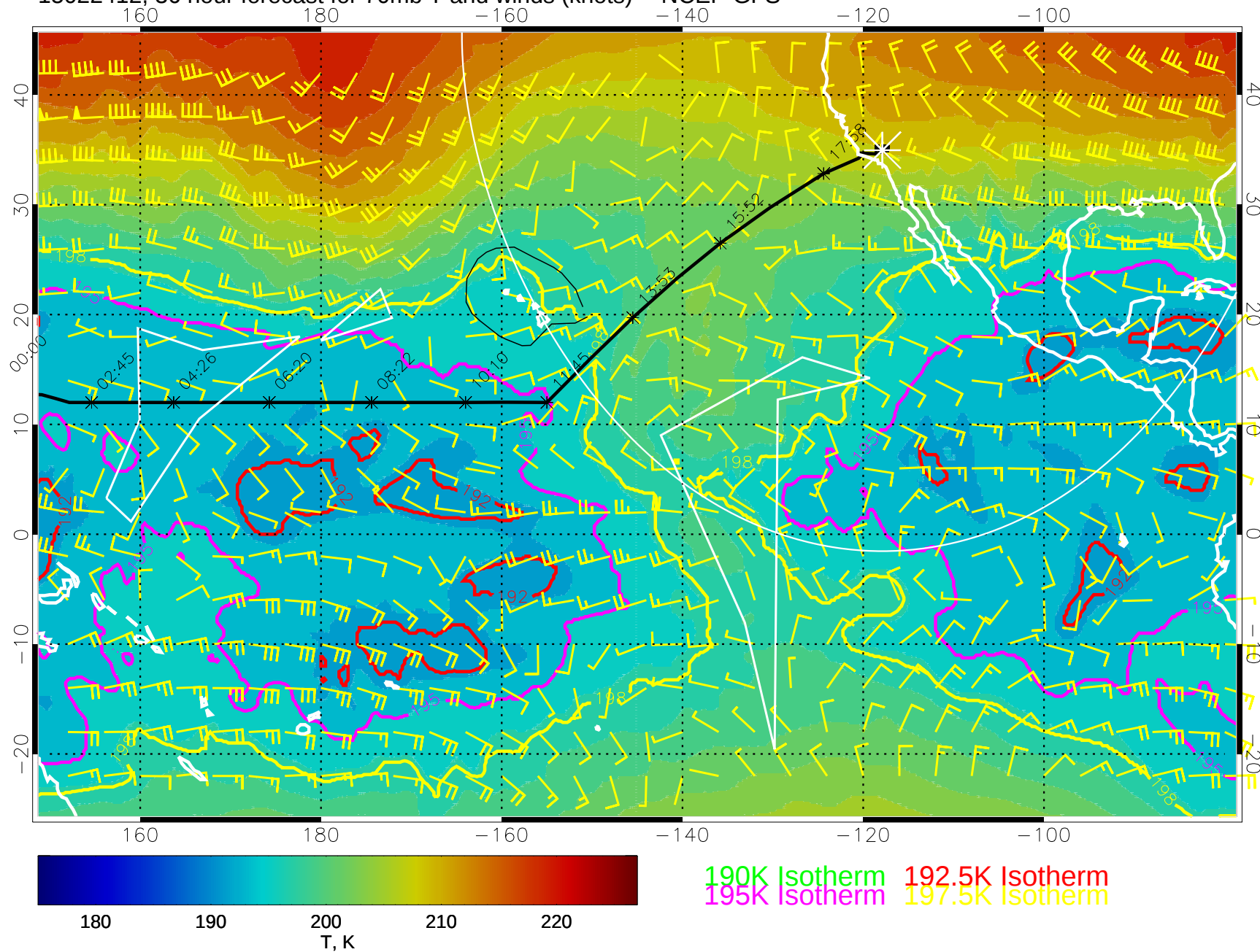
15022412, 36 hour forecast for 70mb T and winds (knots) -- NCEP GFS
