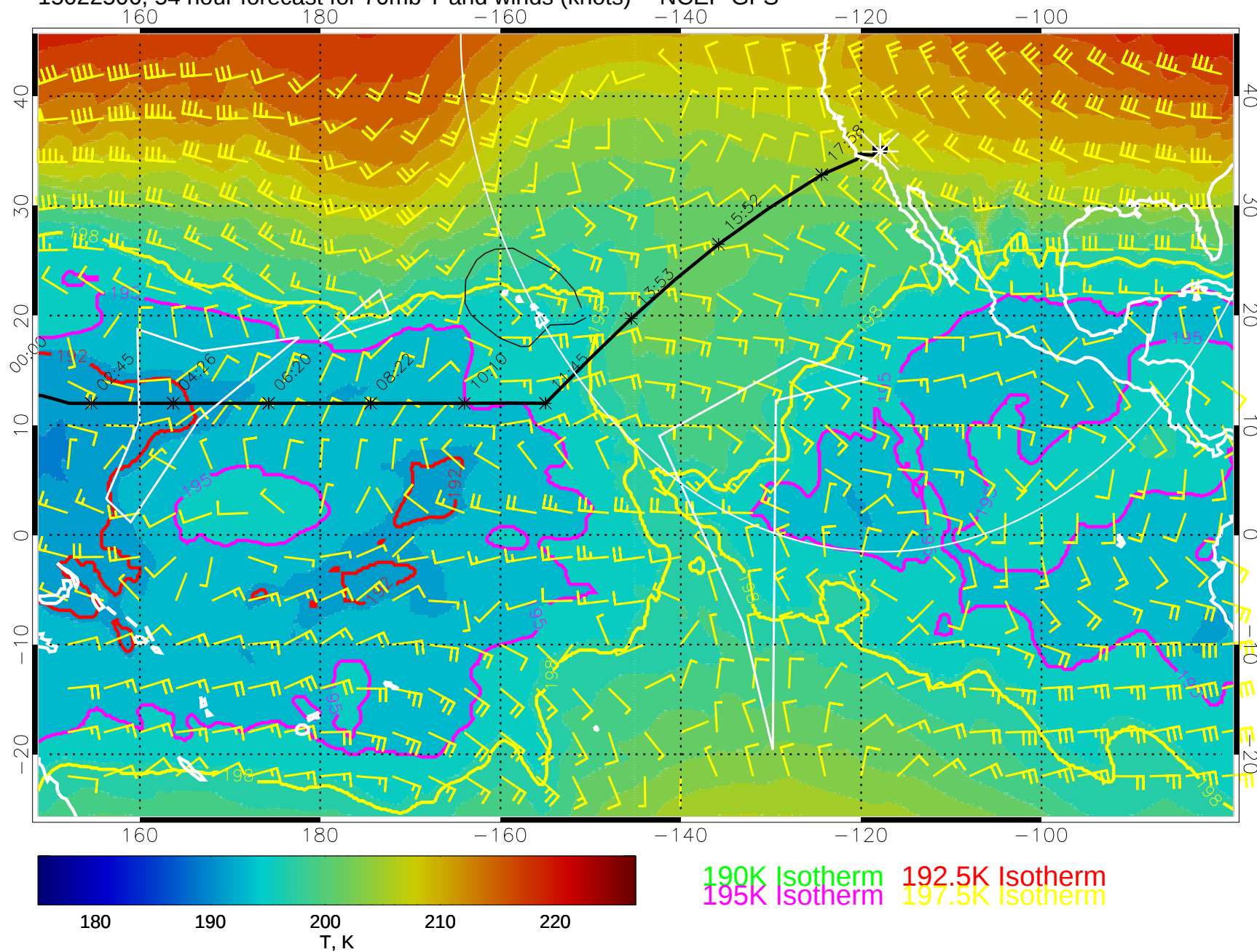
15022506, 54 hour forecast for 70mb T and winds (knots) -- NCEP GFS
