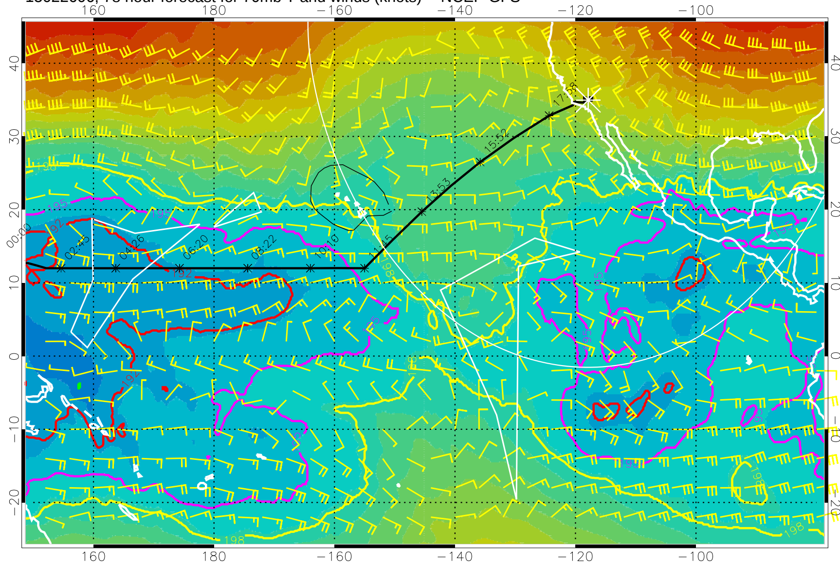
15022606, 78 hour forecast for 70mb T and winds (knots) -- NCEP GFS
