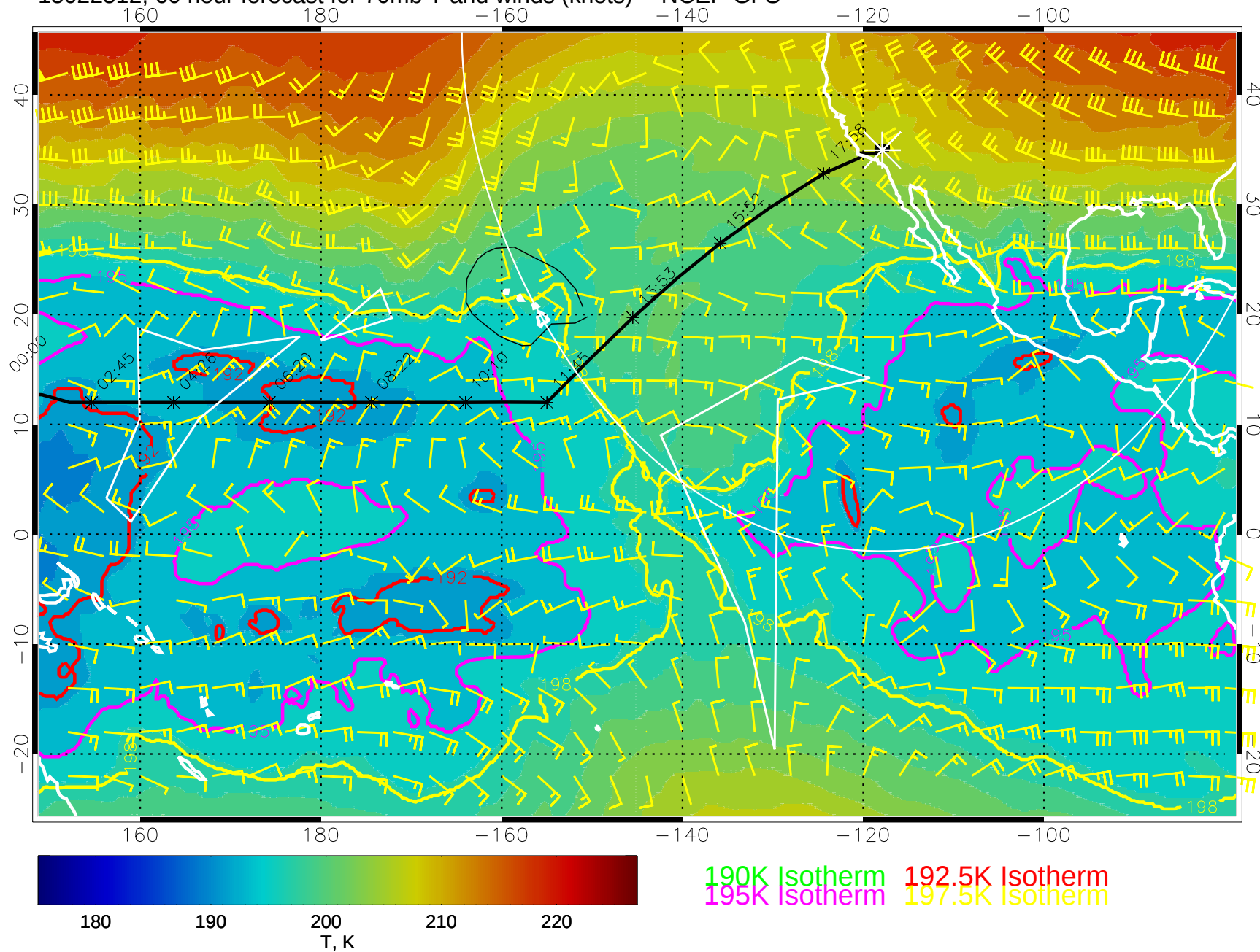
15022512, 60 hour forecast for 70mb T and winds (knots) -- NCEP GFS
