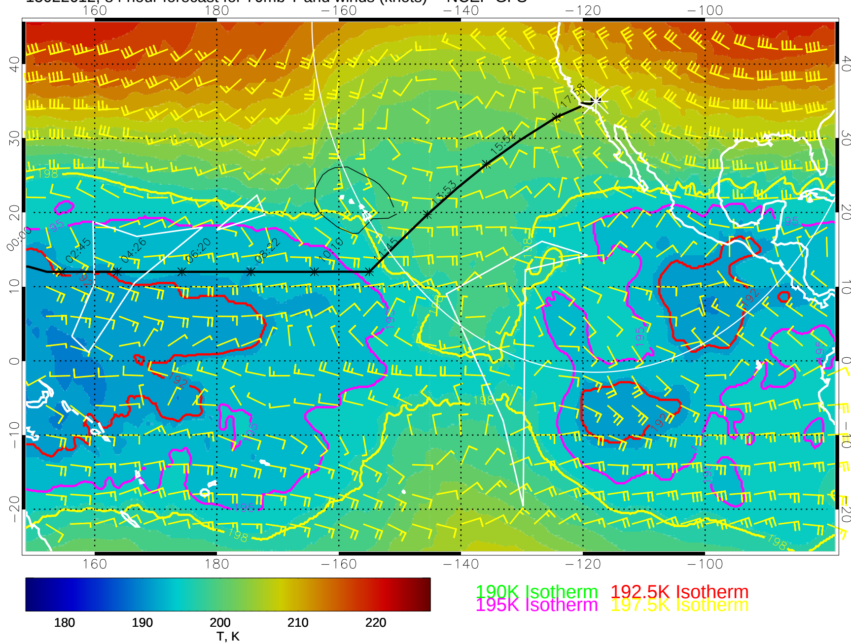
15022612, 84 hour forecast for 70mb T and winds (knots) -- NCEP GFS
