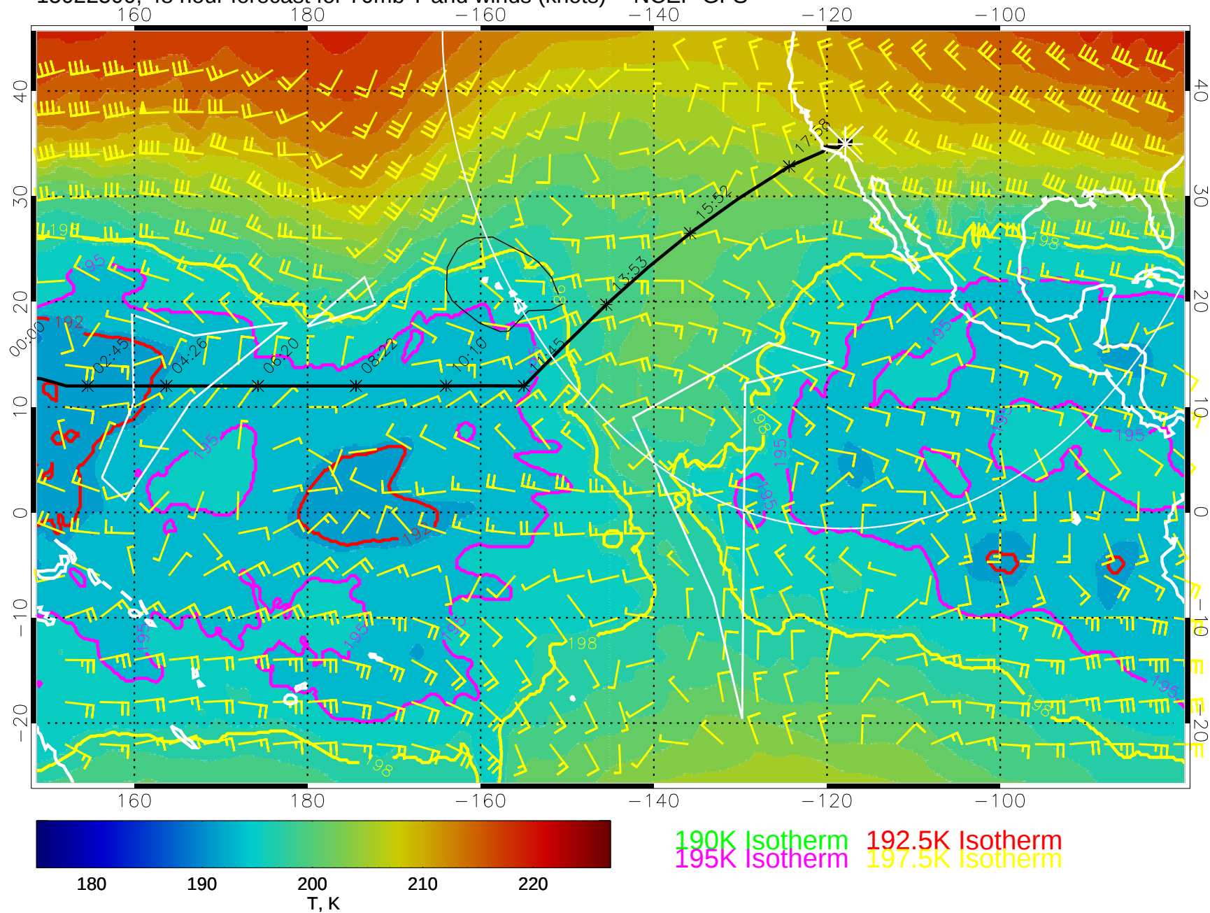
15022500, 48 hour forecast for 70mb T and winds (knots) -- NCEP GFS
