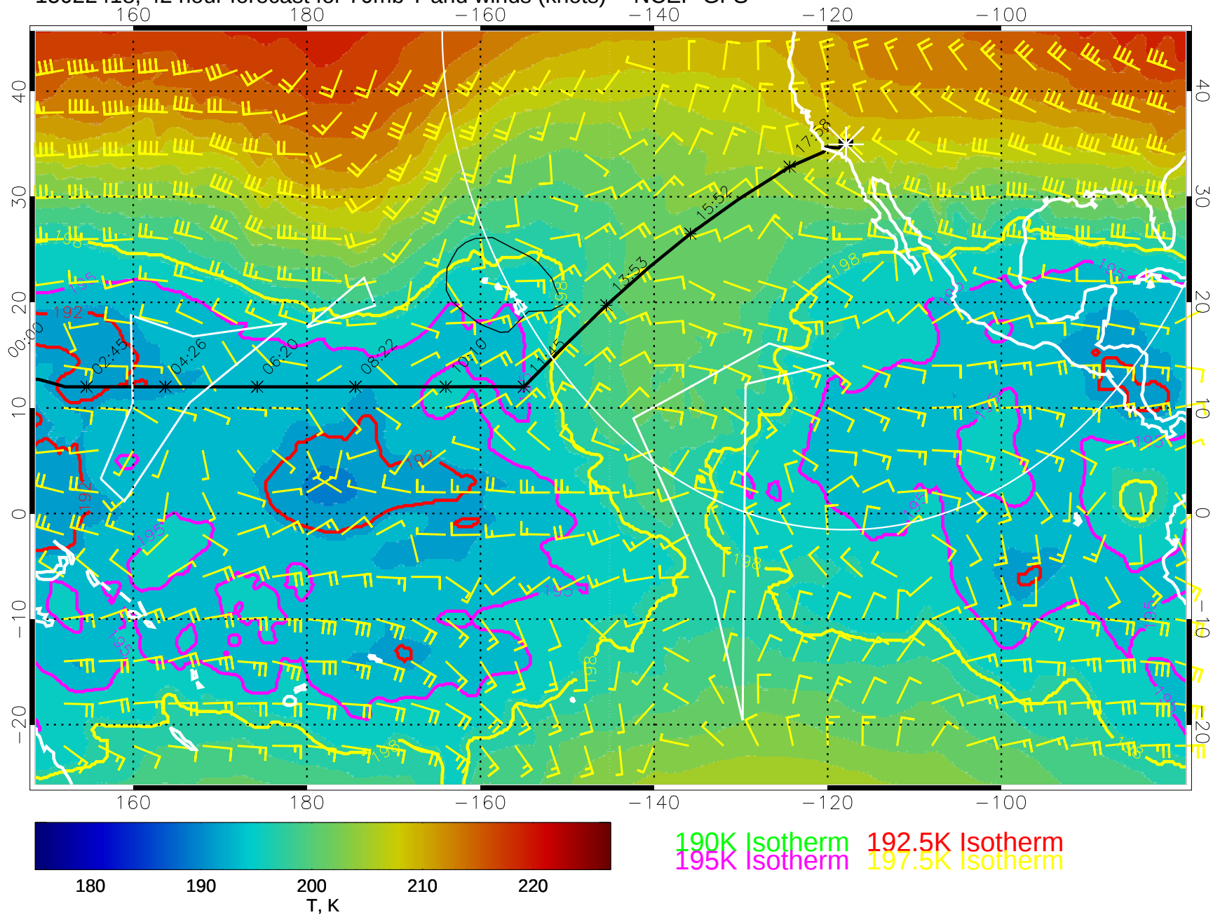
15022418, 42 hour forecast for 70mb T and winds (knots) -- NCEP GFS
