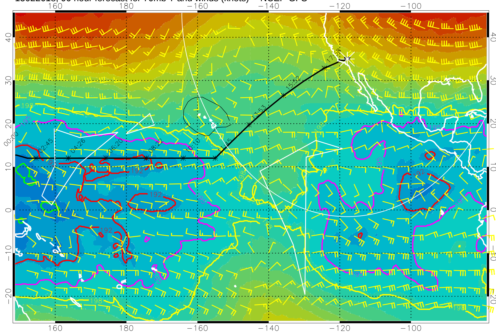
15022618, 90 hour forecast for 70mb T and winds (knots) -- NCEP GFS
