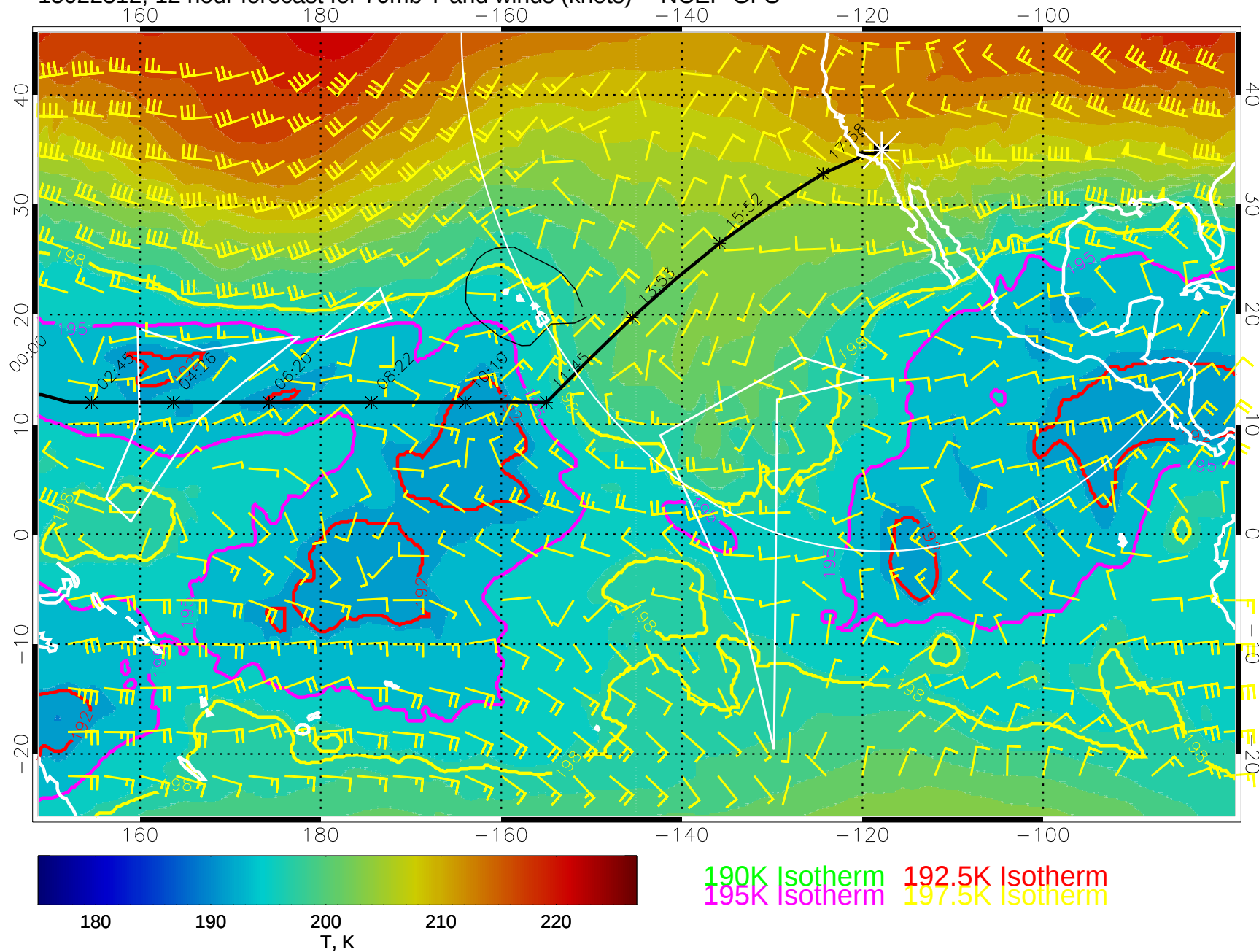
15022312, 12 hour forecast for 70mb T and winds (knots) -- NCEP GFS
