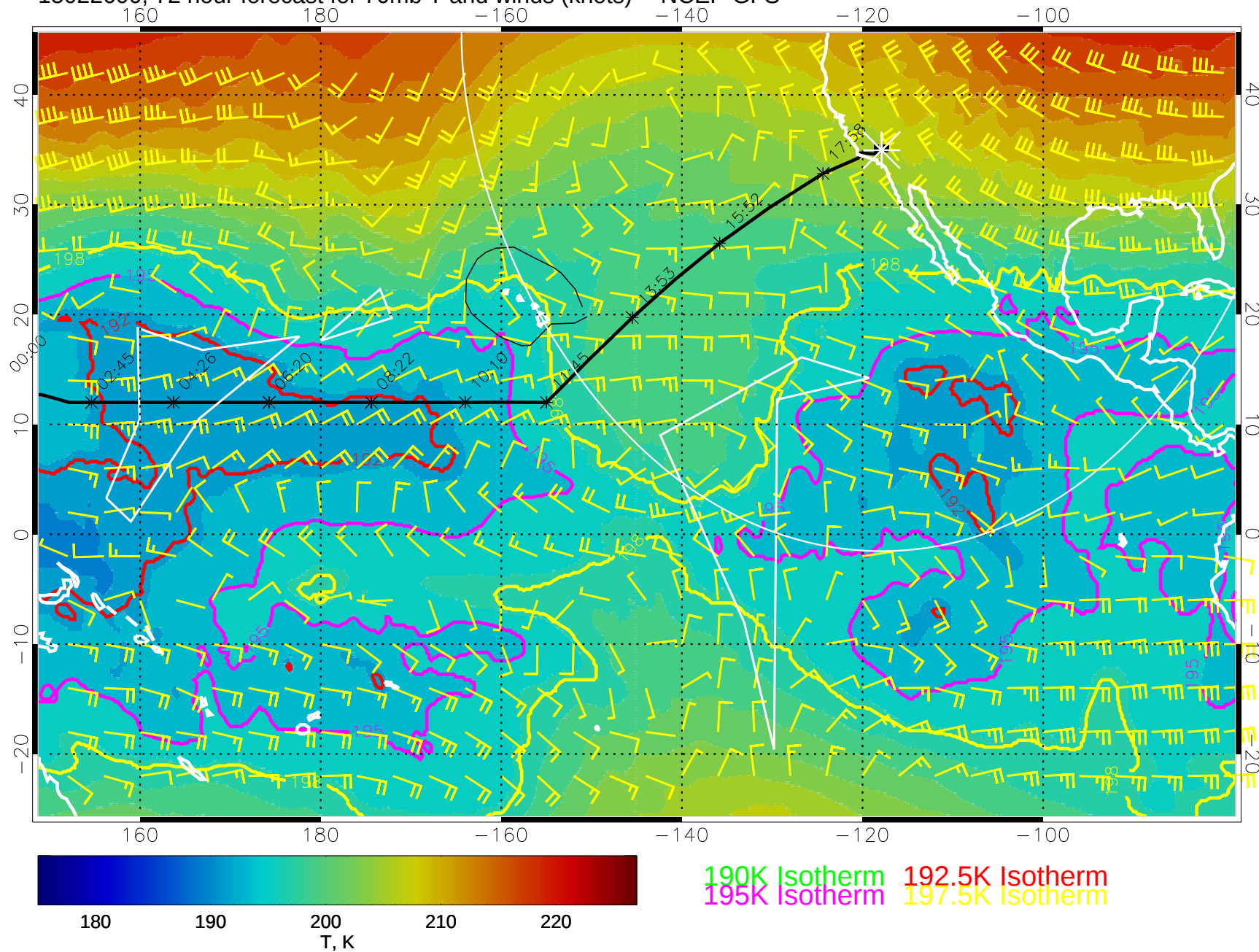
15022600, 72 hour forecast for 70mb T and winds (knots) -- NCEP GFS
