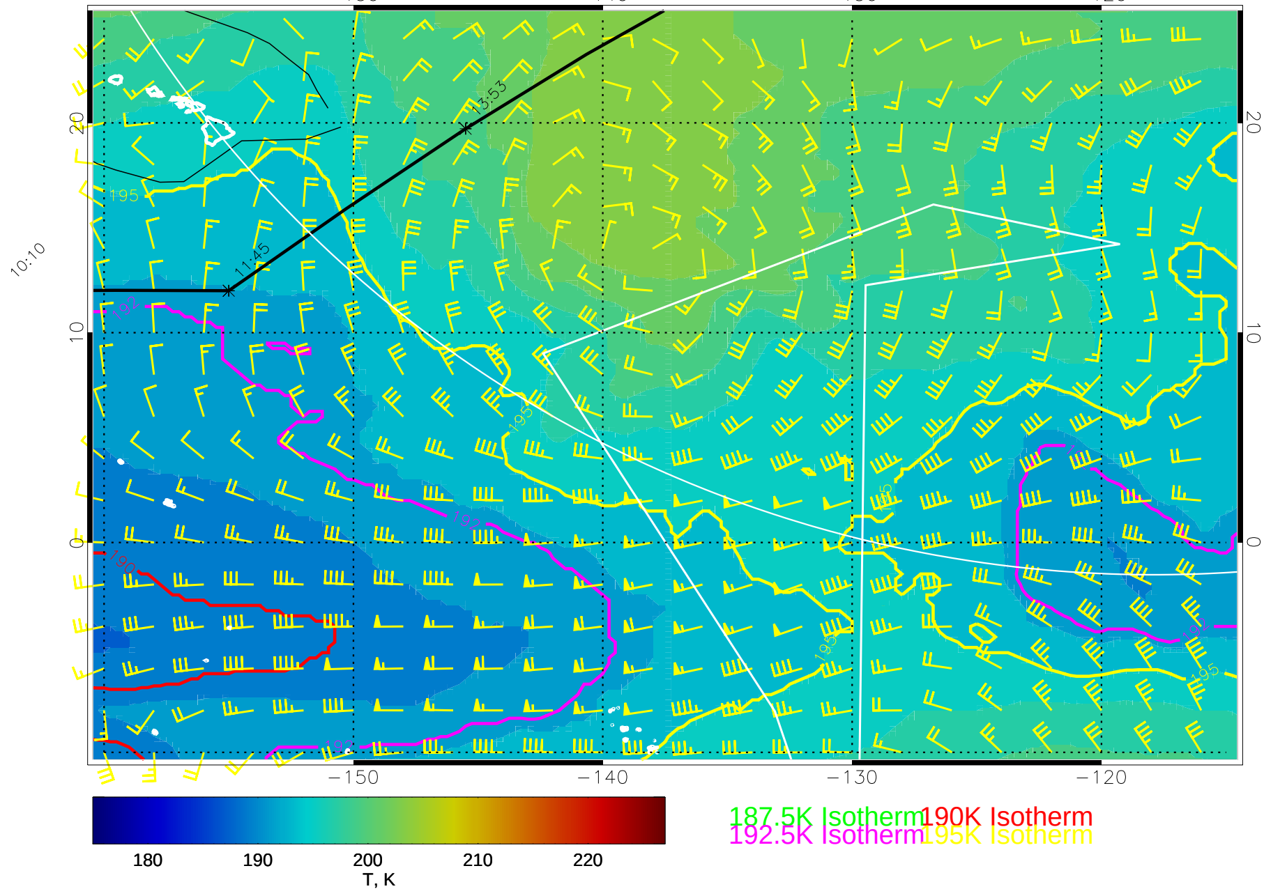
15022600, 72 hour forecast for 100mb T and winds (knots) -- NCEP GFS
