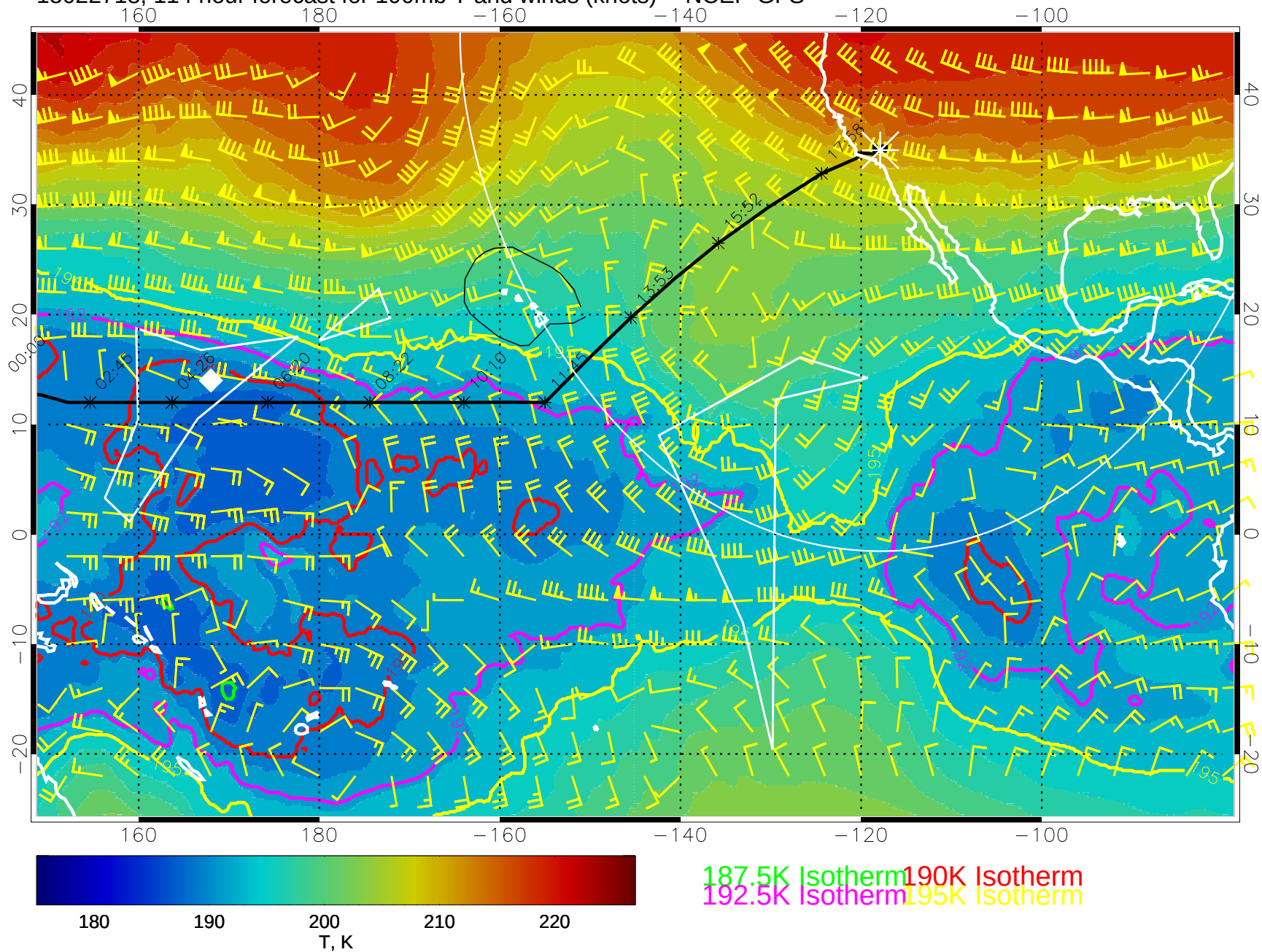
15022718, 114 hour forecast for 100mb T and winds (knots) -- NCEP GFS
