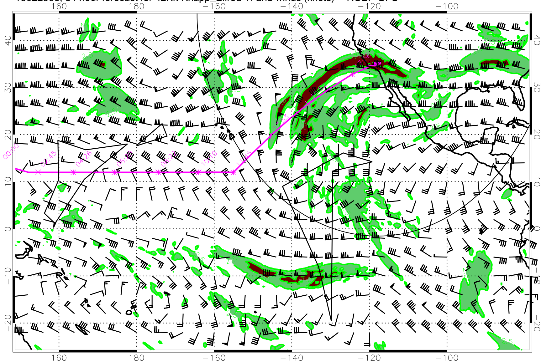
15022506, 54 hour forecast for 42Kft Knapp_Ellrod TI and winds (knots) -- NCEP GFS
