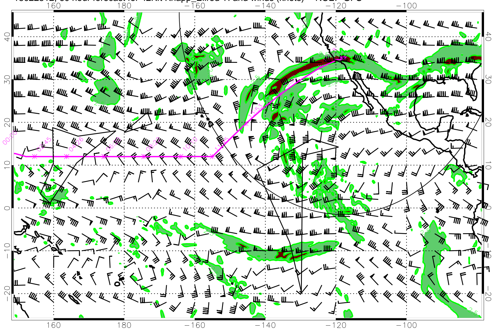
15022512, 60 hour forecast for 42Kft Knapp_Ellrod TI and winds (knots) -- NCEP GFS
