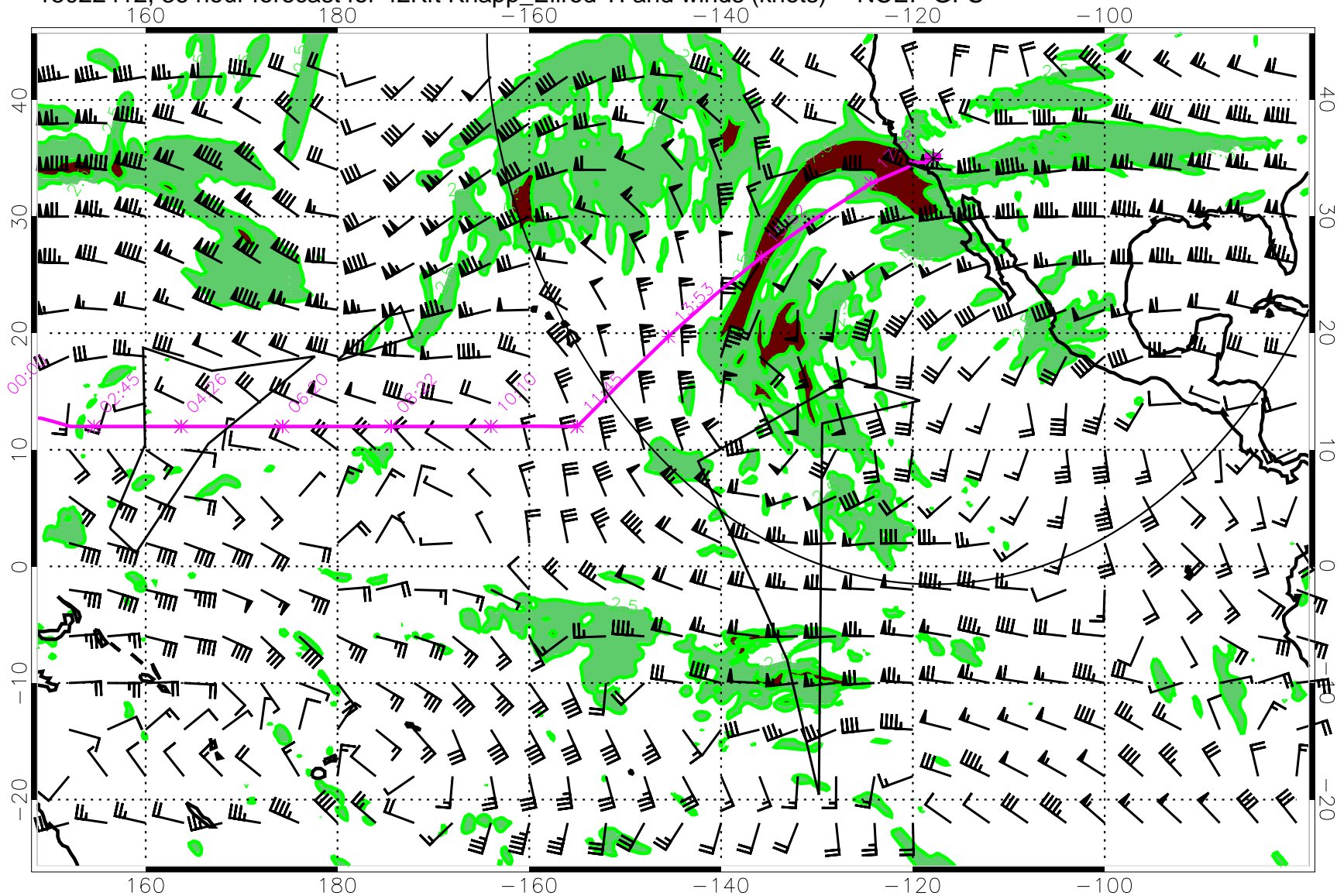
15022412, 36 hour forecast for 42Kft Knapp_Ellrod TI and winds (knots) -- NCEP GFS
