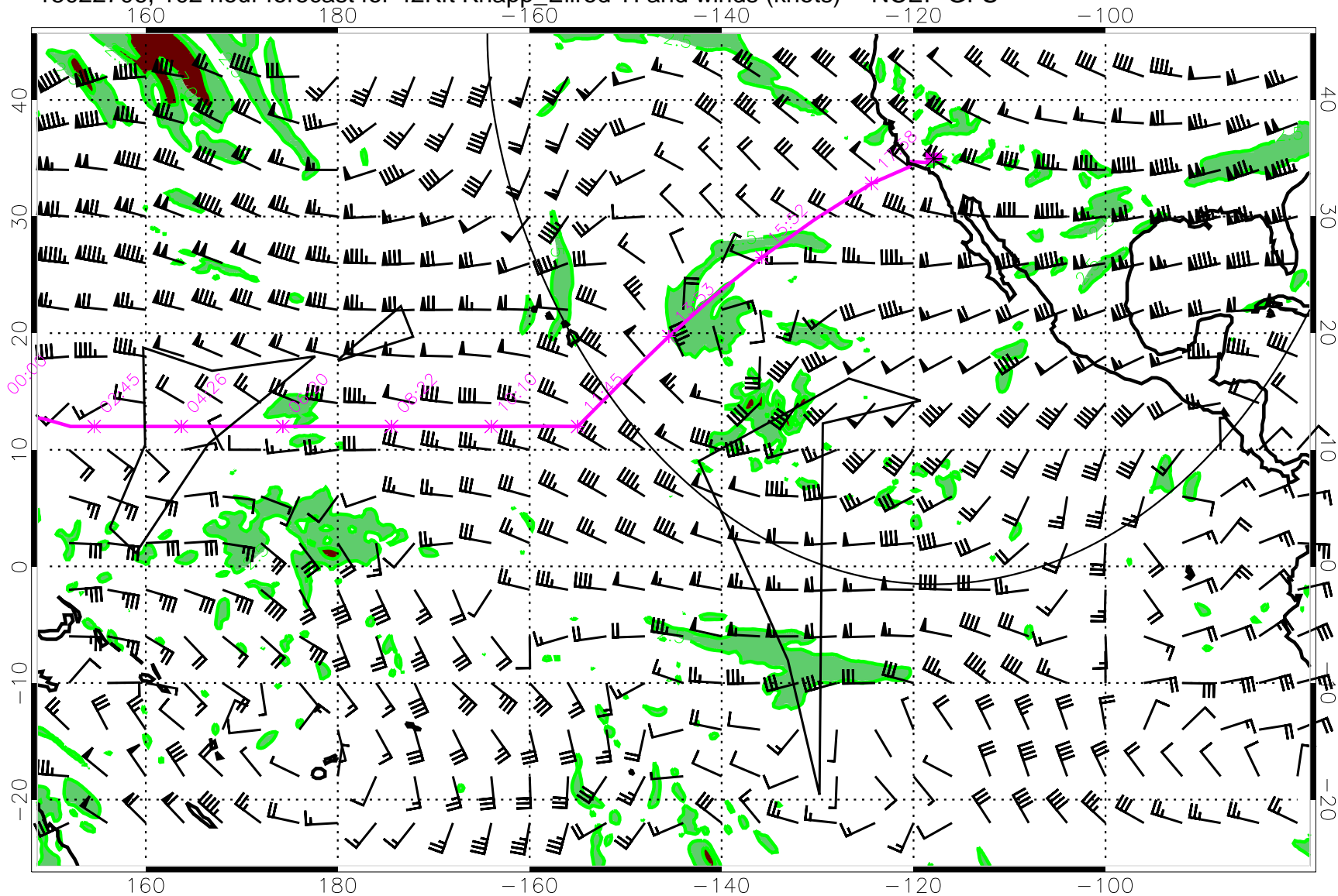
15022706, 102 hour forecast for 42Kft Knapp_Ellrod TI and winds (knots) -- NCEP GFS
