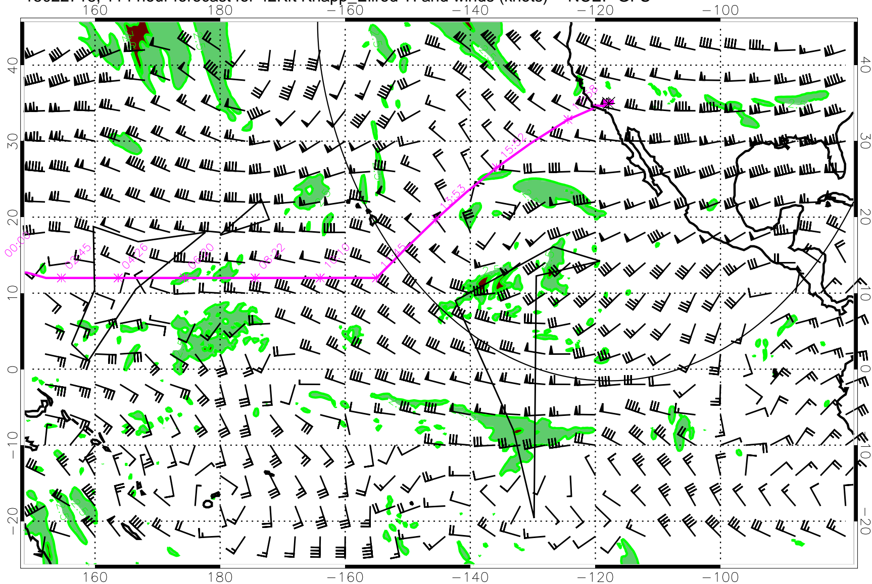
15022718, 114 hour forecast for 42Kft Knapp_Ellrod TI and winds (knots) -- NCEP GFS
