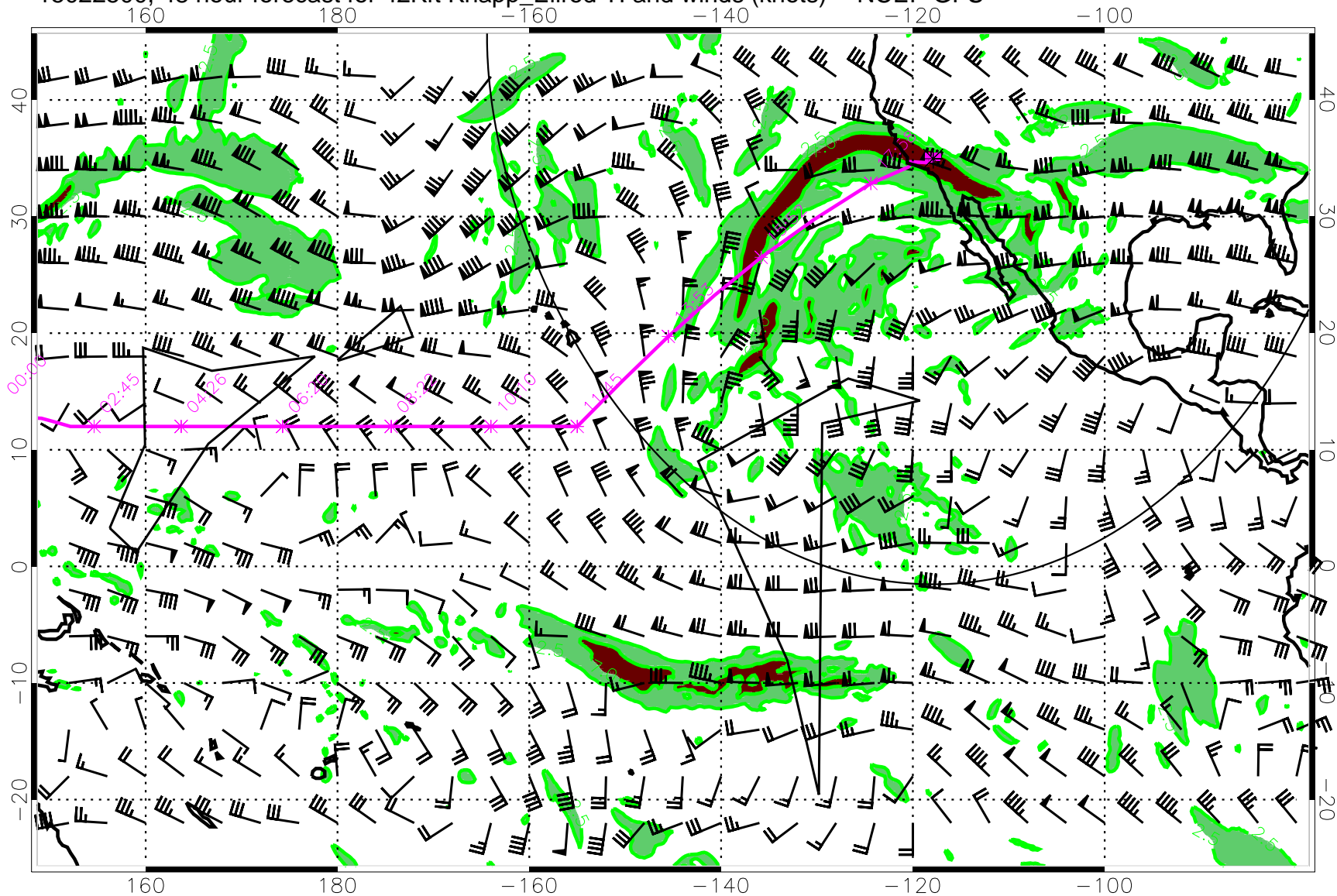
15022500, 48 hour forecast for 42Kft Knapp_Ellrod TI and winds (knots) -- NCEP GFS
