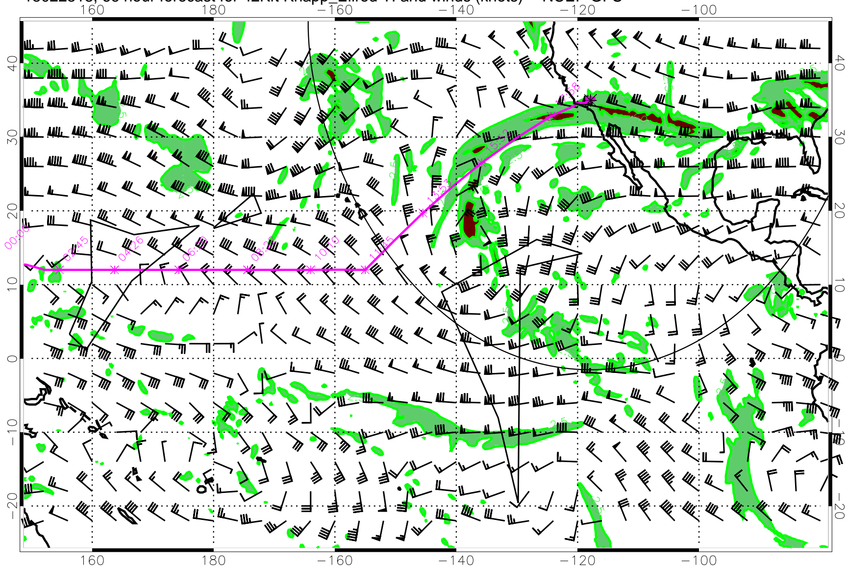
15022518, 66 hour forecast for 42Kft Knapp_Ellrod TI and winds (knots) -- NCEP GFS
