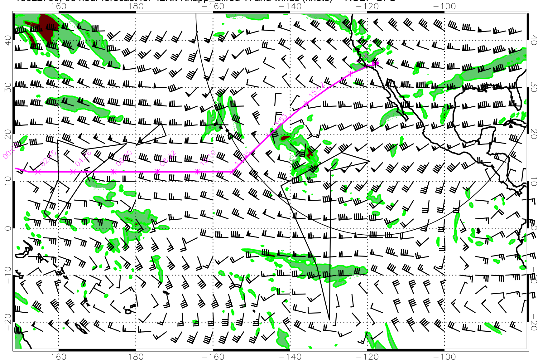
15022700, 96 hour forecast for 42Kft Knapp_Ellrod TI and winds (knots) -- NCEP GFS
