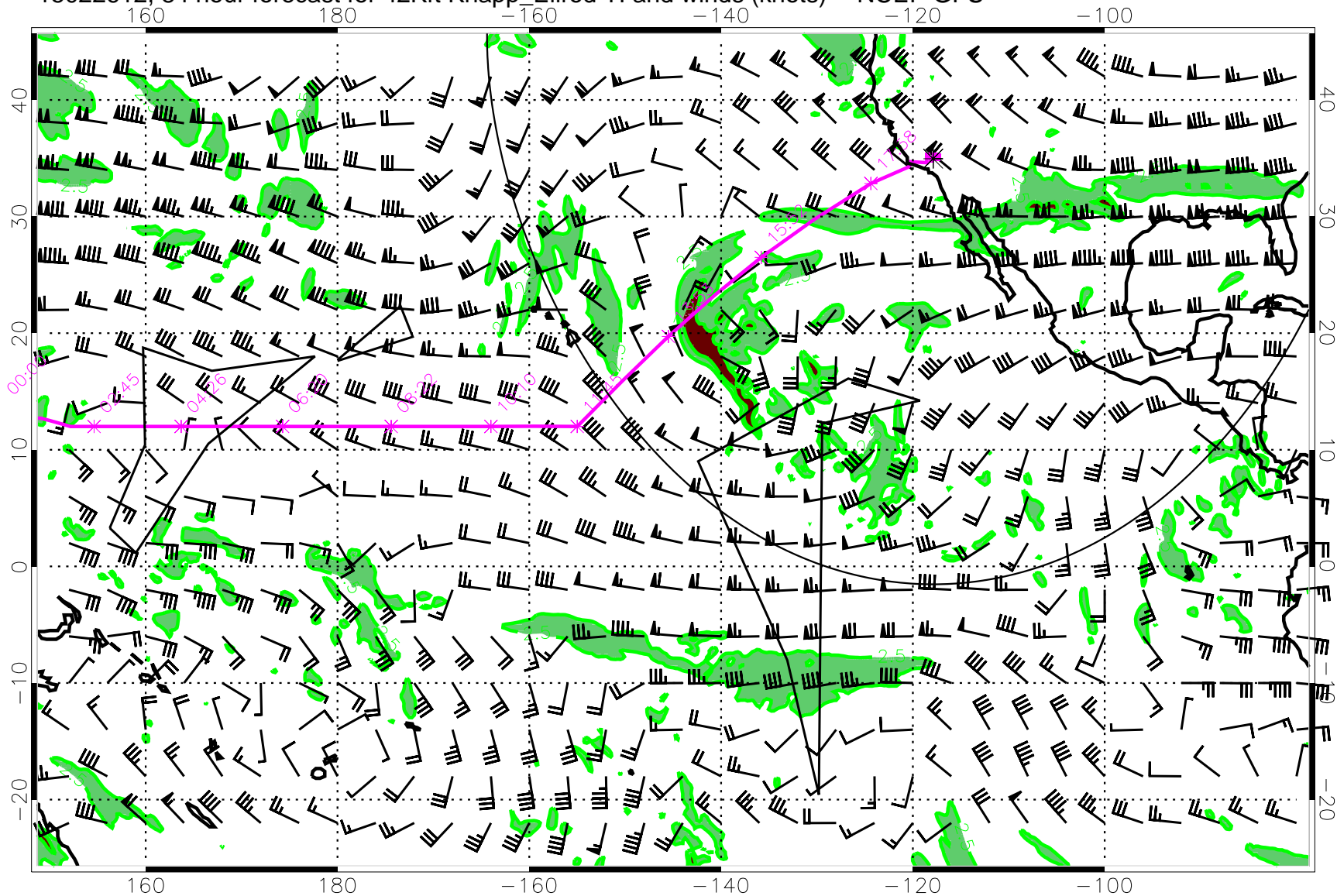
15022612, 84 hour forecast for 42Kft Knapp_Ellrod TI and winds (knots) -- NCEP GFS
