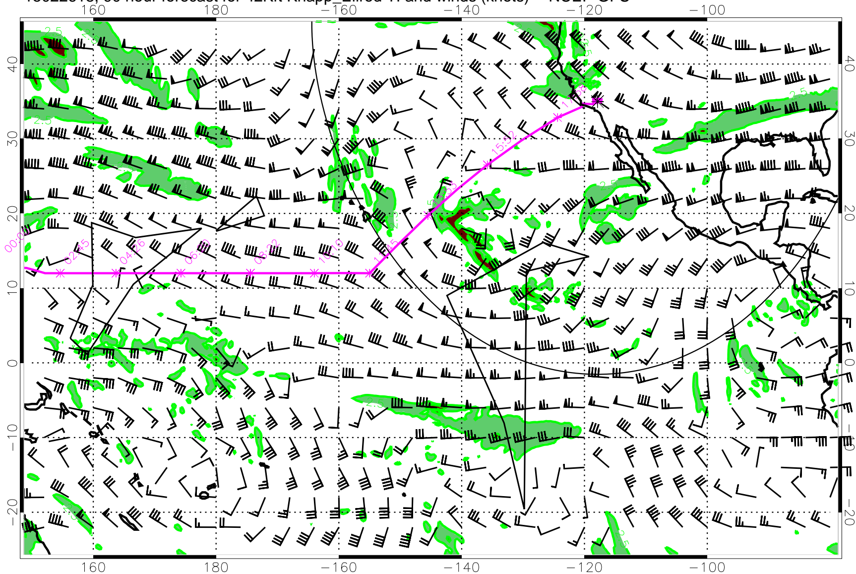
15022618, 90 hour forecast for 42Kft Knapp_Ellrod TI and winds (knots) -- NCEP GFS
