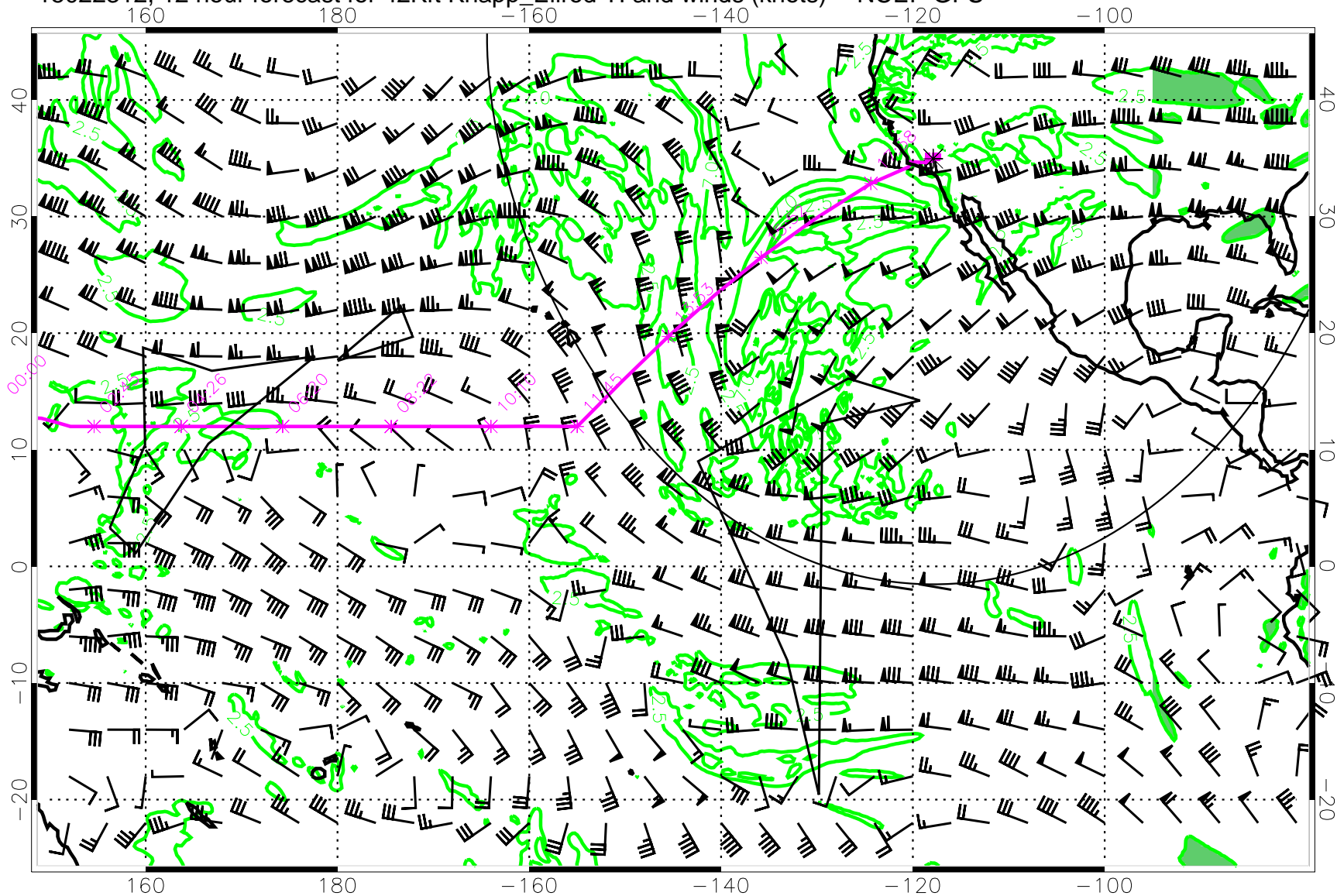
15022312, 12 hour forecast for 42Kft Knapp_Ellrod TI and winds (knots) -- NCEP GFS
