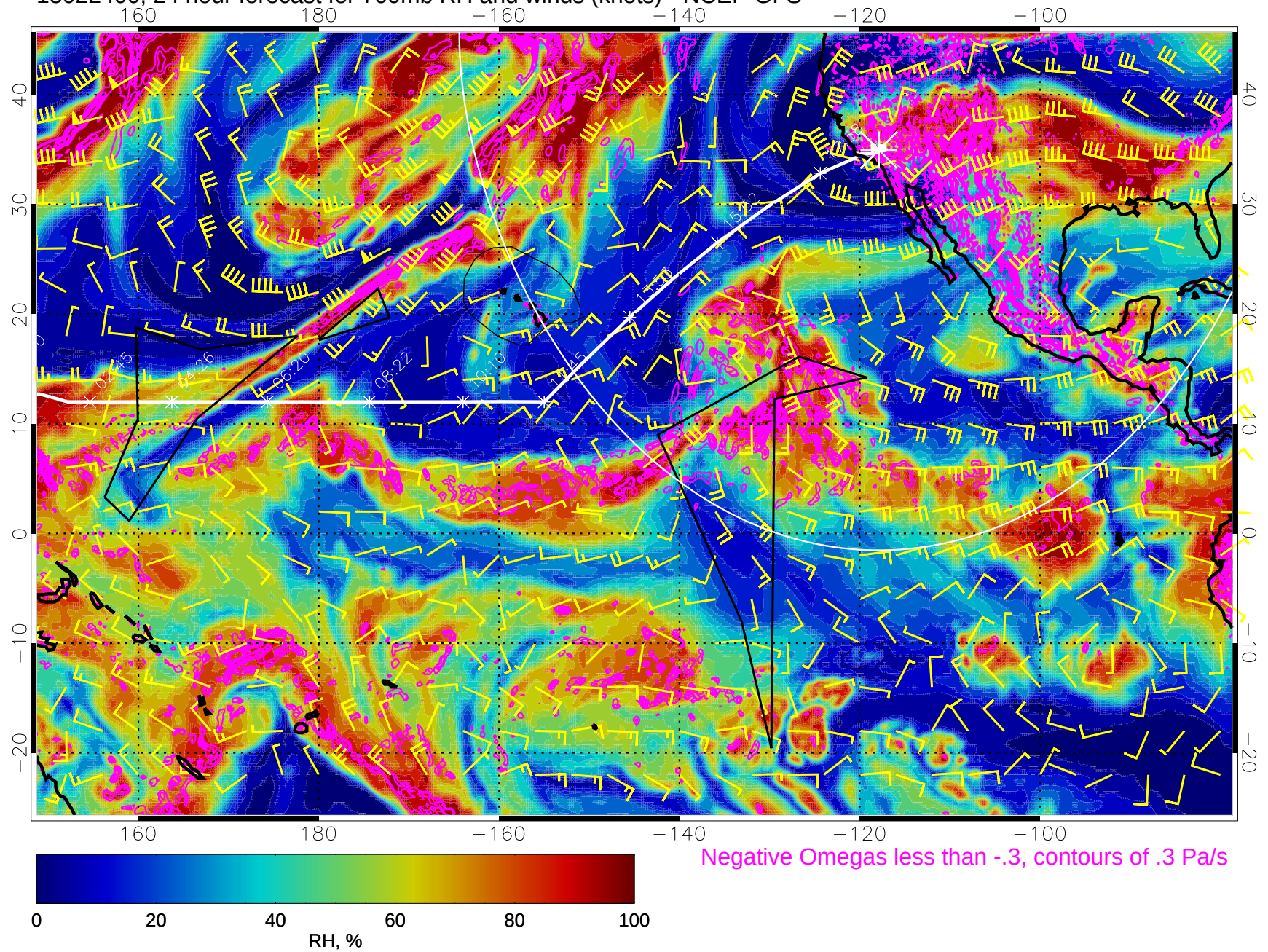
15022400, 24 hour forecast for 700mb RH and winds (knots) - NCEP GFS
