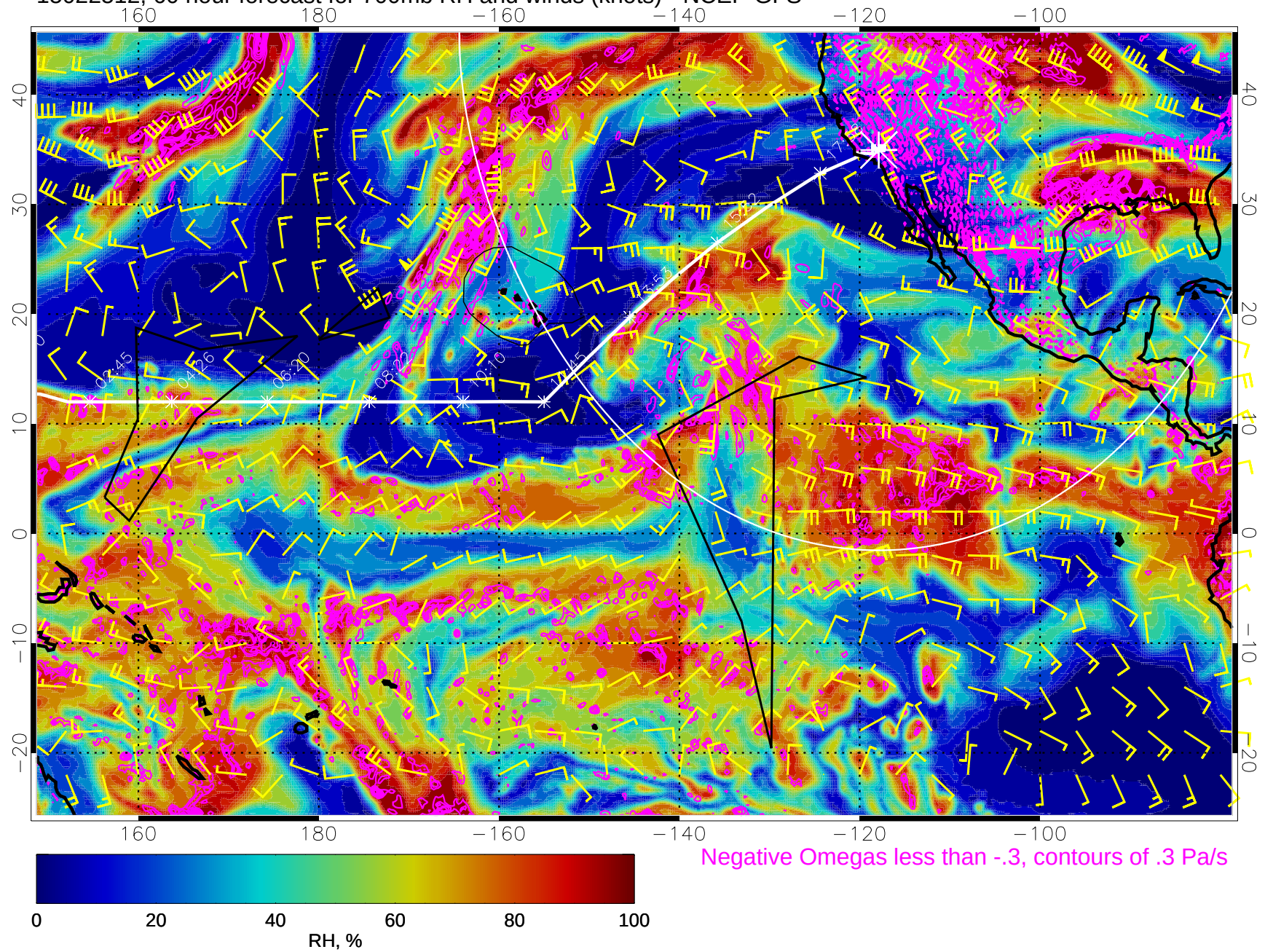
15022512, 60 hour forecast for 700mb RH and winds (knots) - NCEP GFS
