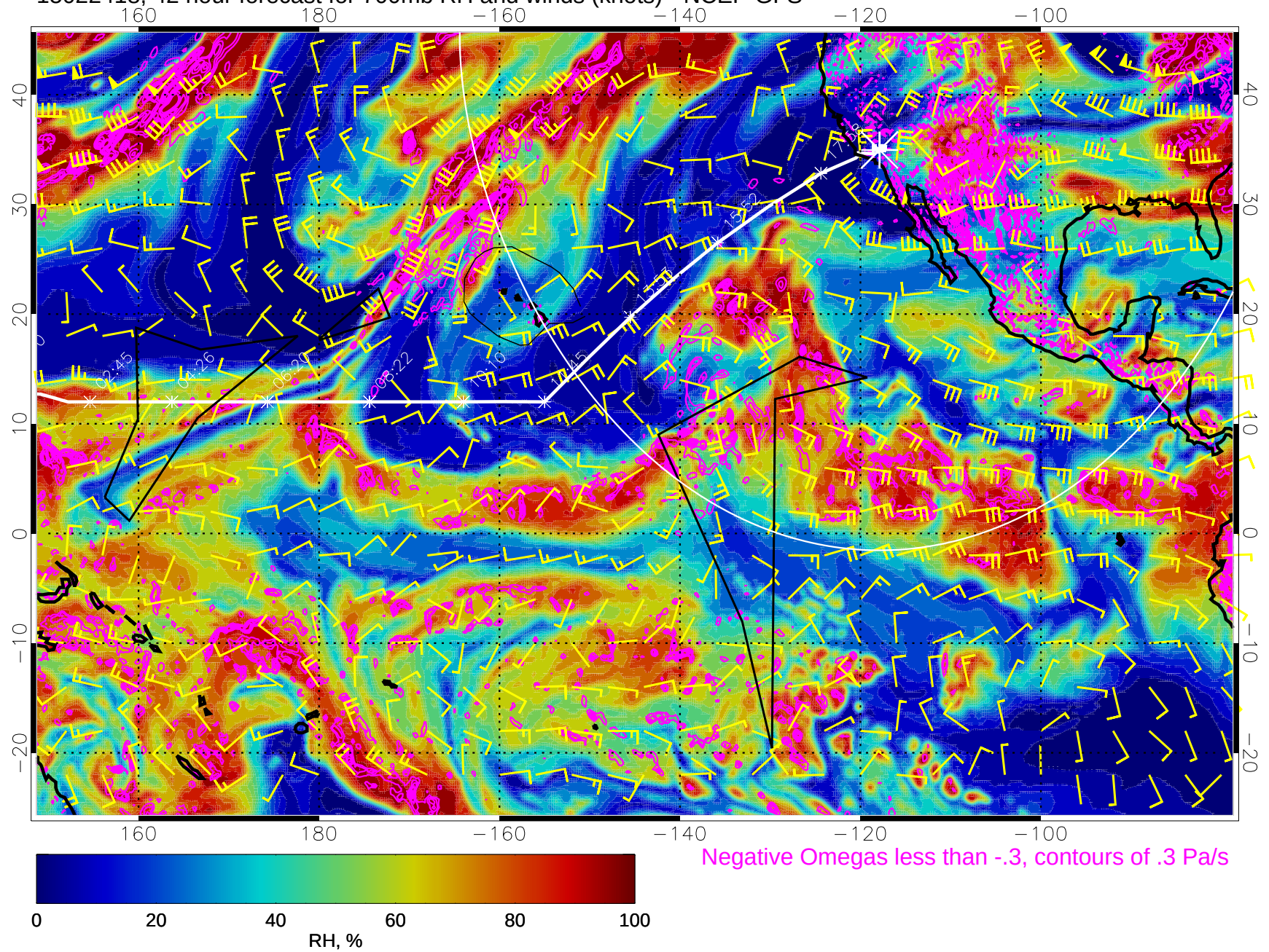
15022418, 42 hour forecast for 700mb RH and winds (knots) - NCEP GFS
