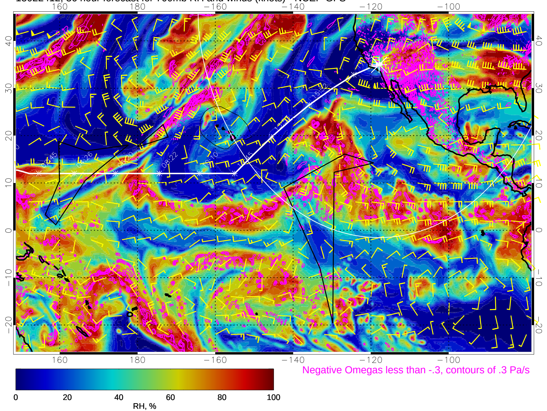
15022412, 36 hour forecast for 700mb RH and winds (knots) - NCEP GFS
