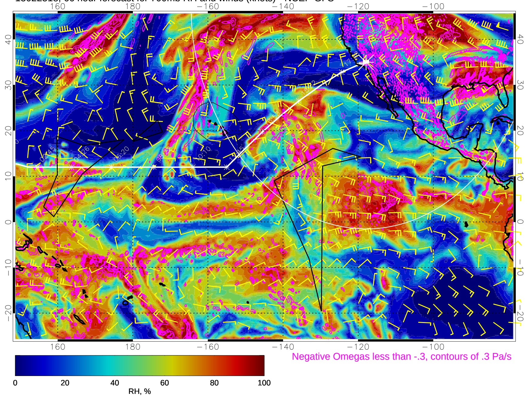
15022518, 66 hour forecast for 700mb RH and winds (knots) - NCEP GFS
