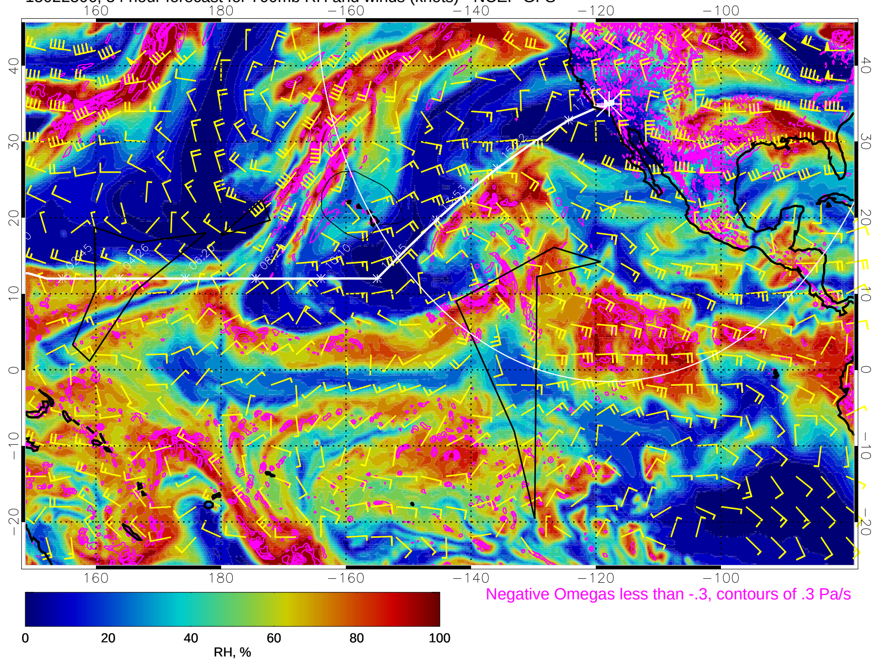
15022506, 54 hour forecast for 700mb RH and winds (knots) - NCEP GFS
