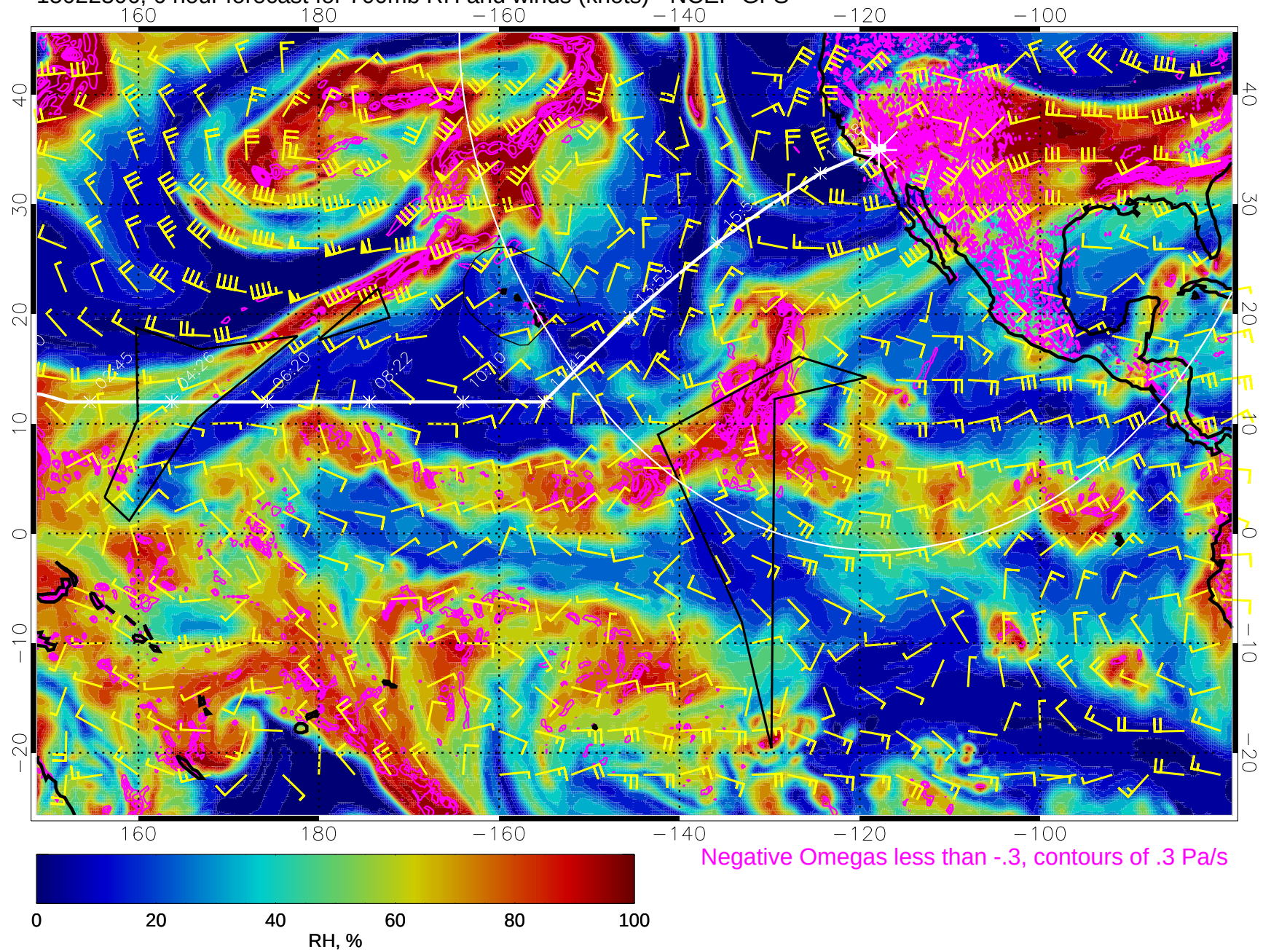
15022306, 6 hour forecast for 700mb RH and winds (knots) - NCEP GFS
