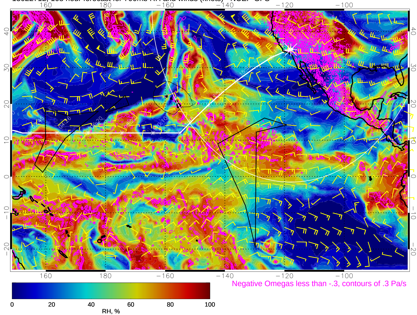
15022712, 108 hour forecast for 700mb RH and winds (knots) - NCEP GFS
