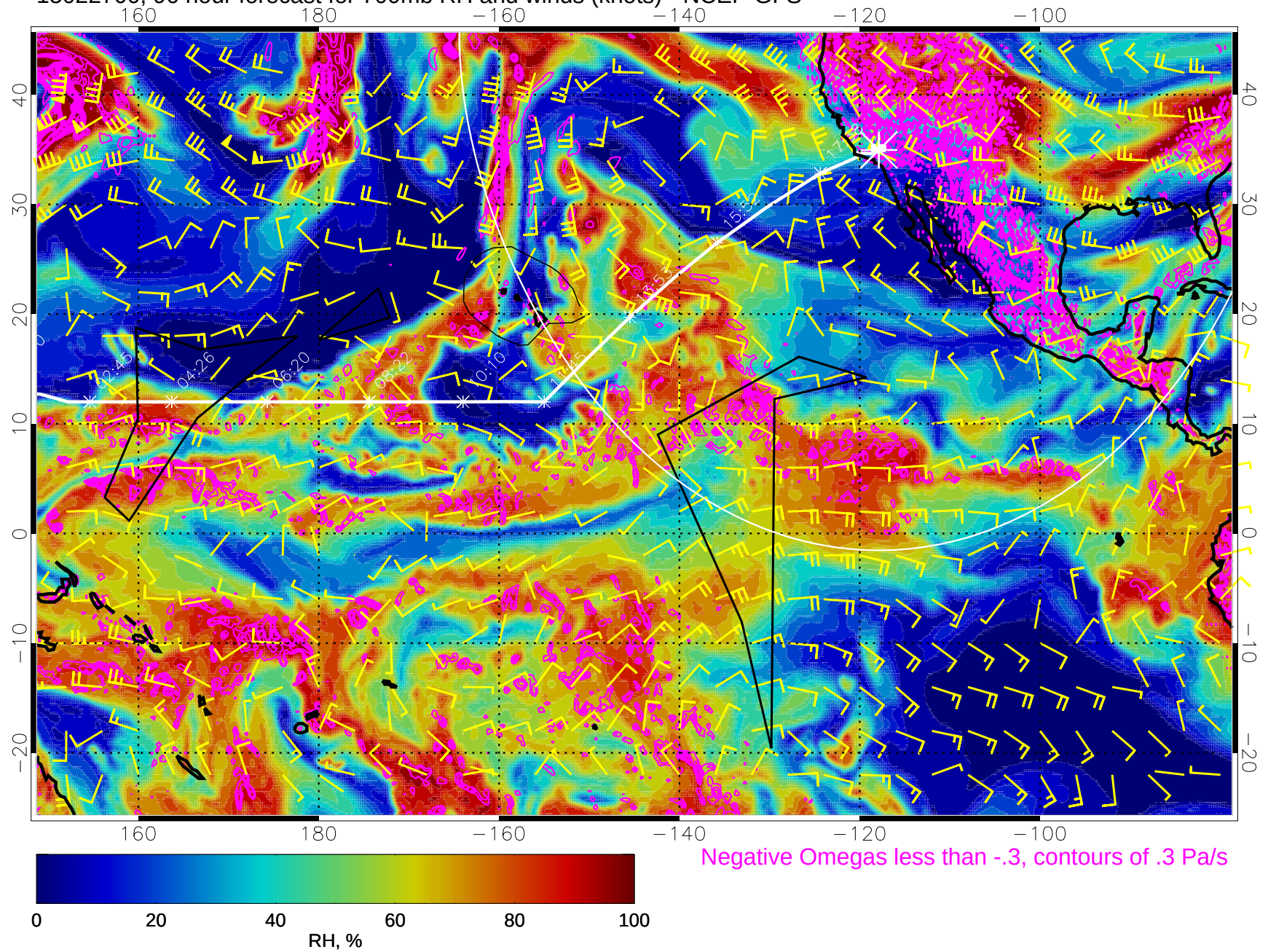
15022700, 96 hour forecast for 700mb RH and winds (knots) - NCEP GFS
