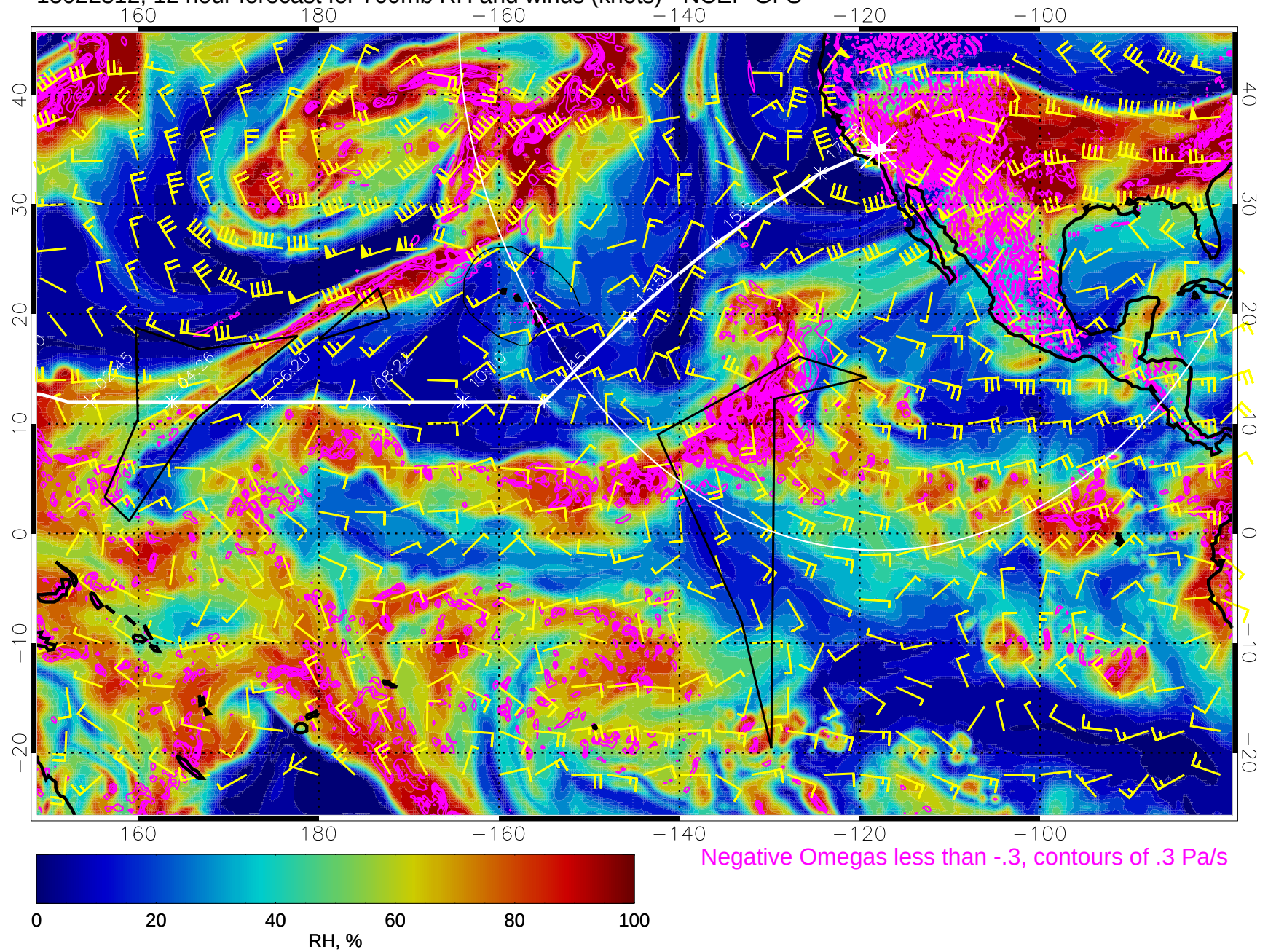
15022312, 12 hour forecast for 700mb RH and winds (knots) - NCEP GFS
