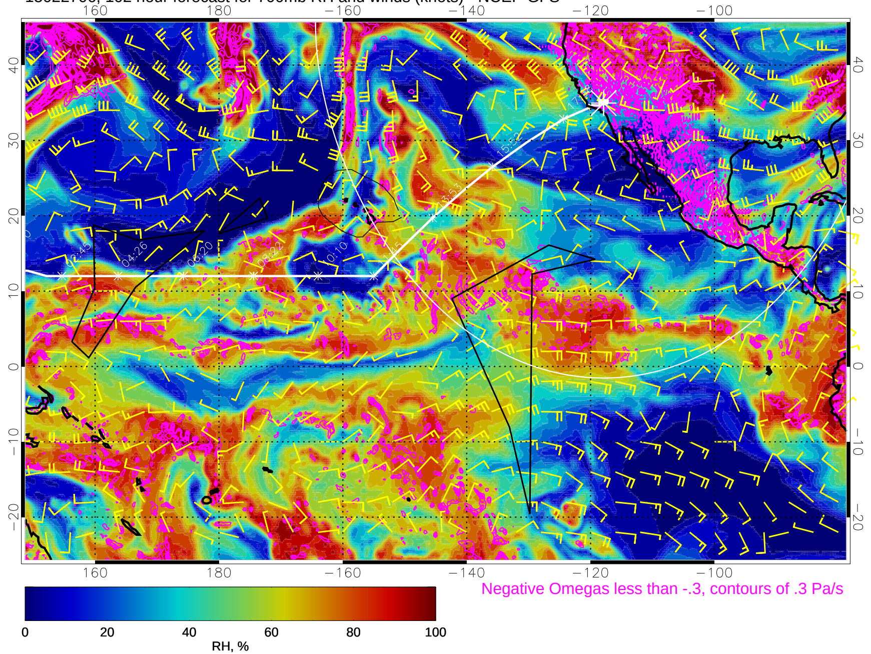
15022706, 102 hour forecast for 700mb RH and winds (knots) - NCEP GFS
