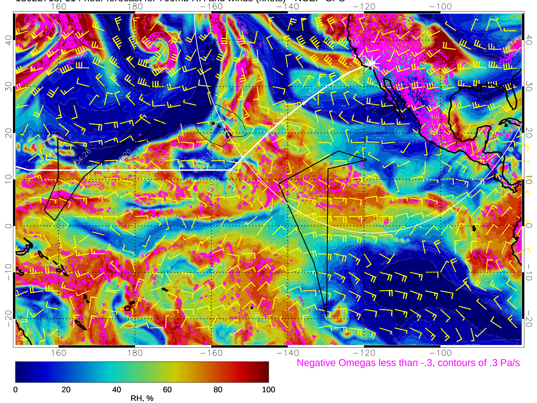
15022718, 114 hour forecast for 700mb RH and winds (knots) - NCEP GFS
