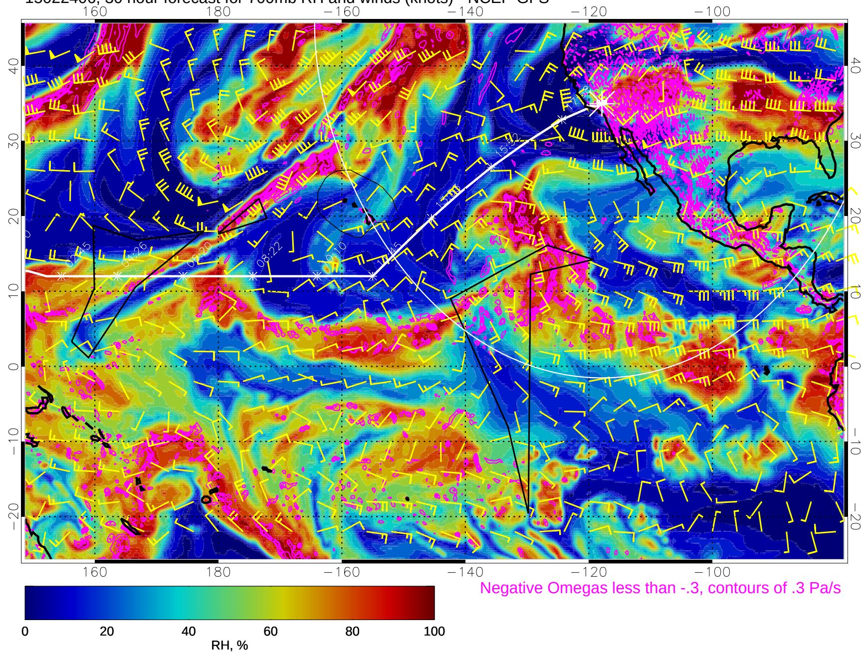
15022406, 30 hour forecast for 700mb RH and winds (knots) - NCEP GFS
