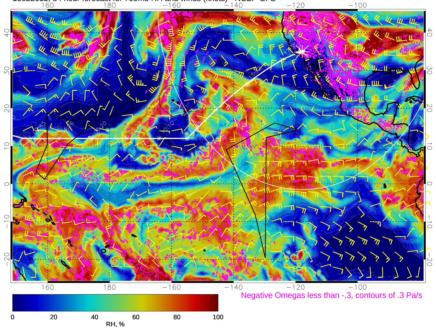
15022612, 84 hour forecast for 700mb RH and winds (knots) - NCEP GFS
