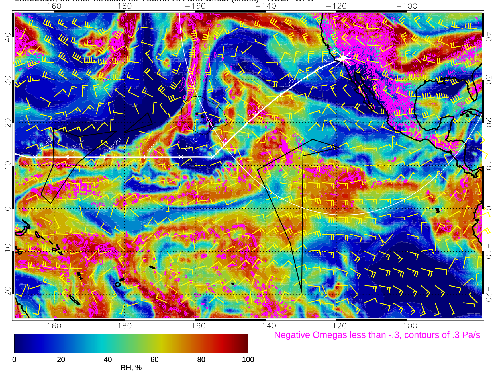
15022618, 90 hour forecast for 700mb RH and winds (knots) - NCEP GFS
