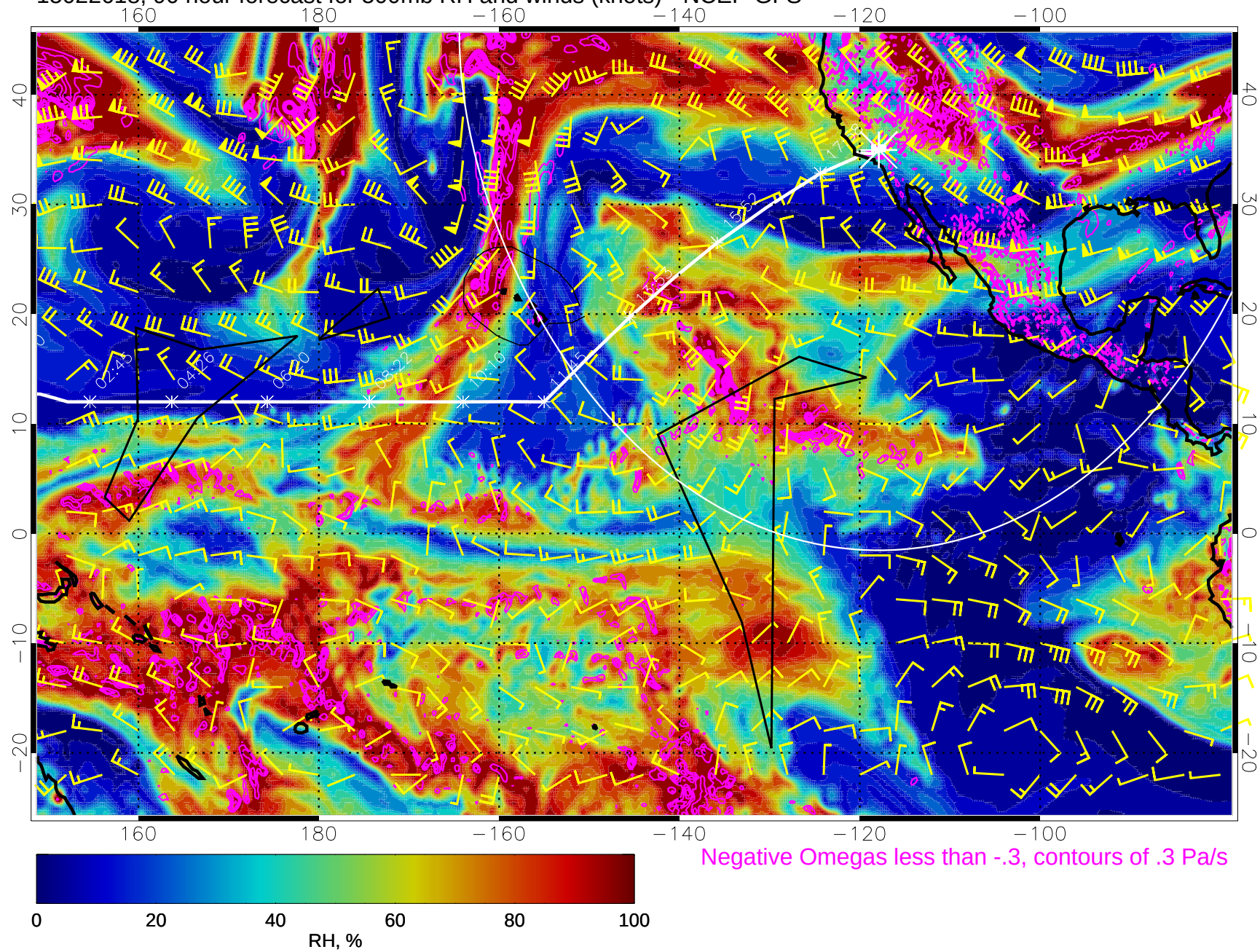
15022618, 90 hour forecast for 500mb RH and winds (knots) - NCEP GFS
