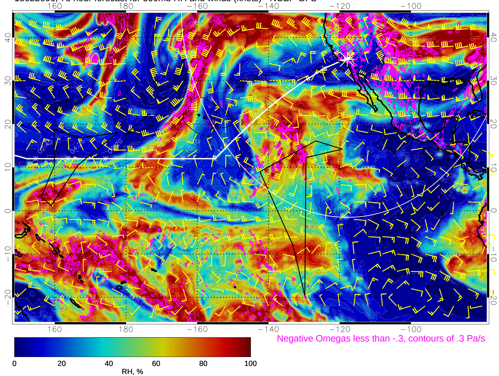
15022606, 78 hour forecast for 500mb RH and winds (knots) - NCEP GFS
