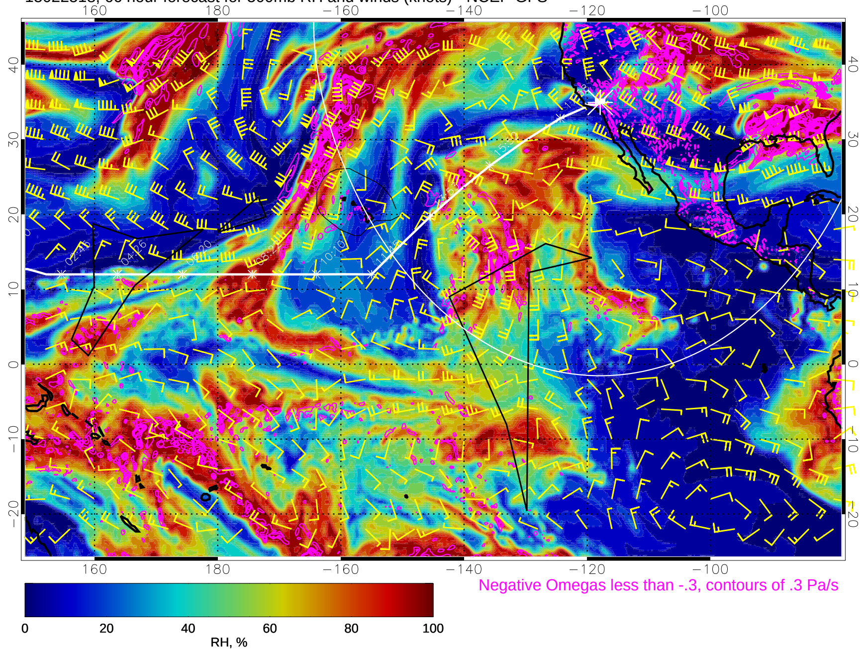
15022518, 66 hour forecast for 500mb RH and winds (knots) - NCEP GFS
