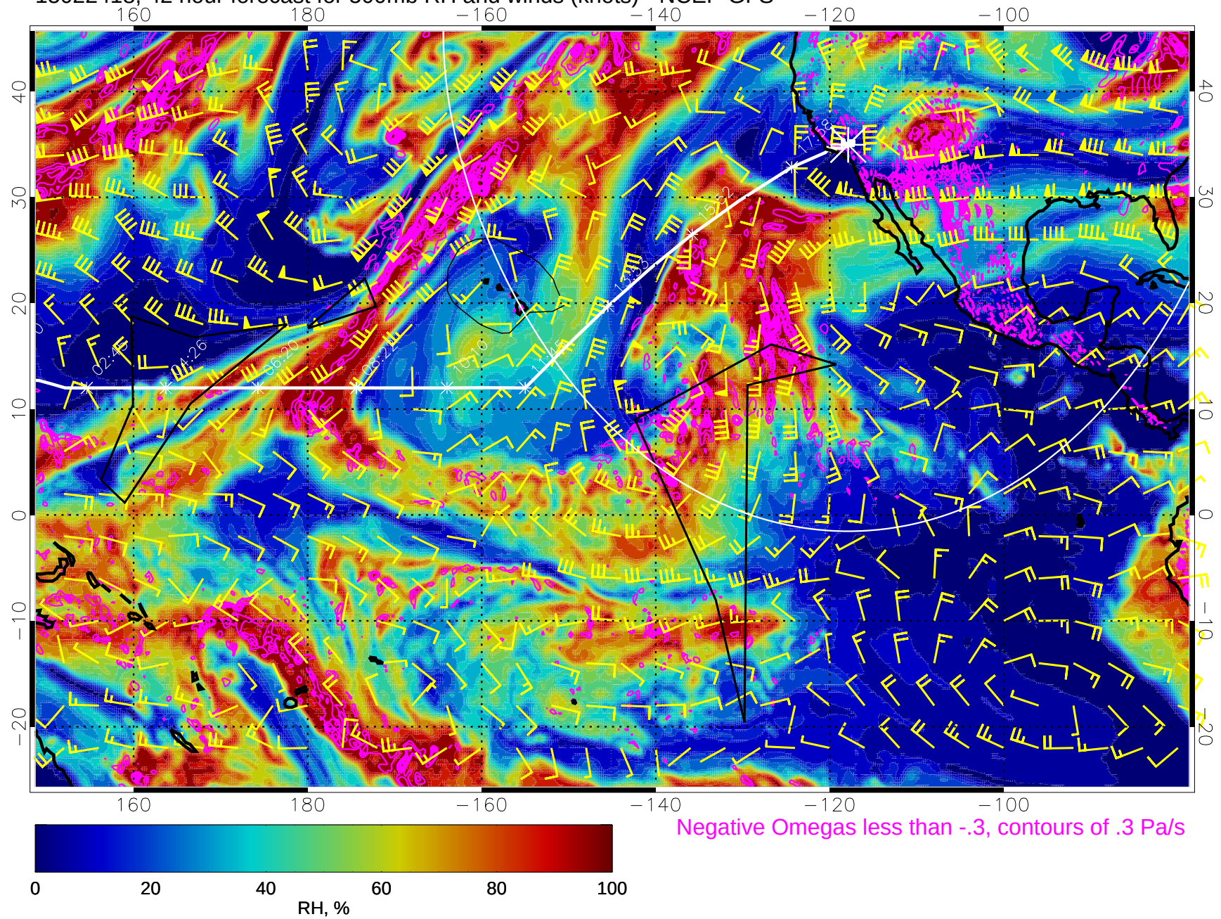
15022418, 42 hour forecast for 500mb RH and winds (knots) - NCEP GFS
