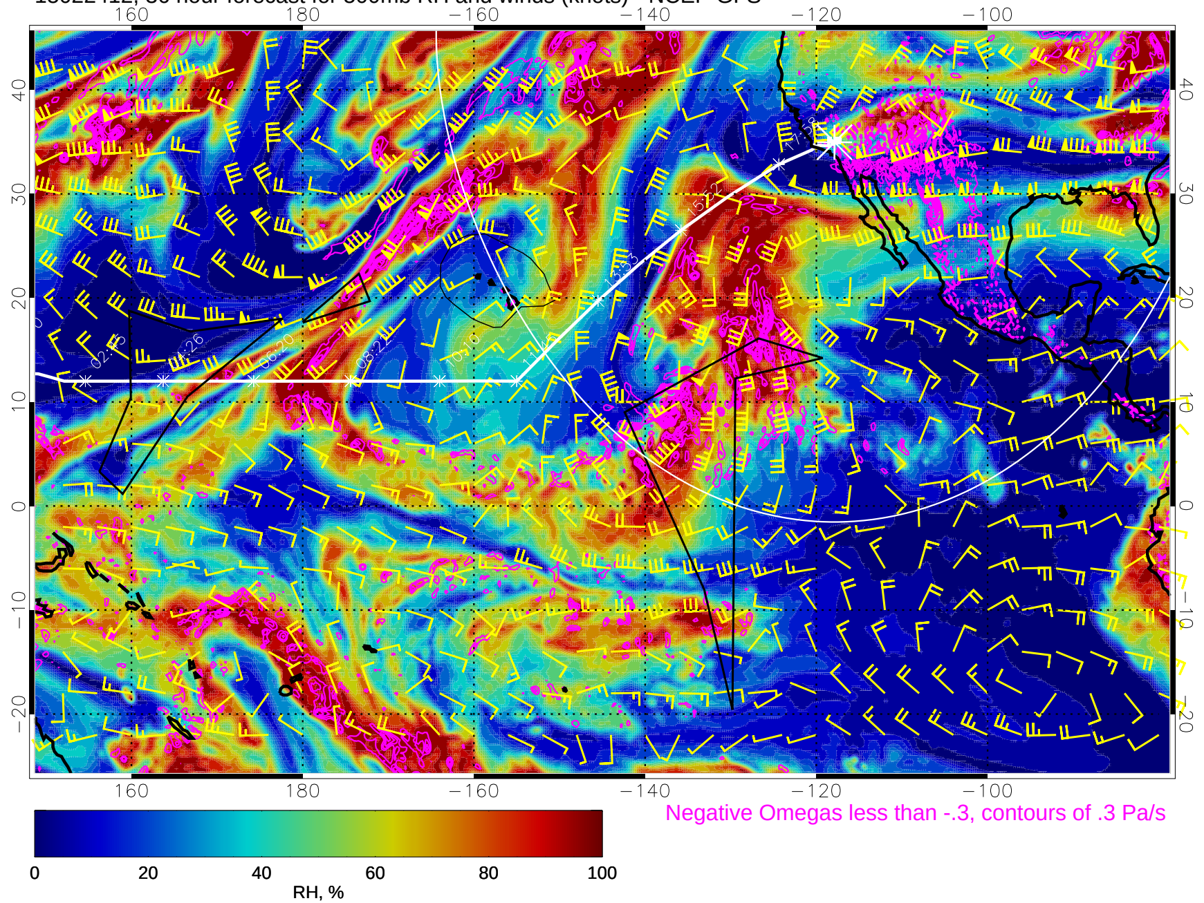
15022412, 36 hour forecast for 500mb RH and winds (knots) - NCEP GFS
