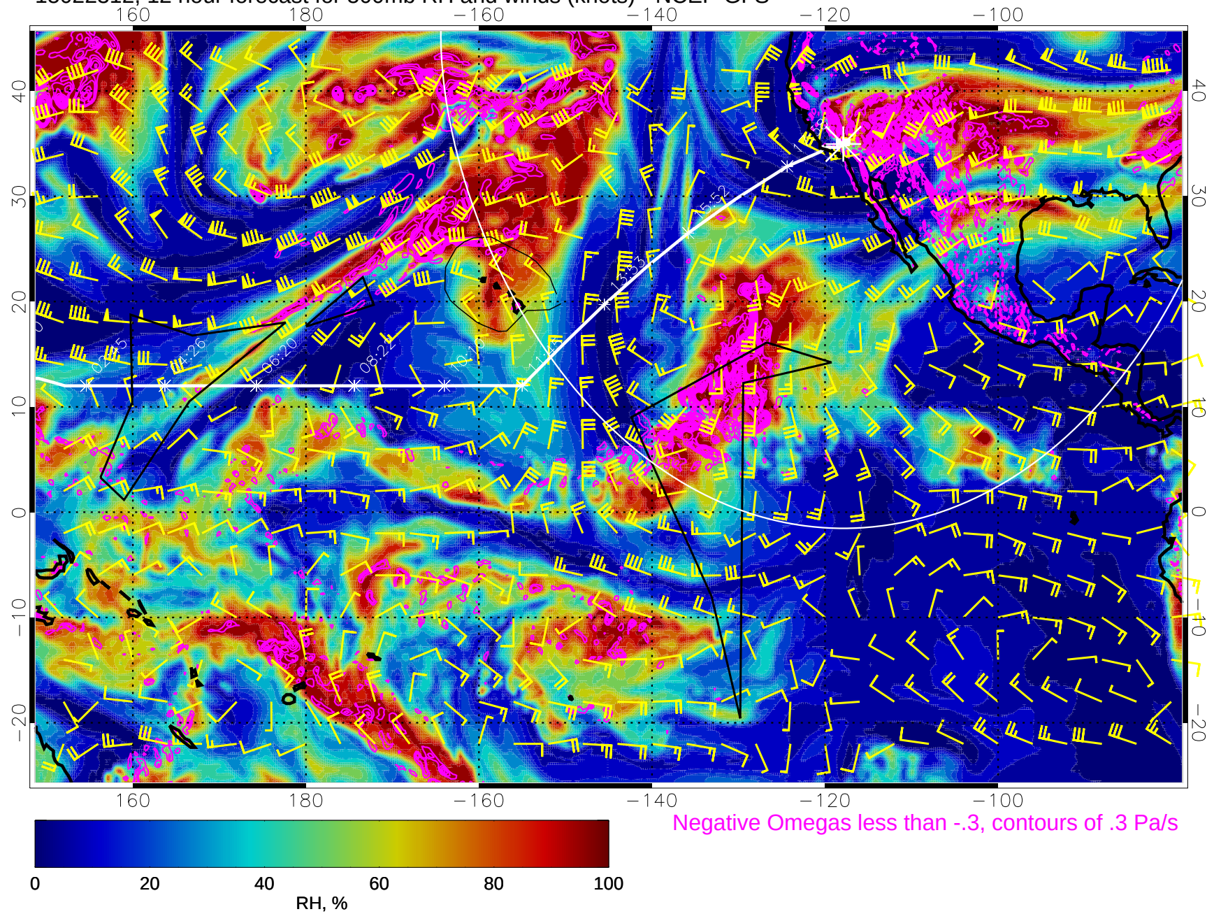
15022312, 12 hour forecast for 500mb RH and winds (knots) - NCEP GFS
