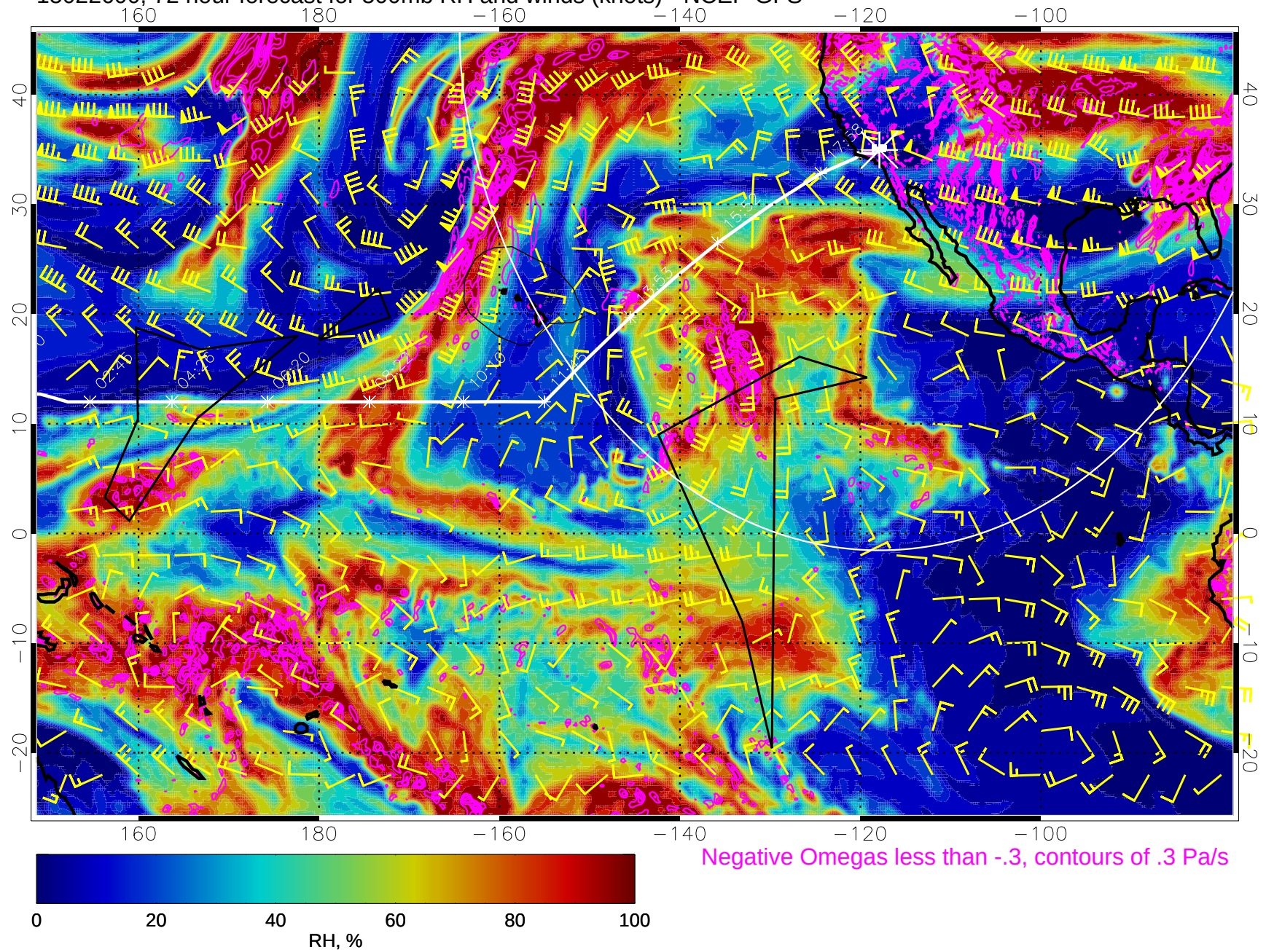
15022600, 72 hour forecast for 500mb RH and winds (knots) - NCEP GFS
