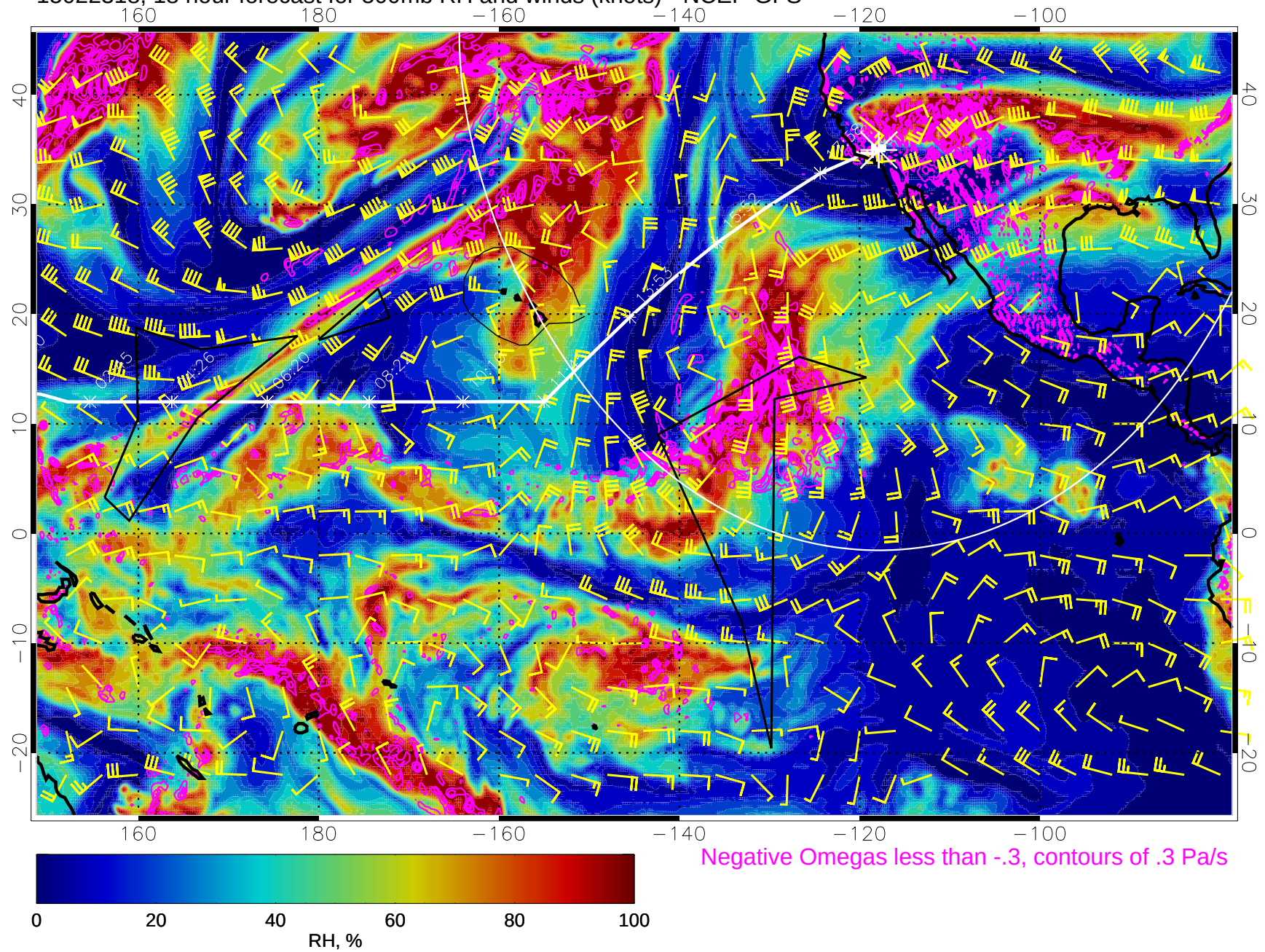
15022318, 18 hour forecast for 500mb RH and winds (knots) - NCEP GFS
