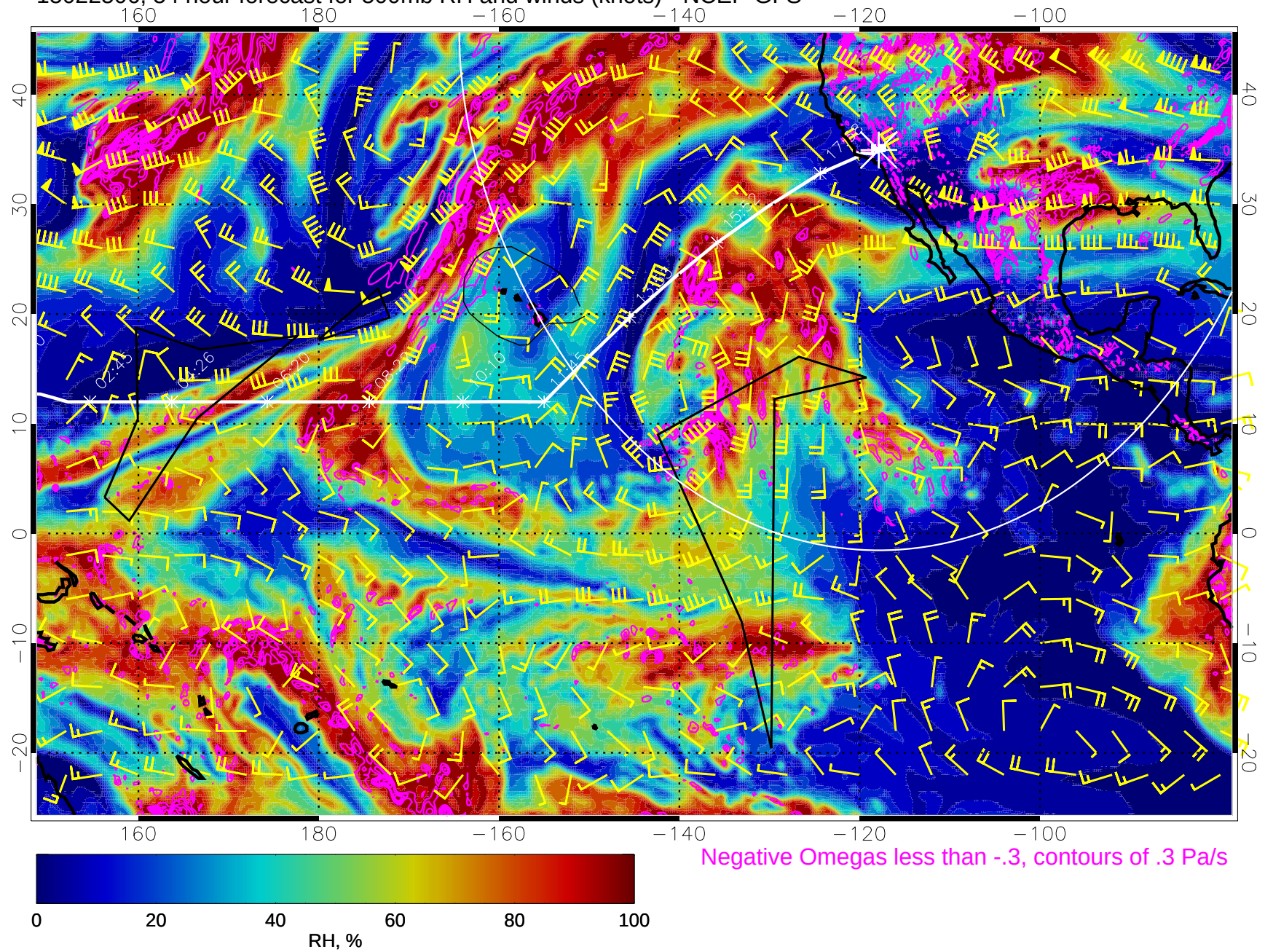
15022506, 54 hour forecast for 500mb RH and winds (knots) - NCEP GFS
