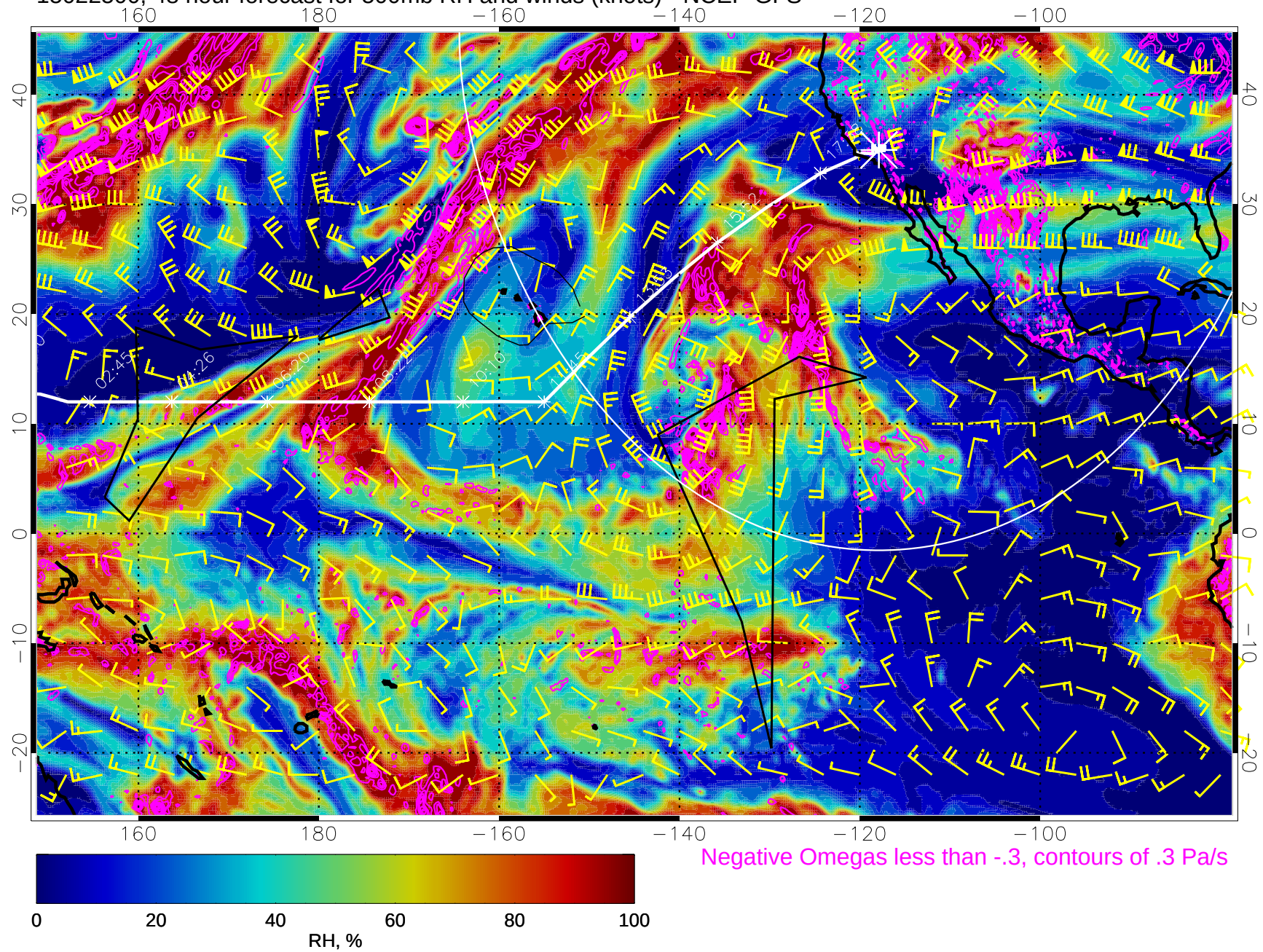
15022500, 48 hour forecast for 500mb RH and winds (knots) - NCEP GFS
