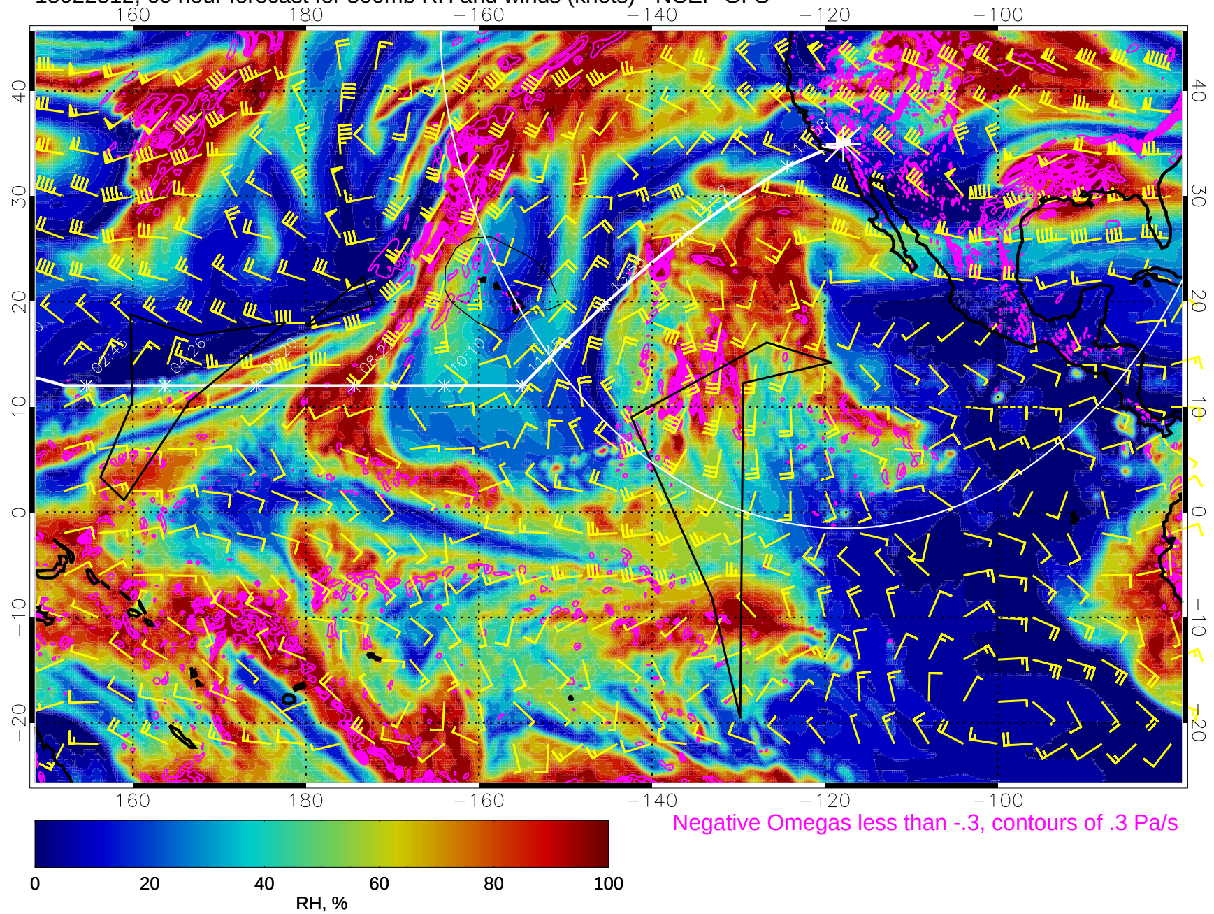
15022512, 60 hour forecast for 500mb RH and winds (knots) - NCEP GFS
