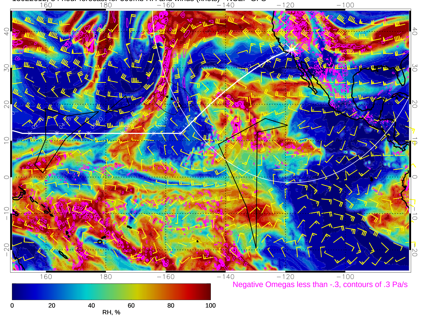
15022612, 84 hour forecast for 500mb RH and winds (knots) - NCEP GFS
