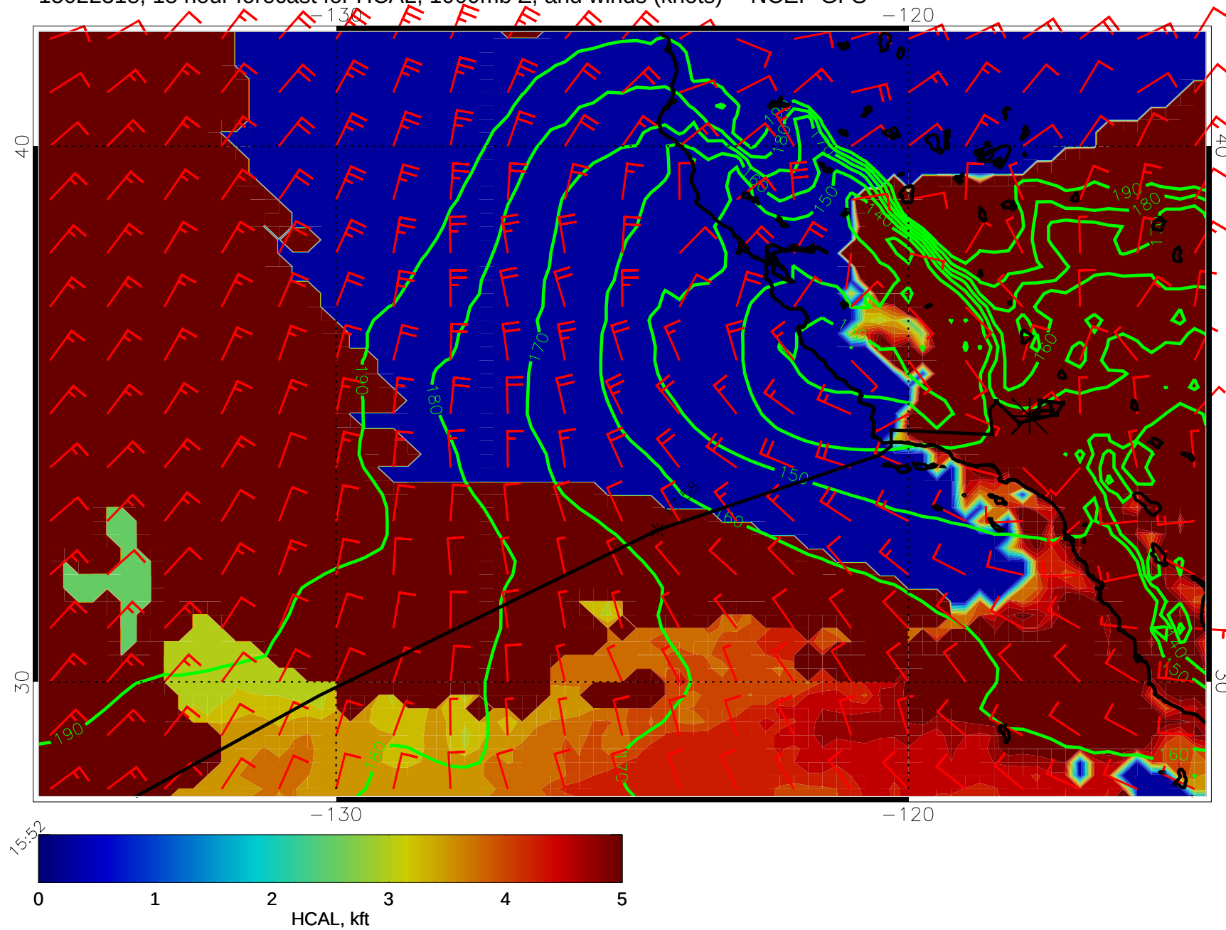
15022318, 18 hour forecast for HCAL, 1000mb Z, and winds (knots) -- NCEP GFS
