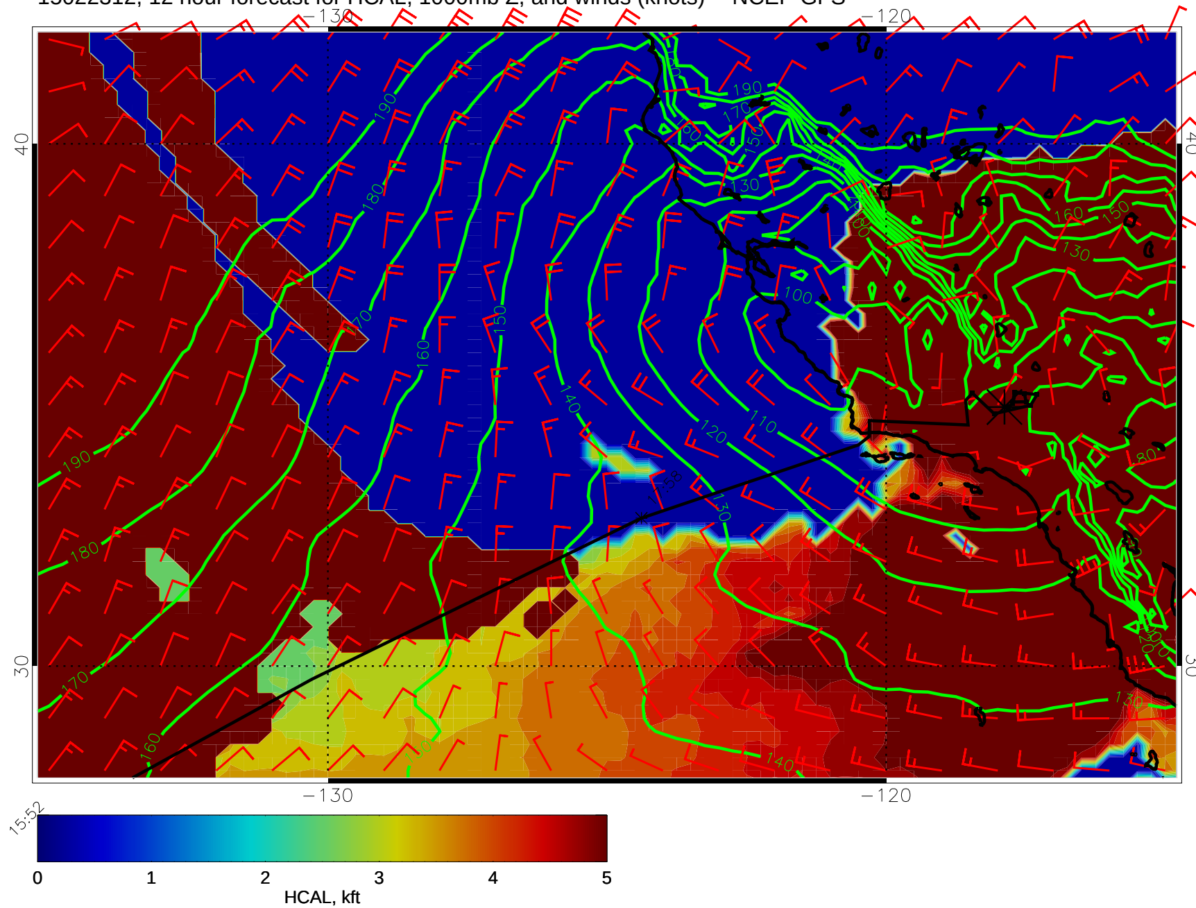
15022312, 12 hour forecast for HCAL, 1000mb Z, and winds (knots) -- NCEP GFS
