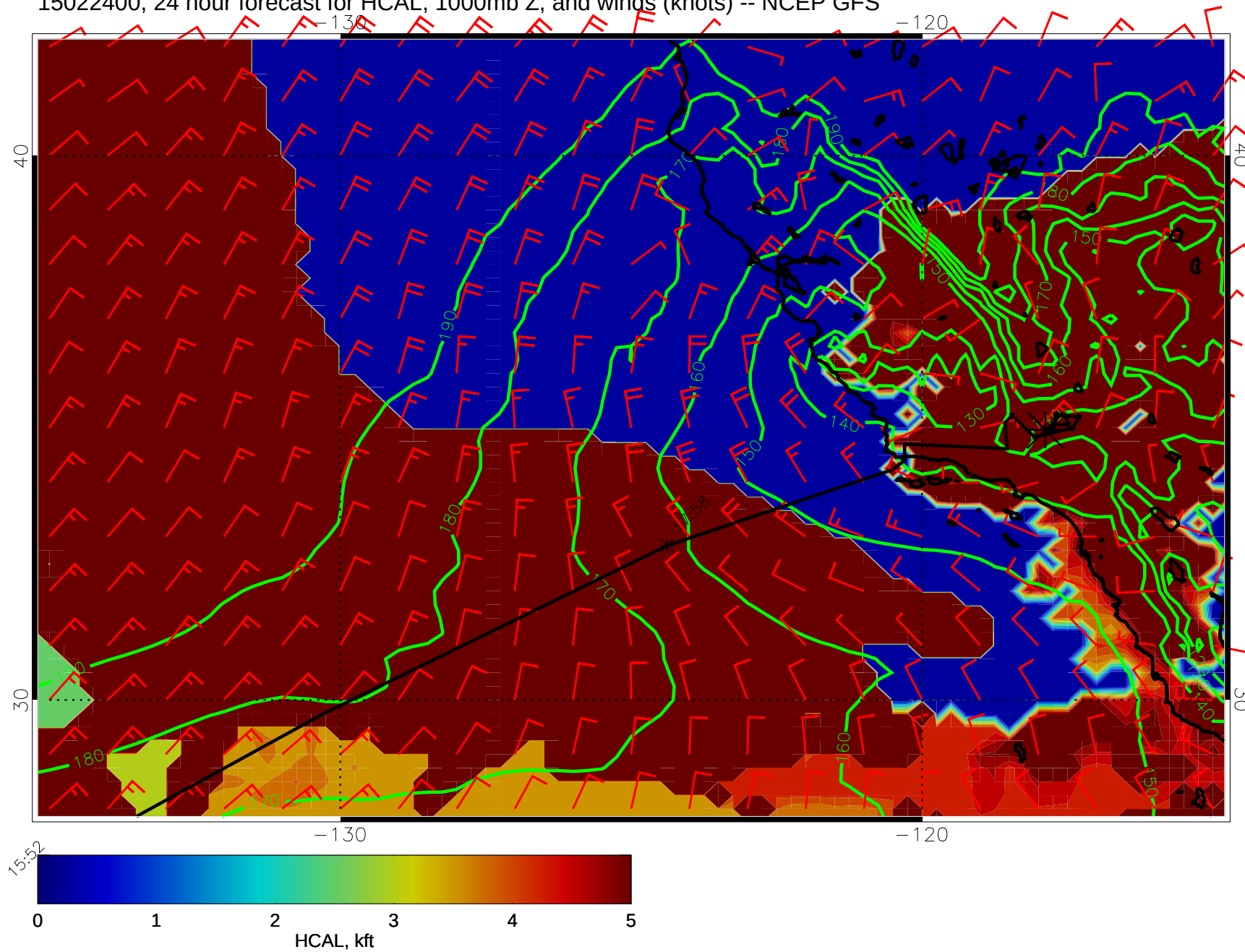
15022400, 24 hour forecast for HCAL, 1000mb Z, and winds (knots) -- NCEP GFS
