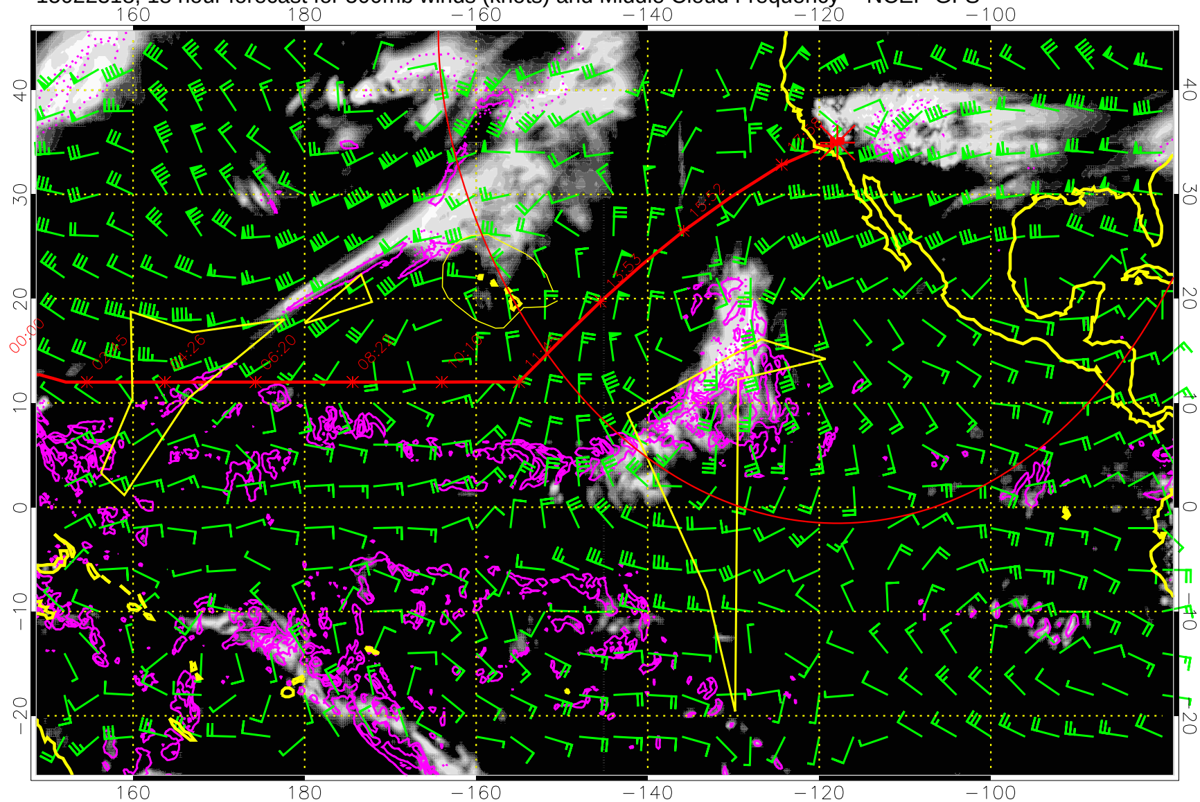
15022318, 18 hour forecast for 500mb winds (knots) and Middle Cloud Frequency -- NCEP GFS
