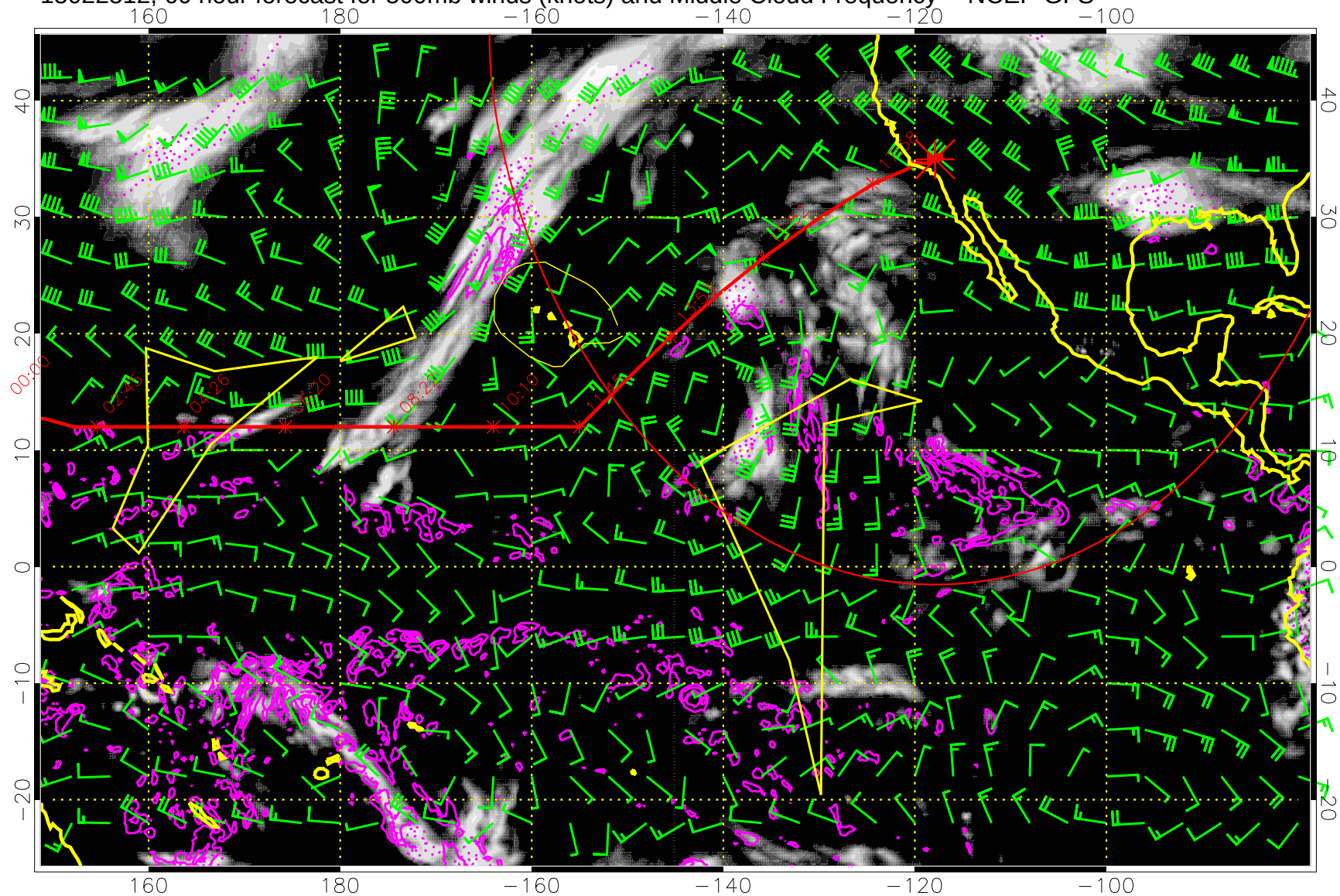
15022512, 60 hour forecast for 500mb winds (knots) and Middle Cloud Frequency -- NCEP GFS
