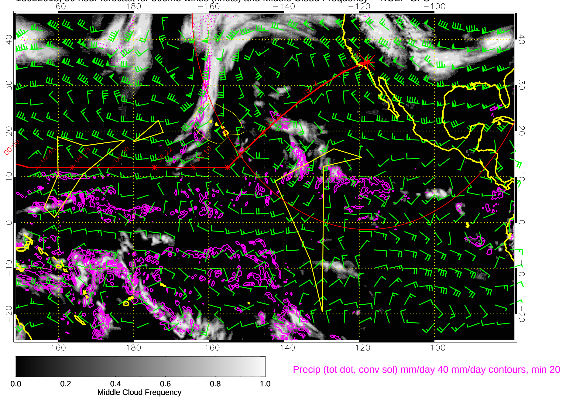
15022618, 90 hour forecast for 500mb winds (knots) and Middle Cloud Frequency -- NCEP GFS
