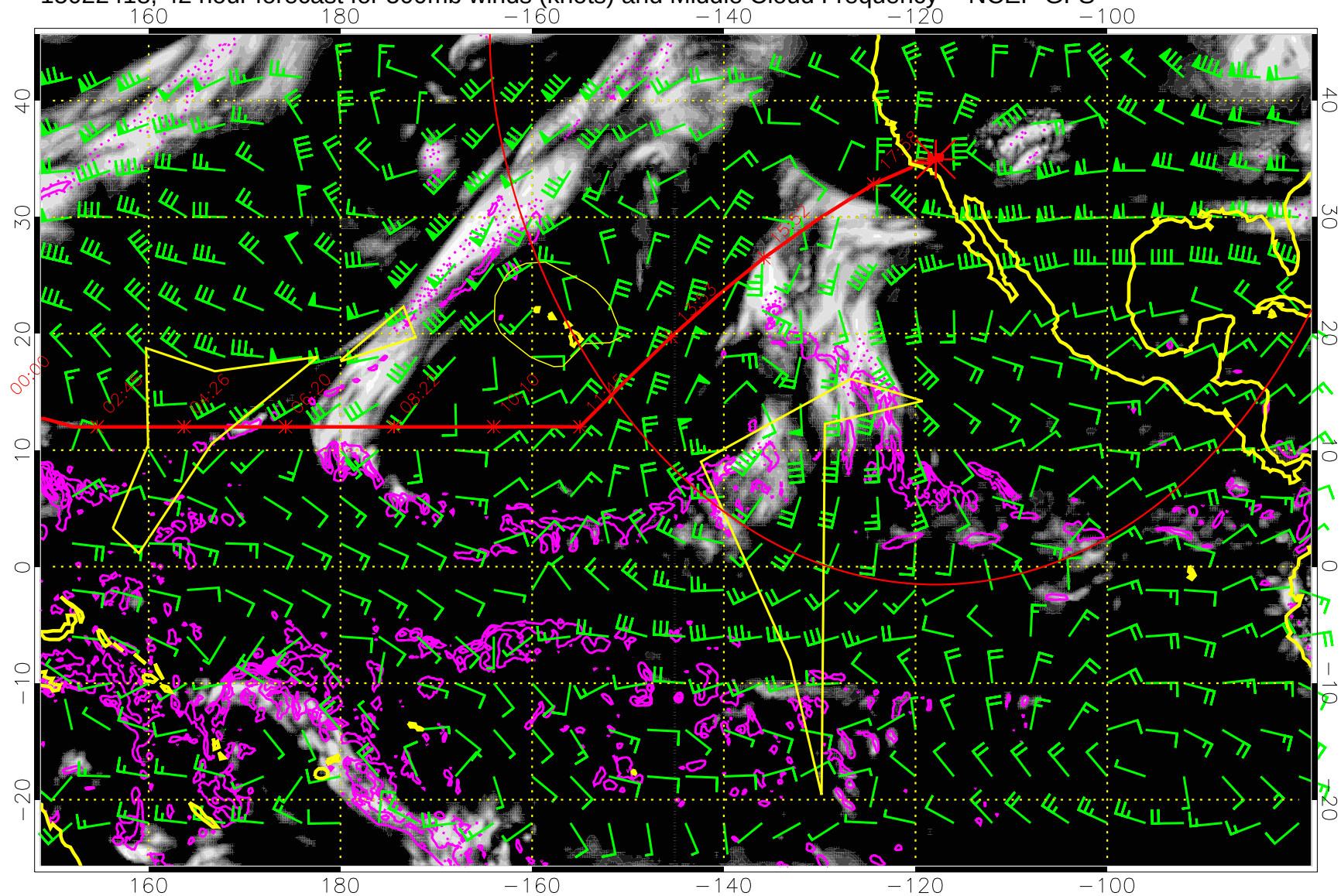
15022418, 42 hour forecast for 500mb winds (knots) and Middle Cloud Frequency -- NCEP GFS
