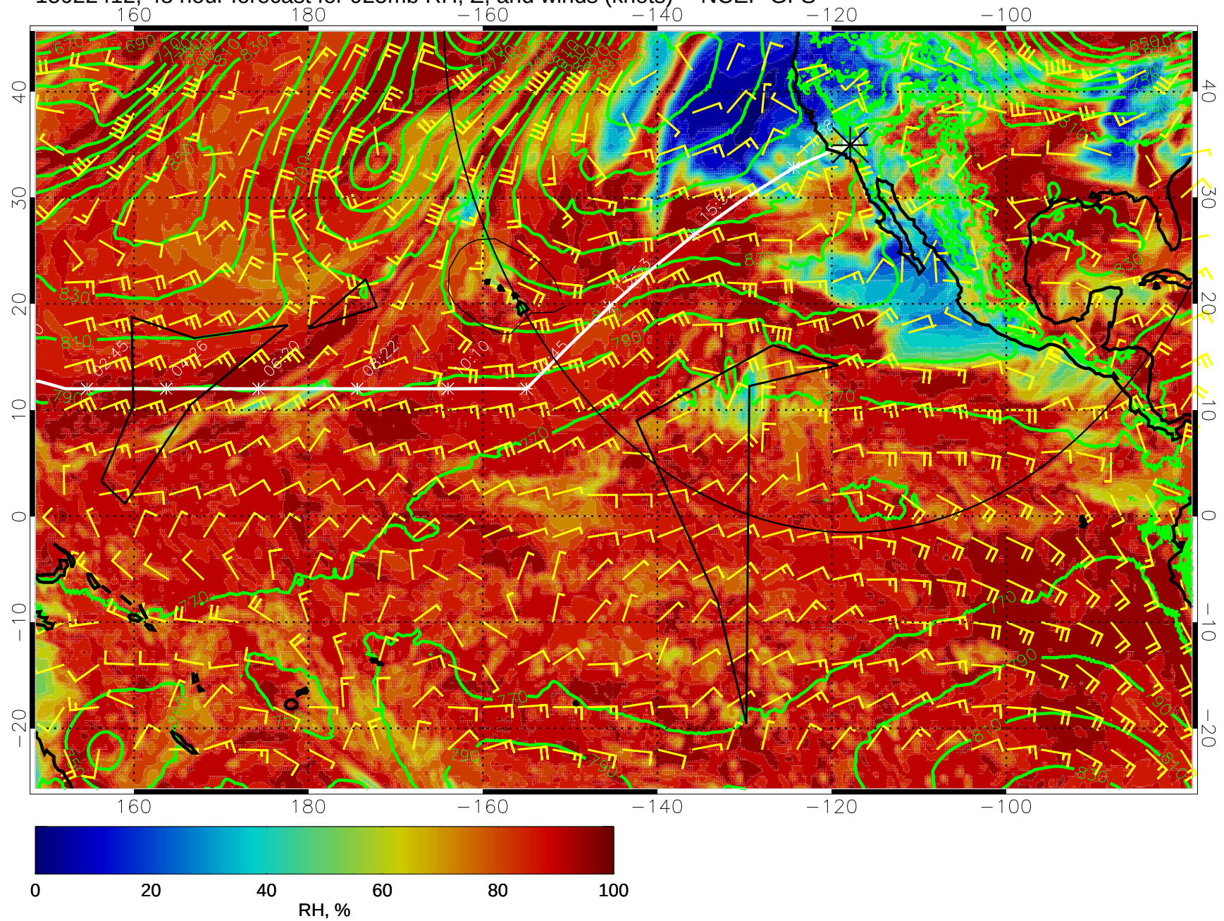
15022412, 48 hour forecast for 925mb RH, Z, and winds (knots) -- NCEP GFS
