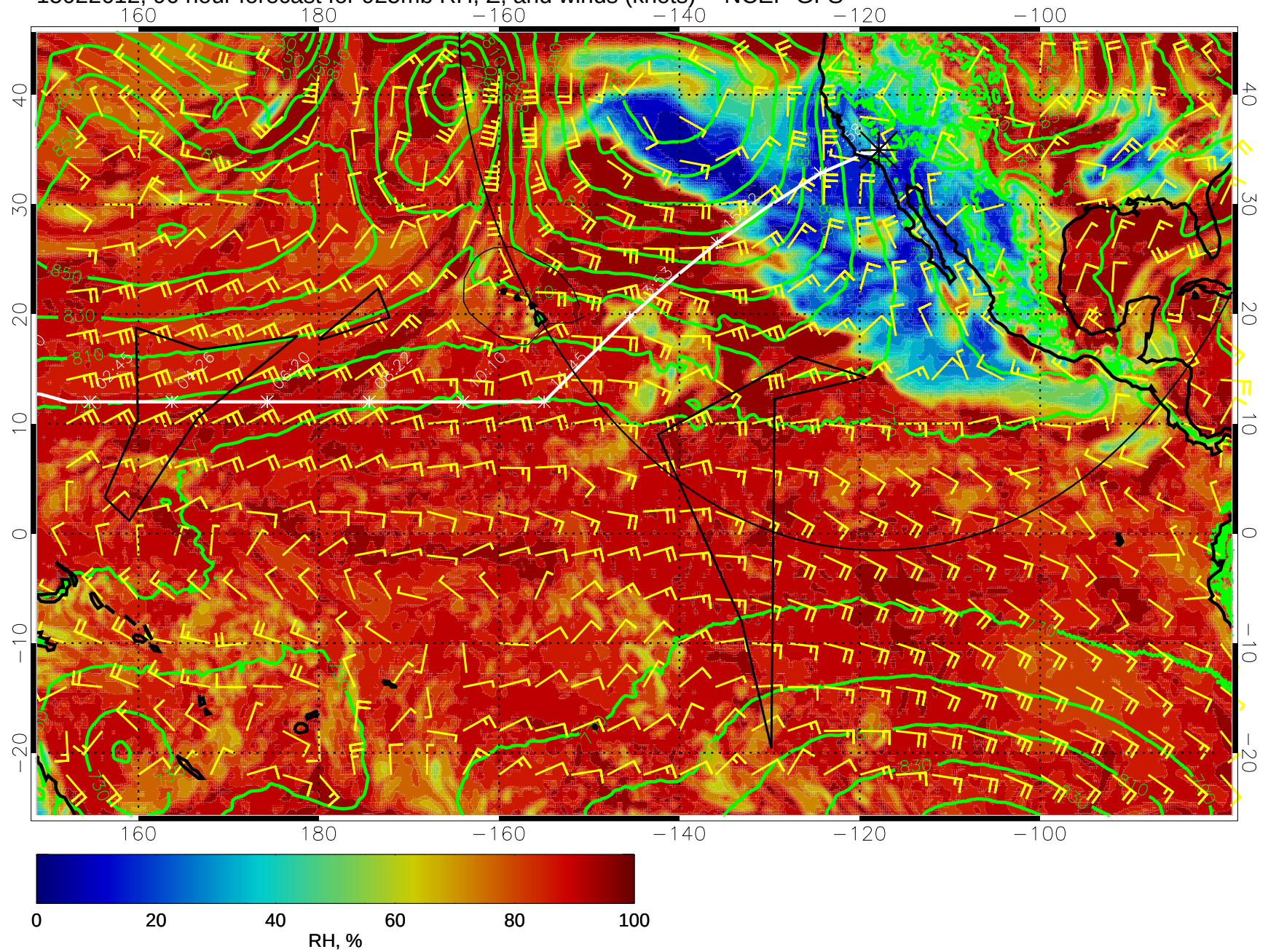
15022612, 96 hour forecast for 925mb RH, Z, and winds (knots) -- NCEP GFS
