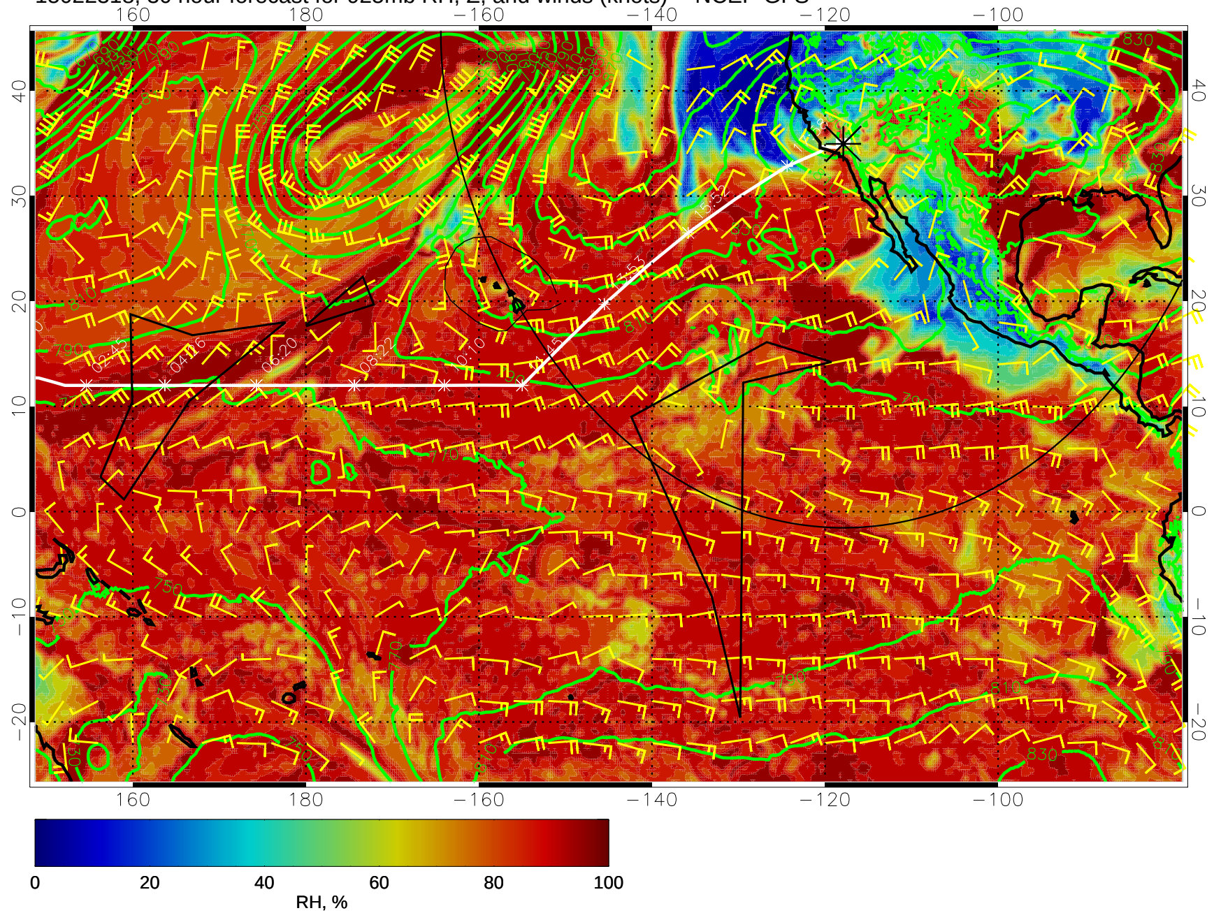
15022318, 30 hour forecast for 925mb RH, Z, and winds (knots) -- NCEP GFS
