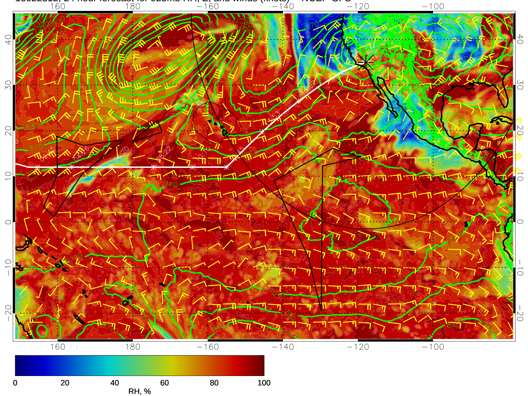
15022312, 24 hour forecast for 925mb RH, Z, and winds (knots) -- NCEP GFS
