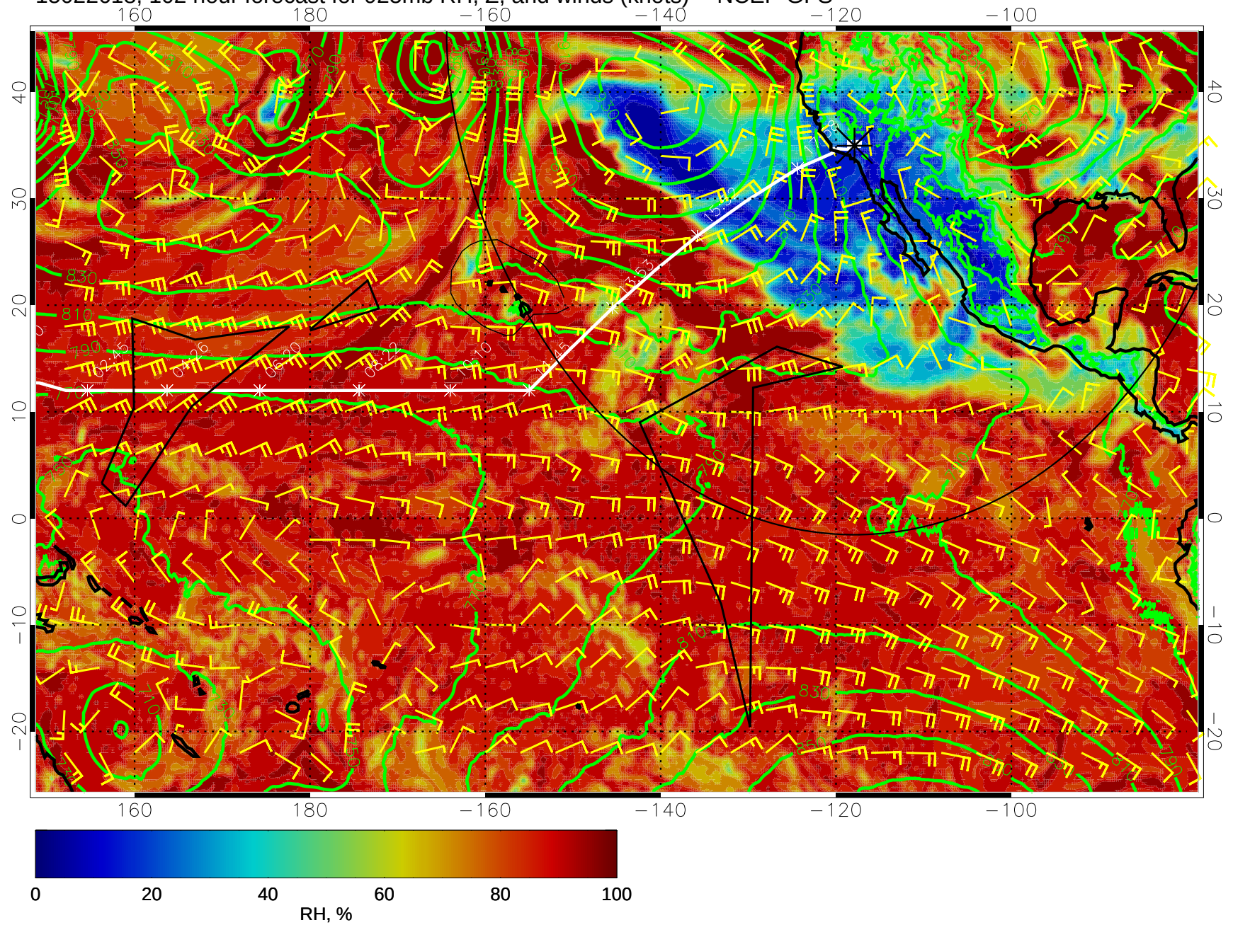
15022618, 102 hour forecast for 925mb RH, Z, and winds (knots) -- NCEP GFS
