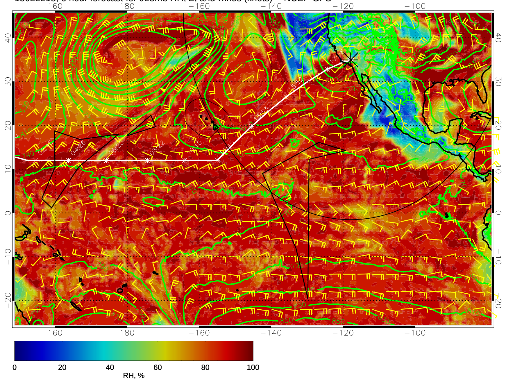
15022218, 6 hour forecast for 925mb RH, Z, and winds (knots) -- NCEP GFS
