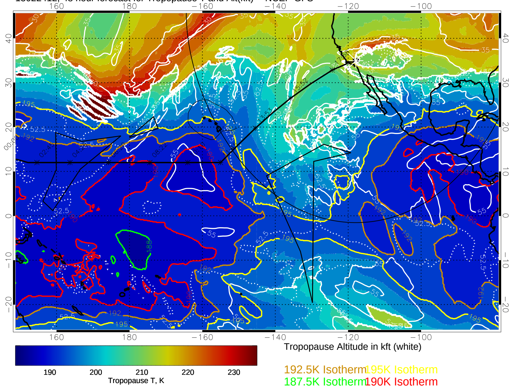
15022412, 48 hour forecast for Tropopause T and Alt(kft) -- NCEP GFS
