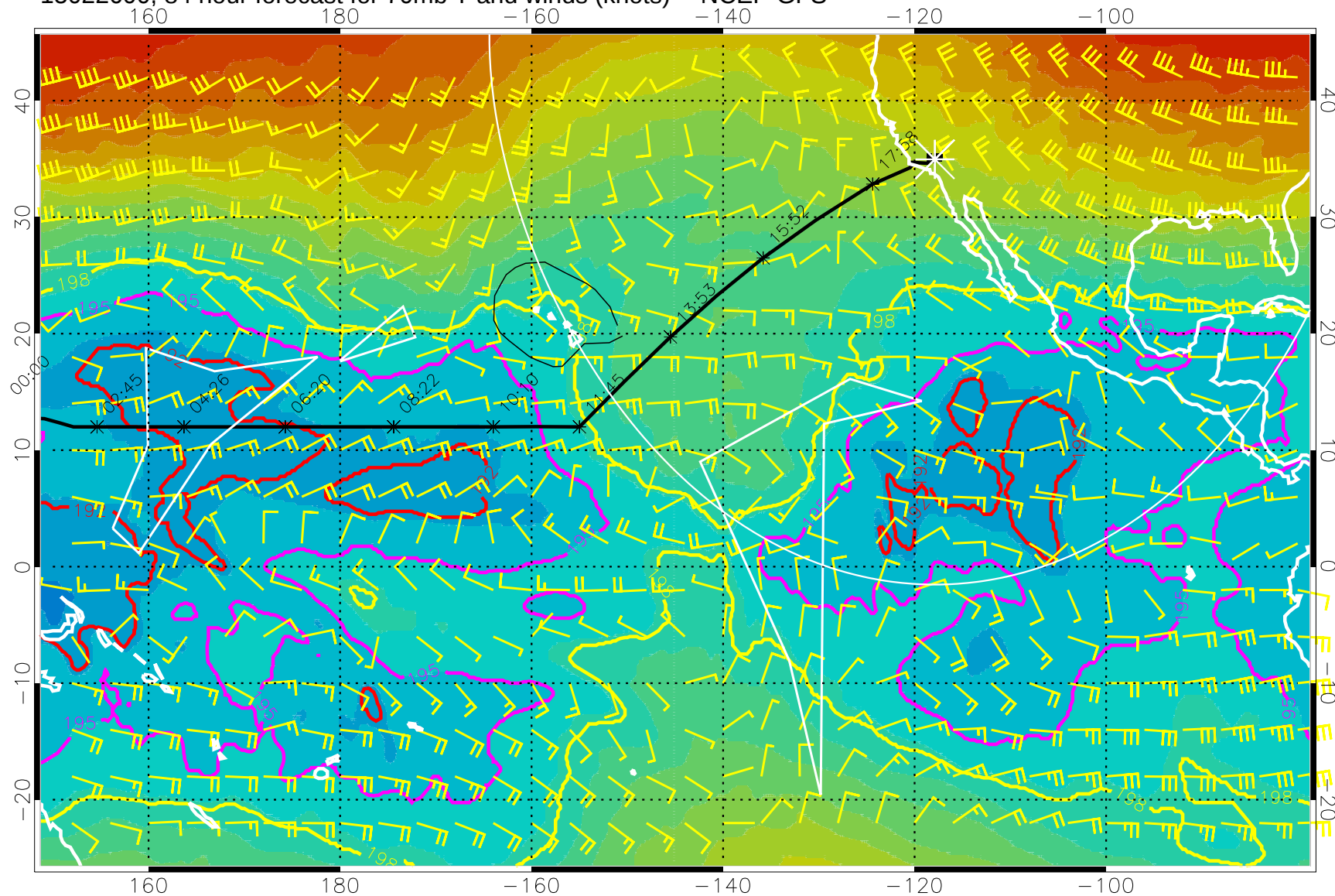
15022600, 84 hour forecast for 70mb T and winds (knots) -- NCEP GFS
