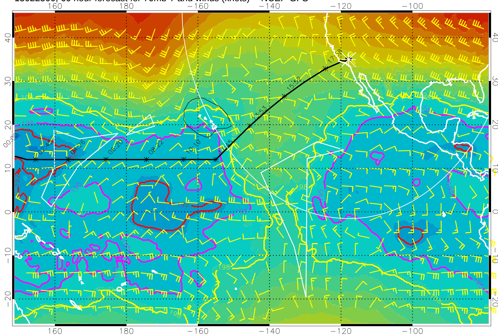
15022500, 60 hour forecast for 70mb T and winds (knots) -- NCEP GFS
