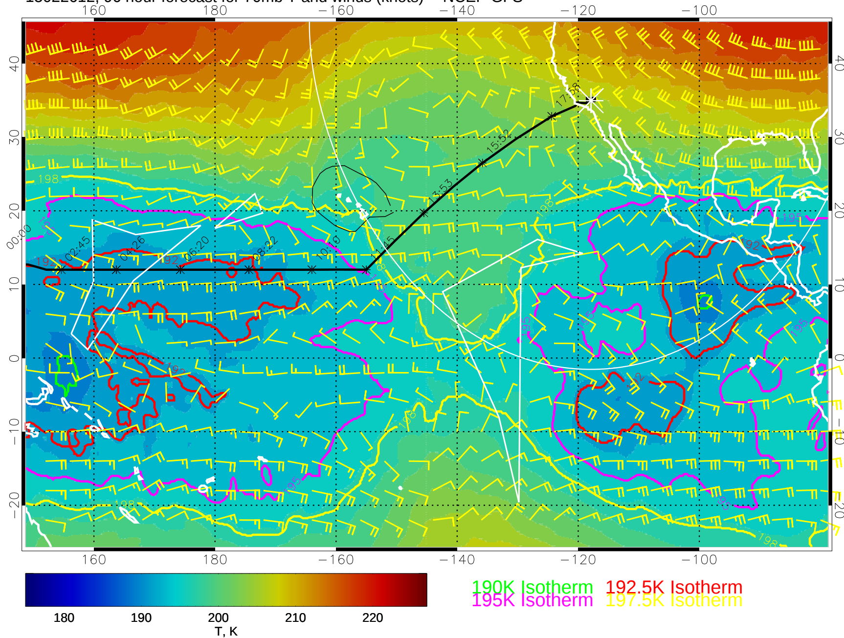
15022612, 96 hour forecast for 70mb T and winds (knots) -- NCEP GFS
