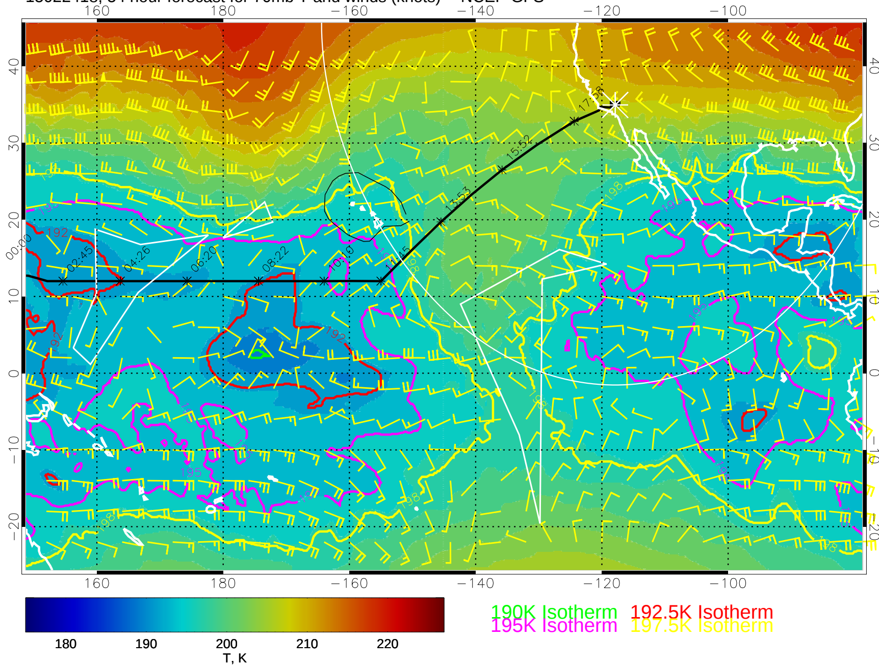
15022418, 54 hour forecast for 70mb T and winds (knots) -- NCEP GFS
