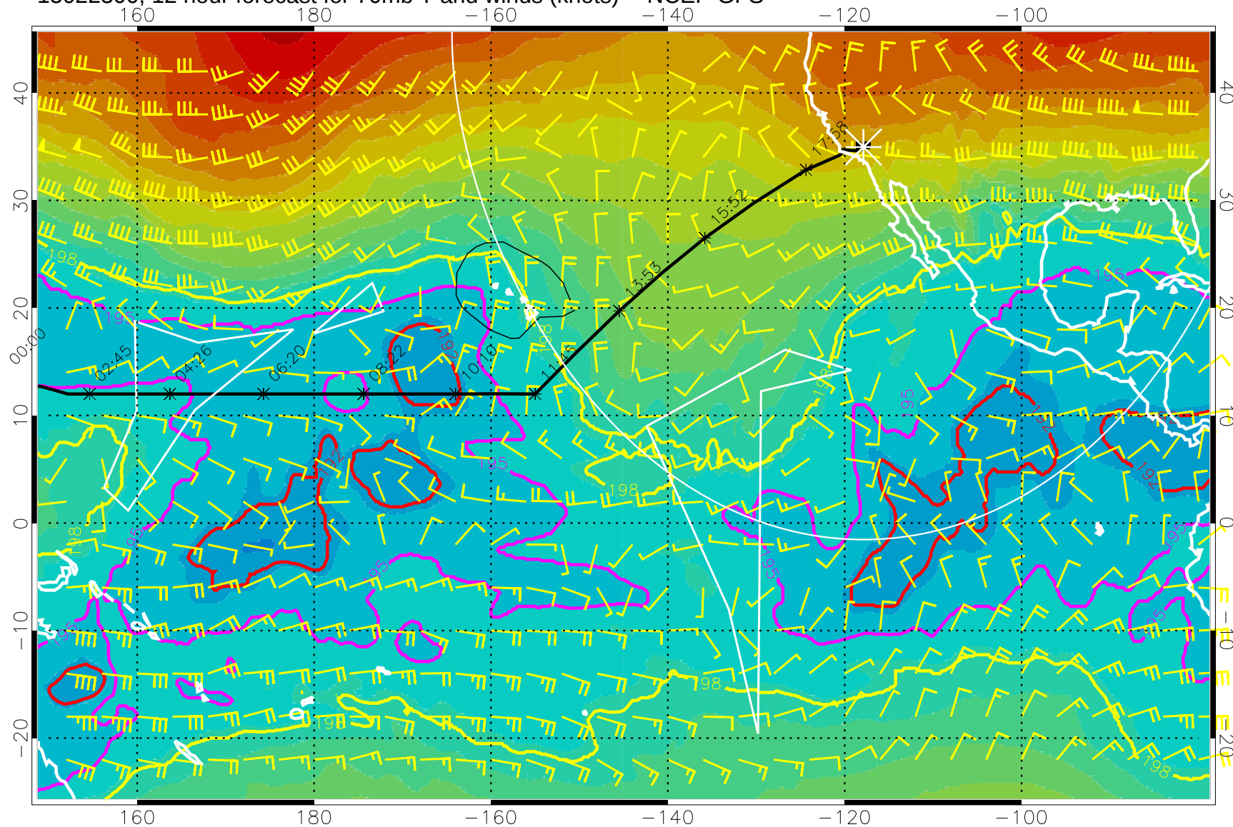
15022300, 12 hour forecast for 70mb T and winds (knots) -- NCEP GFS
