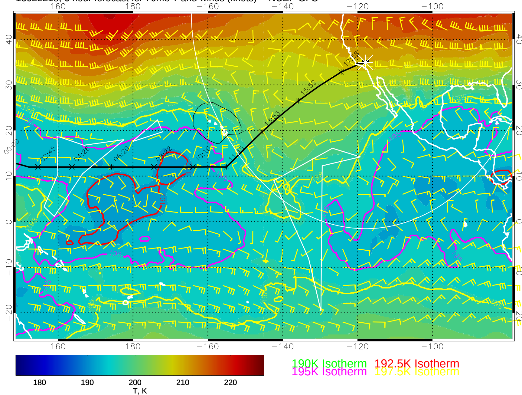
15022218, 6 hour forecast for 70mb T and winds (knots) -- NCEP GFS
