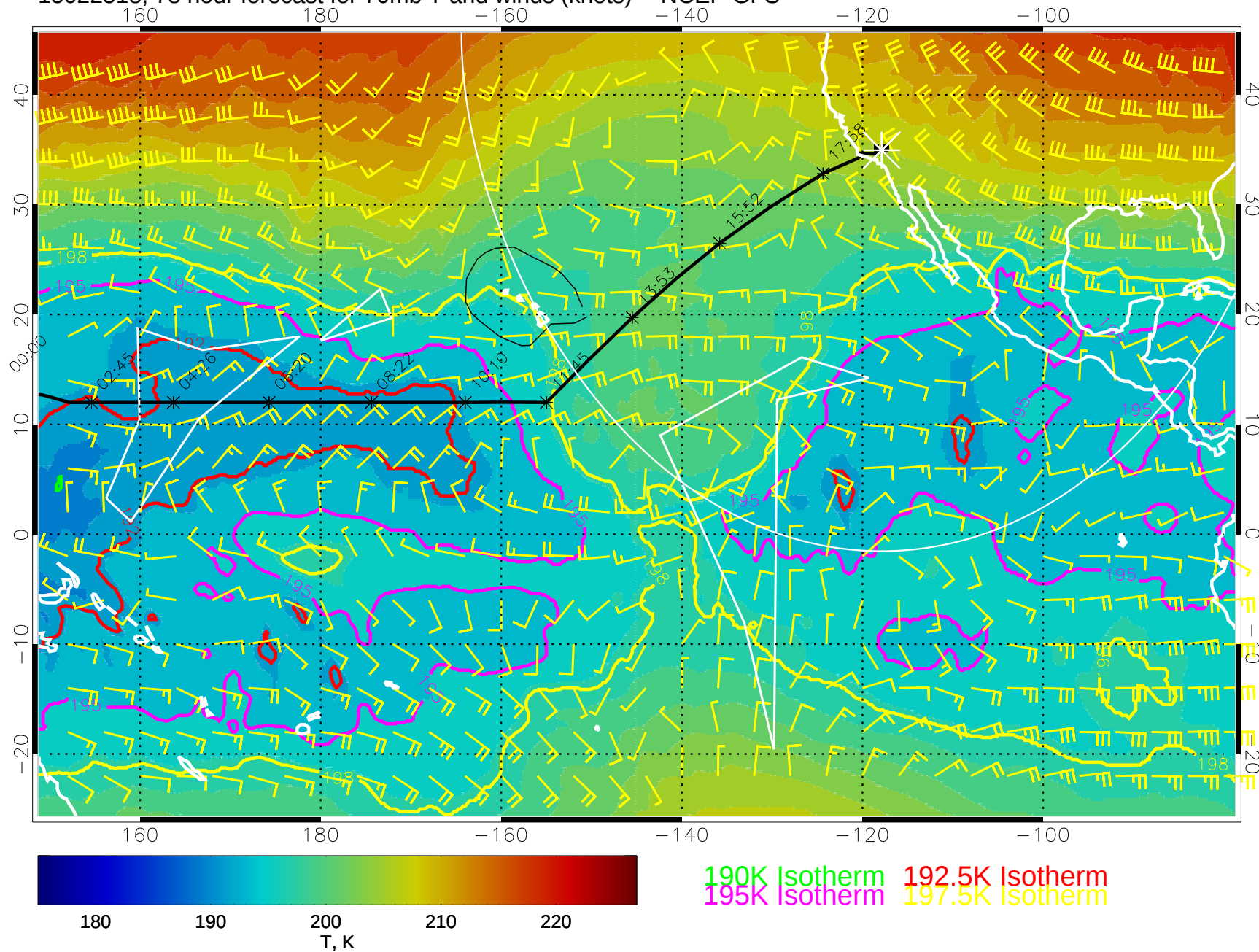
15022518, 78 hour forecast for 70mb T and winds (knots) -- NCEP GFS
