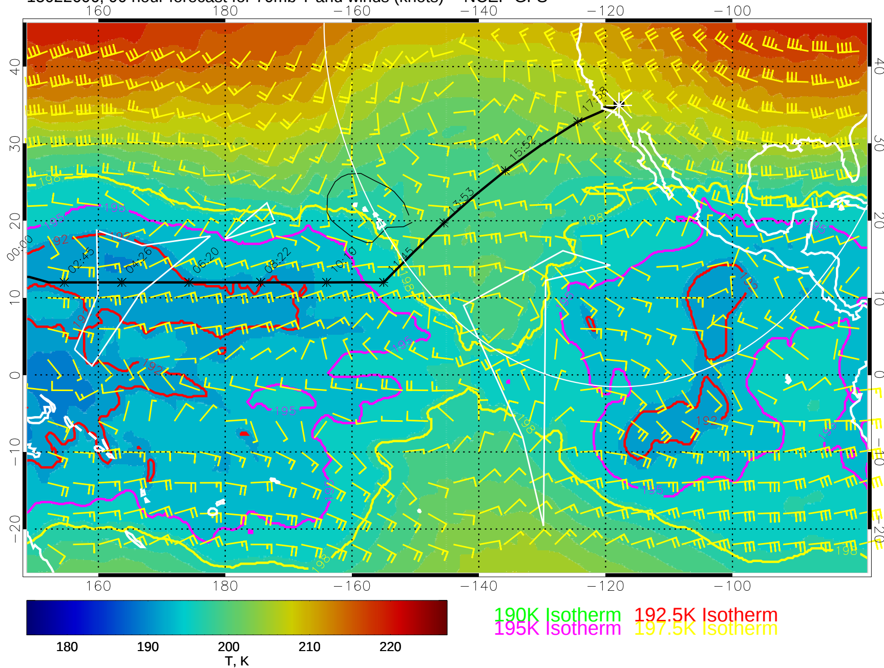
15022606, 90 hour forecast for 70mb T and winds (knots) -- NCEP GFS
