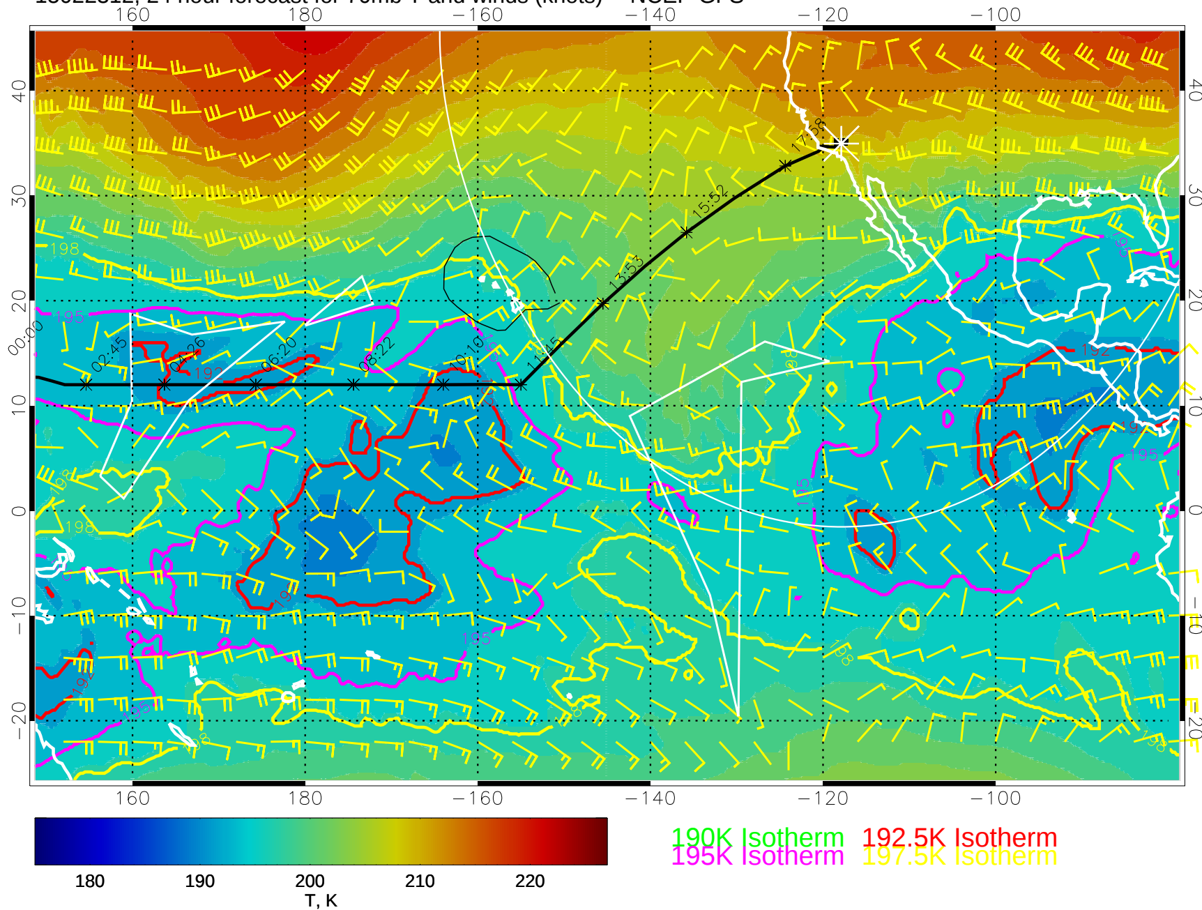
15022312, 24 hour forecast for 70mb T and winds (knots) -- NCEP GFS
