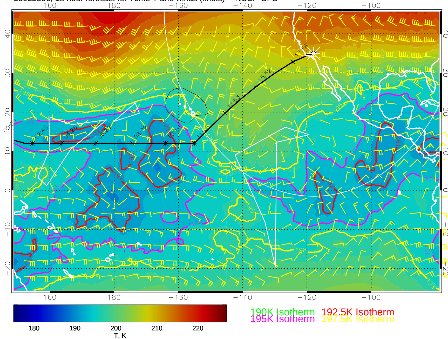
15022306, 18 hour forecast for 70mb T and winds (knots) -- NCEP GFS
