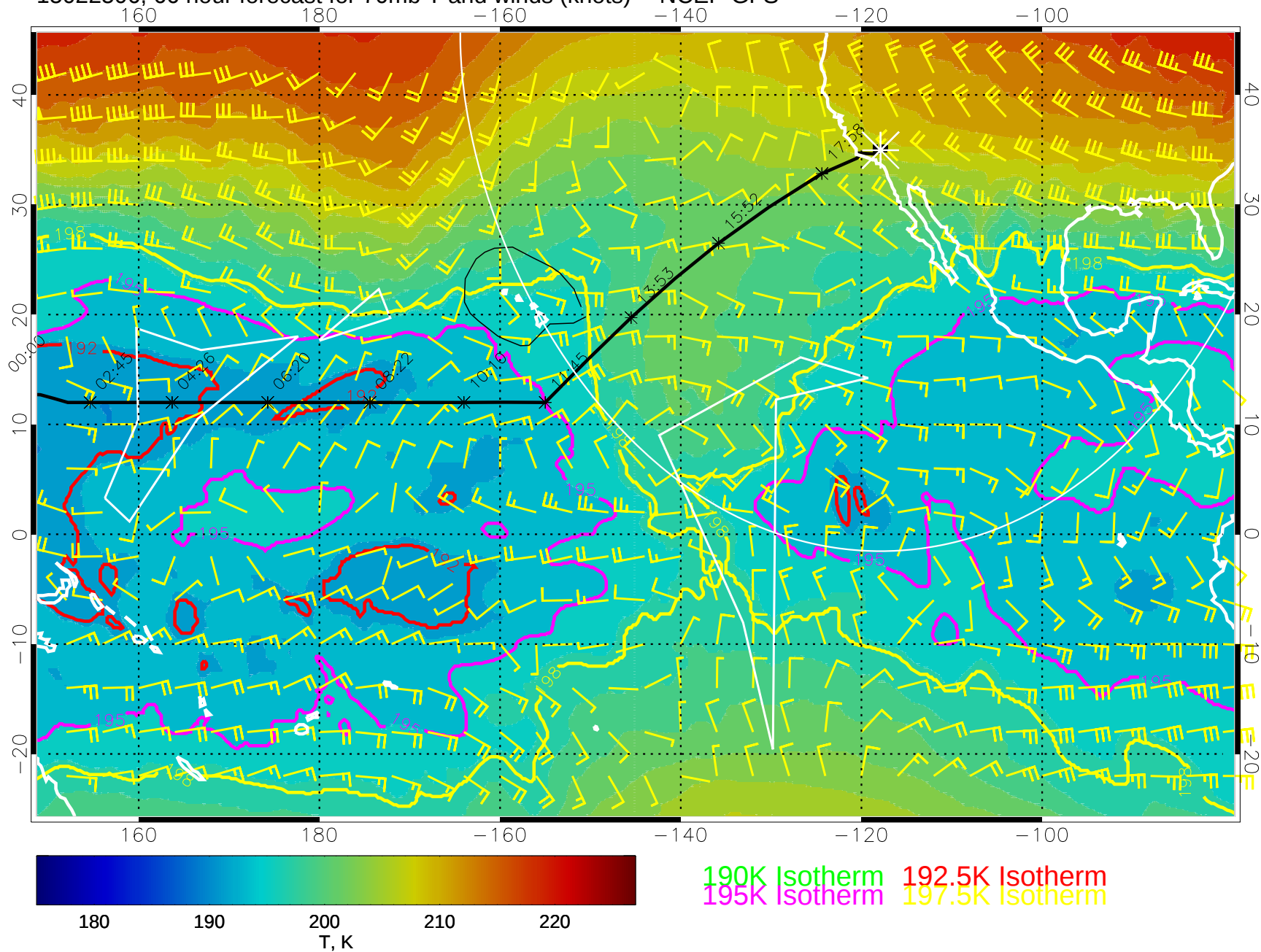
15022506, 66 hour forecast for 70mb T and winds (knots) -- NCEP GFS
