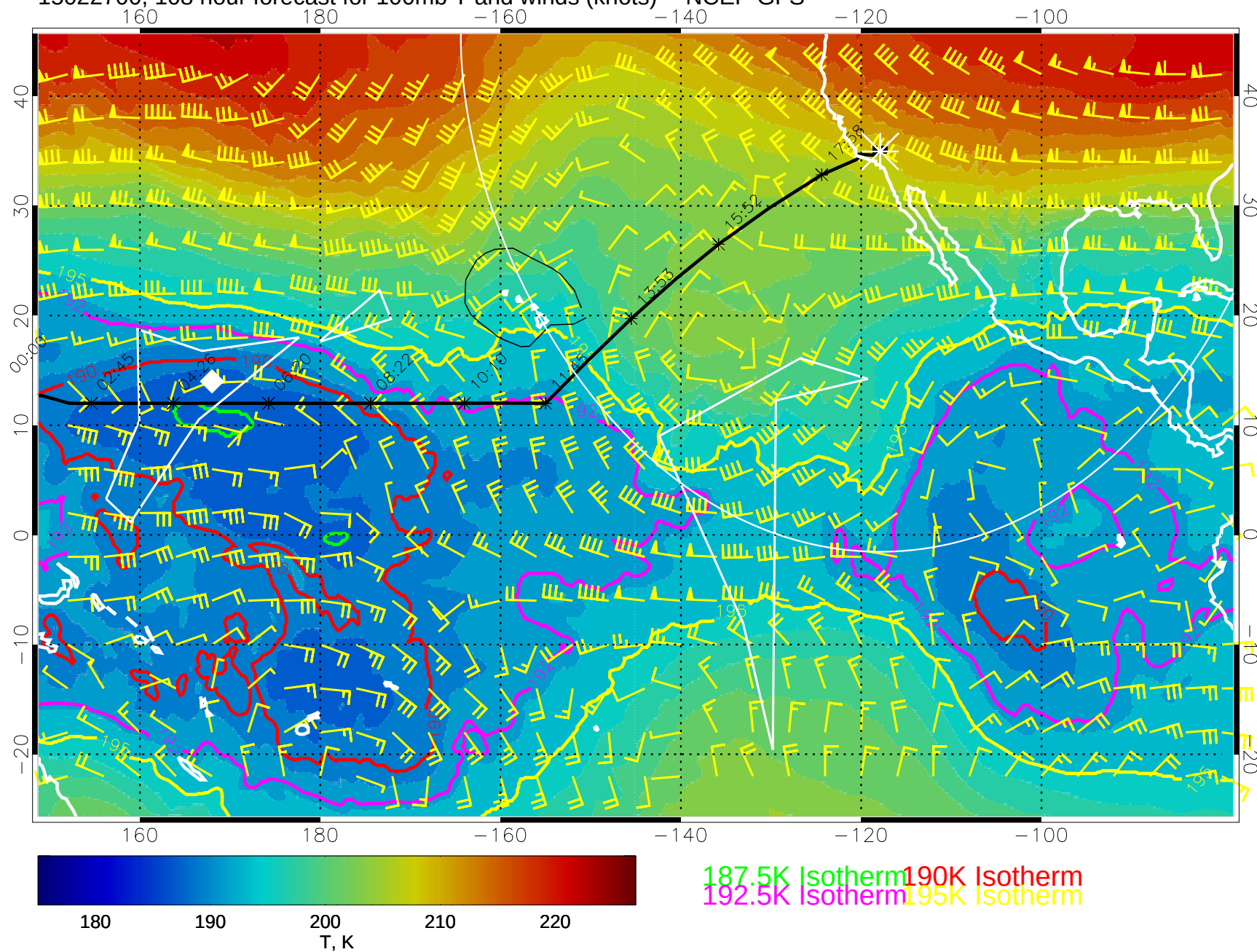
15022700, 108 hour forecast for 100mb T and winds (knots) -- NCEP GFS
