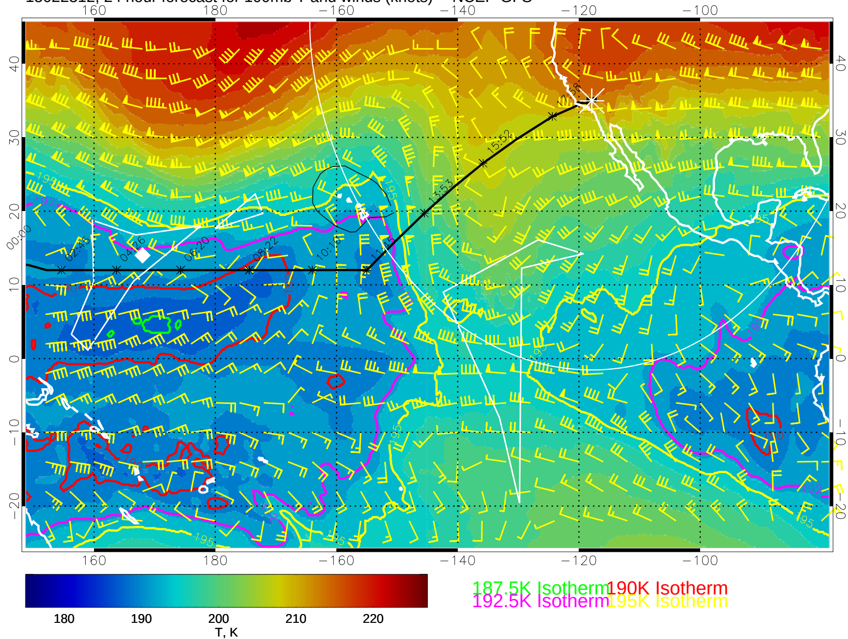
15022312, 24 hour forecast for 100mb T and winds (knots) -- NCEP GFS
