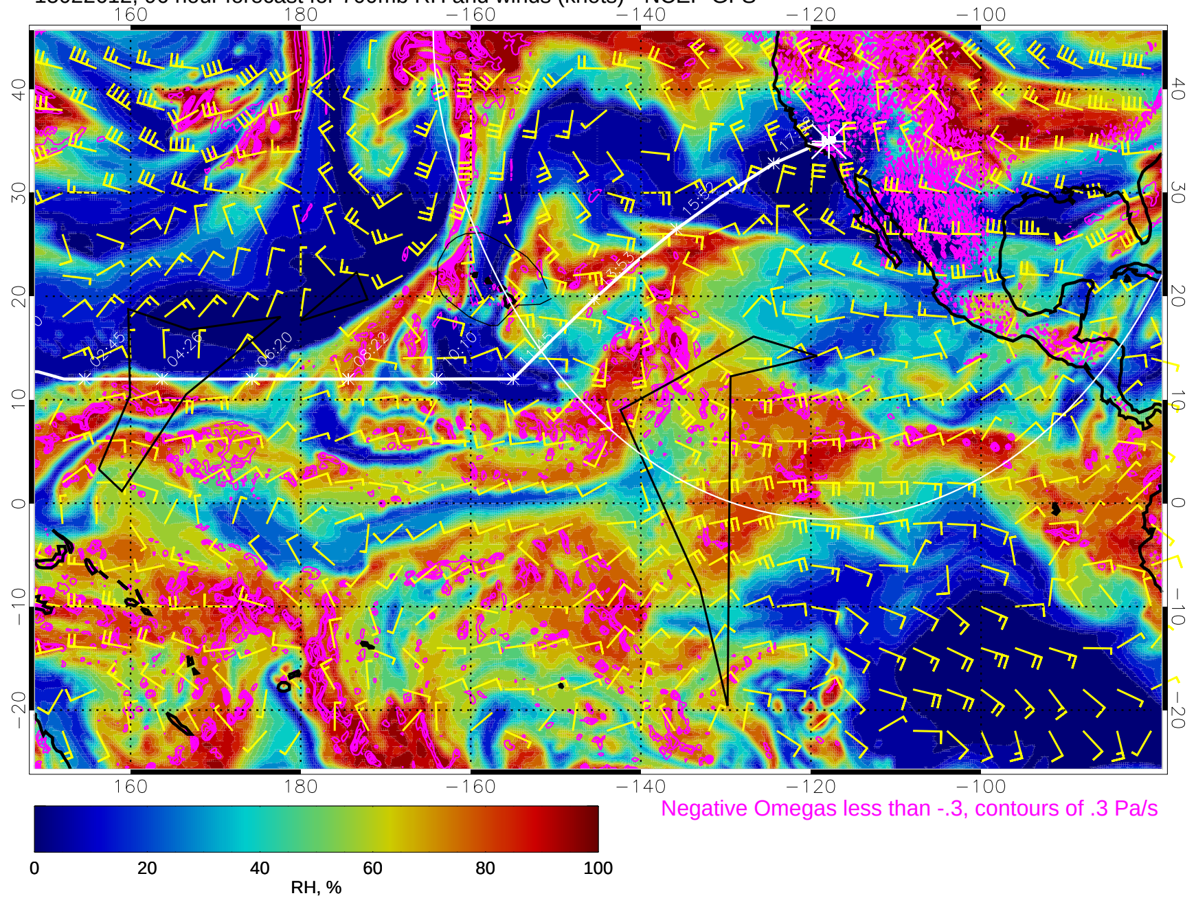
15022612, 96 hour forecast for 700mb RH and winds (knots) - NCEP GFS
