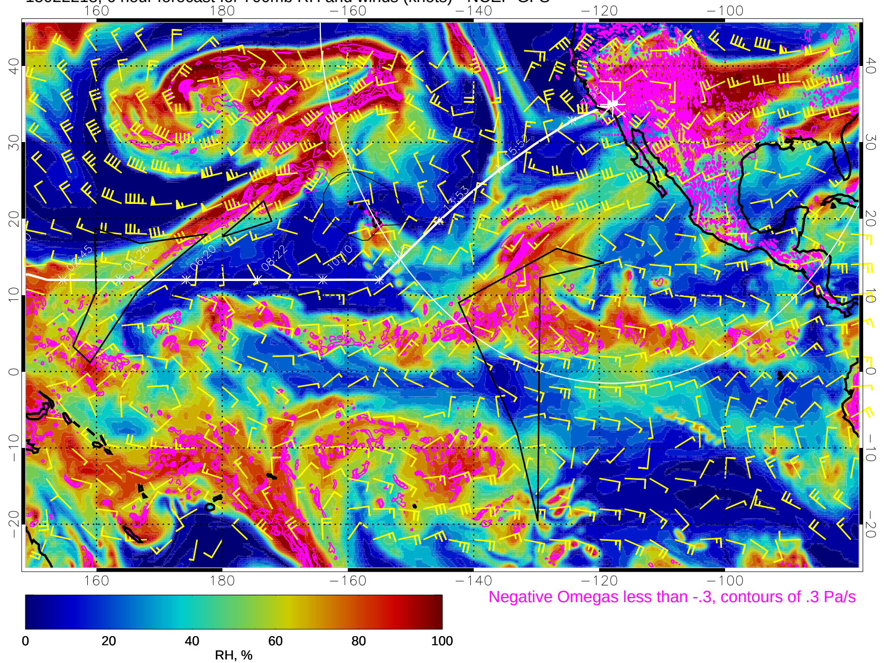
15022218, 6 hour forecast for 700mb RH and winds (knots) - NCEP GFS
