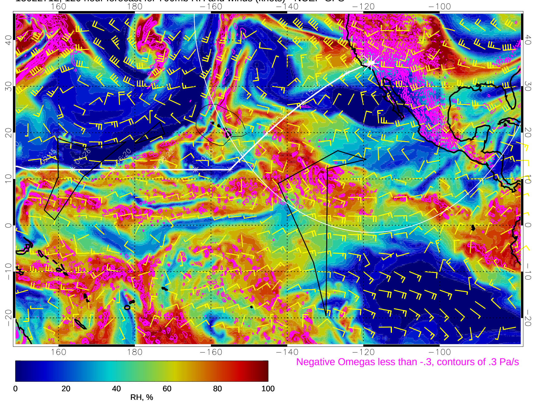
15022712, 120 hour forecast for 700mb RH and winds (knots) - NCEP GFS
