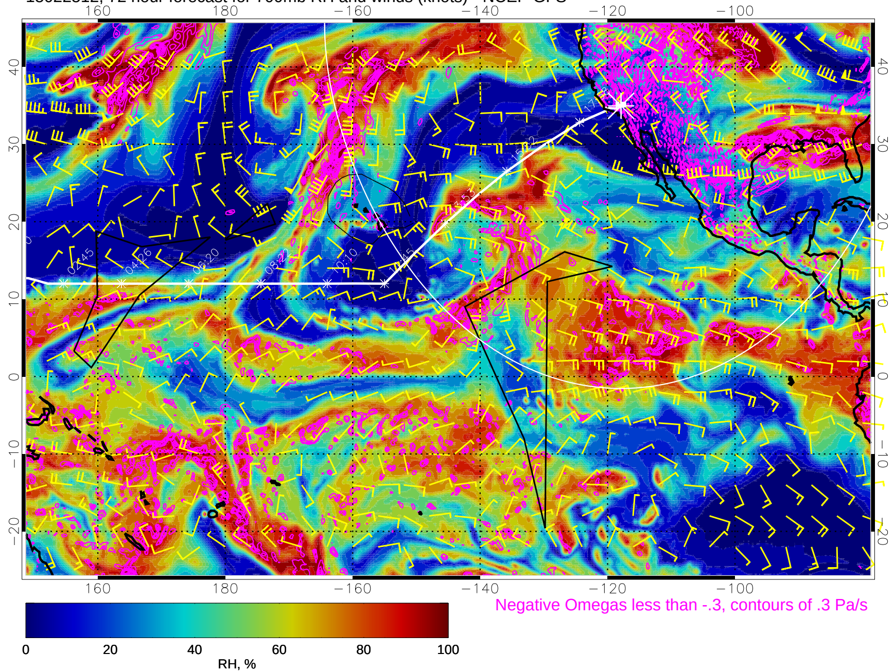
15022512, 72 hour forecast for 700mb RH and winds (knots) - NCEP GFS
