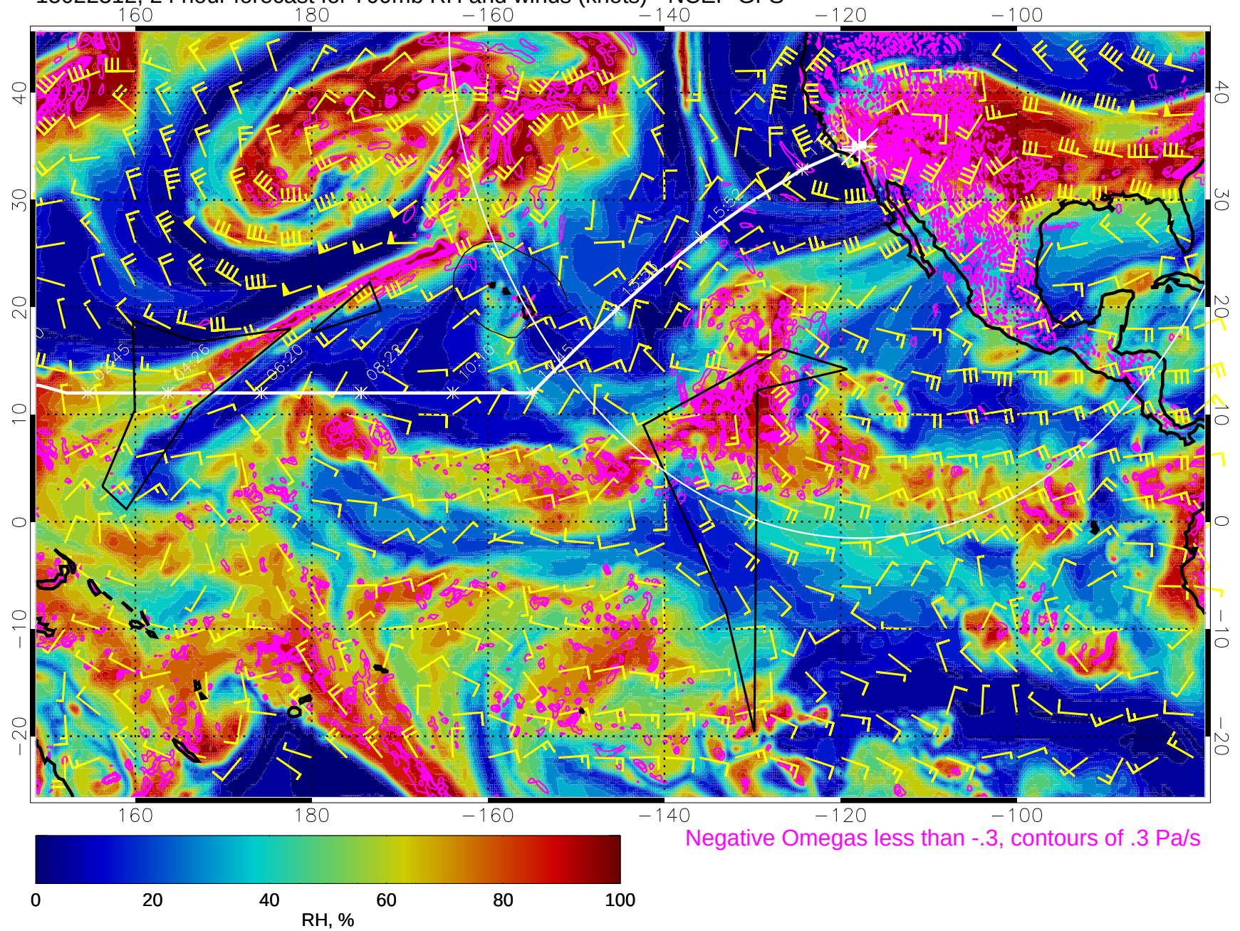
15022312, 24 hour forecast for 700mb RH and winds (knots) - NCEP GFS
