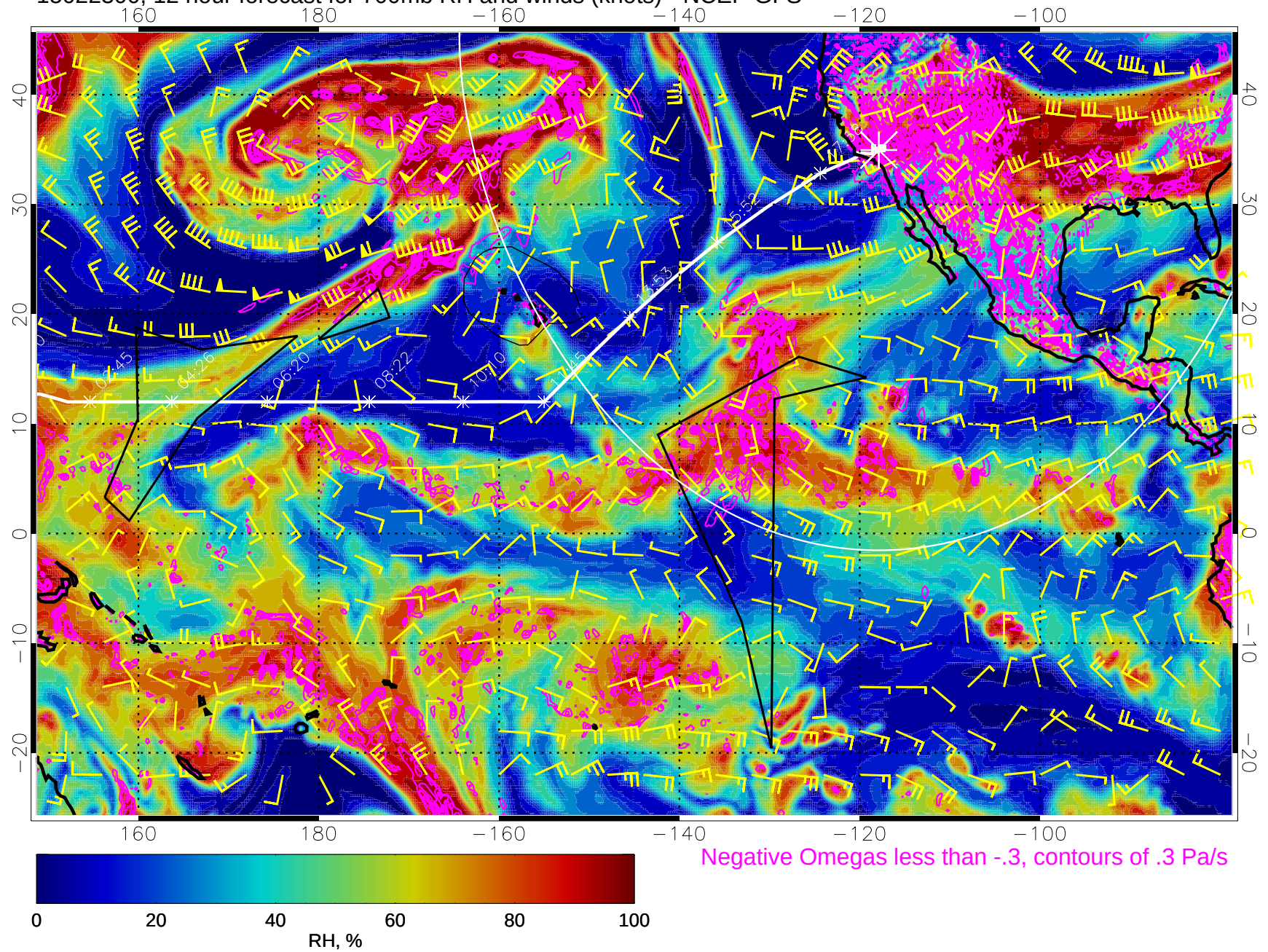
15022300, 12 hour forecast for 700mb RH and winds (knots) - NCEP GFS
