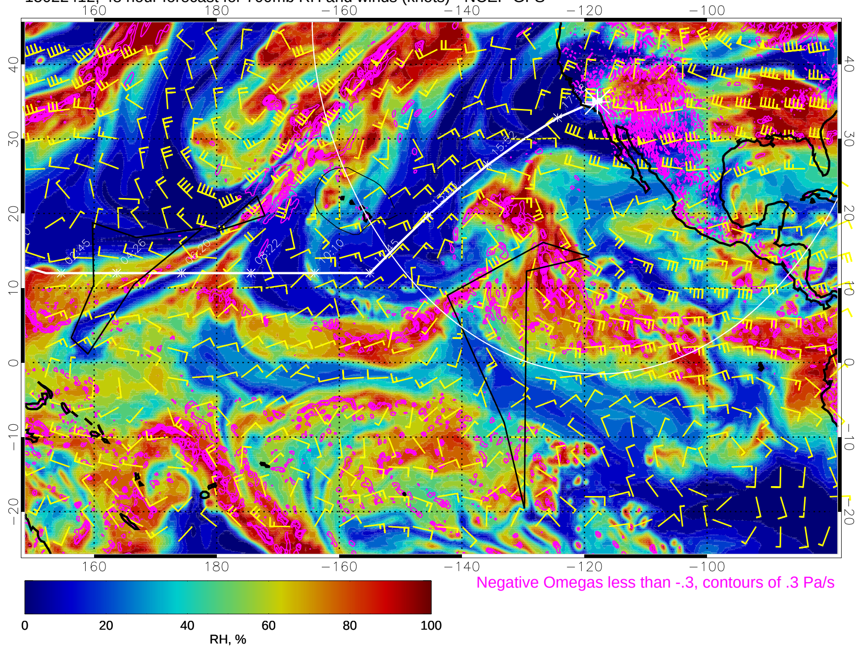
15022412, 48 hour forecast for 700mb RH and winds (knots) - NCEP GFS
