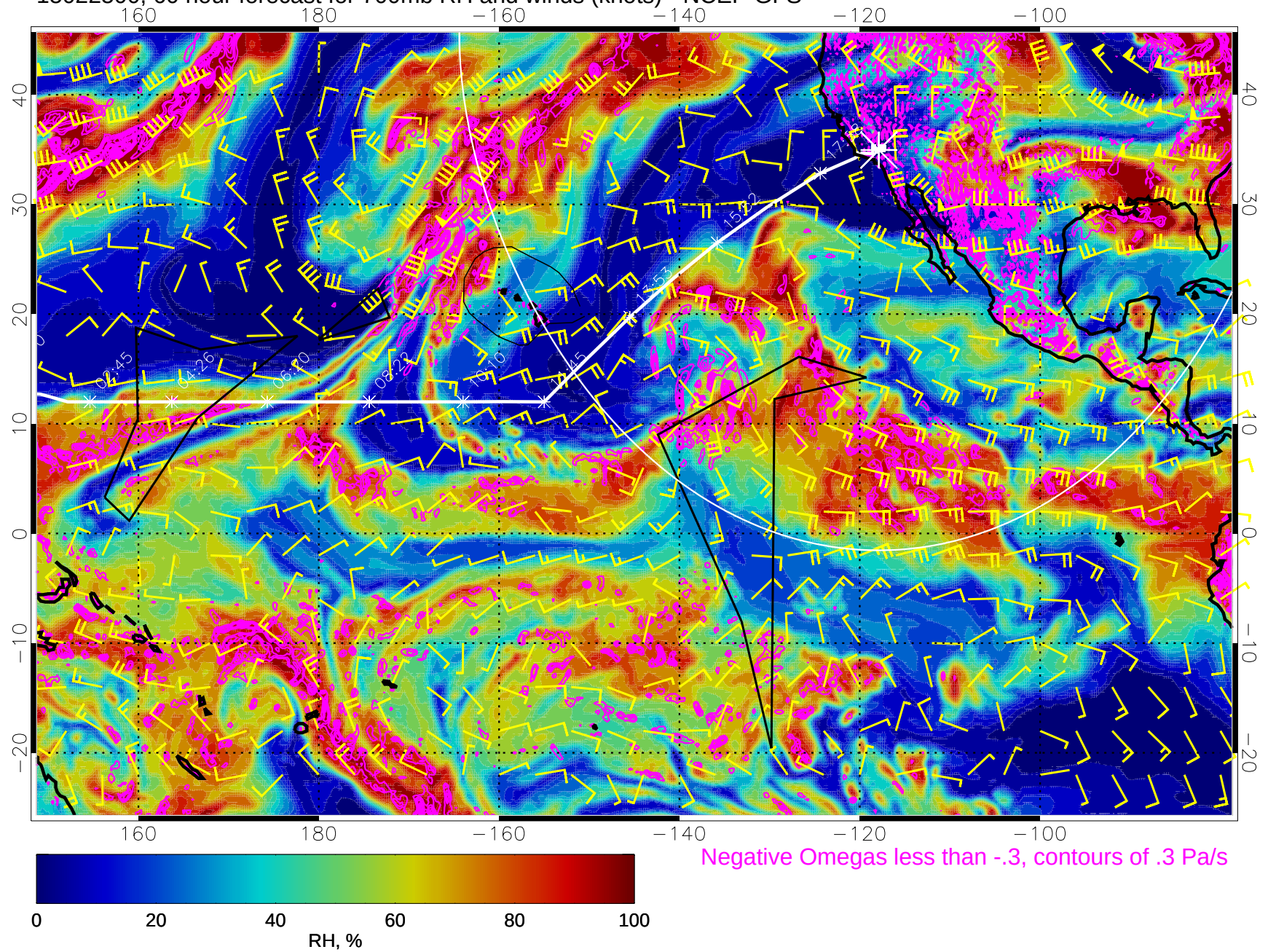
15022500, 60 hour forecast for 700mb RH and winds (knots) - NCEP GFS
