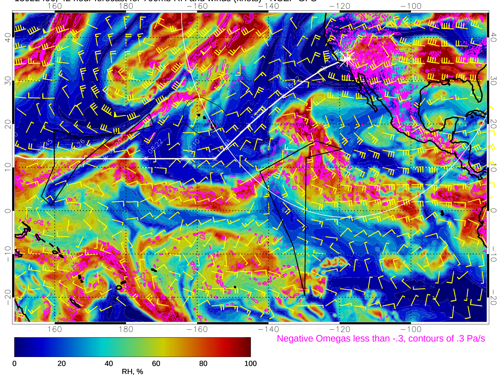
15022406, 42 hour forecast for 700mb RH and winds (knots) - NCEP GFS
