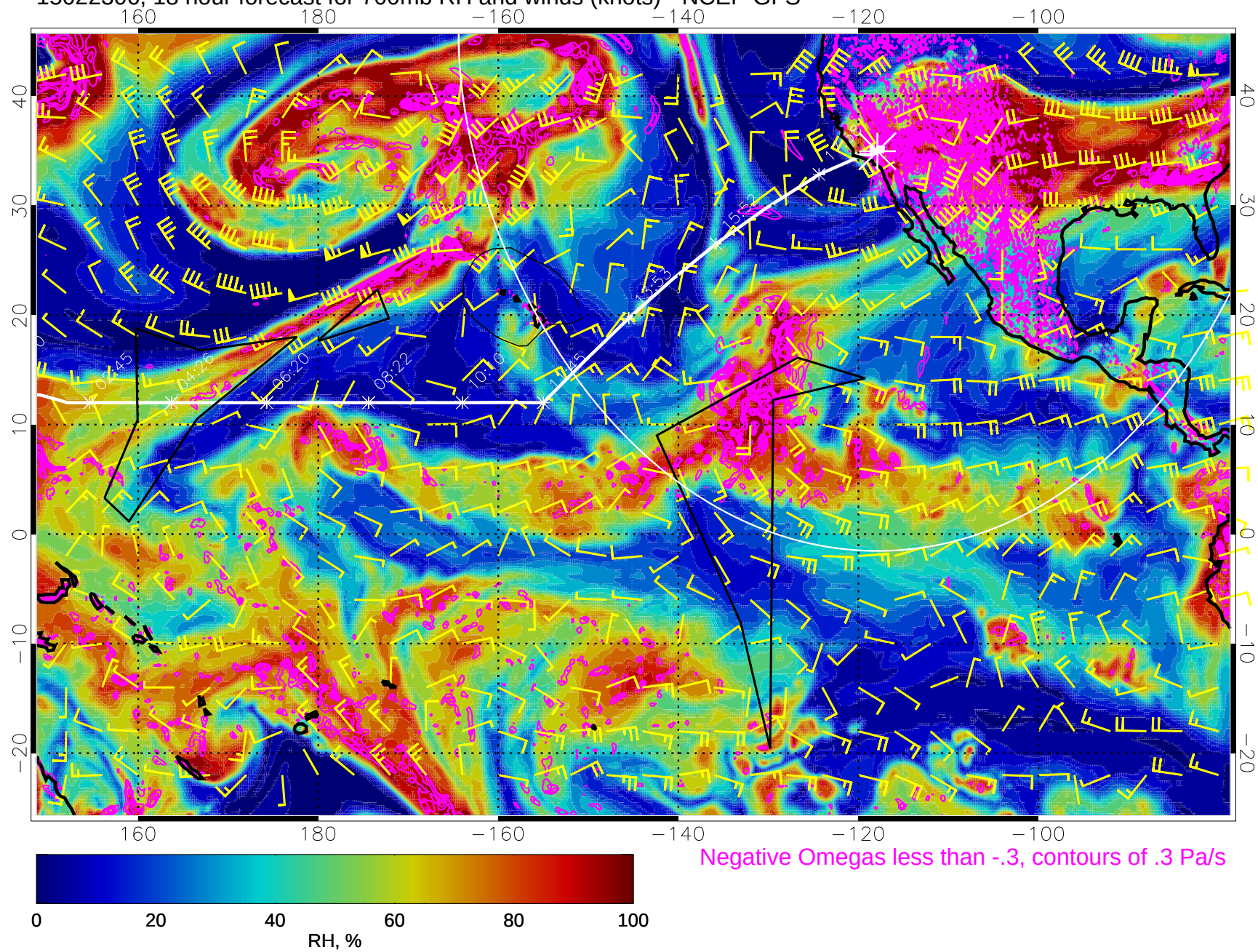
15022306, 18 hour forecast for 700mb RH and winds (knots) - NCEP GFS
