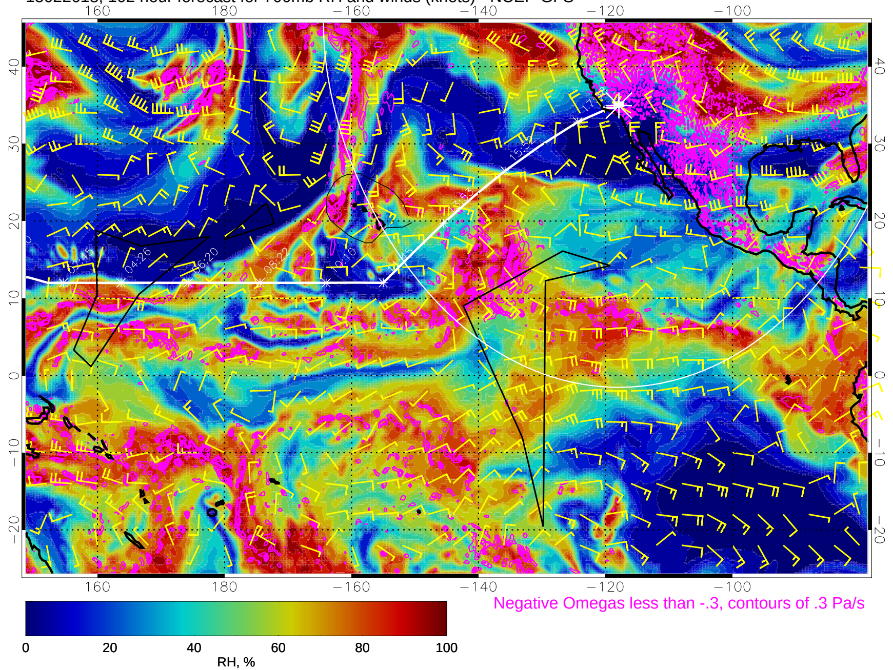
15022618, 102 hour forecast for 700mb RH and winds (knots) - NCEP GFS
