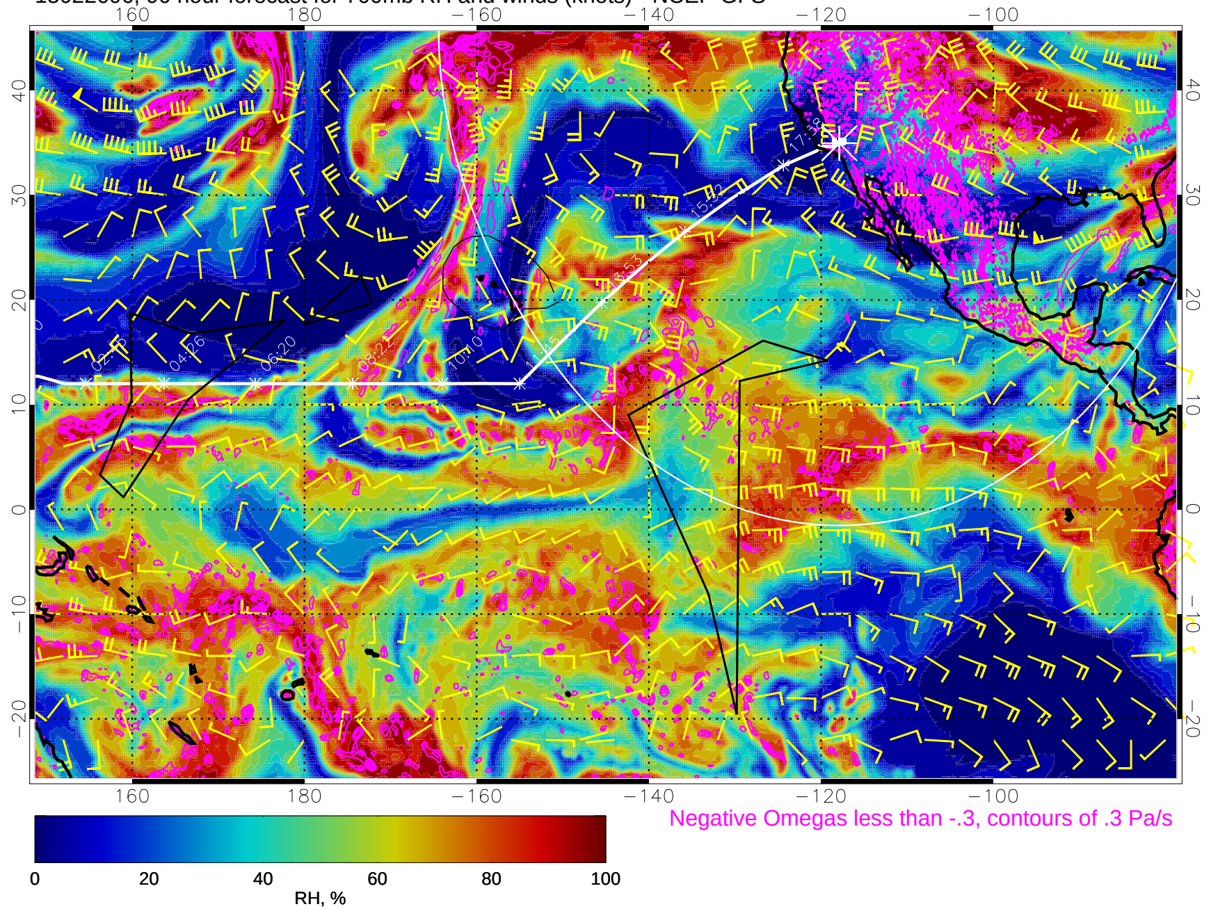
15022606, 90 hour forecast for 700mb RH and winds (knots) - NCEP GFS
