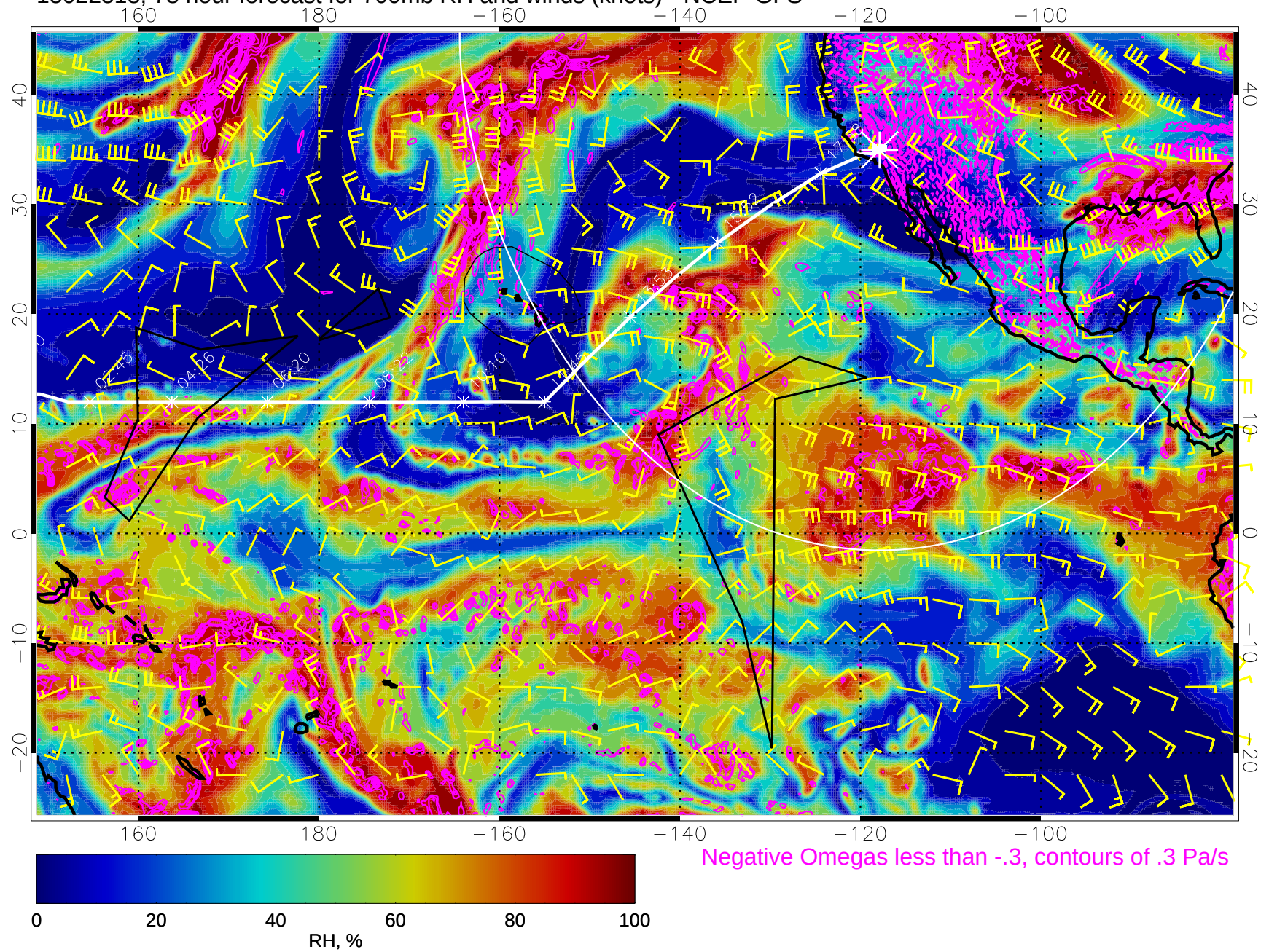
15022518, 78 hour forecast for 700mb RH and winds (knots) - NCEP GFS
