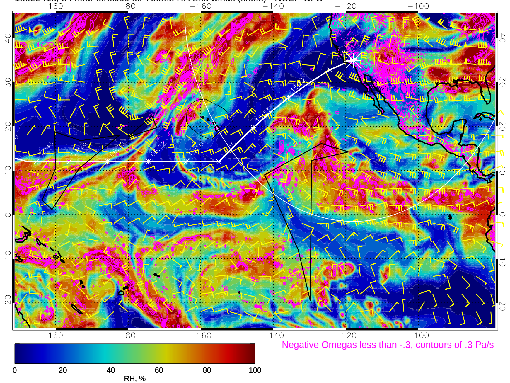
15022418, 54 hour forecast for 700mb RH and winds (knots) - NCEP GFS
