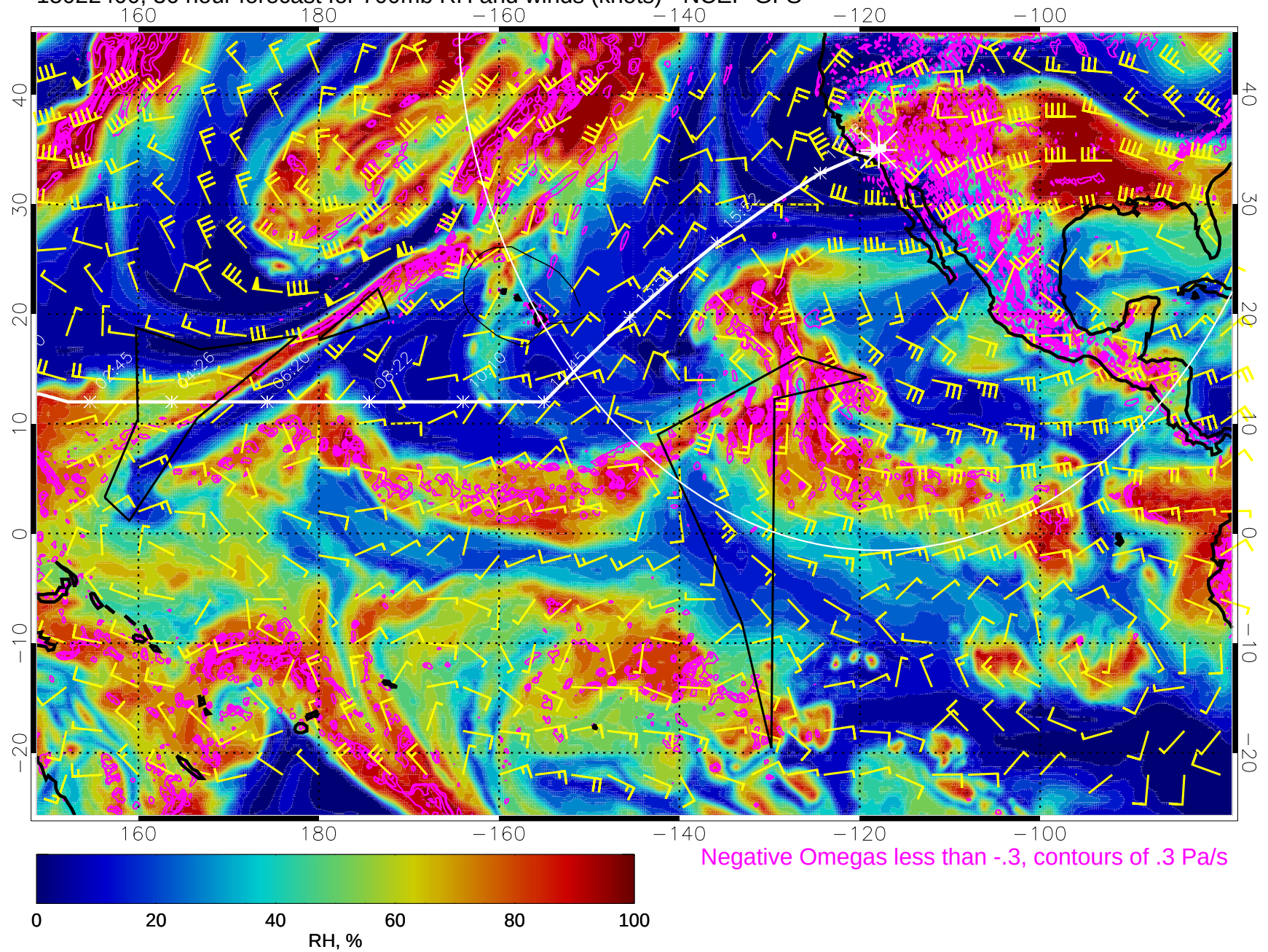
15022400, 36 hour forecast for 700mb RH and winds (knots) - NCEP GFS
