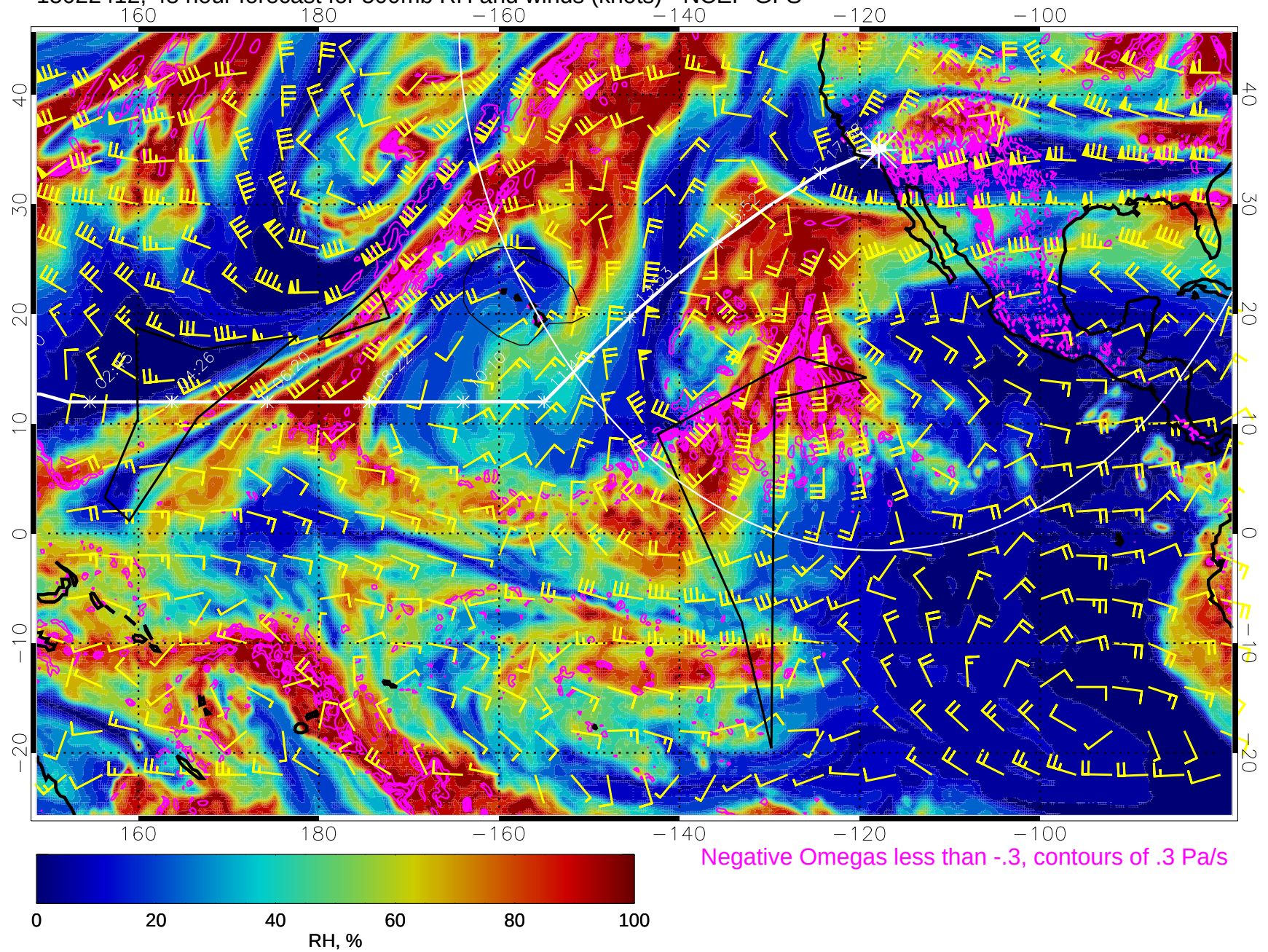
15022412, 48 hour forecast for 500mb RH and winds (knots) - NCEP GFS
