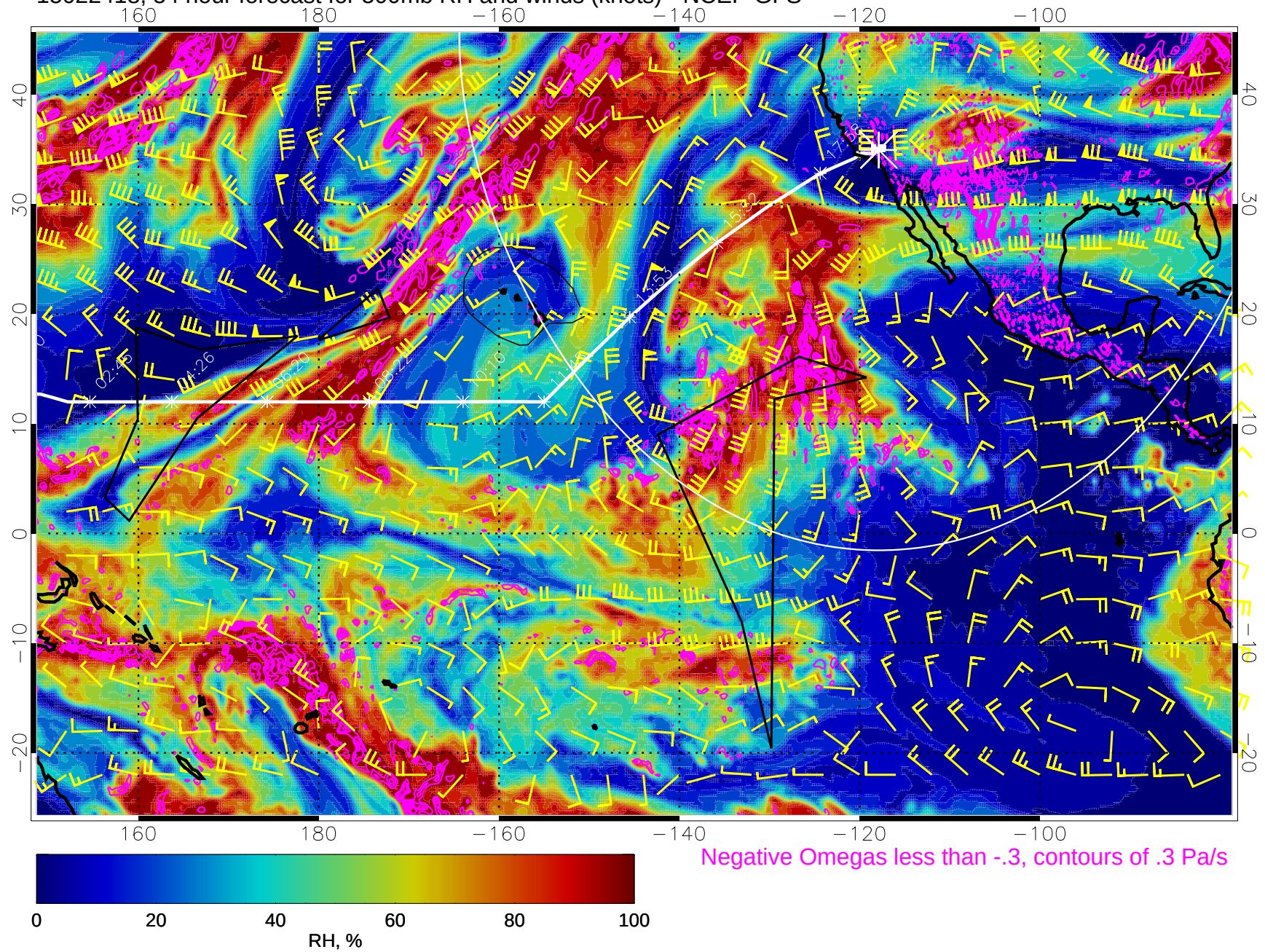
15022418, 54 hour forecast for 500mb RH and winds (knots) - NCEP GFS
