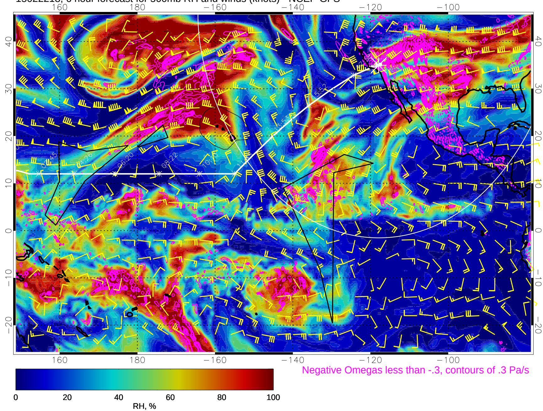
15022218, 6 hour forecast for 500mb RH and winds (knots) - NCEP GFS
