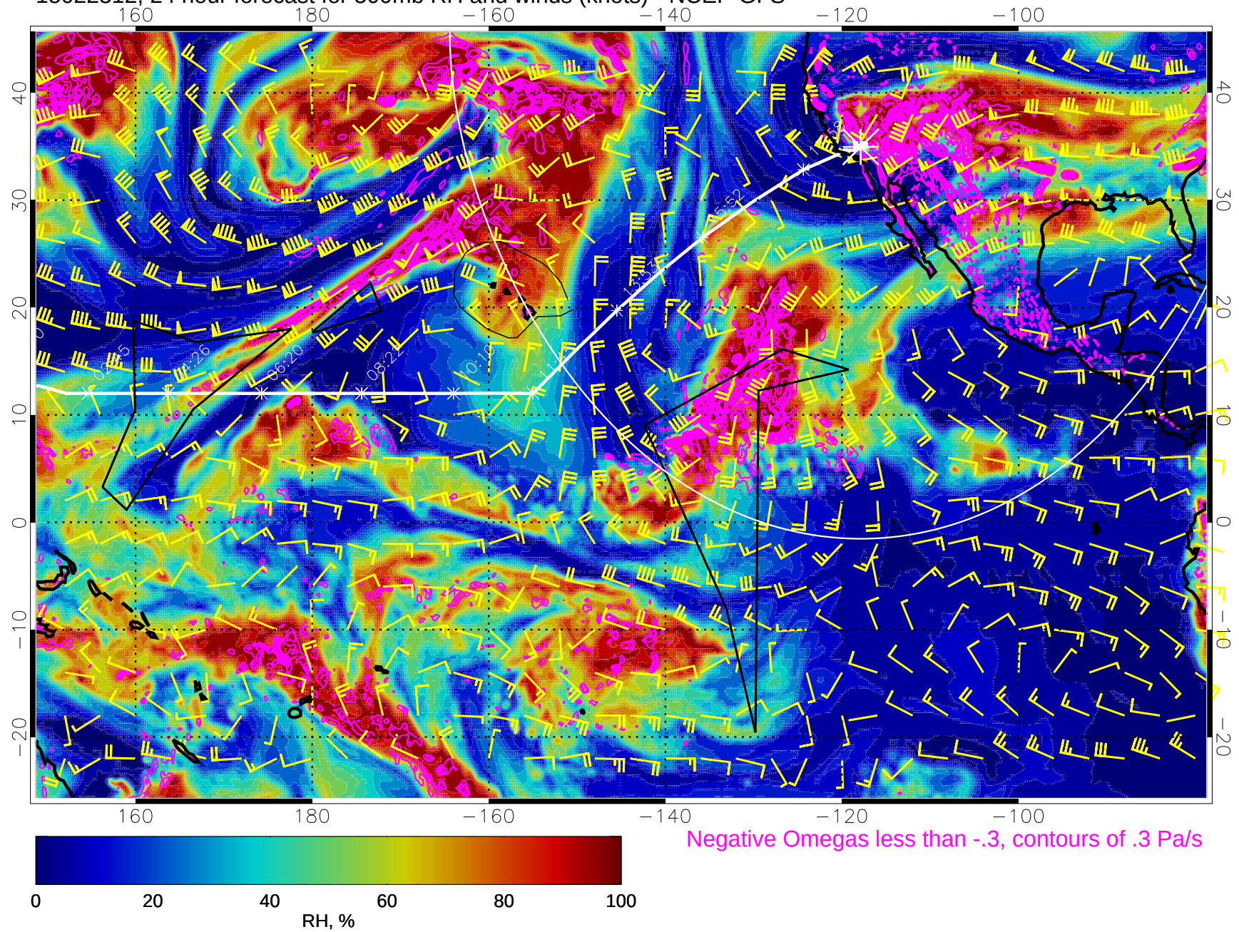
15022312, 24 hour forecast for 500mb RH and winds (knots) - NCEP GFS
