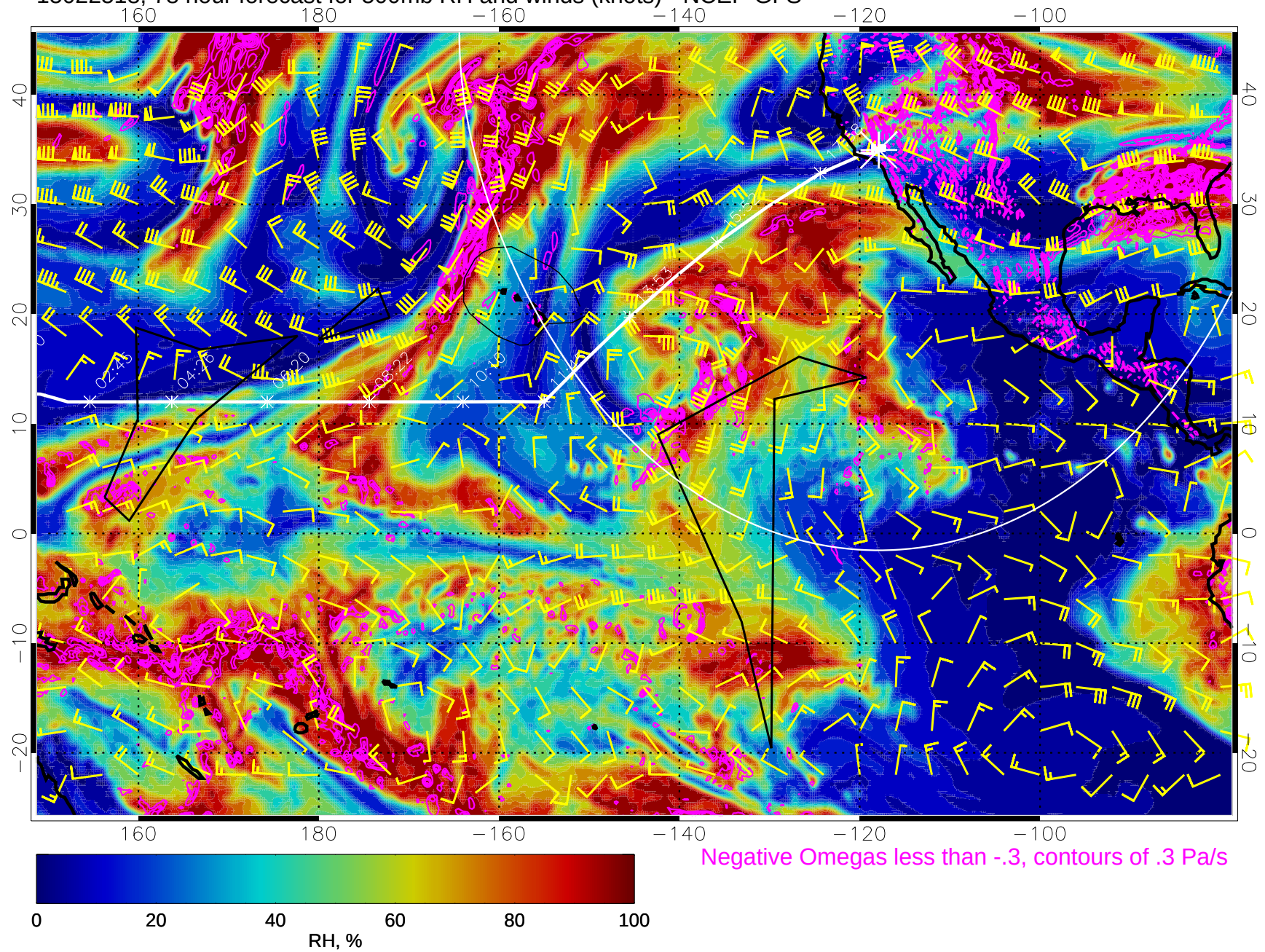
15022518, 78 hour forecast for 500mb RH and winds (knots) - NCEP GFS
