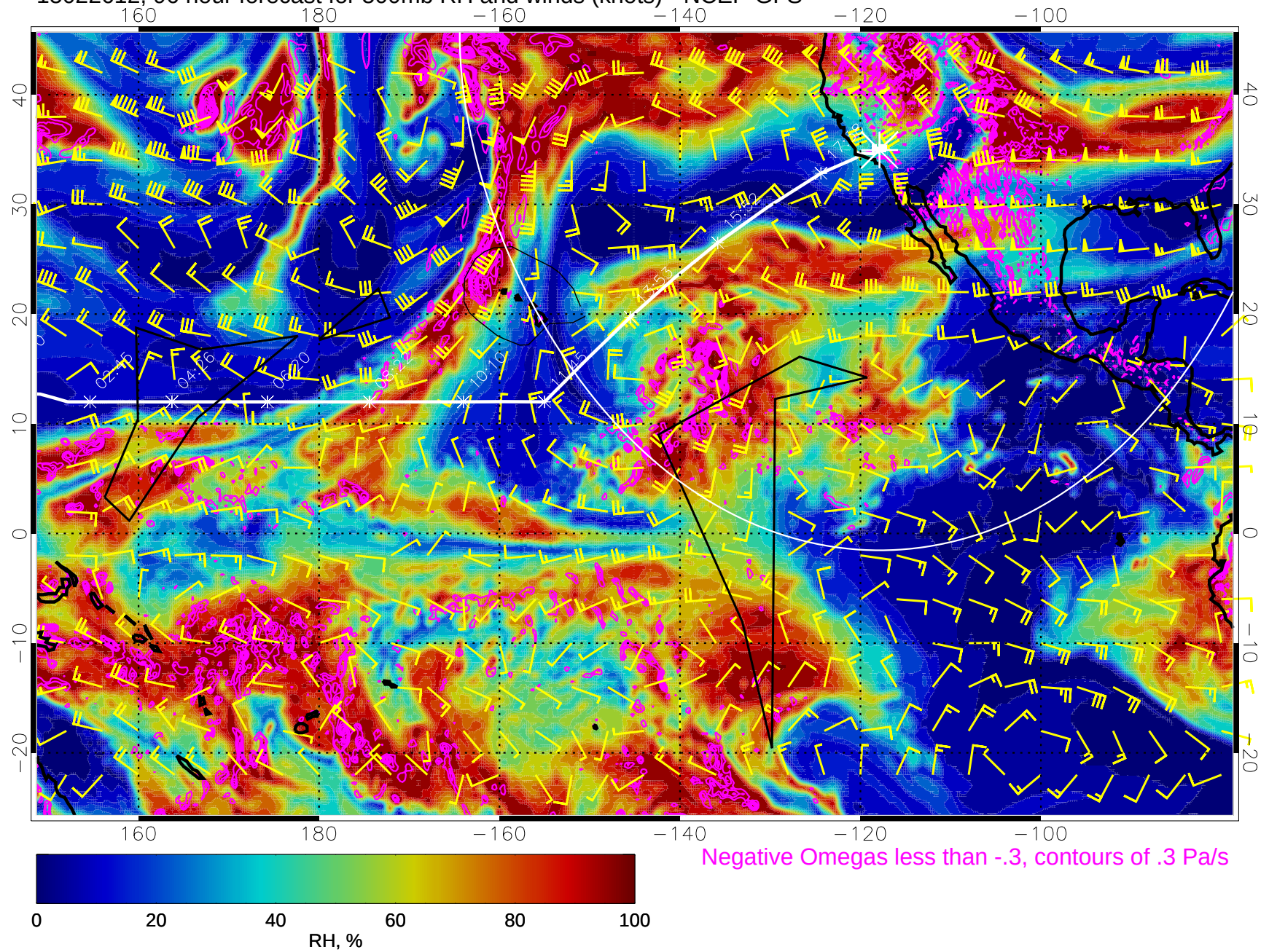
15022612, 96 hour forecast for 500mb RH and winds (knots) - NCEP GFS
