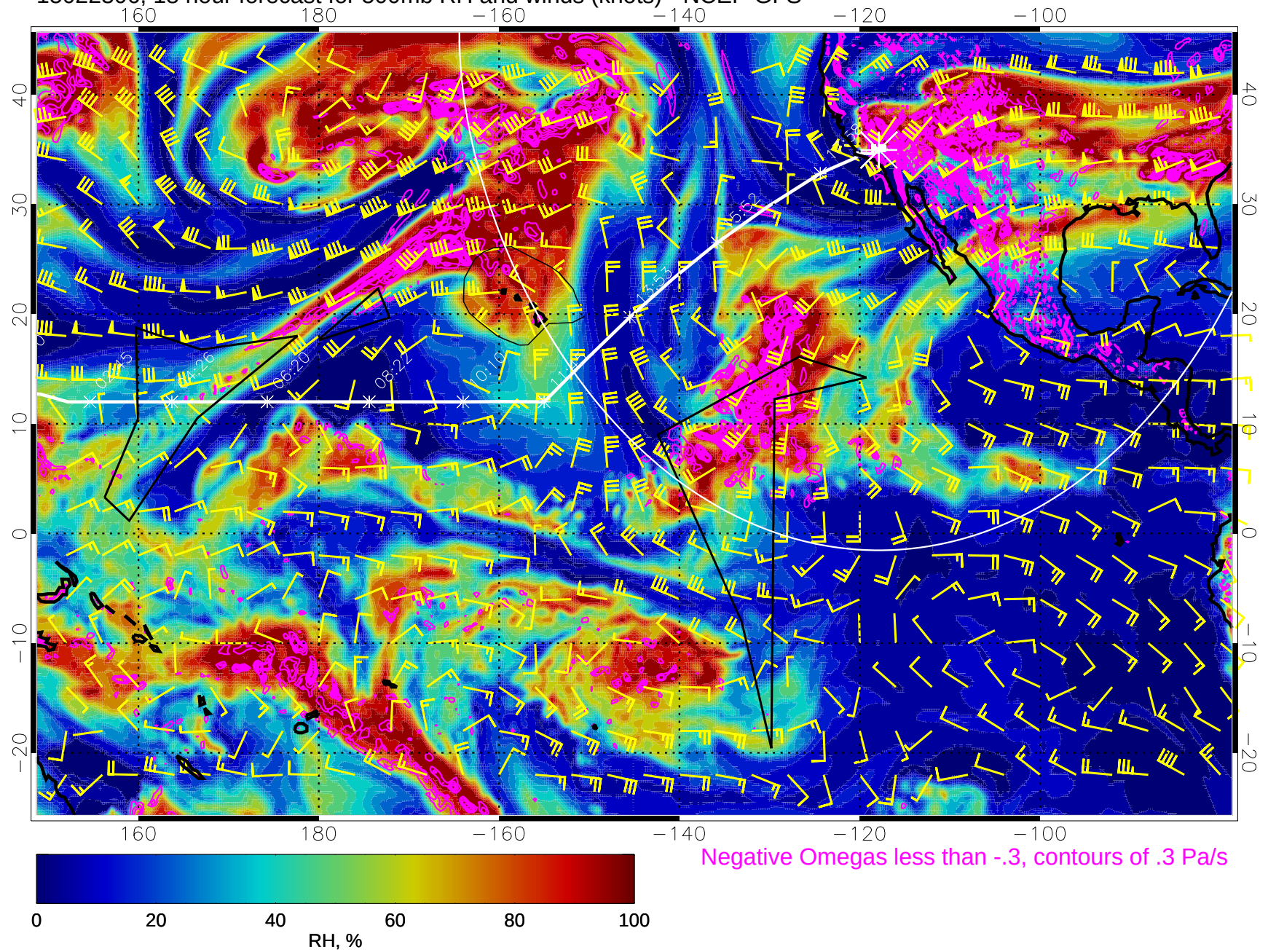
15022306, 18 hour forecast for 500mb RH and winds (knots) - NCEP GFS
