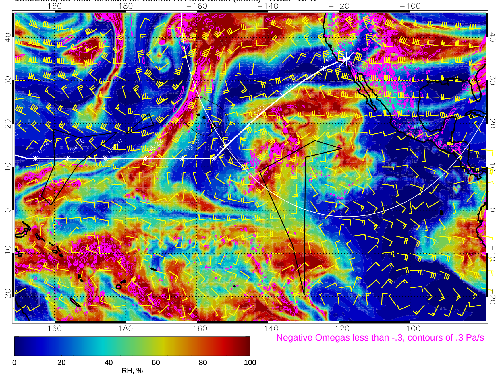
15022606, 90 hour forecast for 500mb RH and winds (knots) - NCEP GFS
