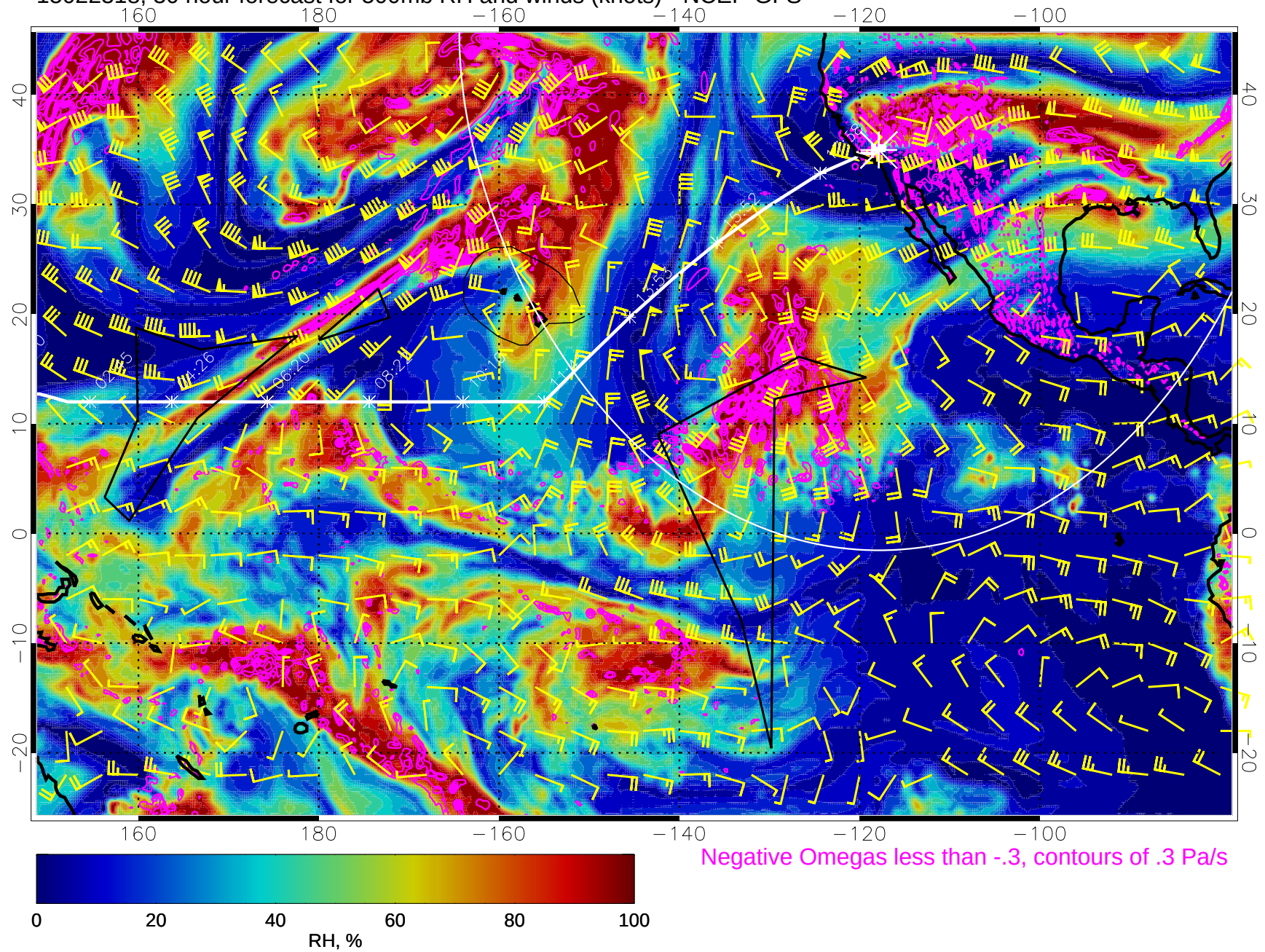
15022318, 30 hour forecast for 500mb RH and winds (knots) - NCEP GFS
