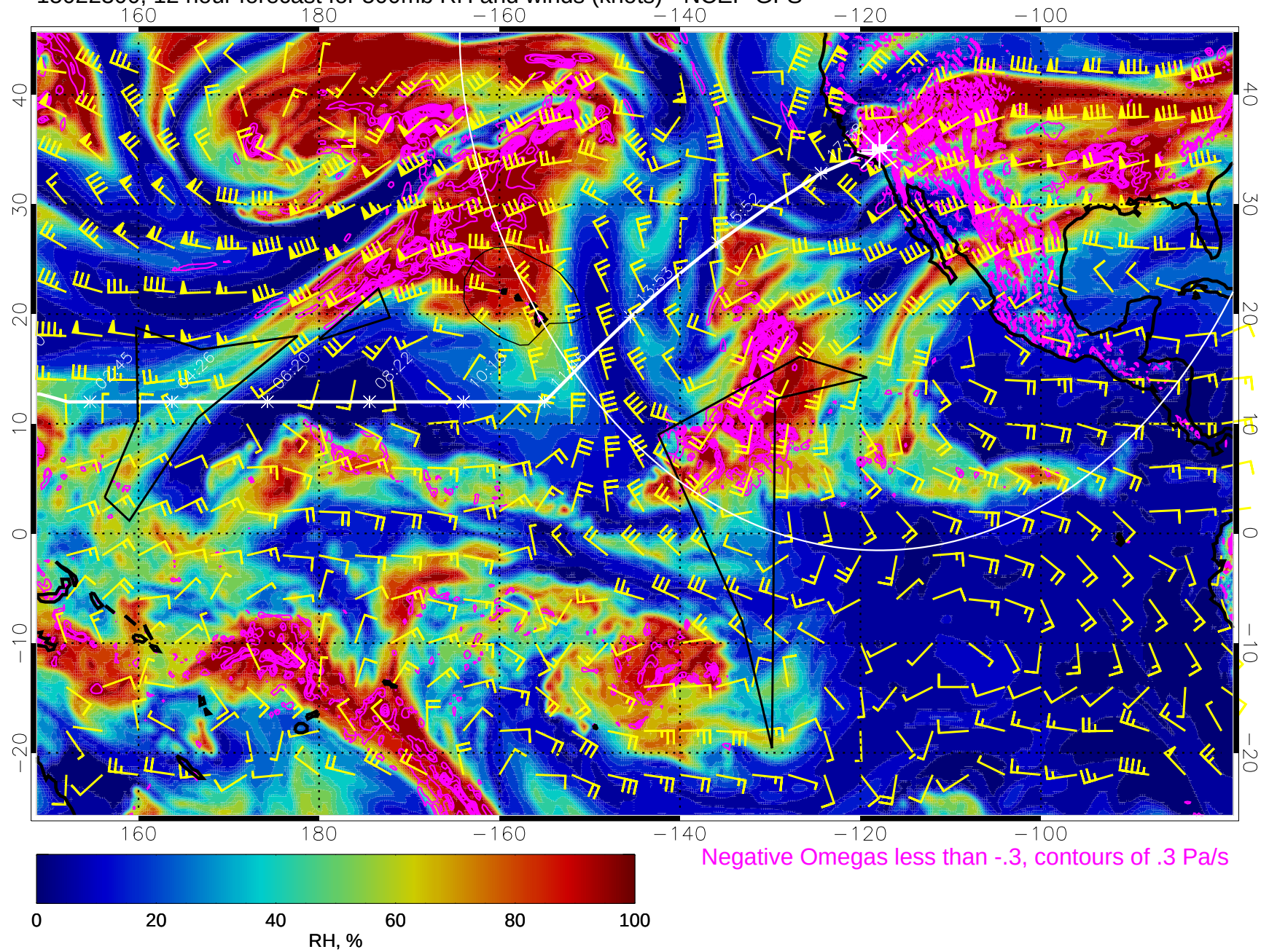
15022300, 12 hour forecast for 500mb RH and winds (knots) - NCEP GFS
