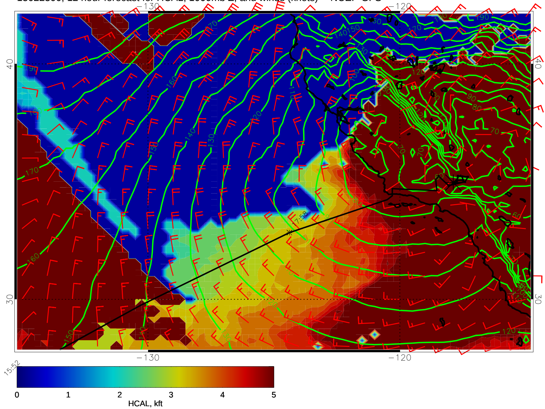
15022300, 12 hour forecast for HCAL, 1000mb Z, and winds (knots) -- NCEP GFS
