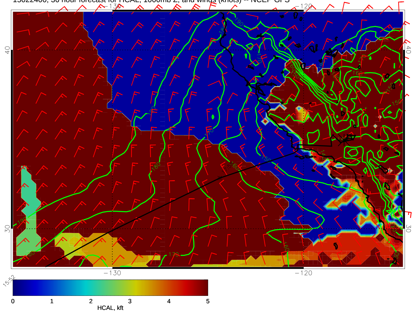
15022400, 36 hour forecast for HCAL, 1000mb Z, and winds (knots) -- NCEP GFS
