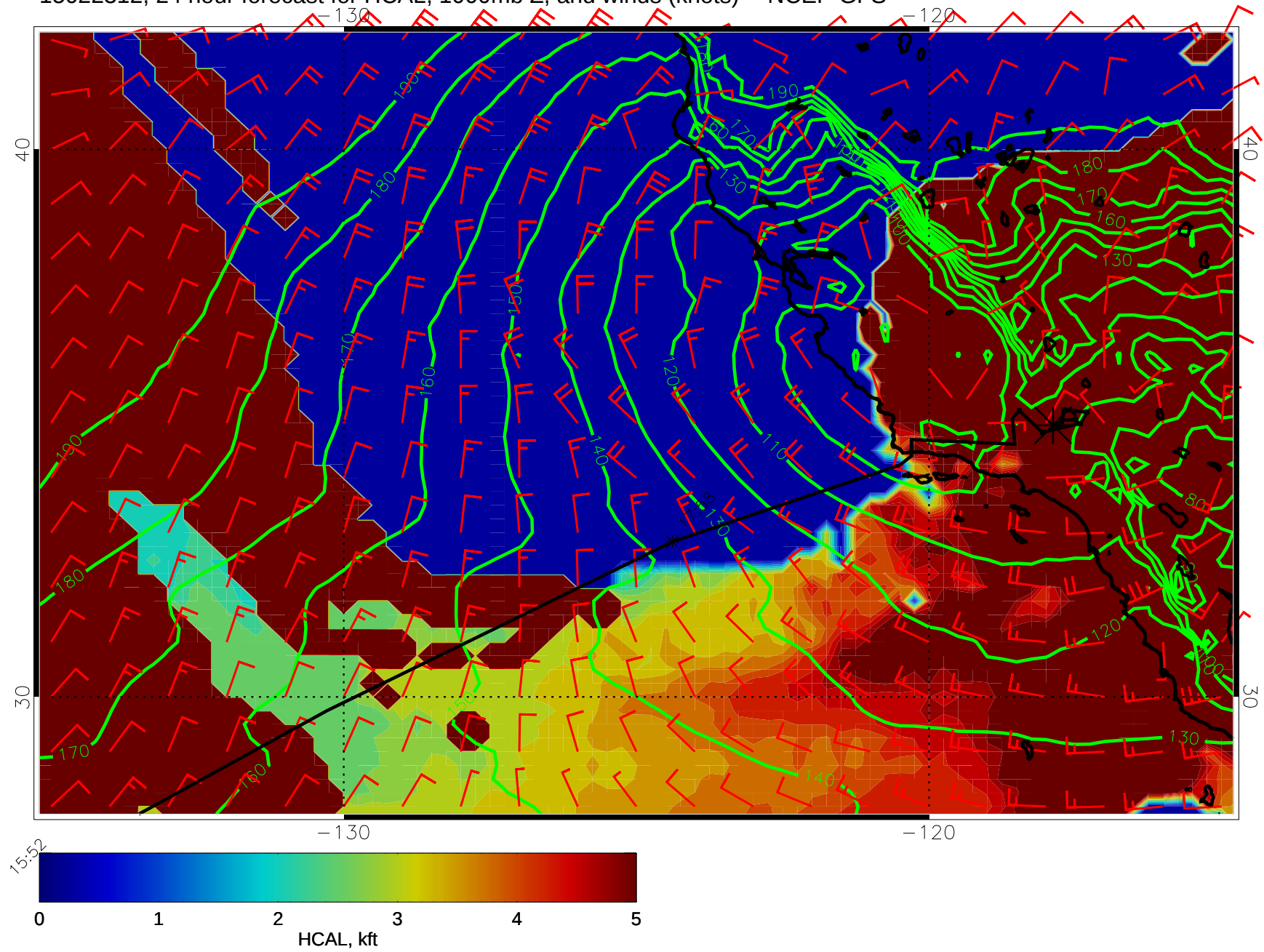
15022312, 24 hour forecast for HCAL, 1000mb Z, and winds (knots) -- NCEP GFS
