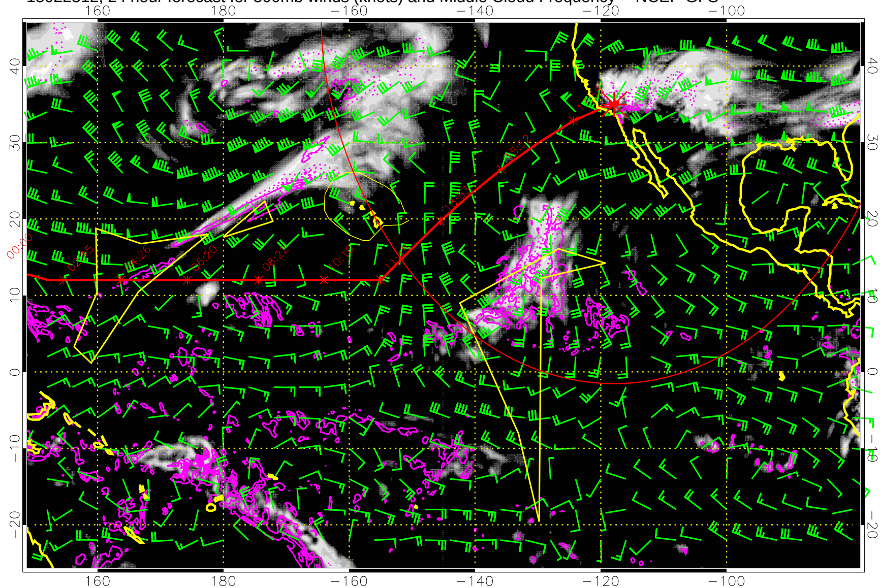
15022312, 24 hour forecast for 500mb winds (knots) and Middle Cloud Frequency -- NCEP GFS
