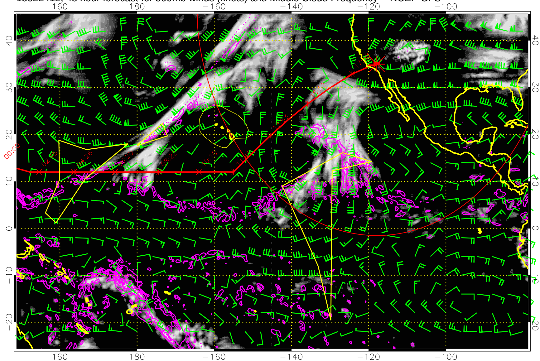
15022412, 48 hour forecast for 500mb winds (knots) and Middle Cloud Frequency -- NCEP GFS
