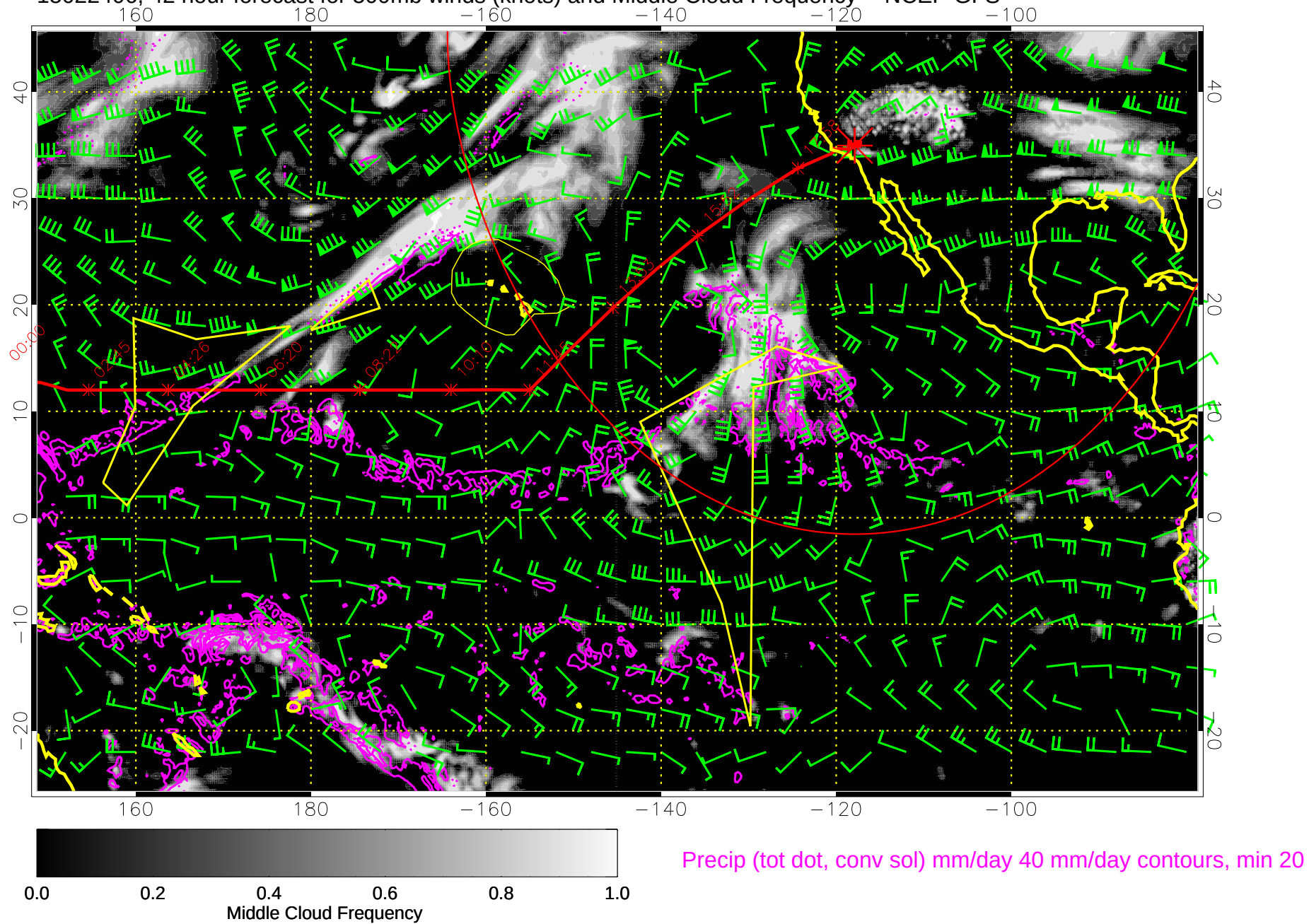
15022406, 42 hour forecast for 500mb winds (knots) and Middle Cloud Frequency -- NCEP GFS
