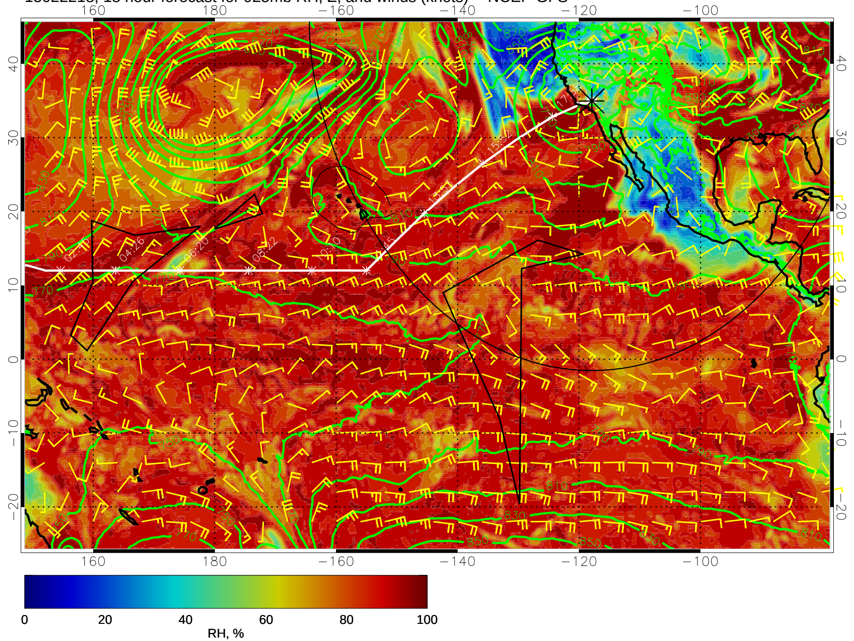
15022218, 18 hour forecast for 925mb RH, Z, and winds (knots) -- NCEP GFS
