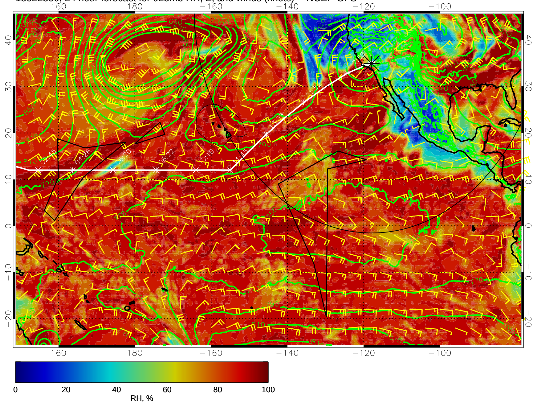
15022300, 24 hour forecast for 925mb RH, Z, and winds (knots) -- NCEP GFS
