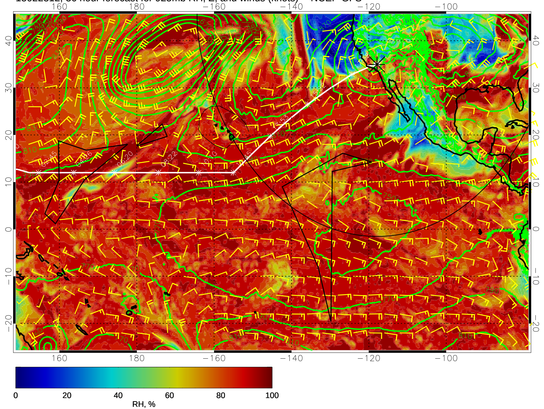
15022312, 36 hour forecast for 925mb RH, Z, and winds (knots) -- NCEP GFS
