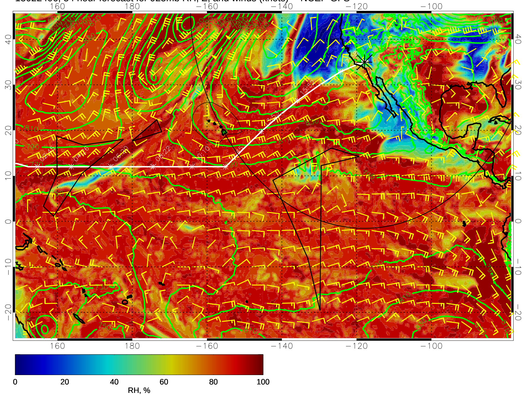
15022406, 54 hour forecast for 925mb RH, Z, and winds (knots) -- NCEP GFS
