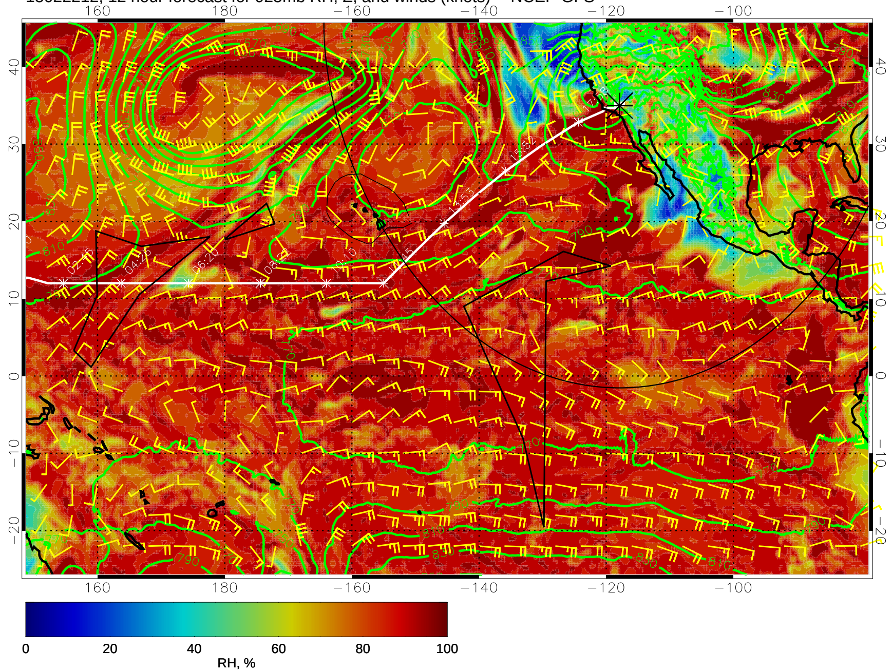
15022212, 12 hour forecast for 925mb RH, Z, and winds (knots) -- NCEP GFS
