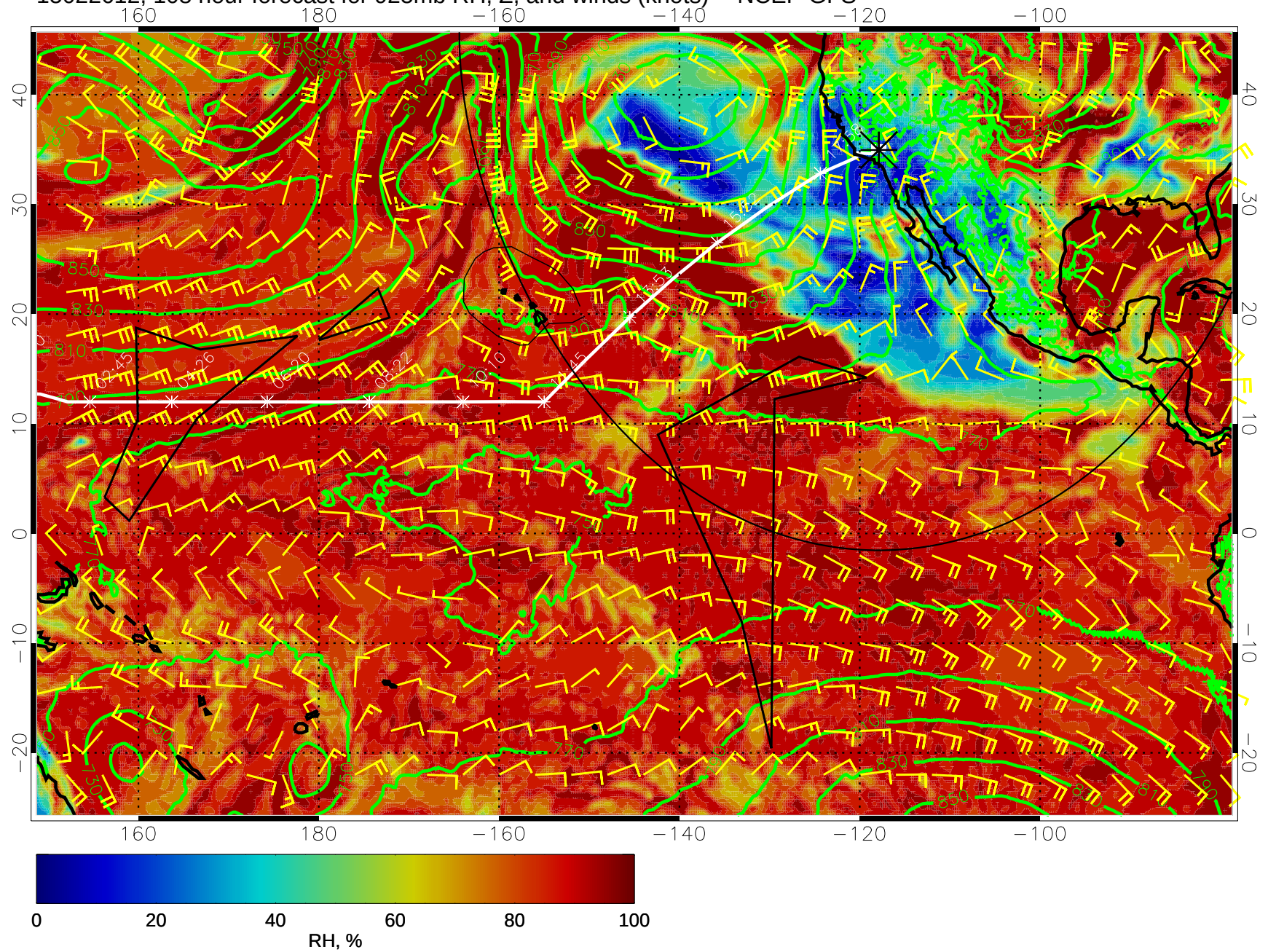
15022612, 108 hour forecast for 925mb RH, Z, and winds (knots) -- NCEP GFS
