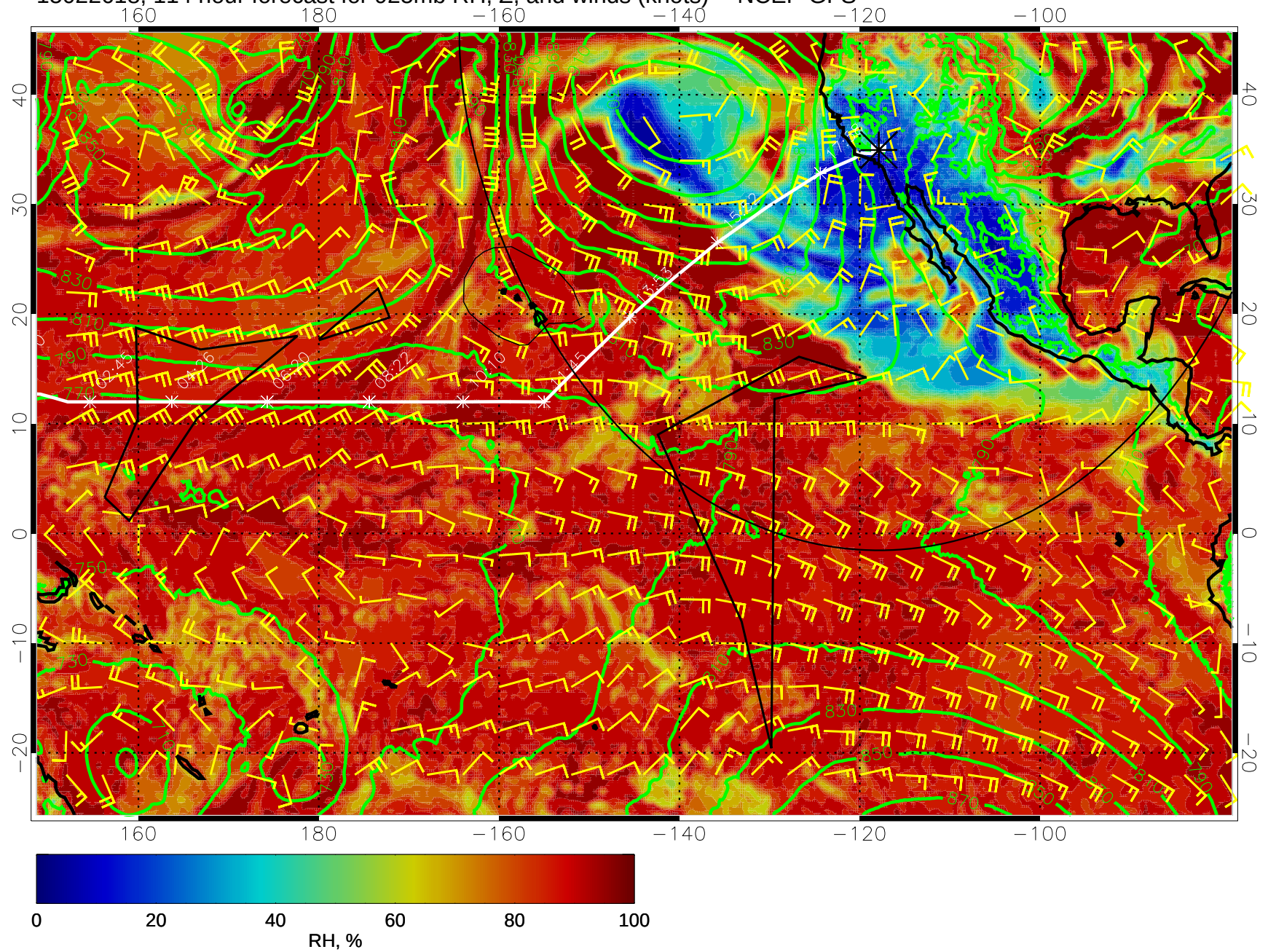
15022618, 114 hour forecast for 925mb RH, Z, and winds (knots) -- NCEP GFS
