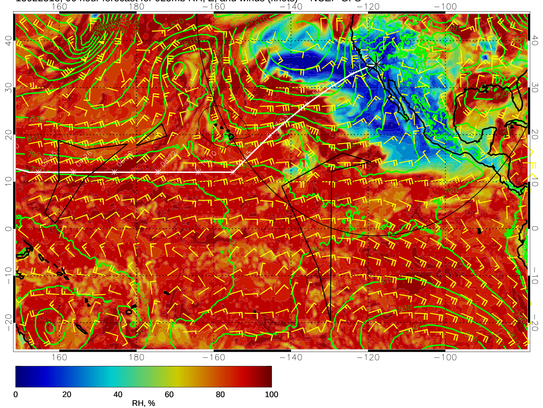
15022518, 90 hour forecast for 925mb RH, Z, and winds (knots) -- NCEP GFS
