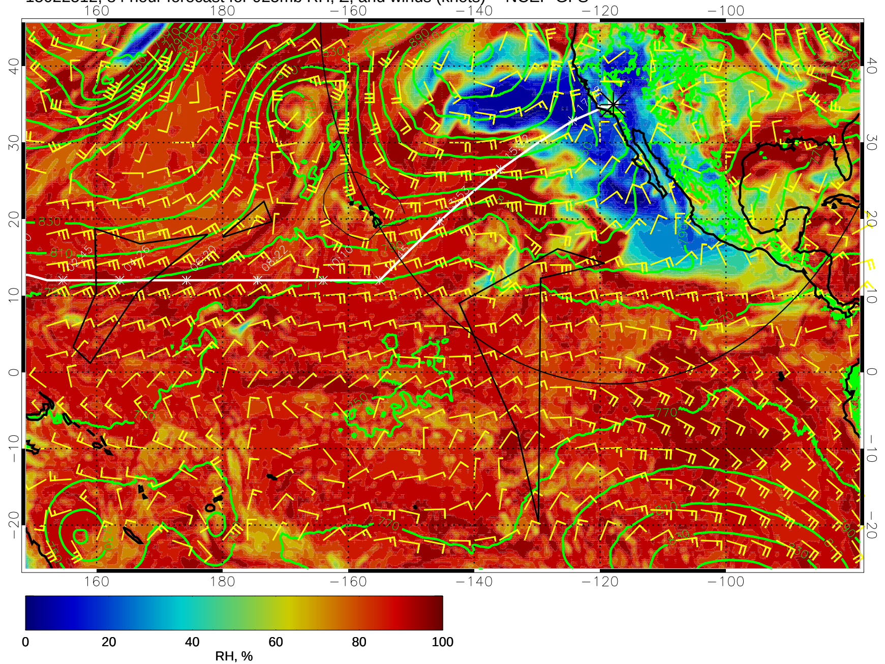
15022512, 84 hour forecast for 925mb RH, Z, and winds (knots) -- NCEP GFS
