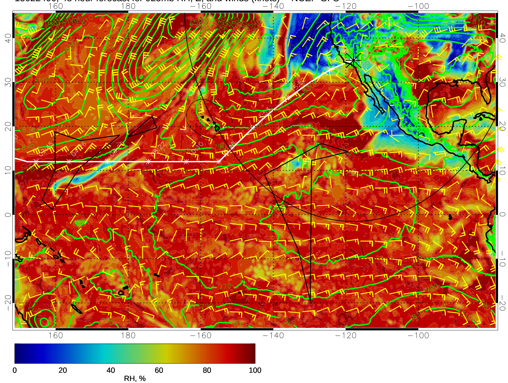
15022400, 48 hour forecast for 925mb RH, Z, and winds (knots) -- NCEP GFS
