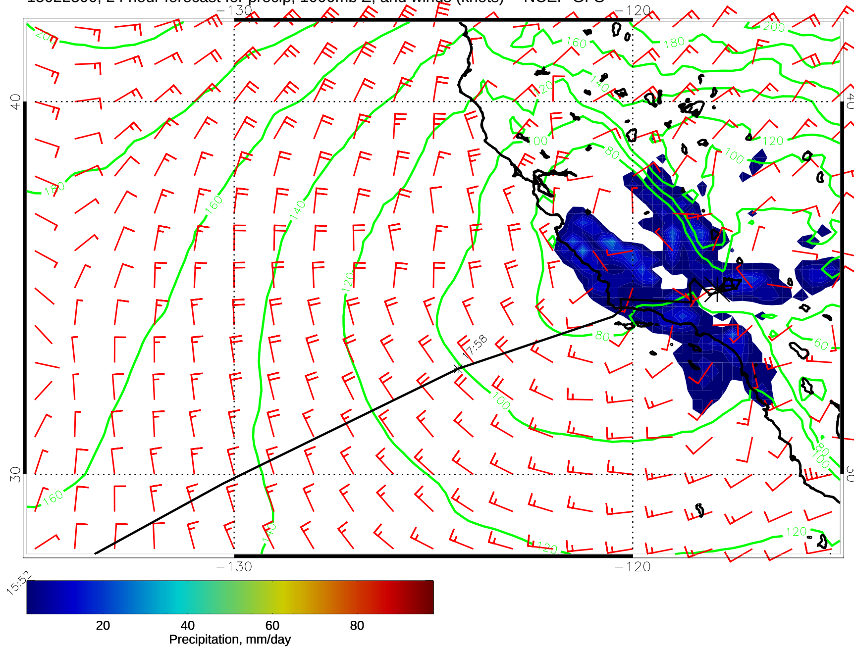
15022300, 24 hour forecast for precip, 1000mb Z, and winds (knots) -- NCEP GFS
