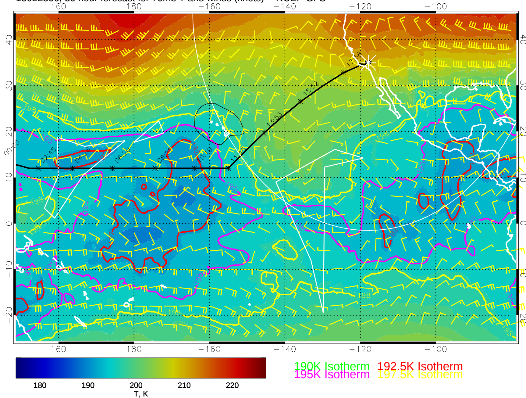
15022306, 30 hour forecast for 70mb T and winds (knots) -- NCEP GFS
