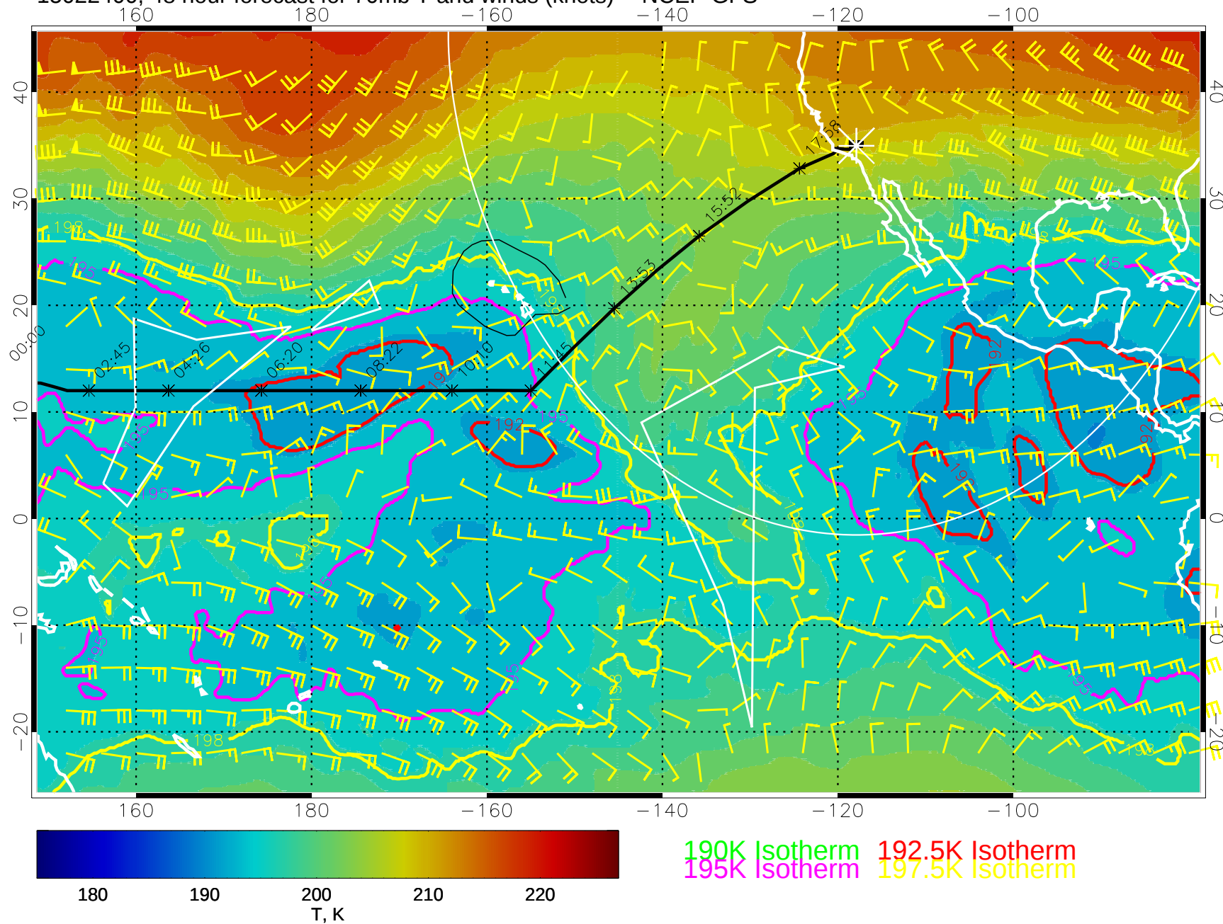
15022400, 48 hour forecast for 70mb T and winds (knots) -- NCEP GFS
