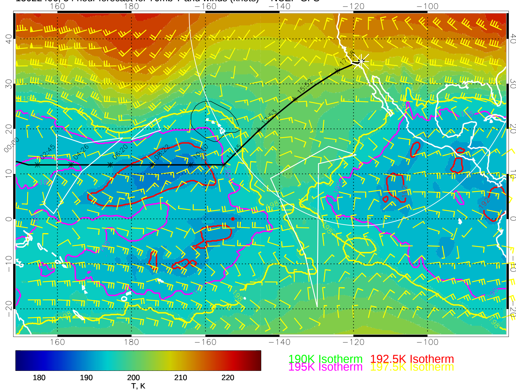
15022406, 54 hour forecast for 70mb T and winds (knots) -- NCEP GFS
