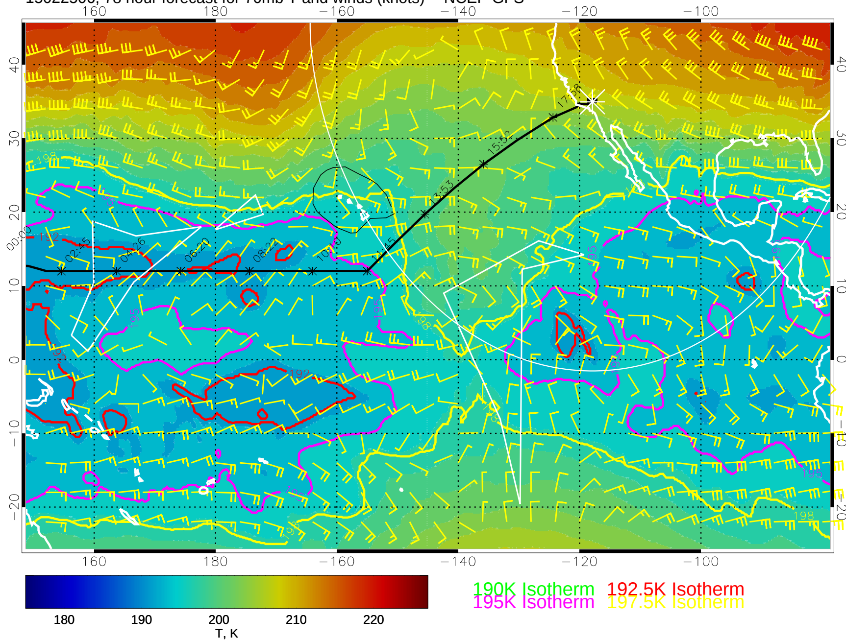
15022506, 78 hour forecast for 70mb T and winds (knots) -- NCEP GFS
