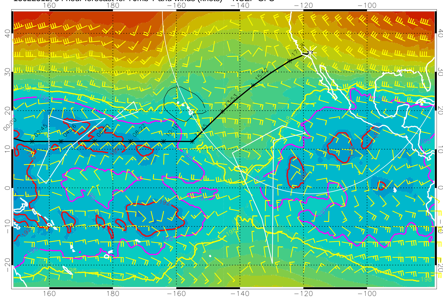
15022512, 84 hour forecast for 70mb T and winds (knots) -- NCEP GFS
