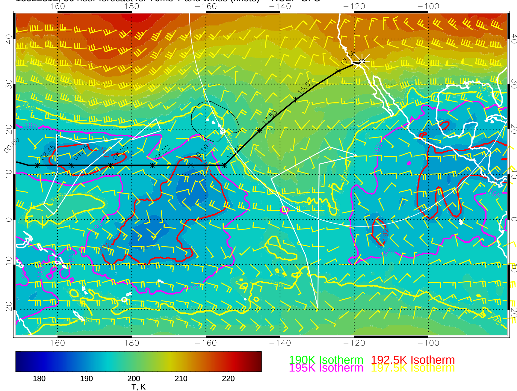
15022312, 36 hour forecast for 70mb T and winds (knots) -- NCEP GFS
