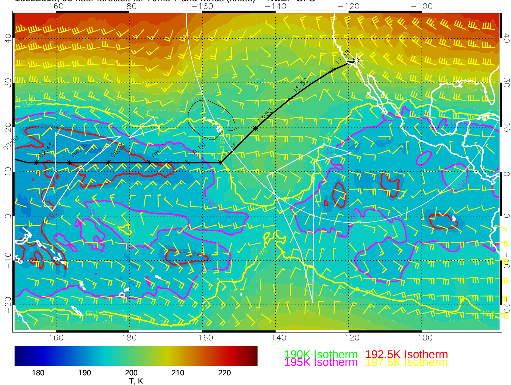
15022518, 90 hour forecast for 70mb T and winds (knots) -- NCEP GFS
