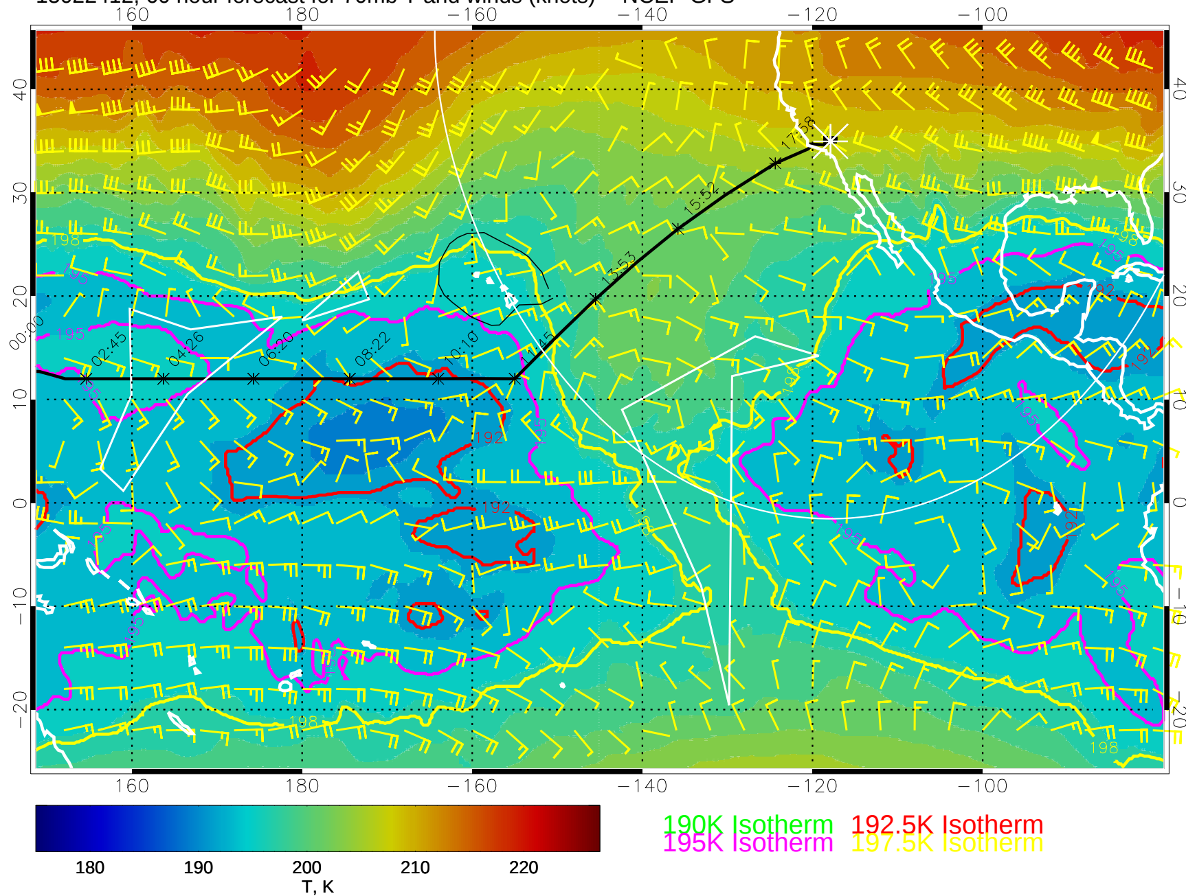
15022412, 60 hour forecast for 70mb T and winds (knots) -- NCEP GFS
