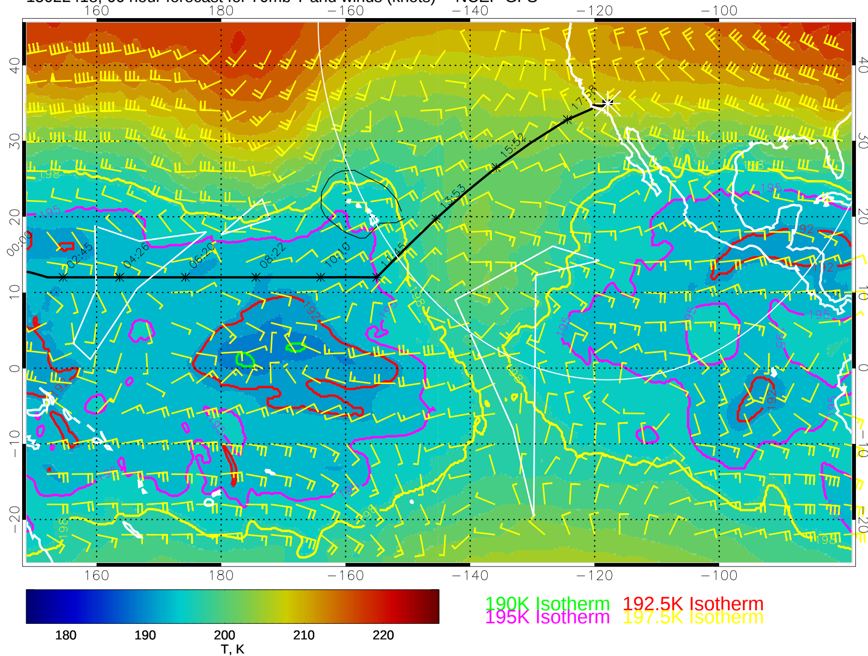
15022418, 66 hour forecast for 70mb T and winds (knots) -- NCEP GFS
