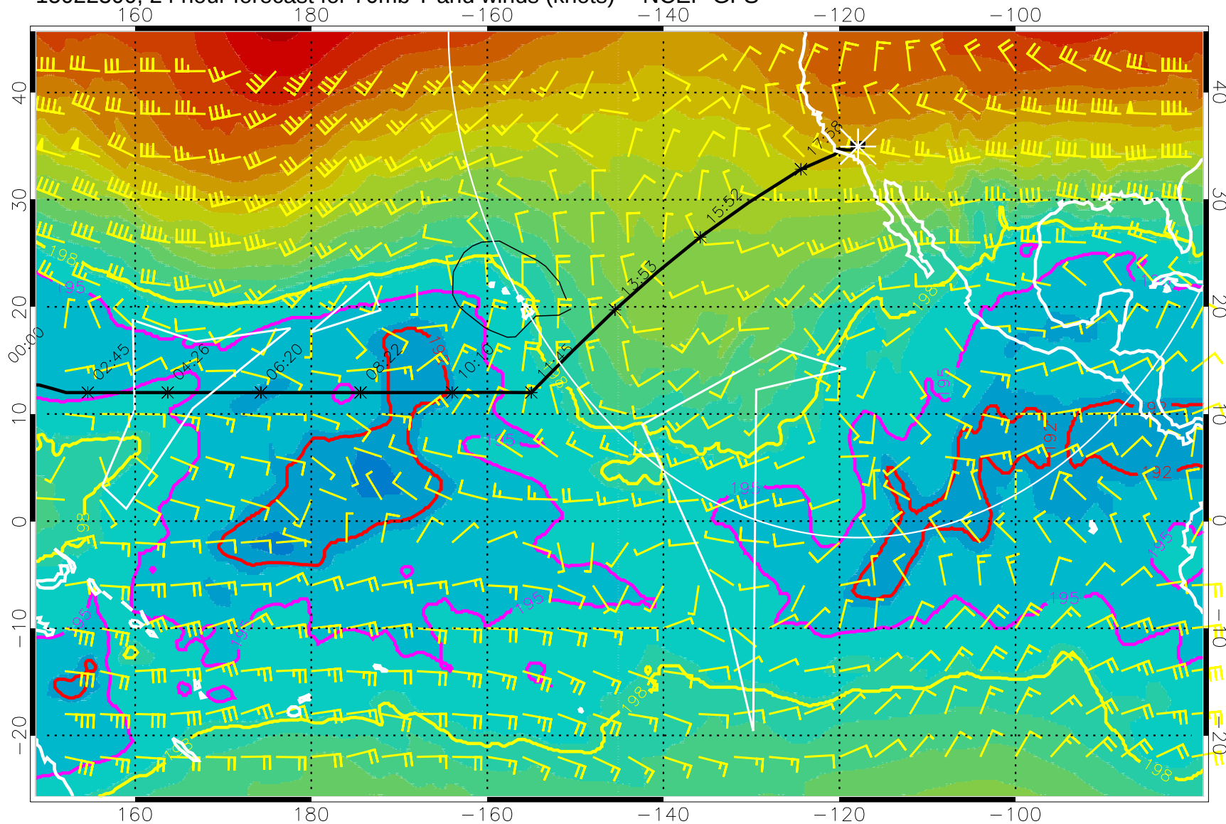
15022300, 24 hour forecast for 70mb T and winds (knots) -- NCEP GFS
