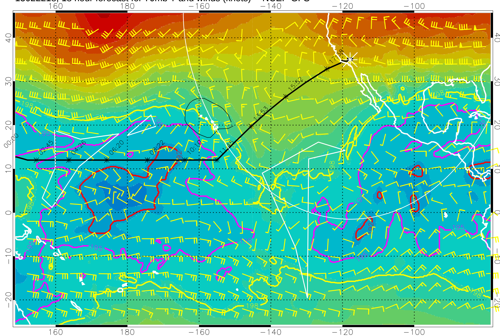
15022218, 18 hour forecast for 70mb T and winds (knots) -- NCEP GFS
