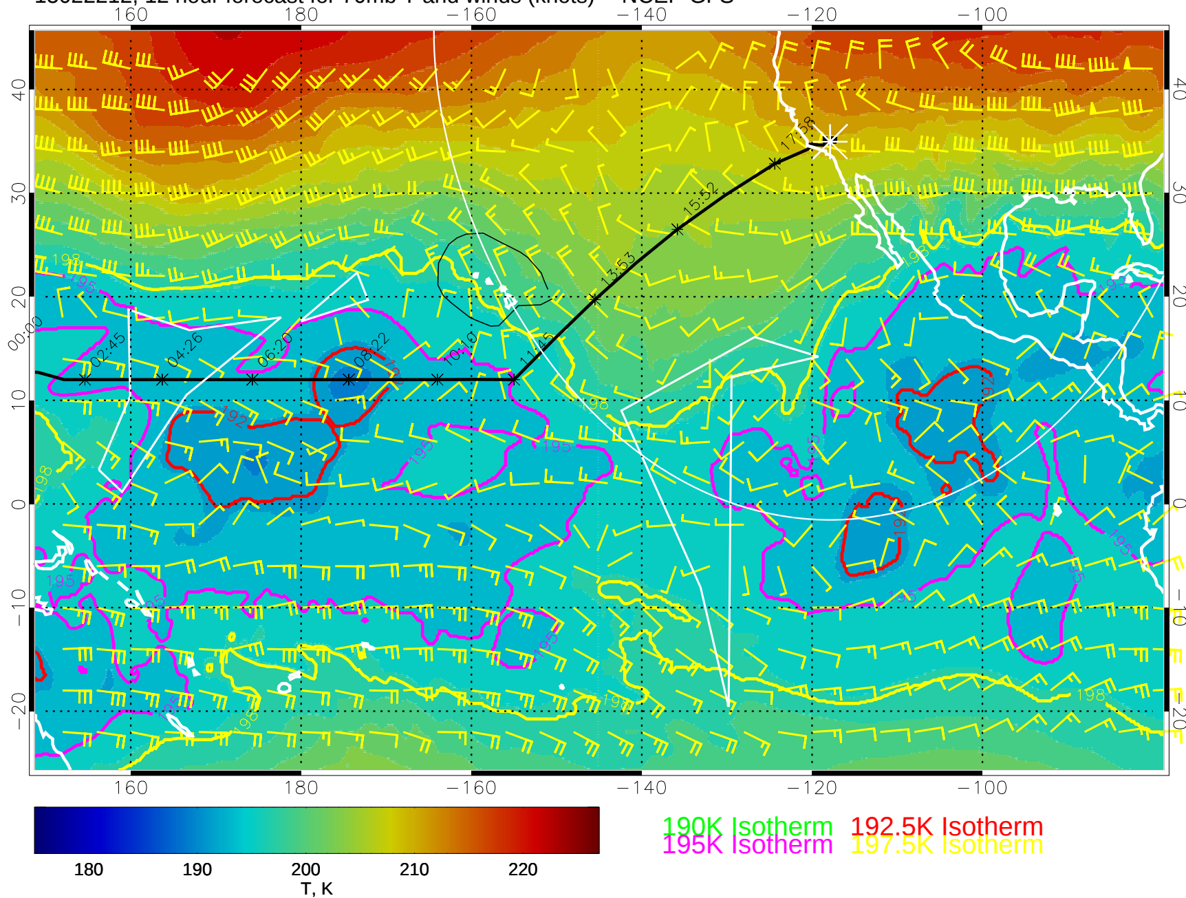
15022212, 12 hour forecast for 70mb T and winds (knots) -- NCEP GFS
