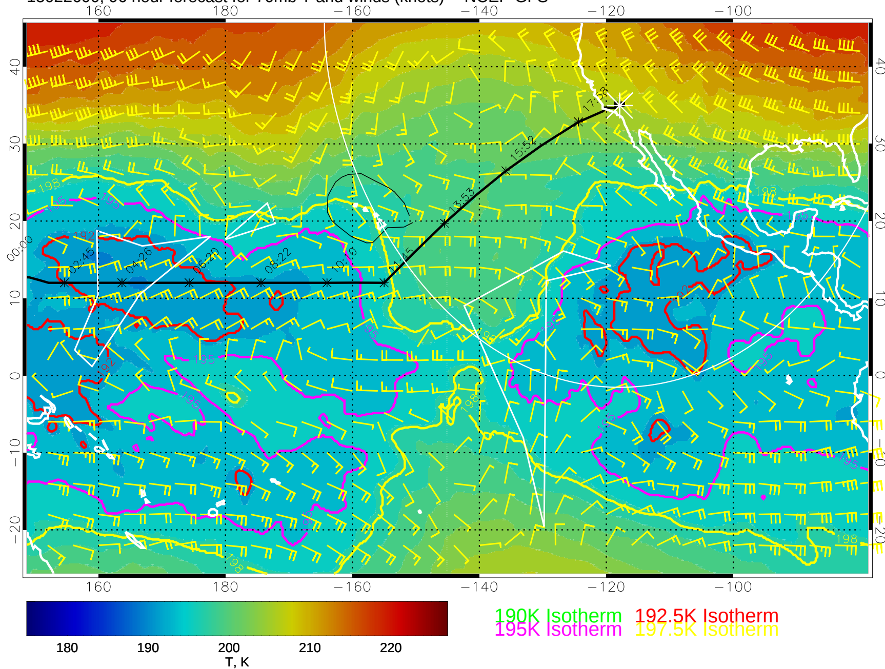
15022600, 96 hour forecast for 70mb T and winds (knots) -- NCEP GFS
