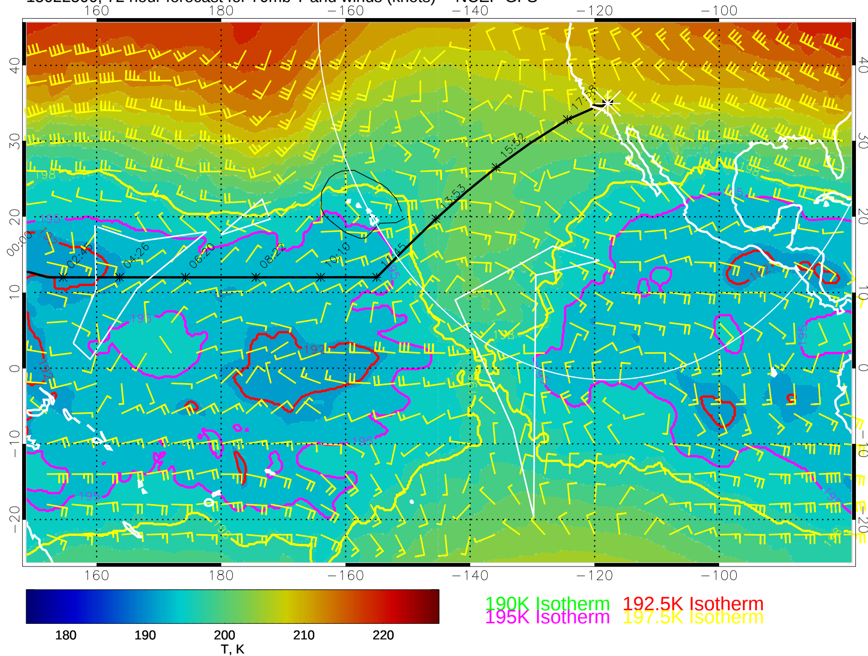
15022500, 72 hour forecast for 70mb T and winds (knots) -- NCEP GFS
