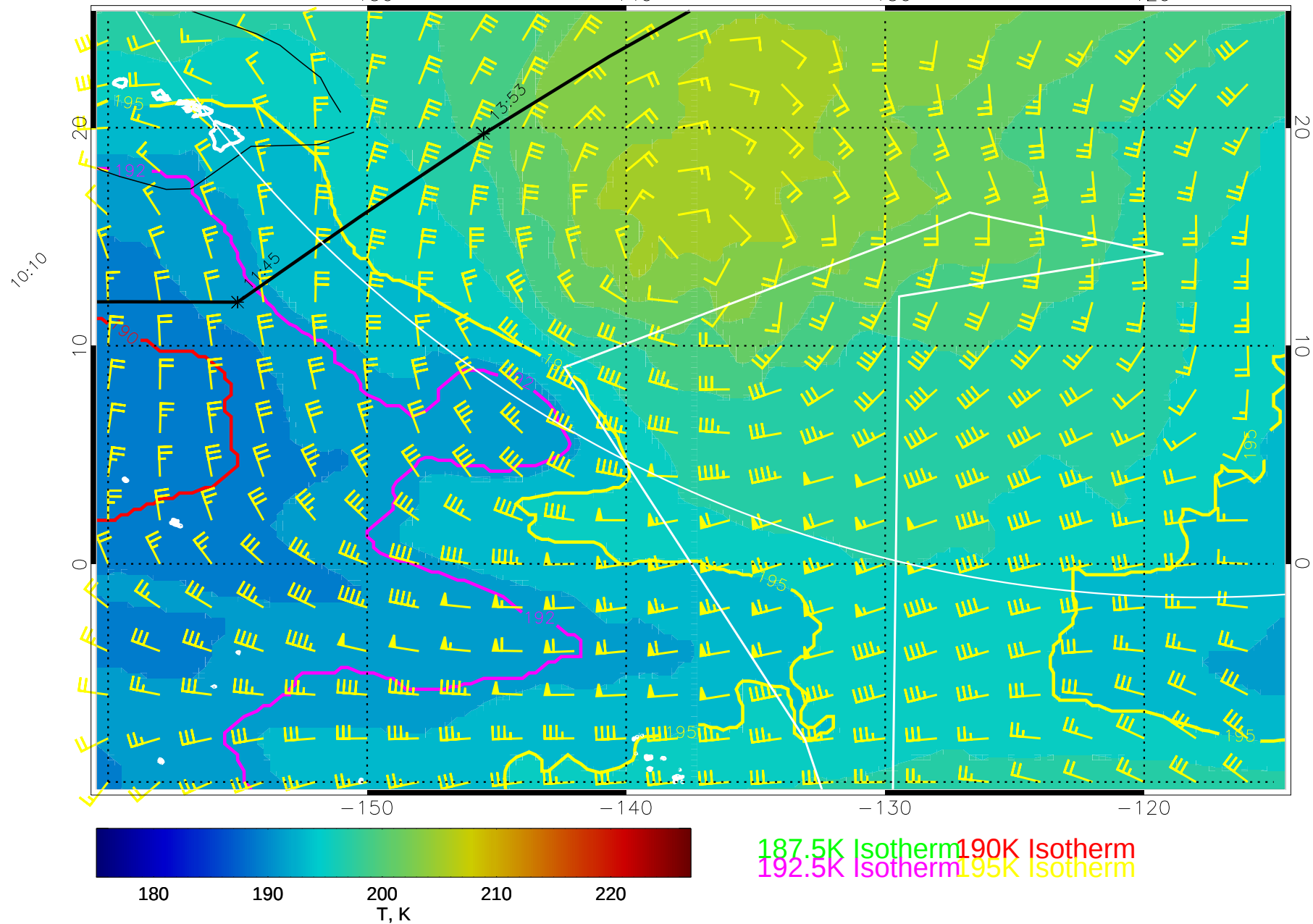
15022500, 72 hour forecast for 100mb T and winds (knots) -- NCEP GFS
