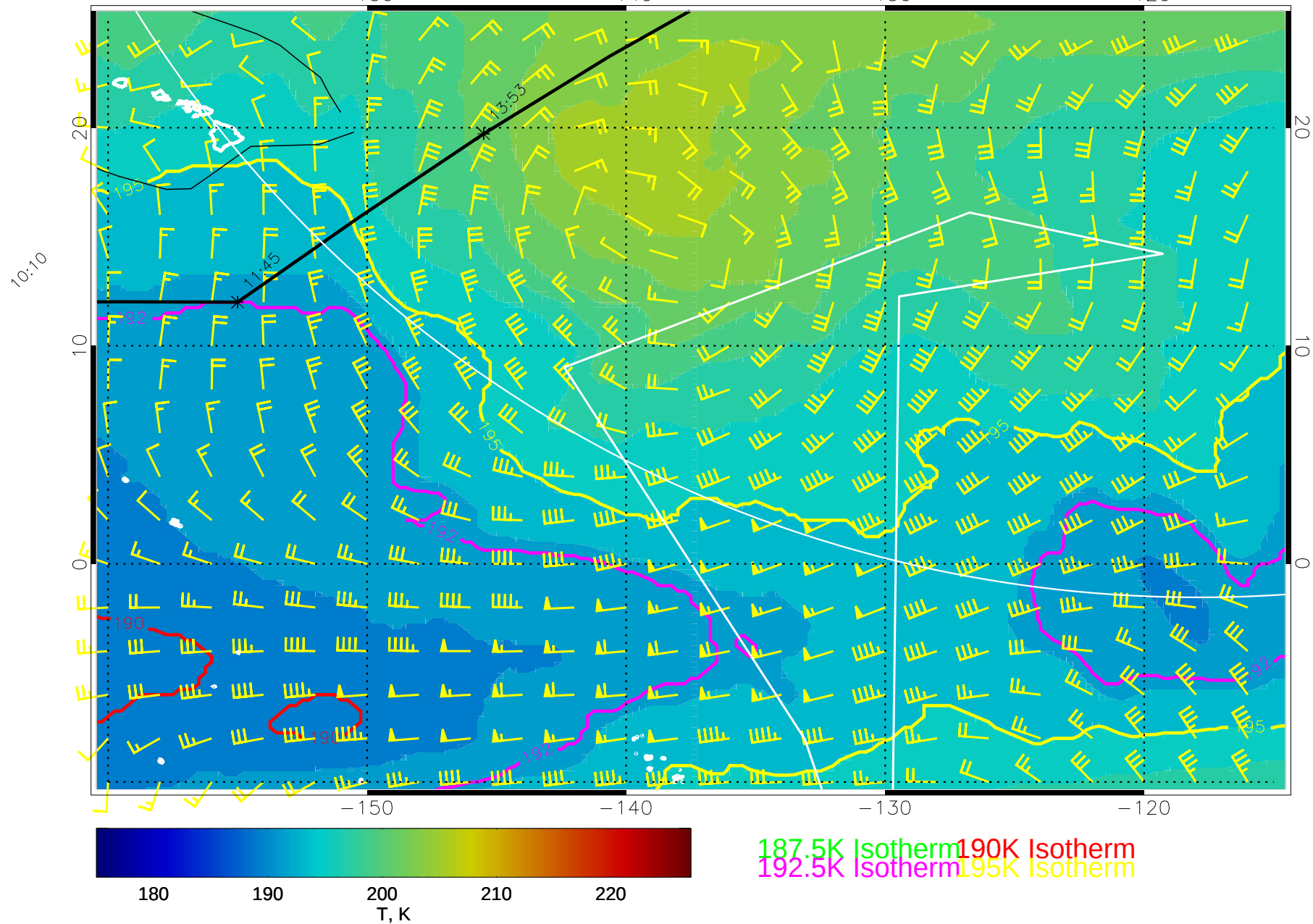
15022600, 96 hour forecast for 100mb T and winds (knots) -- NCEP GFS
