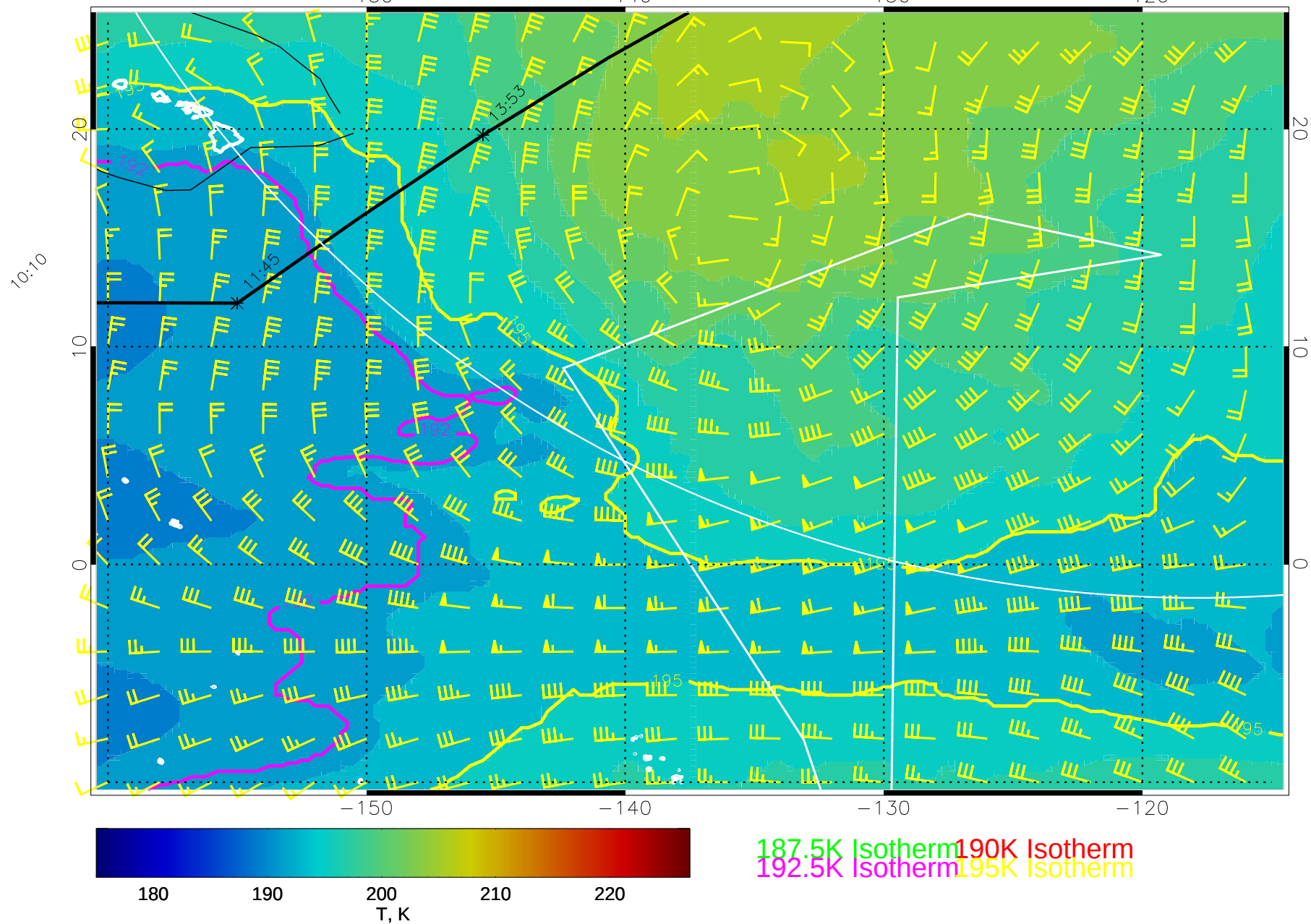
15022412, 60 hour forecast for 100mb T and winds (knots) -- NCEP GFS
