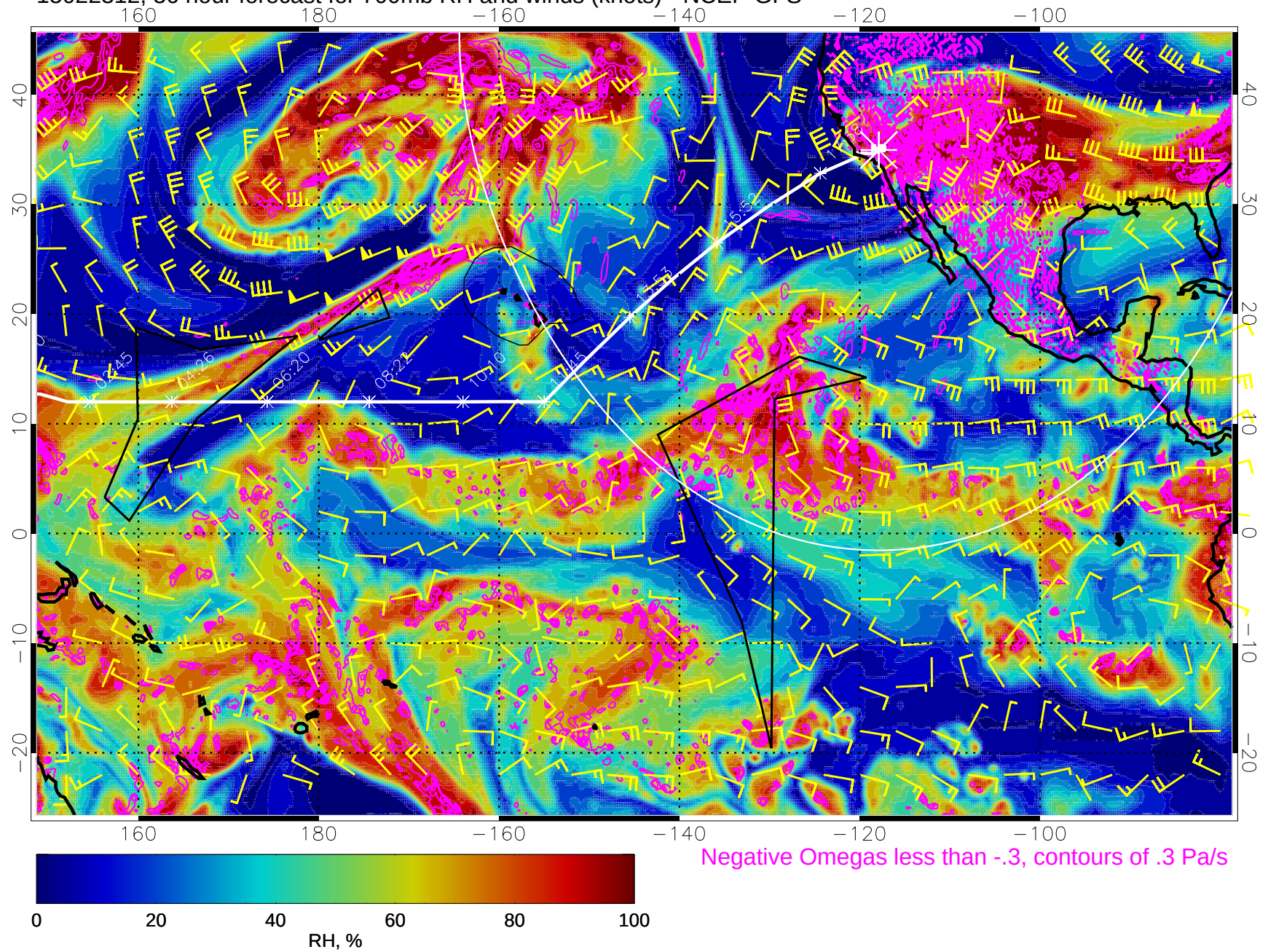
15022312, 36 hour forecast for 700mb RH and winds (knots) - NCEP GFS
