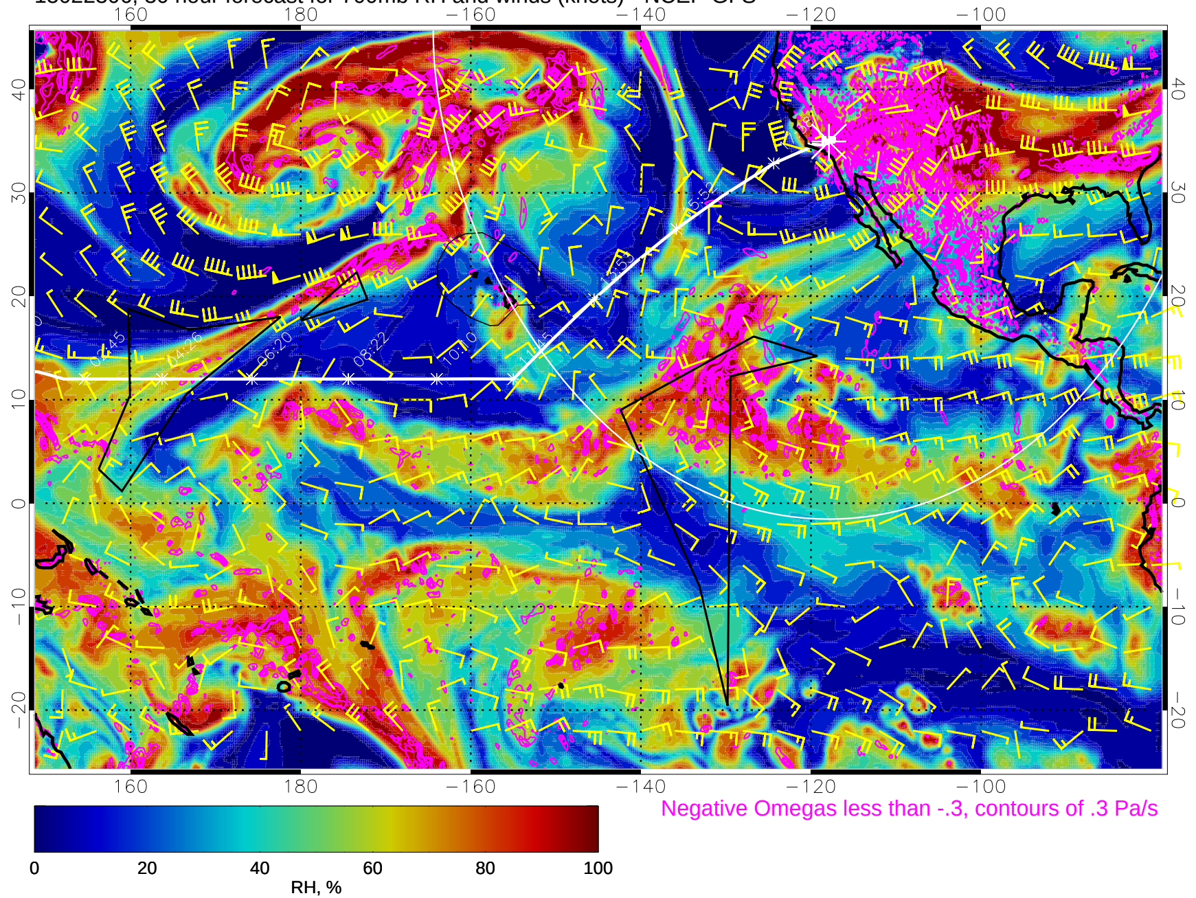
15022306, 30 hour forecast for 700mb RH and winds (knots) - NCEP GFS
