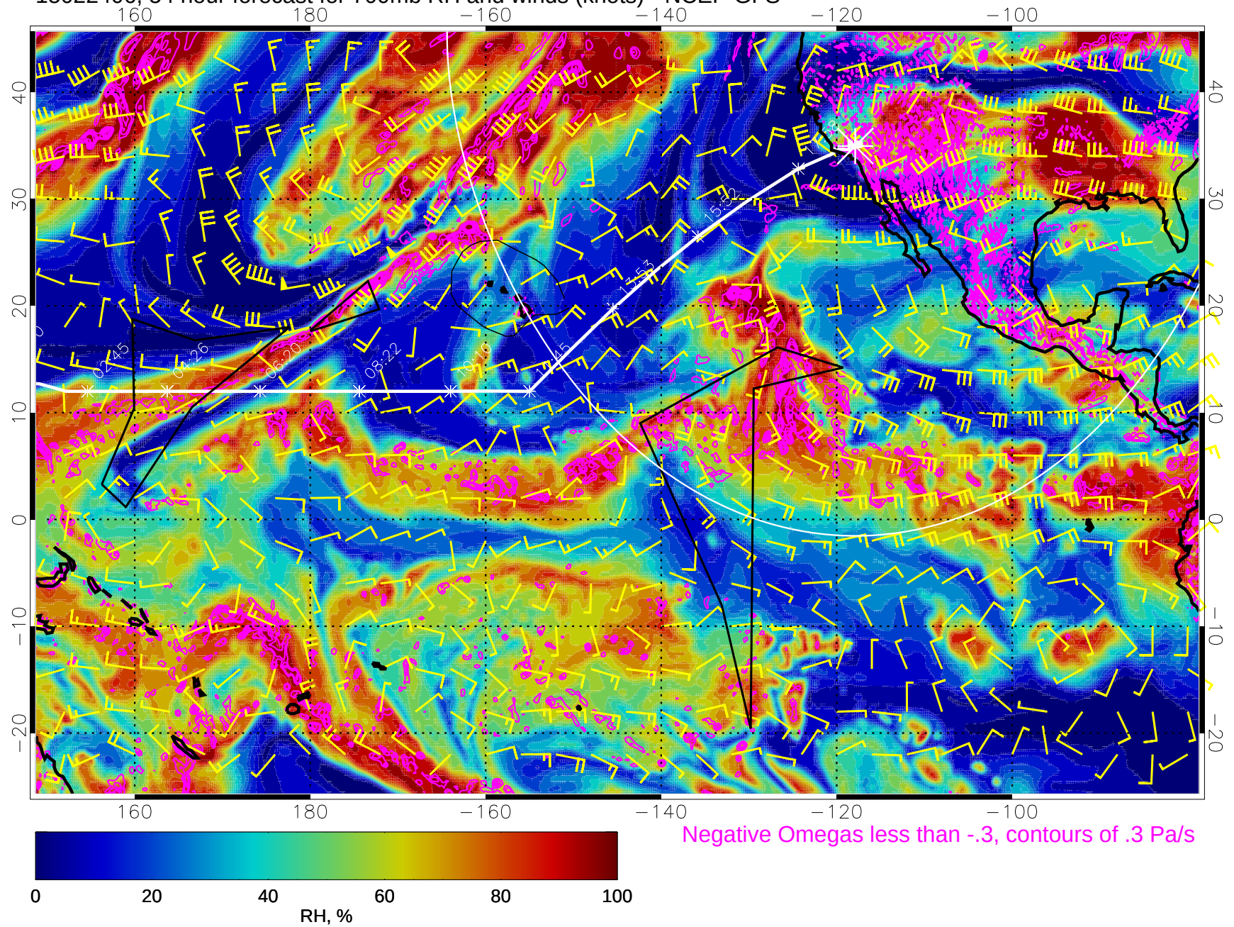
15022406, 54 hour forecast for 700mb RH and winds (knots) - NCEP GFS
