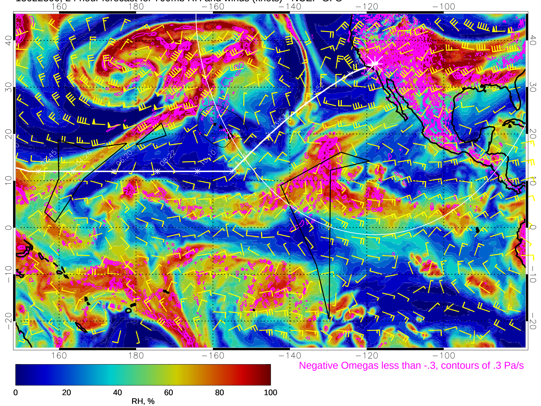
15022300, 24 hour forecast for 700mb RH and winds (knots) - NCEP GFS
