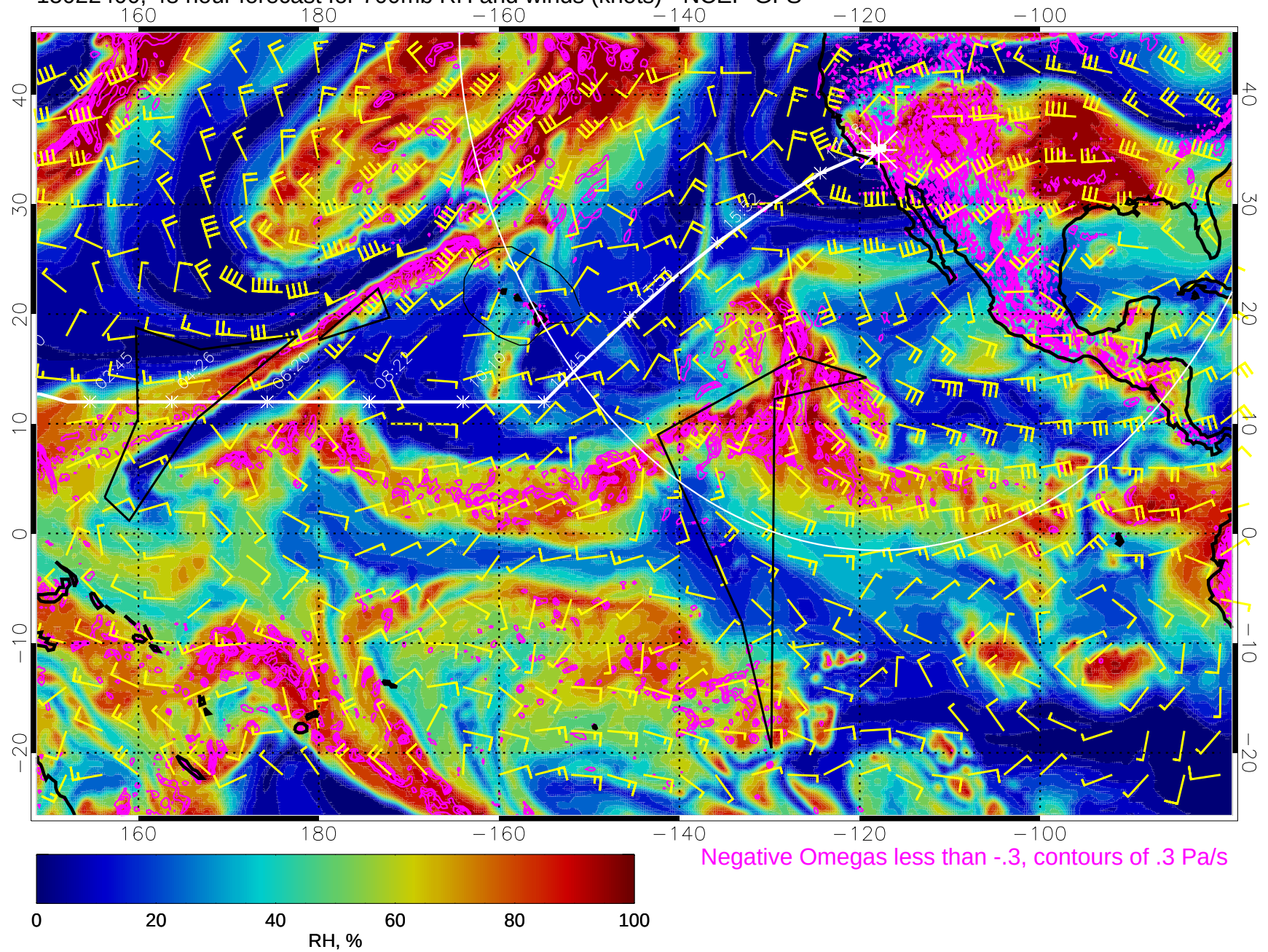
15022400, 48 hour forecast for 700mb RH and winds (knots) - NCEP GFS
