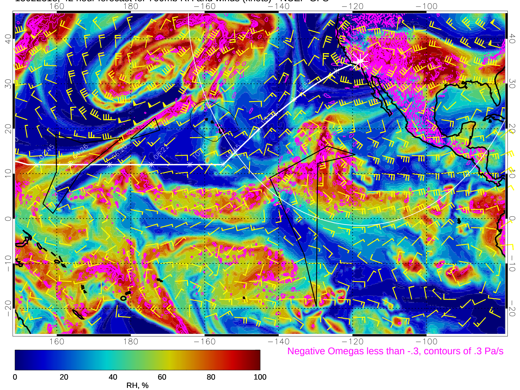
15022318, 42 hour forecast for 700mb RH and winds (knots) - NCEP GFS
