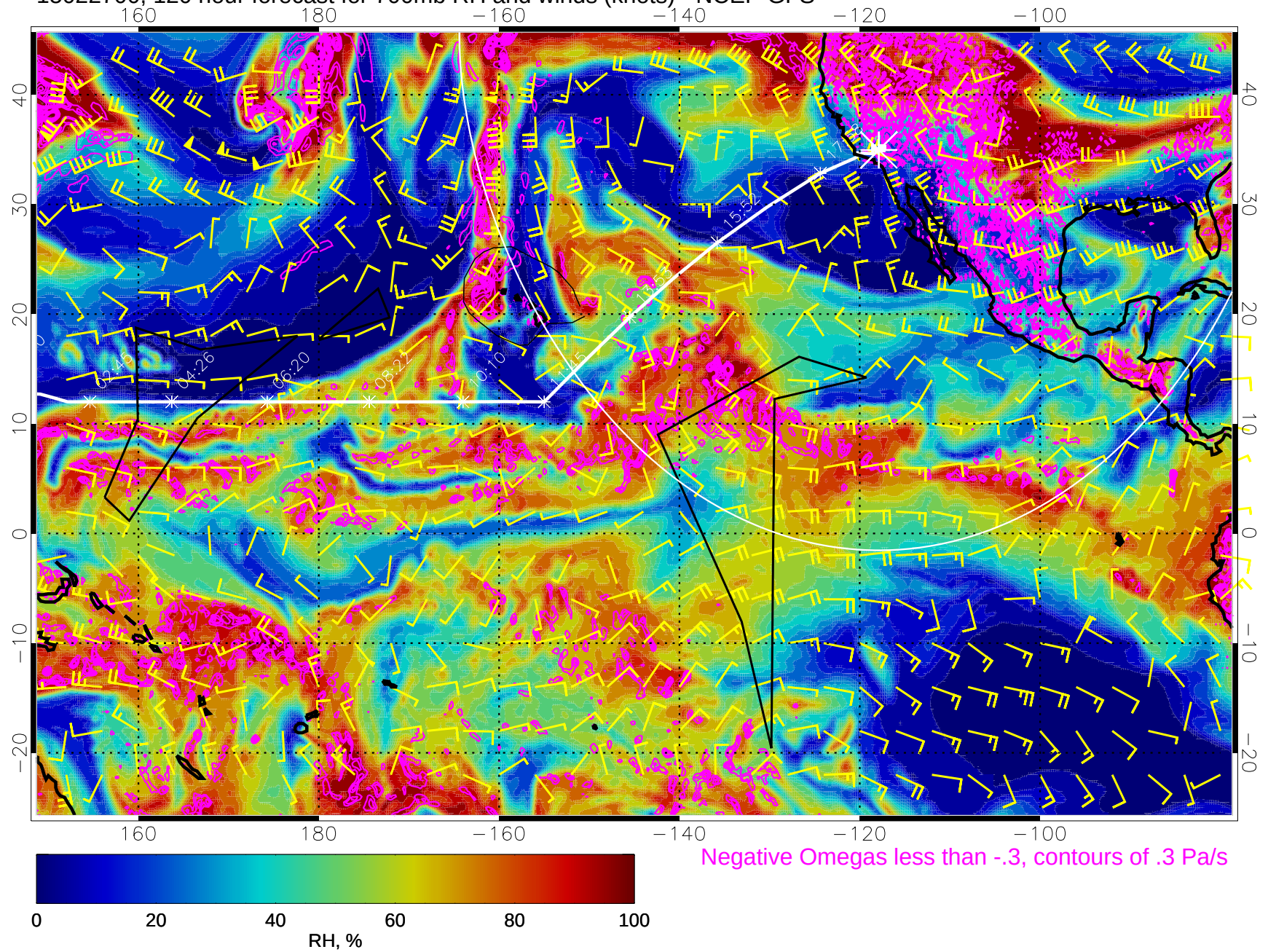
15022700, 120 hour forecast for 700mb RH and winds (knots) - NCEP GFS
