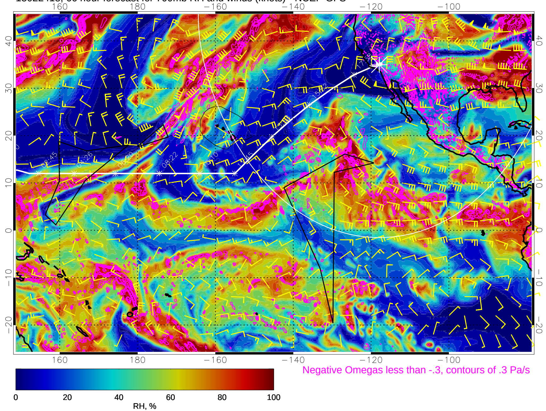
15022418, 66 hour forecast for 700mb RH and winds (knots) - NCEP GFS
