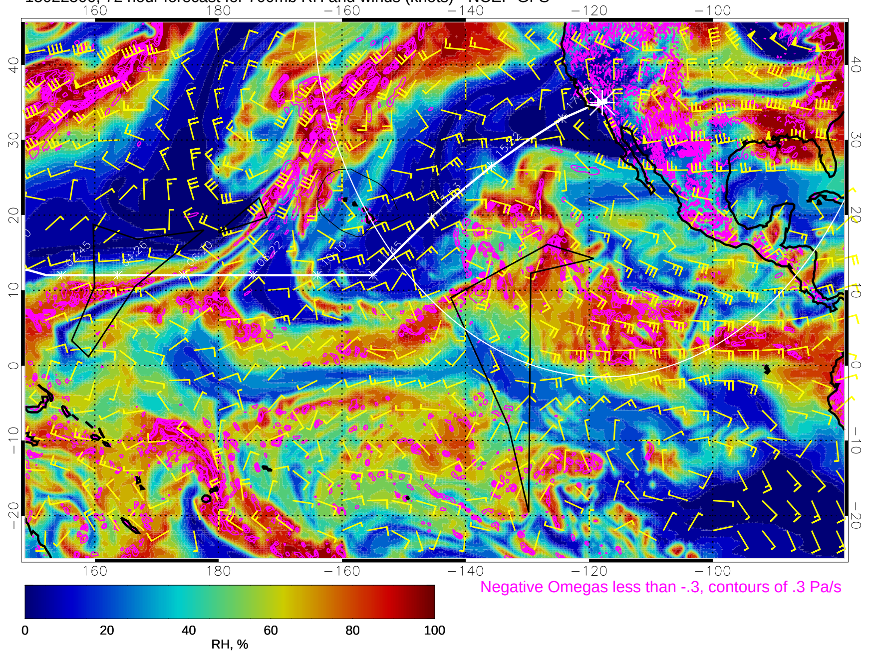
15022500, 72 hour forecast for 700mb RH and winds (knots) - NCEP GFS
