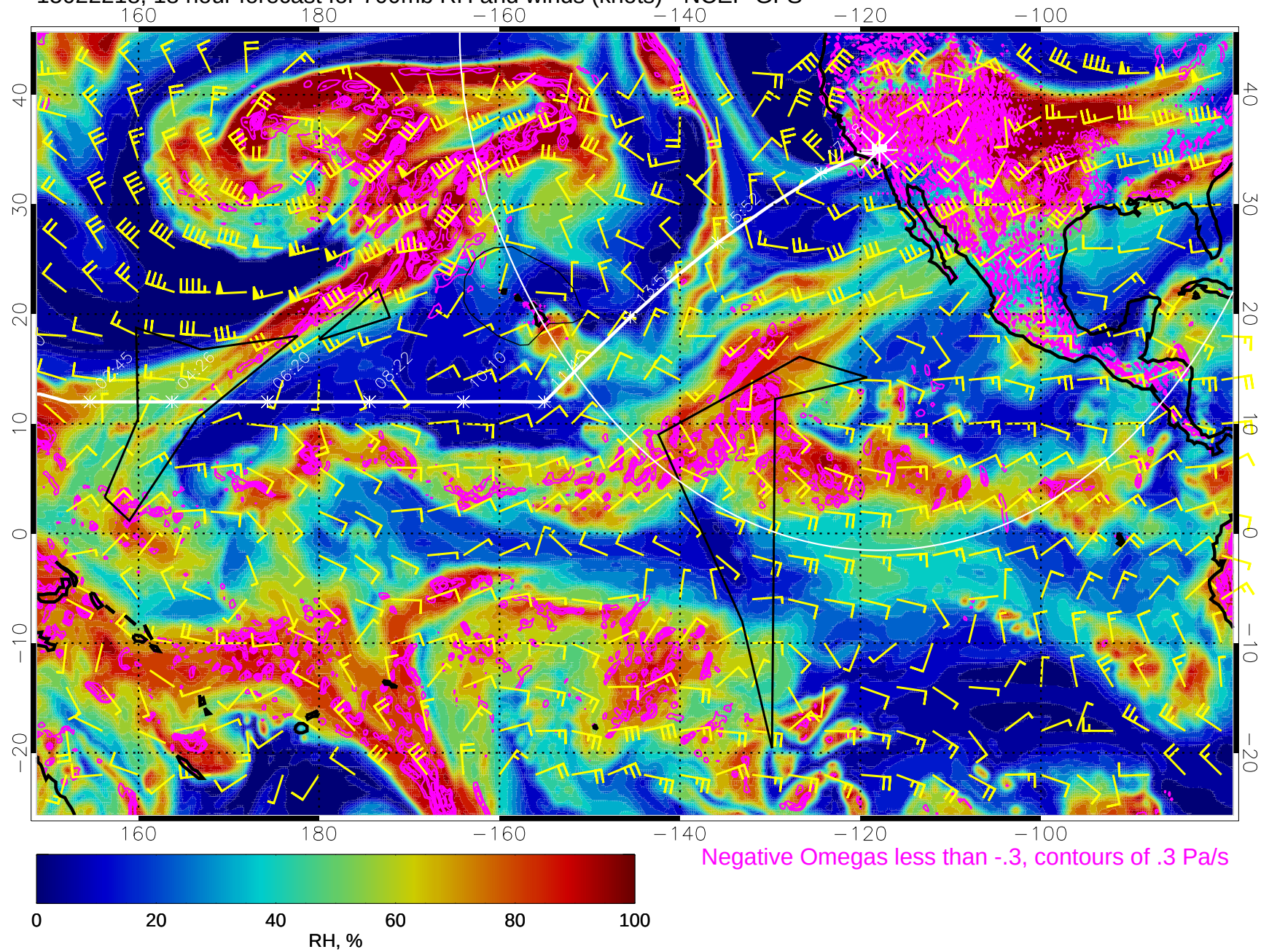
15022218, 18 hour forecast for 700mb RH and winds (knots) - NCEP GFS
