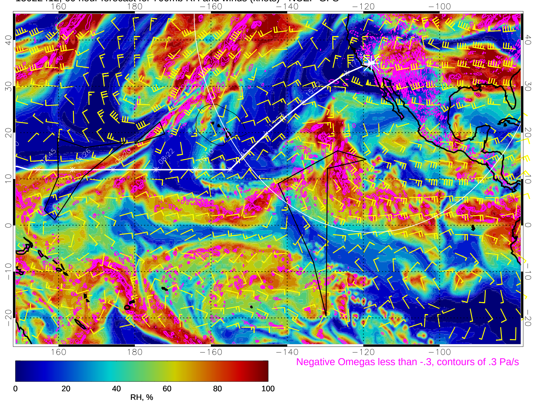
15022412, 60 hour forecast for 700mb RH and winds (knots) - NCEP GFS
