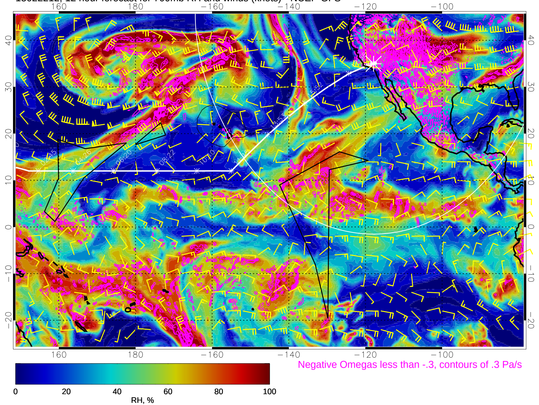
15022212, 12 hour forecast for 700mb RH and winds (knots) - NCEP GFS
