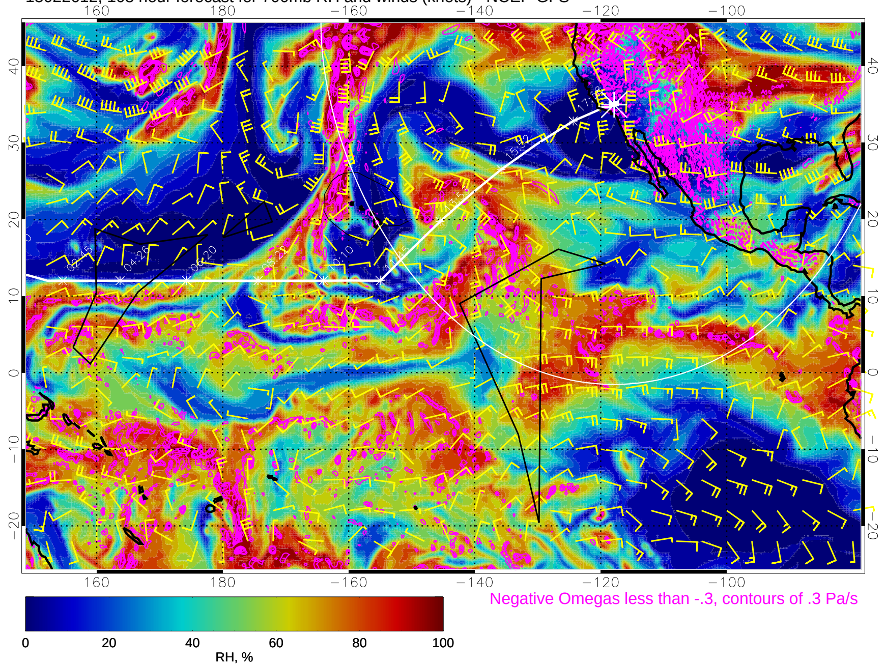
15022612, 108 hour forecast for 700mb RH and winds (knots) - NCEP GFS
