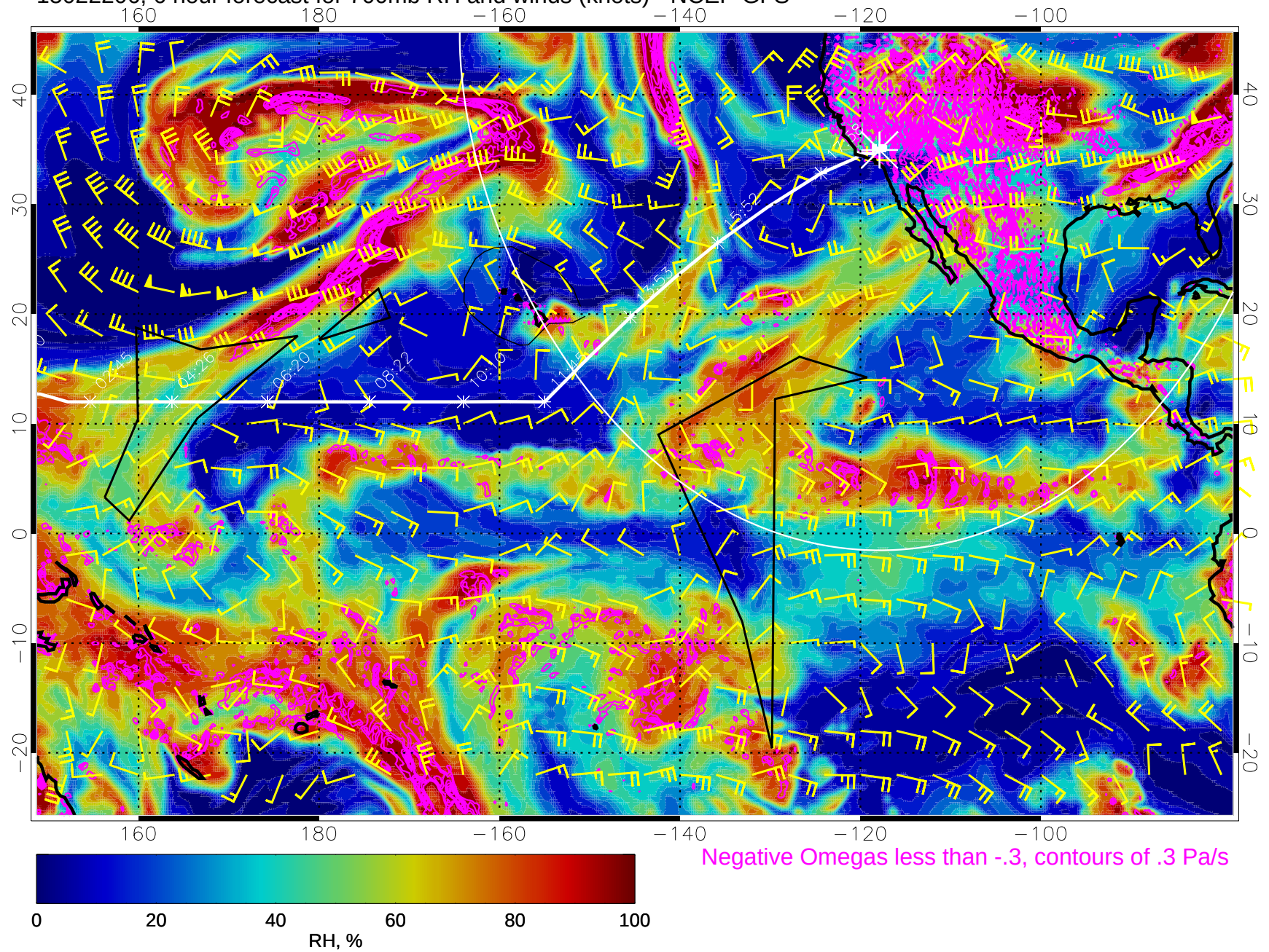
15022206, 6 hour forecast for 700mb RH and winds (knots) - NCEP GFS
