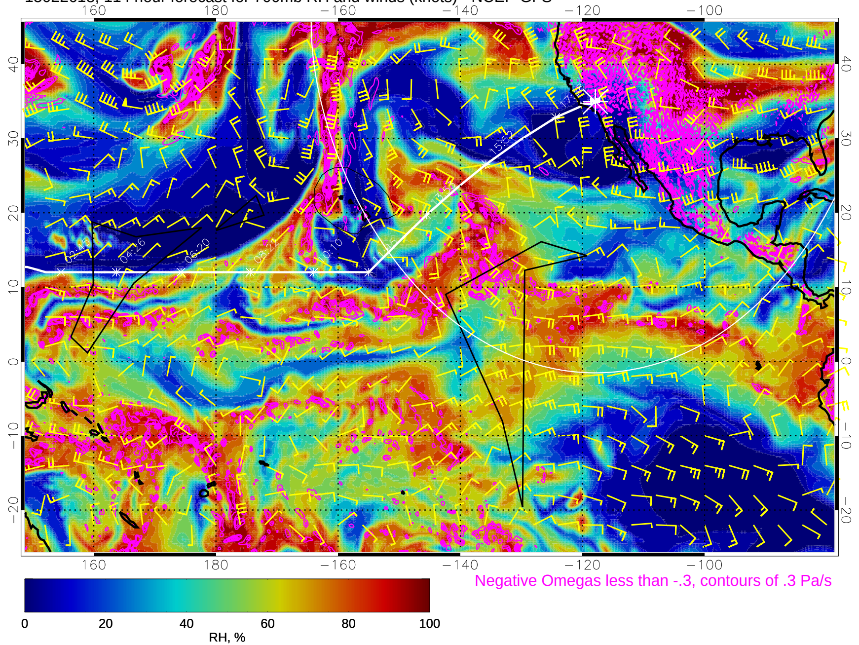
15022618, 114 hour forecast for 700mb RH and winds (knots) - NCEP GFS
